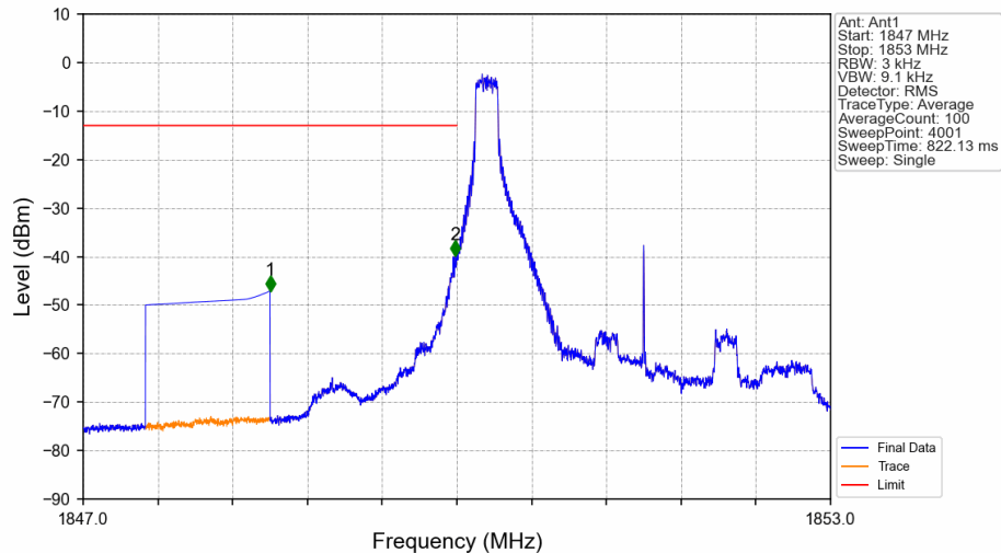
Band25_3MHz_QPSK_LCH_1851.5MHz_RB_1_0_NTNV
