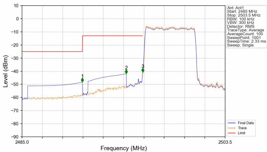
Band41_5MHz_16QAM_LCH_2498.5MHz_RB_25_0_NTNV
