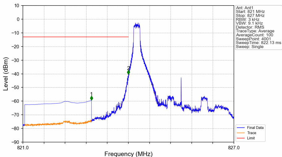
Band26b_3MHz_QPSK_LCH_825.5MHz_RB_1_0_NTNV
