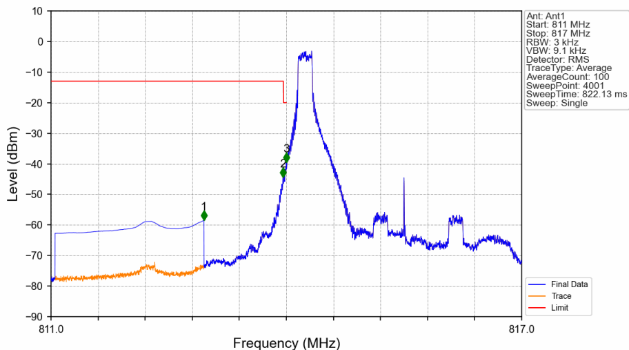
Band26a_3MHz_QPSK_LCH_815.5MHz_RB_1_0_NTNV
