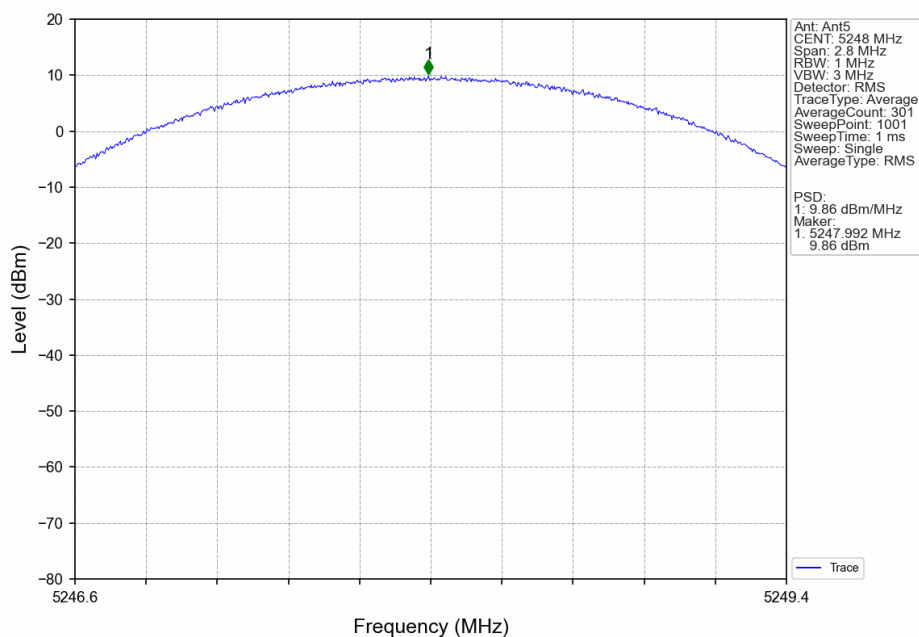
1.4M_HCH_5248MHz_Ant5_NTNV
