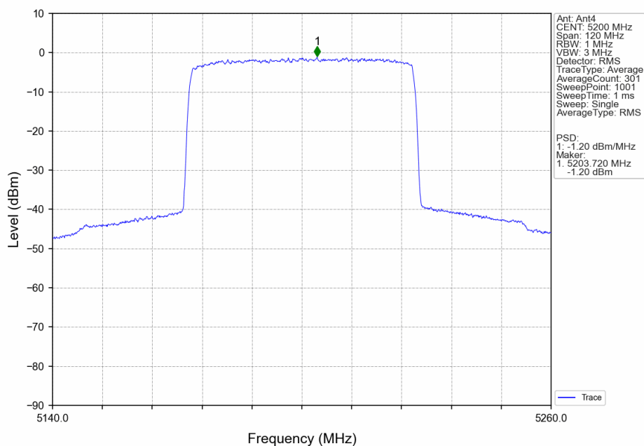
60M_MCH_5200MHz_Ant4_NTNV
