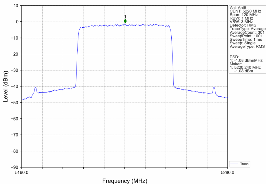
60M_HCH_5220MHz_Ant5_NTNV
