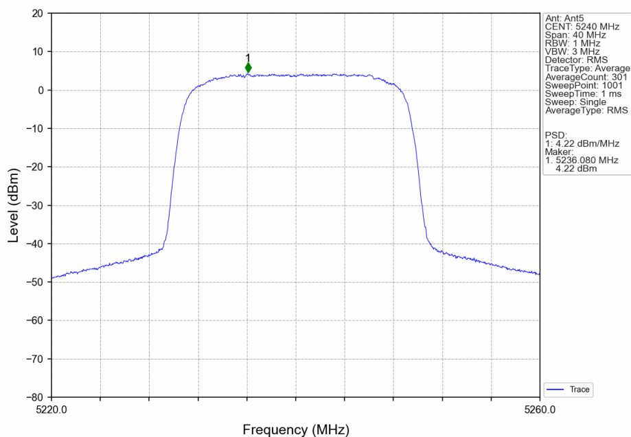
20M_HCH_5240MHz_Ant5_NTNV
