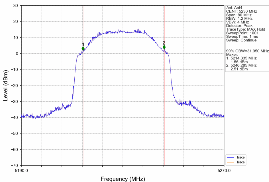
40M_HCH_5230MHz_Ant4_NTNV
