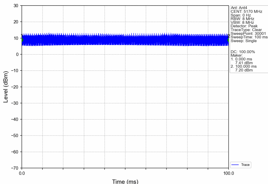
40M_LCH_5170MHz_Ant4_NTNV
