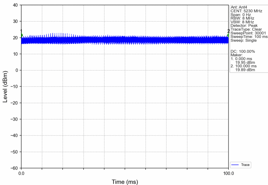
40M_HCH_5230MHz_Ant4_NTNV
