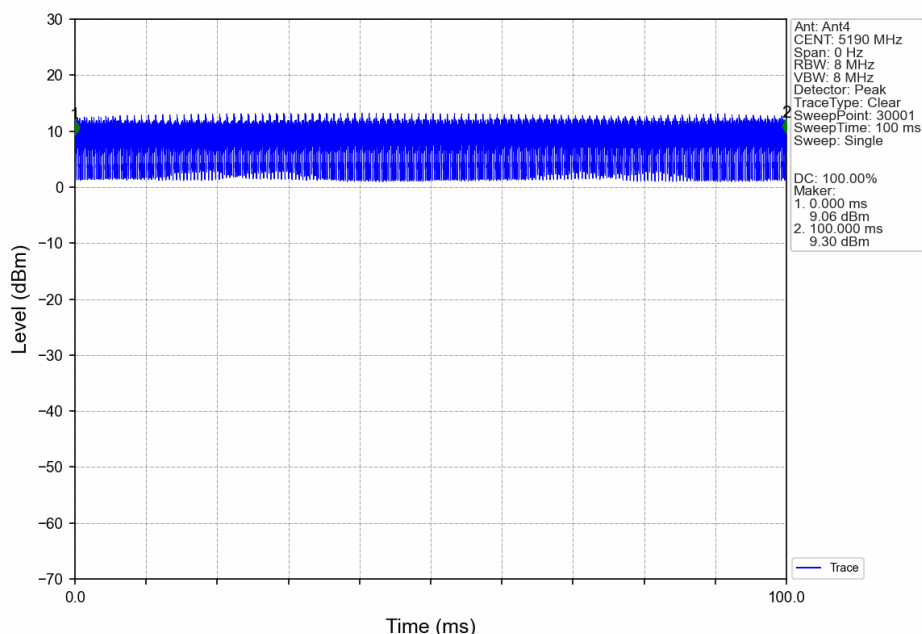
80M_LCH_5190MHz_Ant4_NTNV
