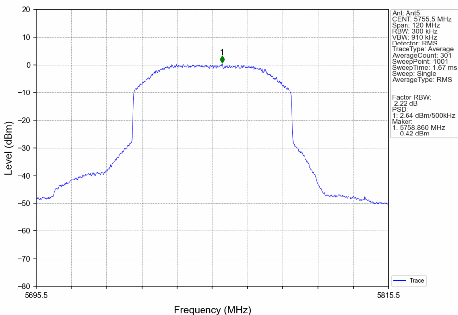
60M_LCH_5755.5MHz_Ant5_NTNV
