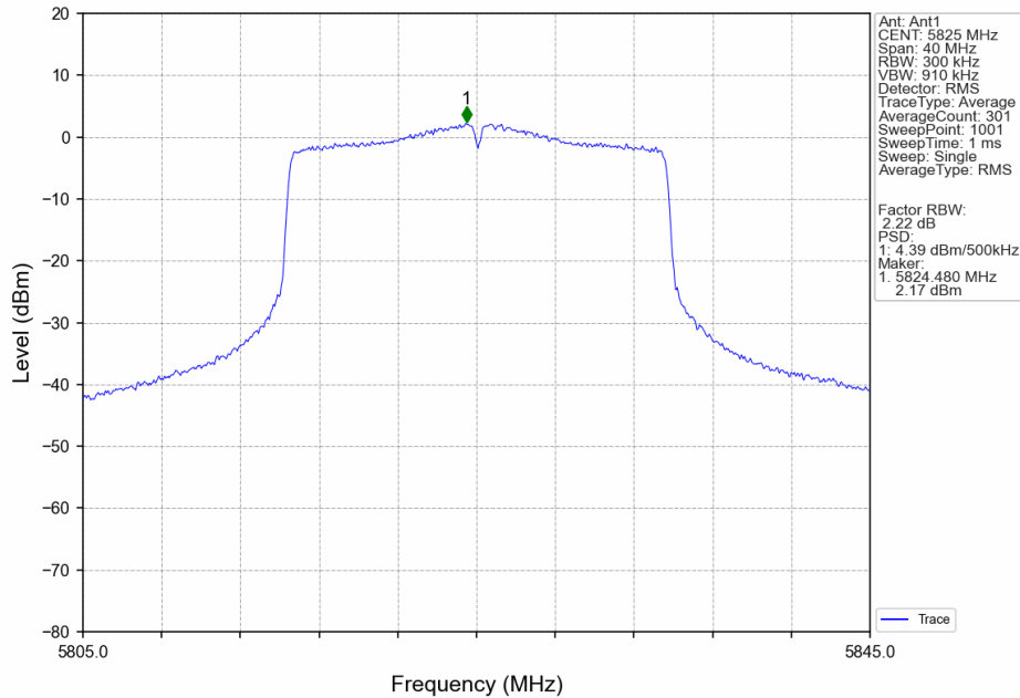
802.11ax(HEW20)_HCH_5825MHz_SU_/_MIMO_NTNV
