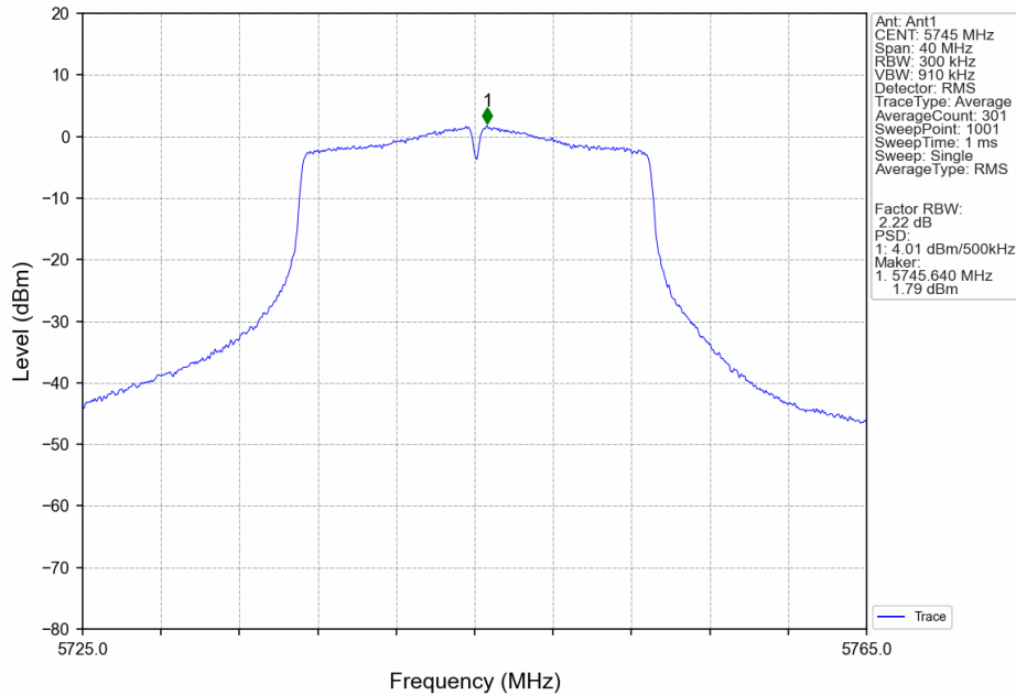
802.11ac(VHT20)_LCH_5745MHz_MIMO_NTNV
