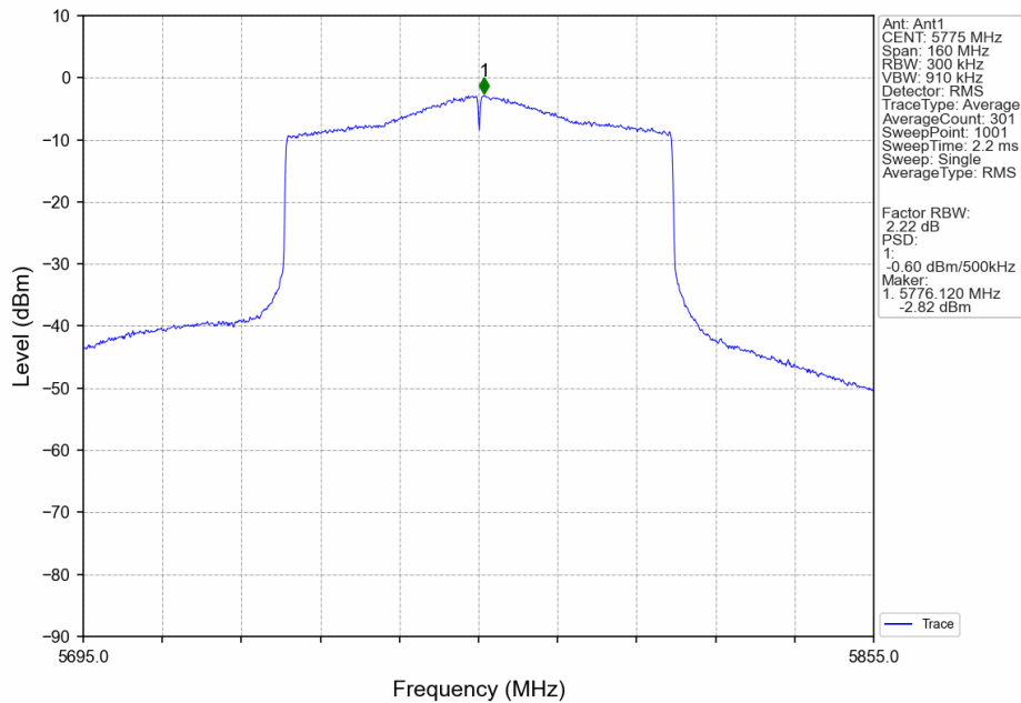
802.11ax(HEW80)_MCH_5775MHz_SU_ / _Ant1_NTNV
