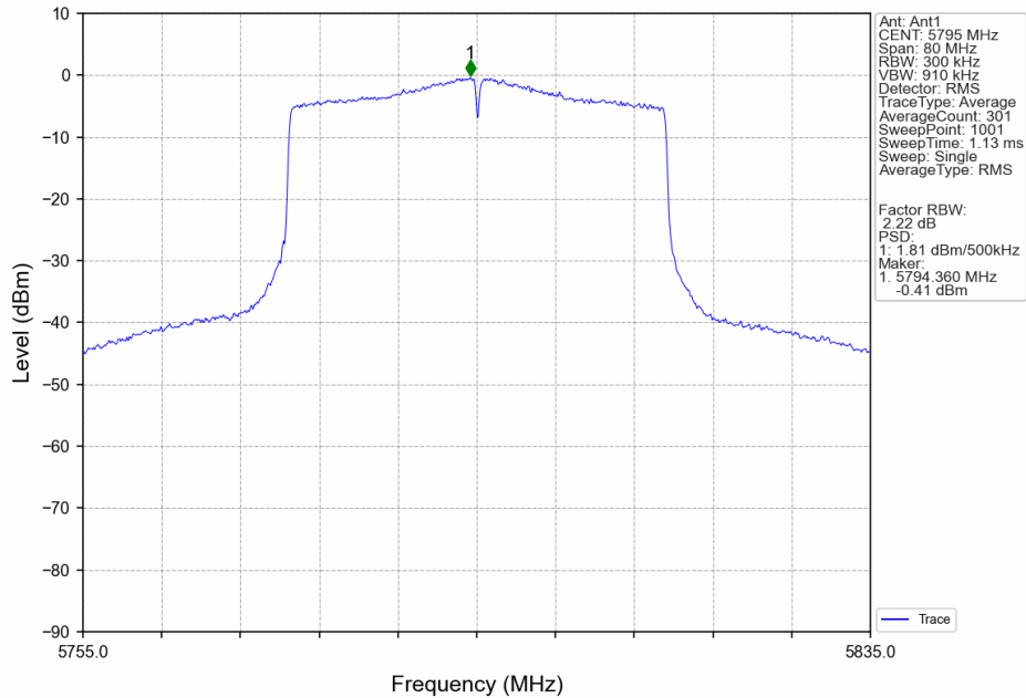
802.11ax(HEW40)_HCH_5795MHz_SU_/_MIMO_NTNV
