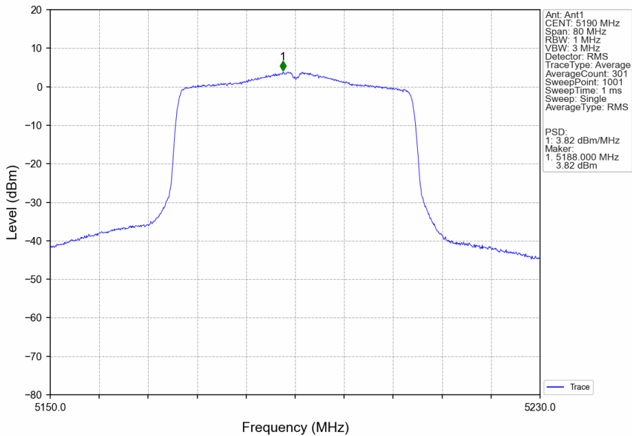
802.11ax(HEW40)_LCH_5190MHz_SU_ / _Ant1_NTNV
