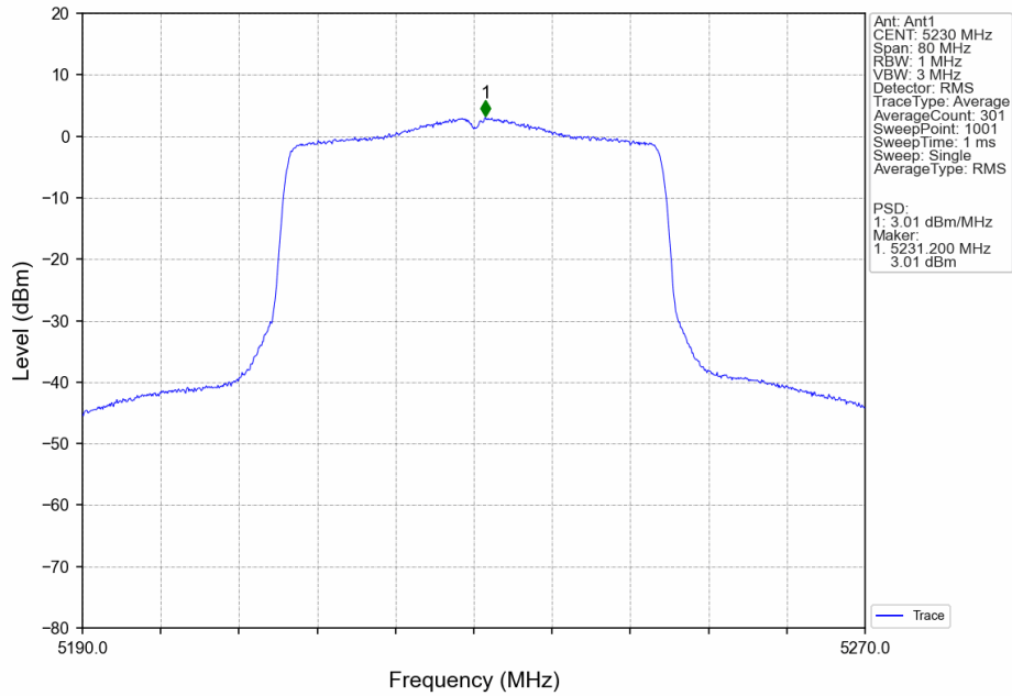
802.11ax(HEW40)_HCH_5230MHz_SU_ / _MIMO_NTNV
