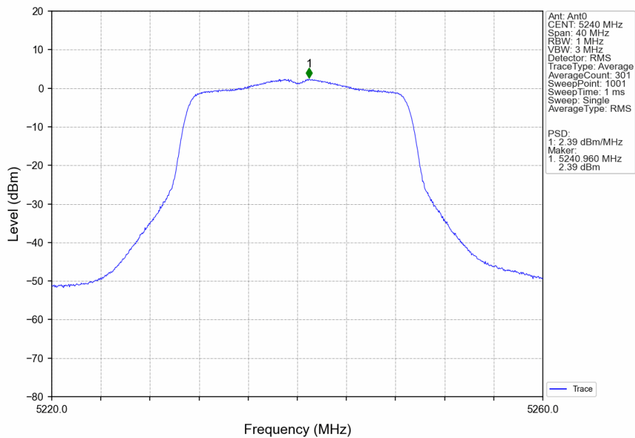
802.11ac(VHT20)_HCH_5240MHz_Ant0_NTNV
