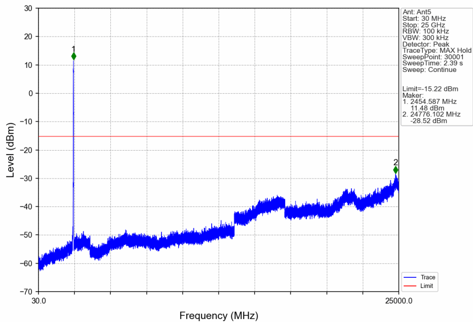
40M_HCH_2452.5MHz_Ant5_NTNV
