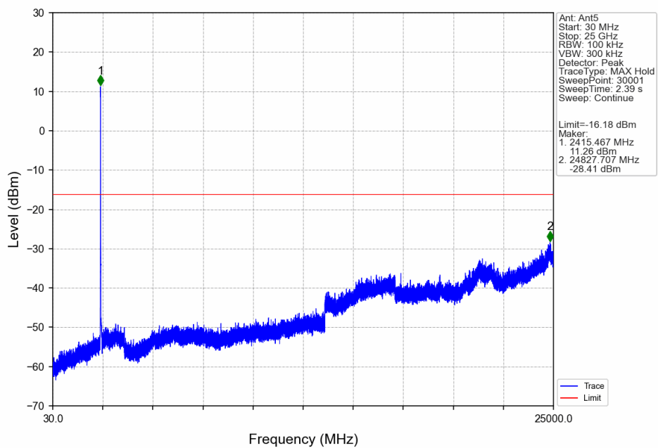
20M_LCH_2412.5MHz_Ant5_NTNV
