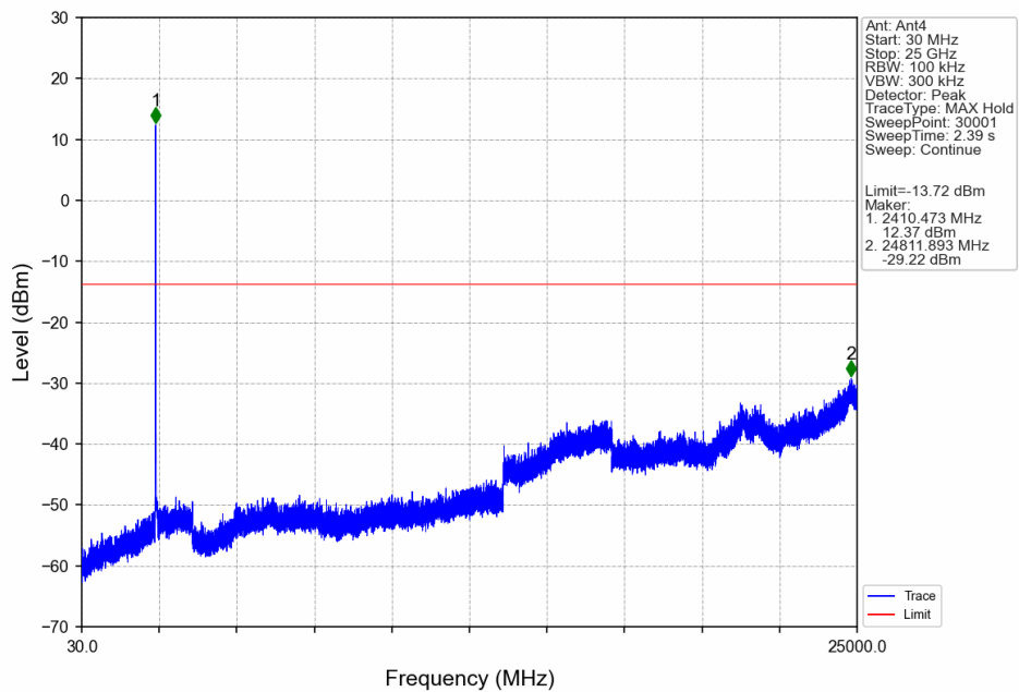
10M_LCH_2407.5MHz_Ant4_NTNV
