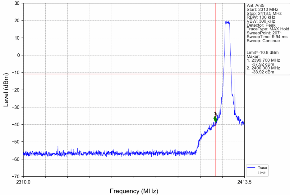
3M_LCH_2405.5MHz_Ant5_NTNV
