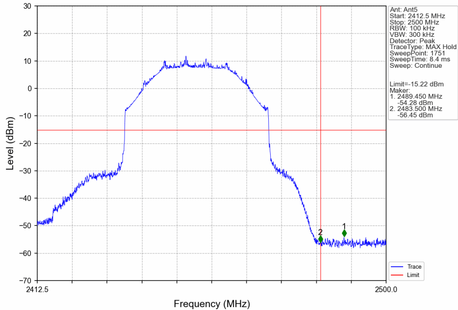
40M_HCH_2452.5MHz_Ant5_NTNV
