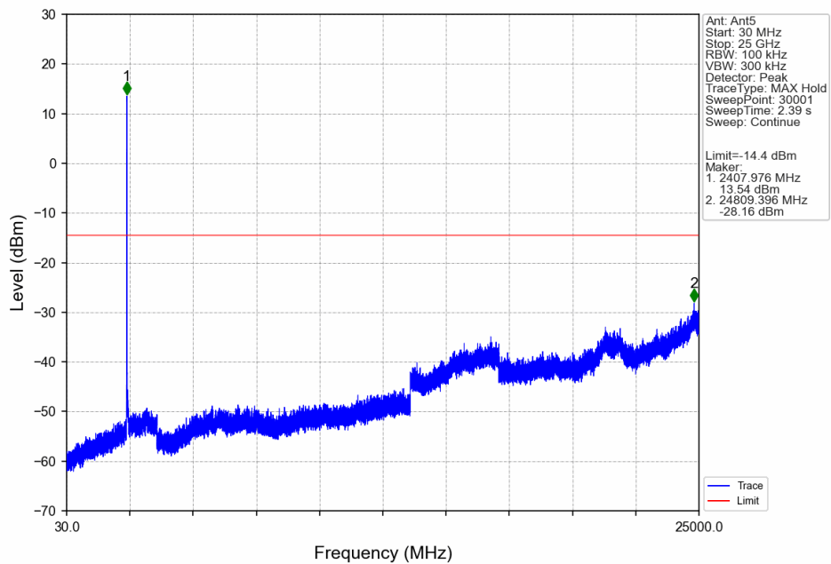
10M_LCH_2407.5MHz_Ant5_NTNV
