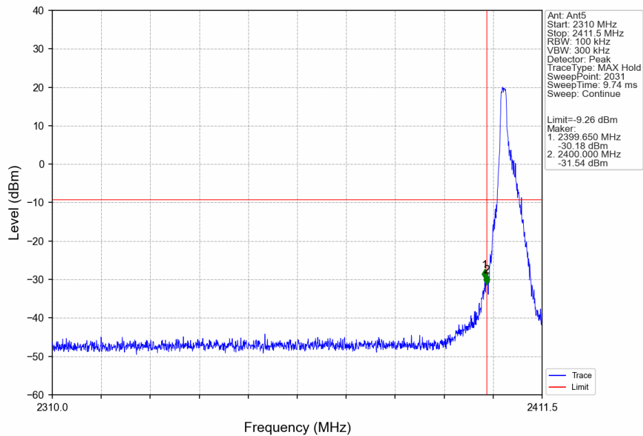
1.4M_LCH_2403.5MHz_Ant5_NTNV
