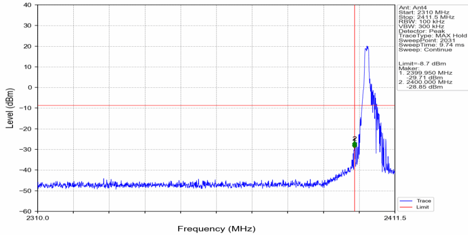
1.4M_LCH_2403.5MHz_Ant4_NTNV
