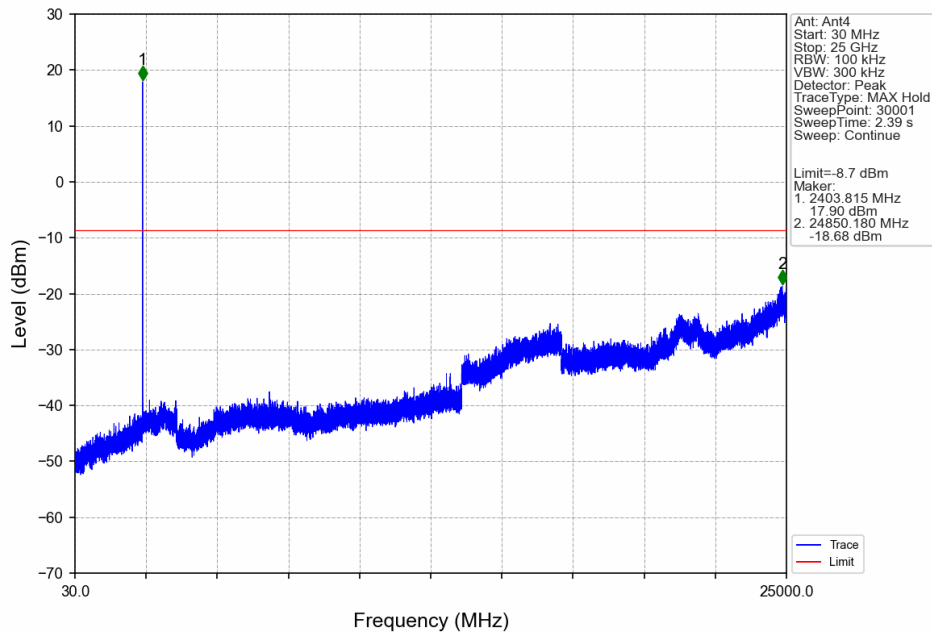
1.4M_LCH_2403.5MHz_Ant4_NTNV
