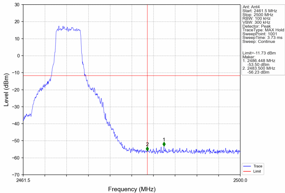
5M_HCH_2469.5MHz_Ant4_NTNV
