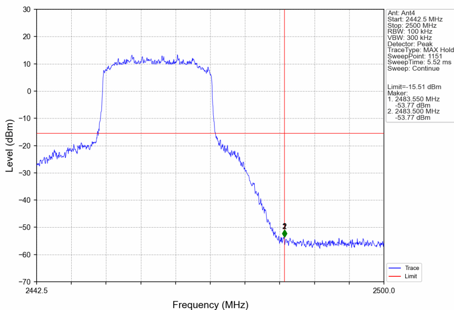
20M_HCH_2462.5MHz_Ant4_NTNV
