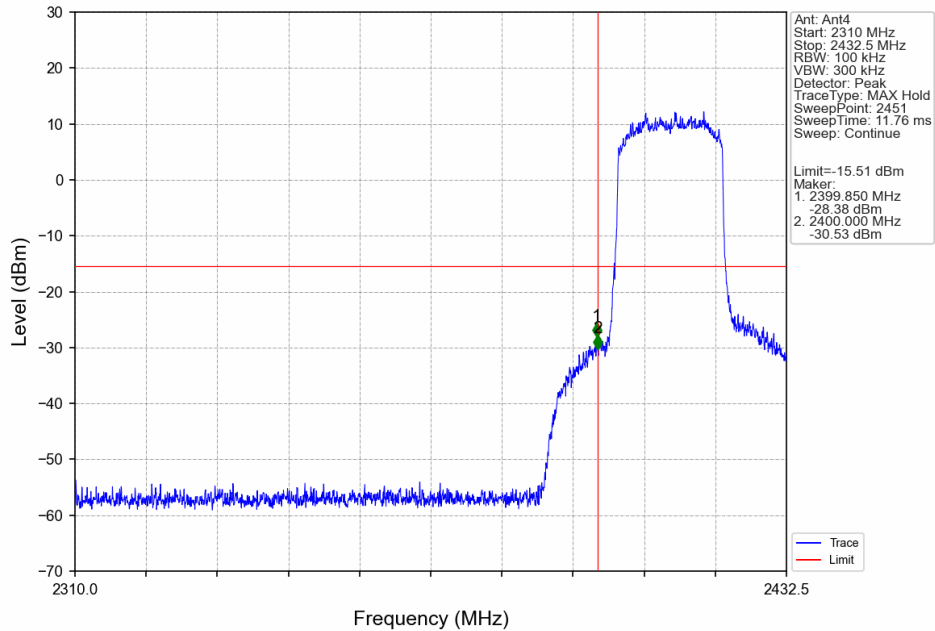
20M_LCH_2412.5MHz_Ant4_NTNV
