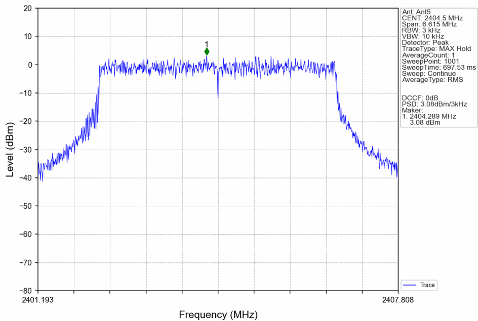
5M_LCH_2404.5MHz_Ant5_NTNV
