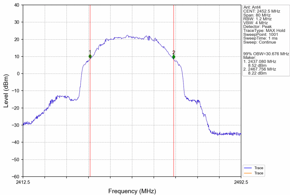
40M_HCH_2452.5MHz_Ant4_NTNV
