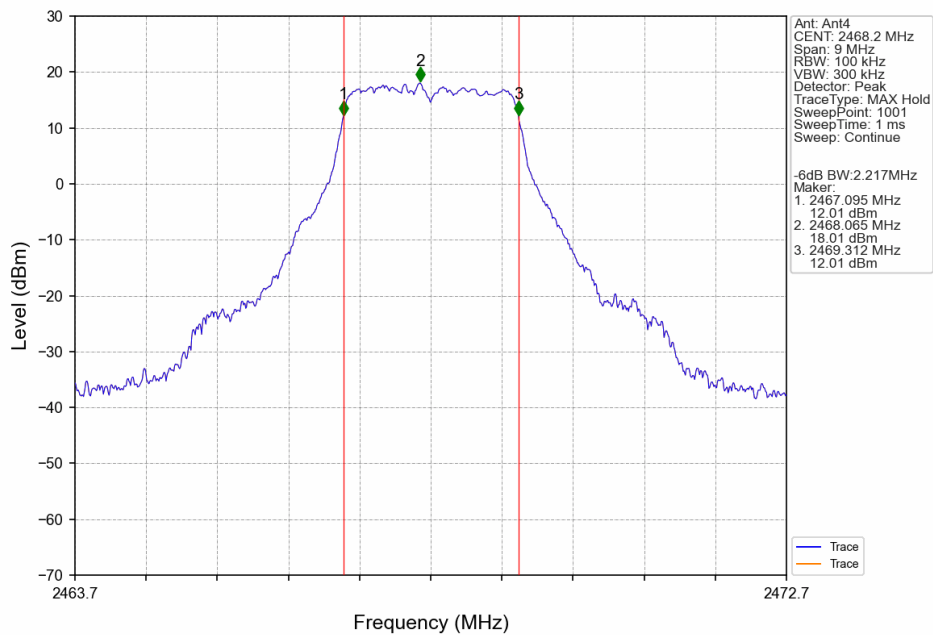
3M_HCH_2468.2MHz_Ant4_NTNV
