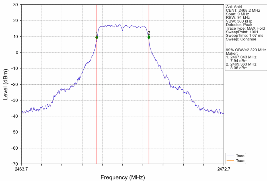
3M_HCH_2468.2MHz_Ant4_NTNV
