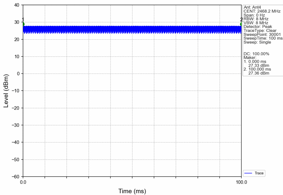
3M_HCH_2468.2MHz_Ant4_NTNV
