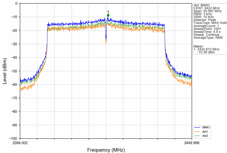
802.11ax(HEW40)_LCH_2422MHz_SU_ / _MIMO_NTNV
