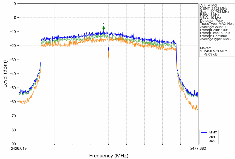
802.11ax(HEW40)_HCH_2452MHz_SU_/_MIMO_NTNV
