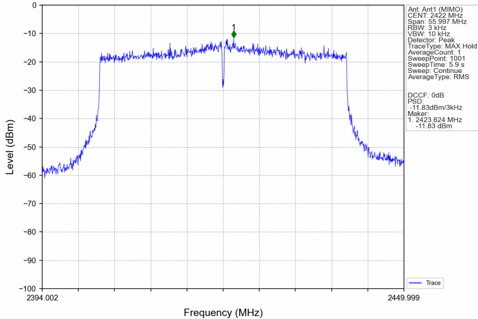
802.11ax(HEW40)_LCH_2422MHz_SU_ / _MIMO_NTNV
