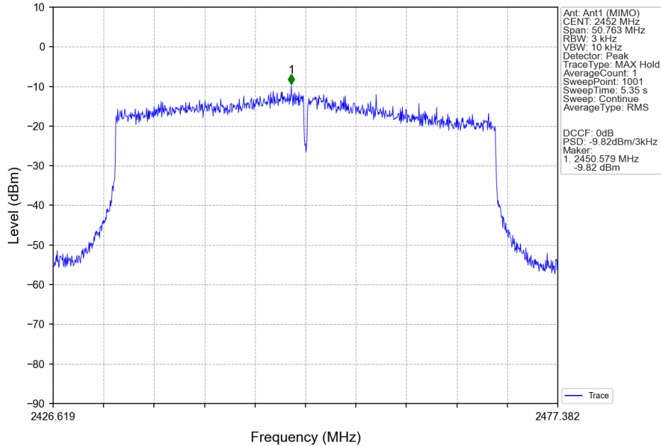
802.11ax(HEW40)_HCH_2452MHz_SU_/_MIMO_NTNV
