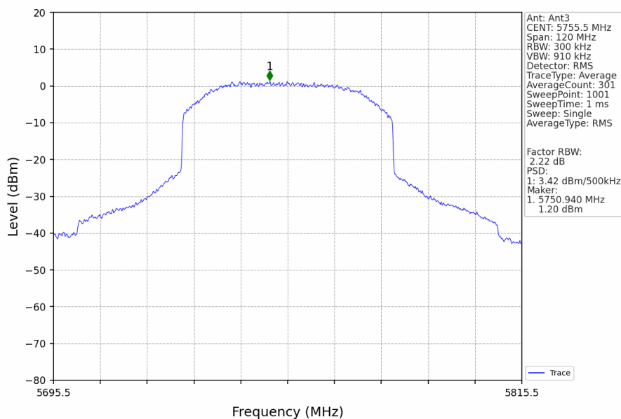
60M_LCH_5755.5MHz_Ant3_NTNV
