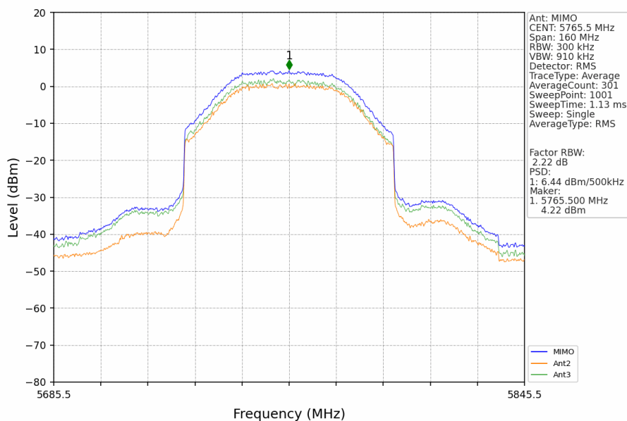
80M_LCH_5765.5MHz_MIMO_NTNV
