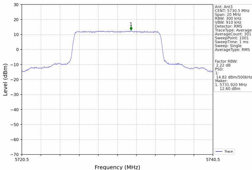
10M_LCH_5730.5MHz_MIMO_NTNV
