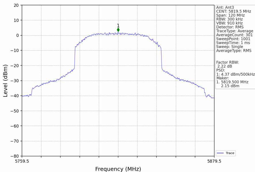
60M_HCH_5819.5MHz_Ant3_NTNV
