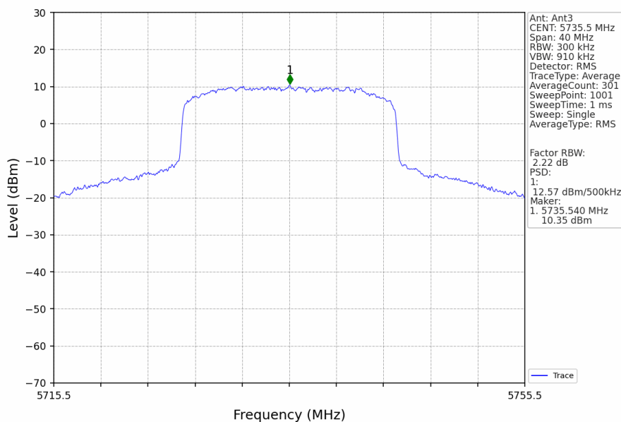
20M_LCH_5735.5MHz_Ant3_NTNV
