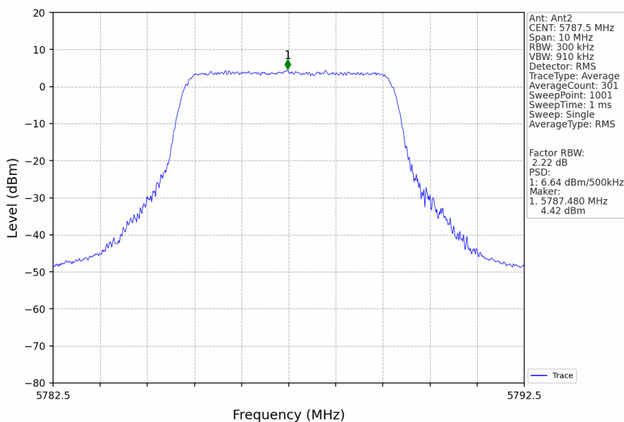
5M_MCH_5787.5MHz_Ant2_NTNV
