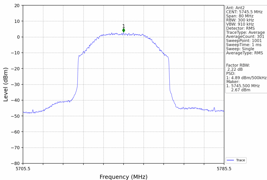
40M_LCH_5745.5MHz_Ant2_NTNV
