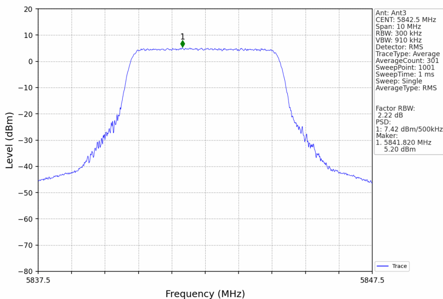
5M_HCH_5842.5MHz_Ant3_NTNV
