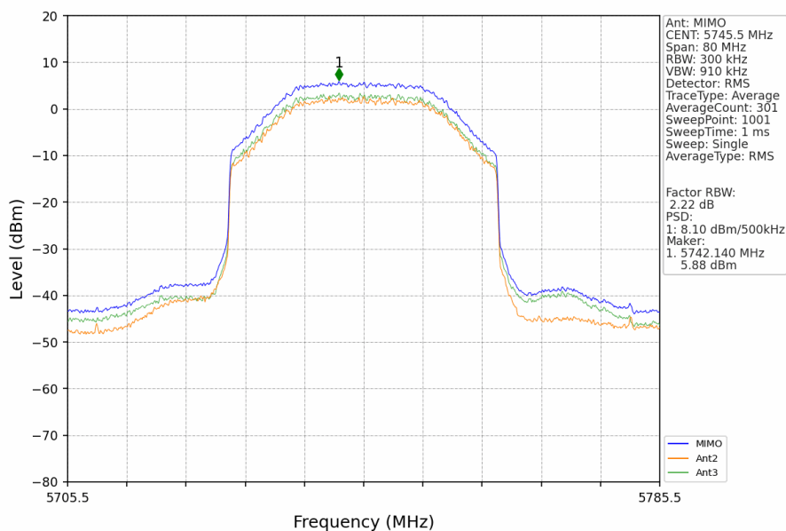
40M_LCH_5745.5MHz_MIMO_NTNV
