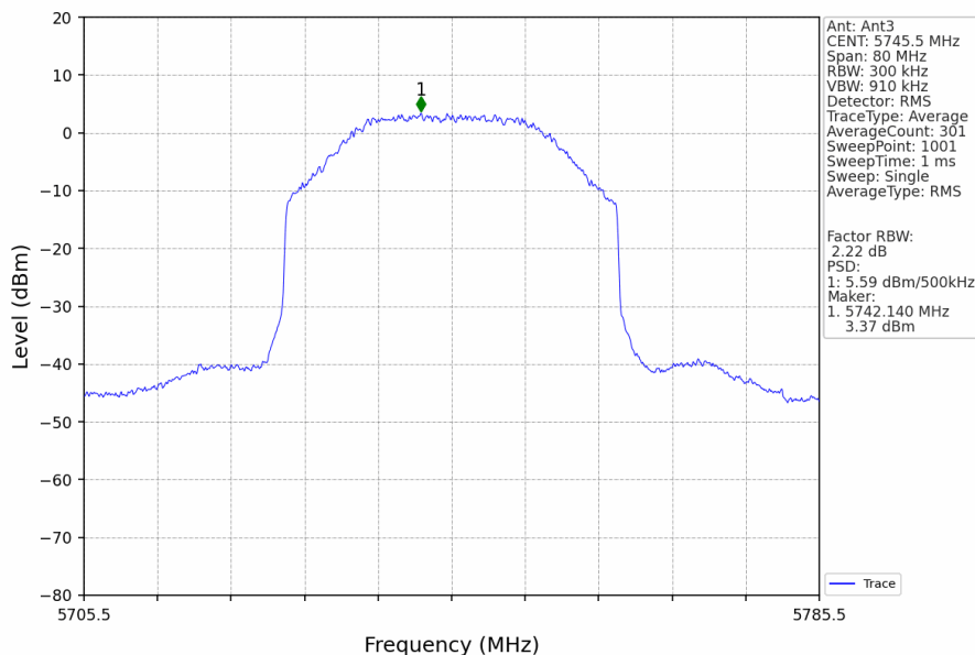
40M_LCH_5745.5MHz_MIMO_NTNV
