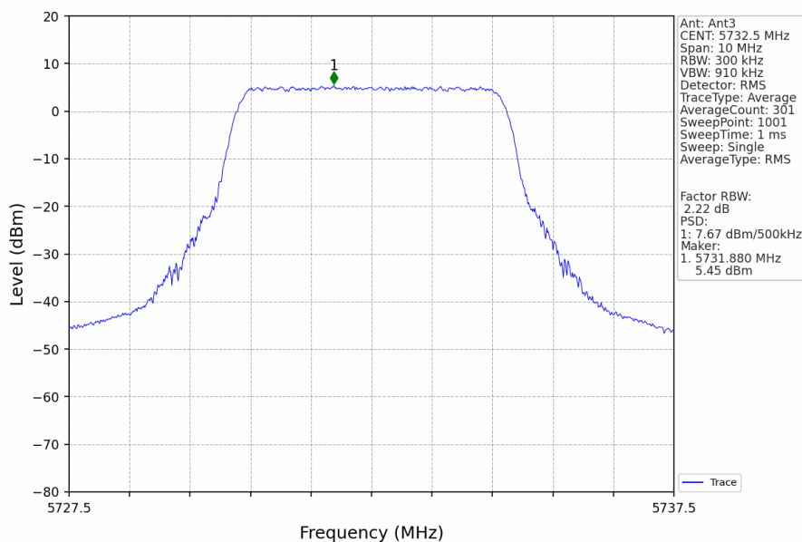
5M_LCH_5732.5MHz_Ant3_NTNV
