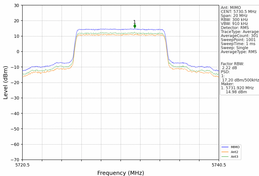
10M_LCH_5730.5MHz_MIMO_NTNV
