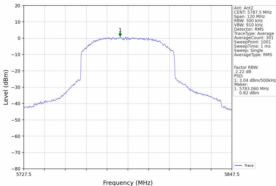
60M_MCH_5787.5MHz_Ant2_NTNV
