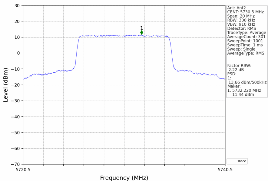
10M_LCH_5730.5MHz_Ant2_NTNV
