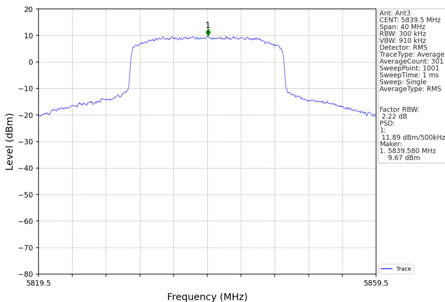
20M_HCH_5839.5MHz_Ant3_NTNV
