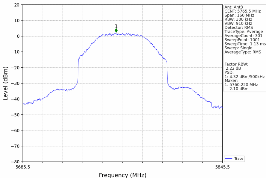
80M_LCH_5765.5MHz_MIMO_NTNV
