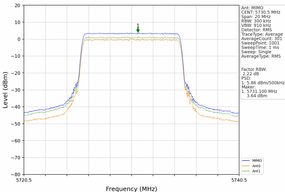
10M_LCH_5730.5MHz_MIMO_NTNV
