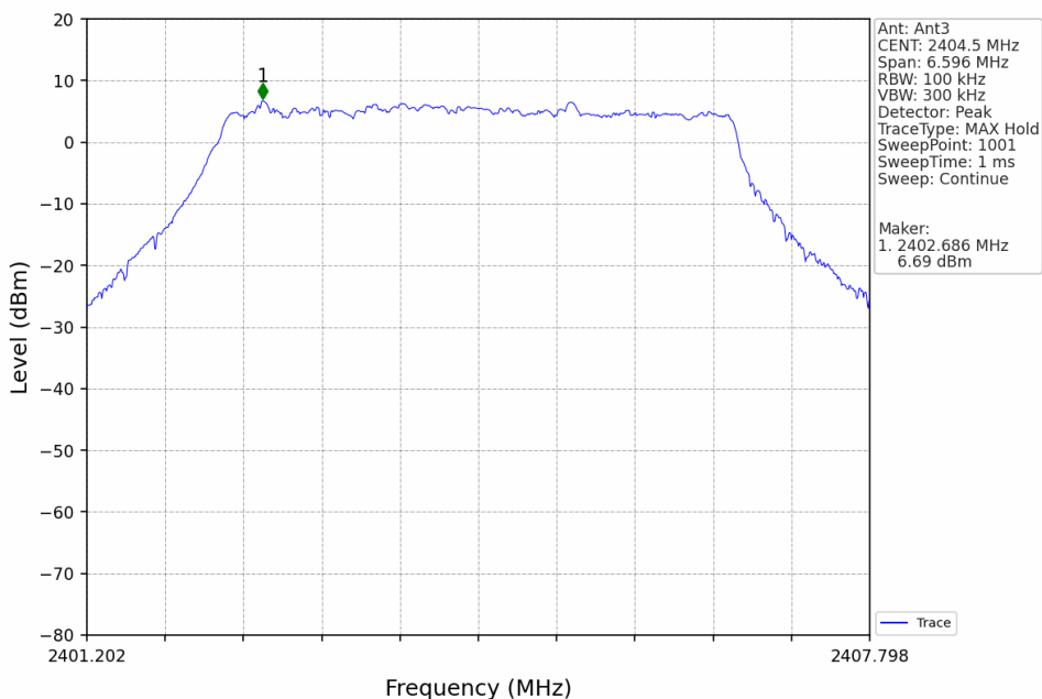
5M_LCH_2404.5MHz_Ant3_NTNV
