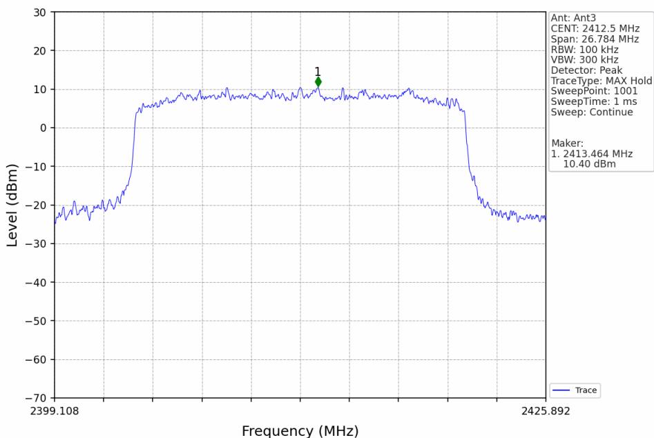
20M_LCH_2412.5MHz_Ant3_NTNV
