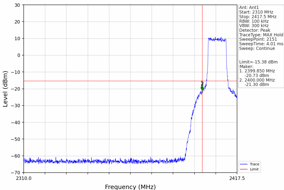
10M_LCH_2407.5MHz_Ant1_NTNV
