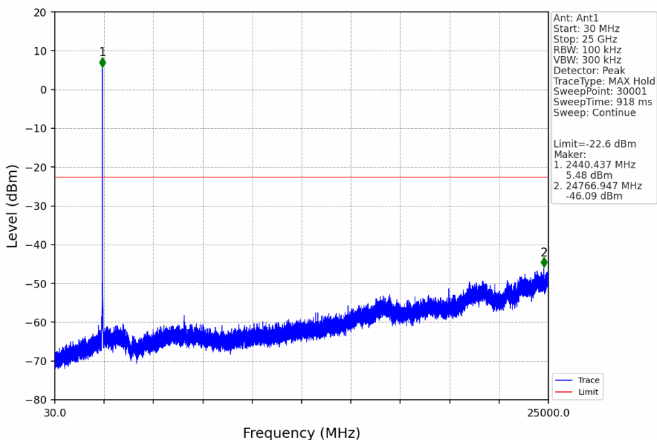
5M_MCH_2439.5MHz_Ant1_NTNV
