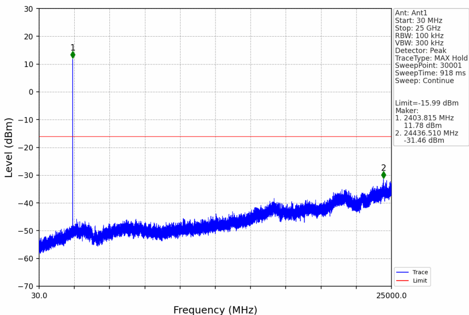
1.4M_LCH_2403.5MHz_Ant1_NTNV
