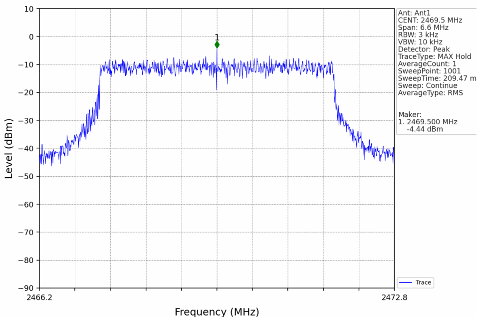
5M_HCH_2469.5MHz_Ant1_NTNV
