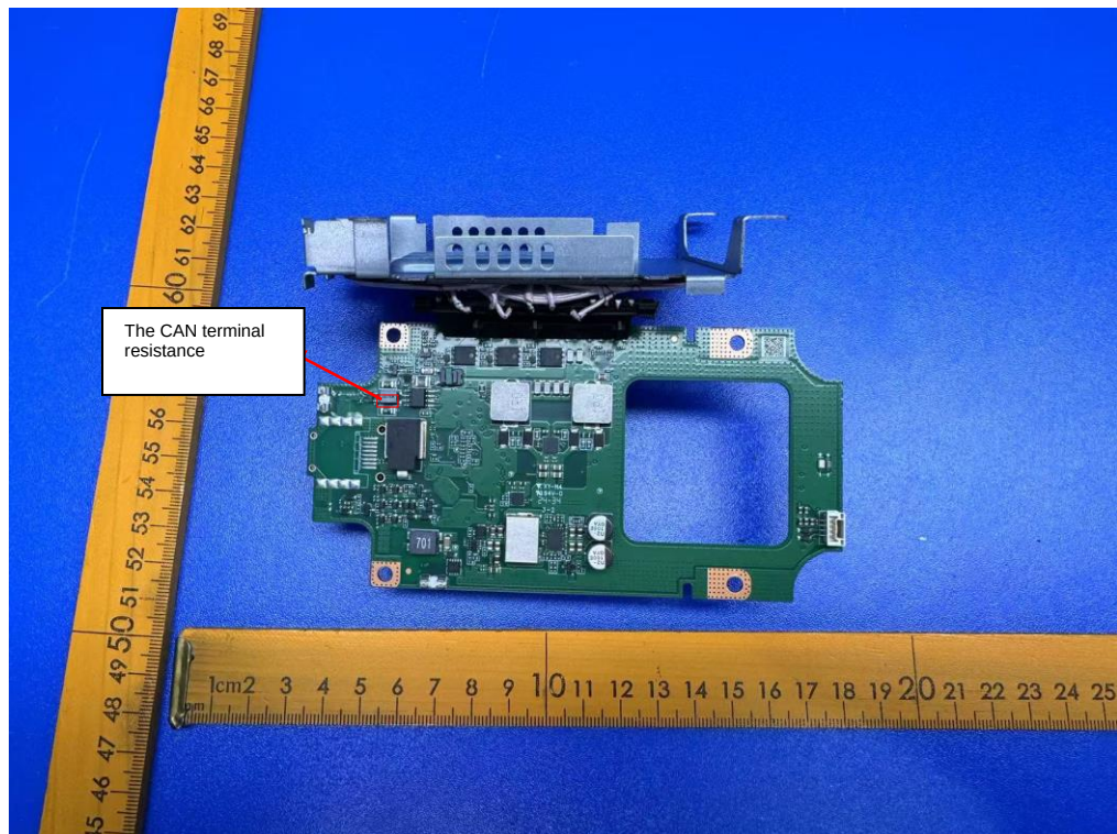
Figure 7 PCB and Coil view
