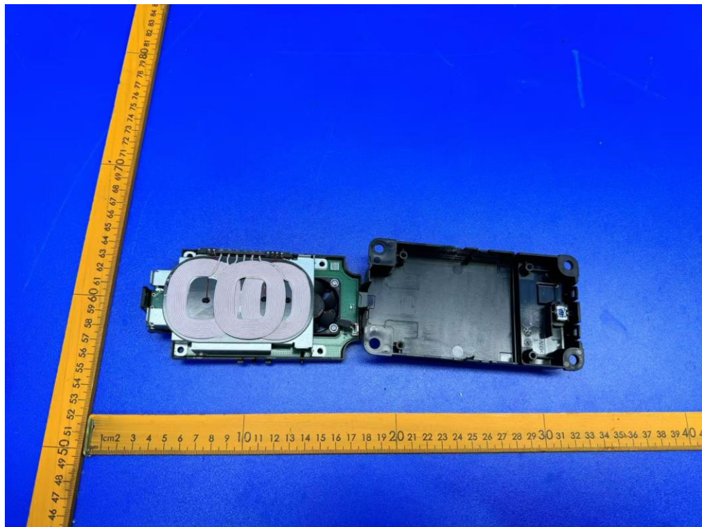
Figure 1 Internal view (TWLC001&TWLC002)
