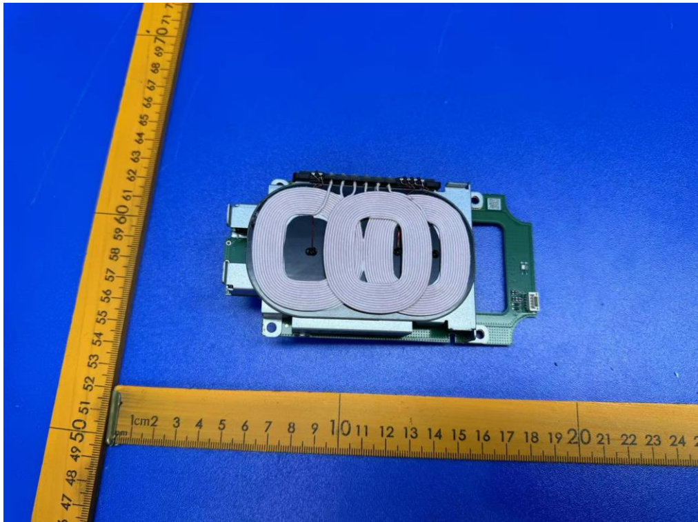
Figure 5 PCB view (TWLC001&TWLC002)
