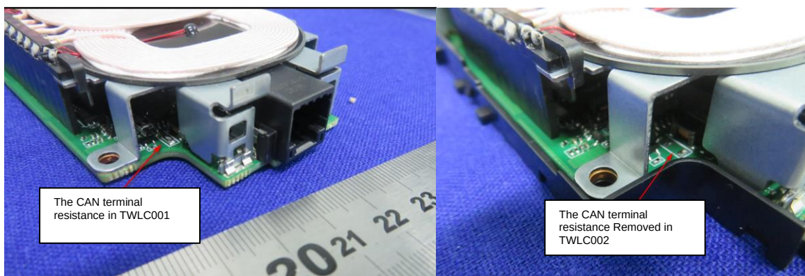
Figure 6 The only difference (TWLC001 VS TWLC002)
