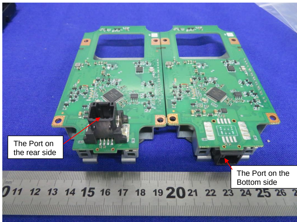
Figure 2 PCB view (TWLC001&TWLC002)
