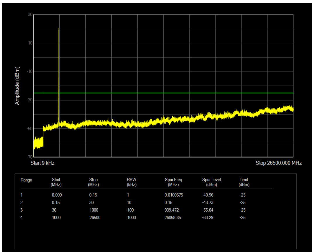
Band41 16QAM BW=10MHz Channel=40090 RB Size=1 Position=#0
