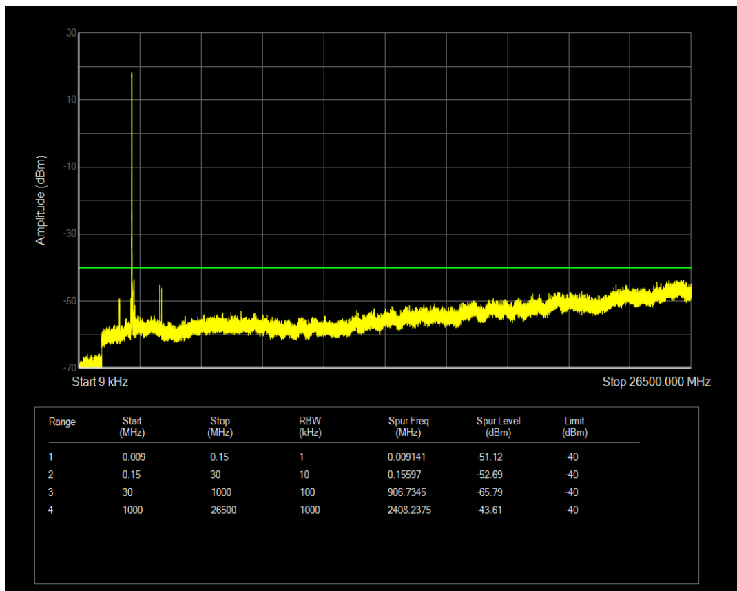
Band40a 16QAM BW=5MHz Channel=38725 RB Size=1 Position=#0
