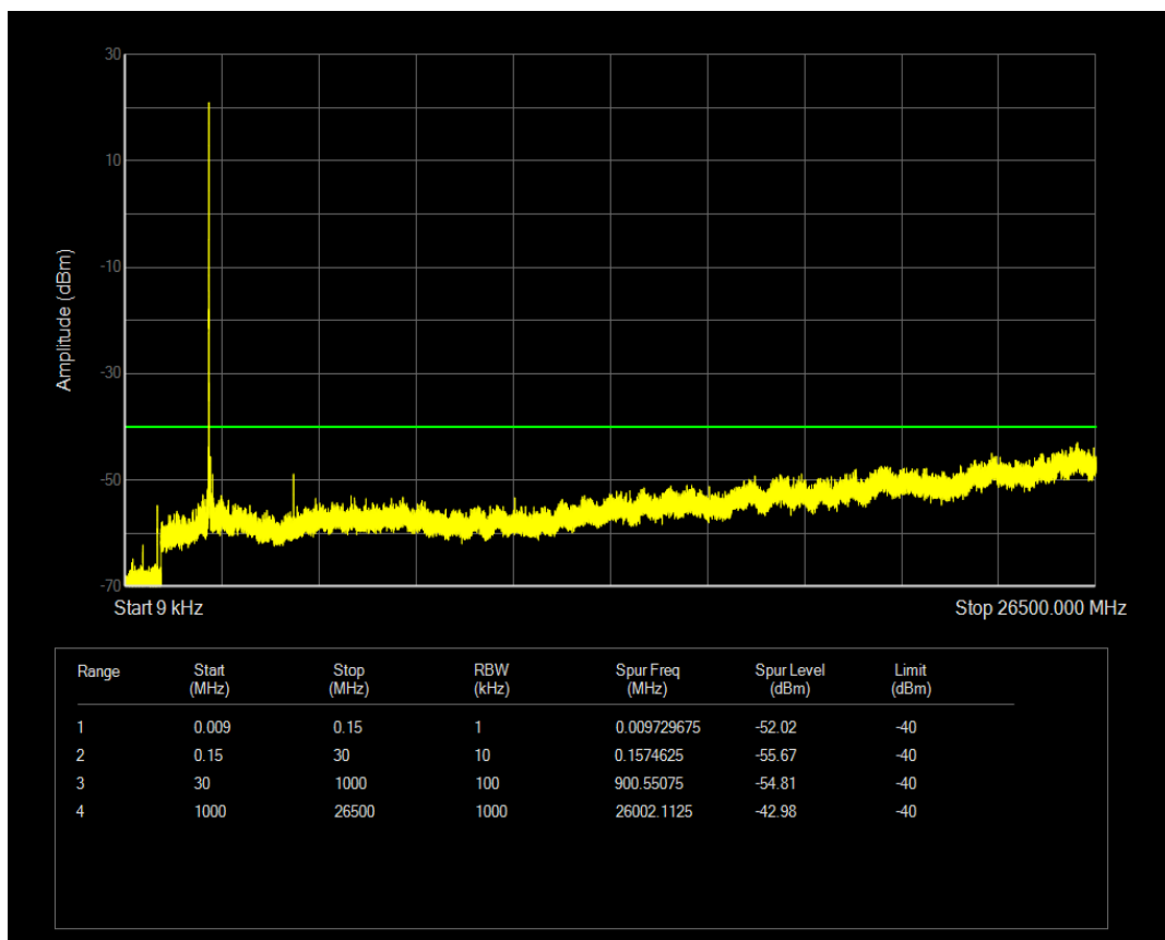
Band40a 16QAM BW=5MHz Channel=38750 RB Size=25 Position=#0
