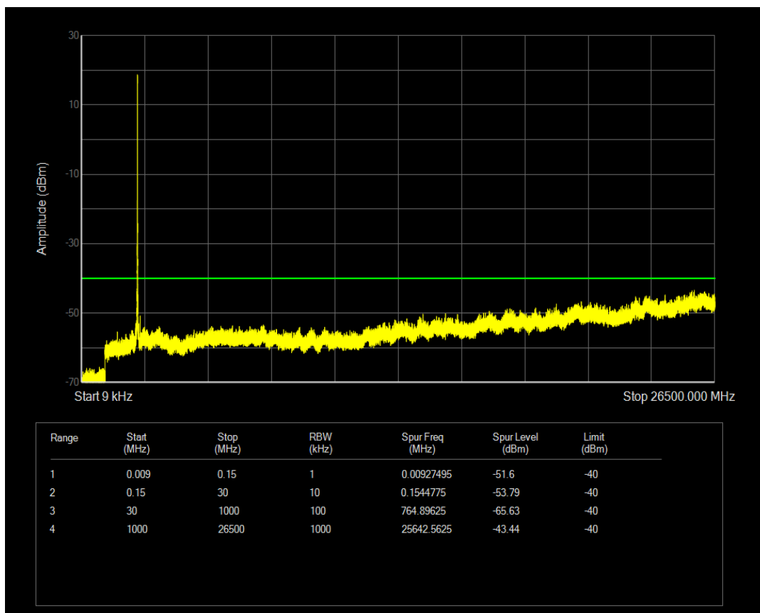
Band40b QPSK BW=5MHz Channel=39175 RB Size=1 Position=#0
