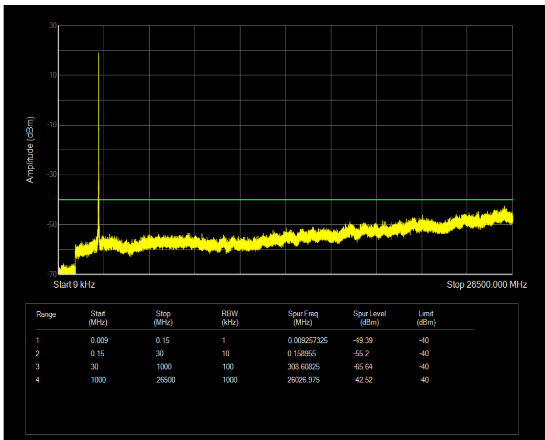
Band40b 16QAM BW=5MHz Channel=39225 RB Size=1 Position=#0
