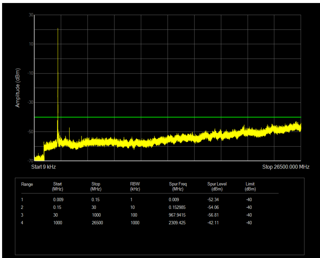
Band40b 16QAM BW=5MHz Channel=39200 RB Size=25 Position=#0
