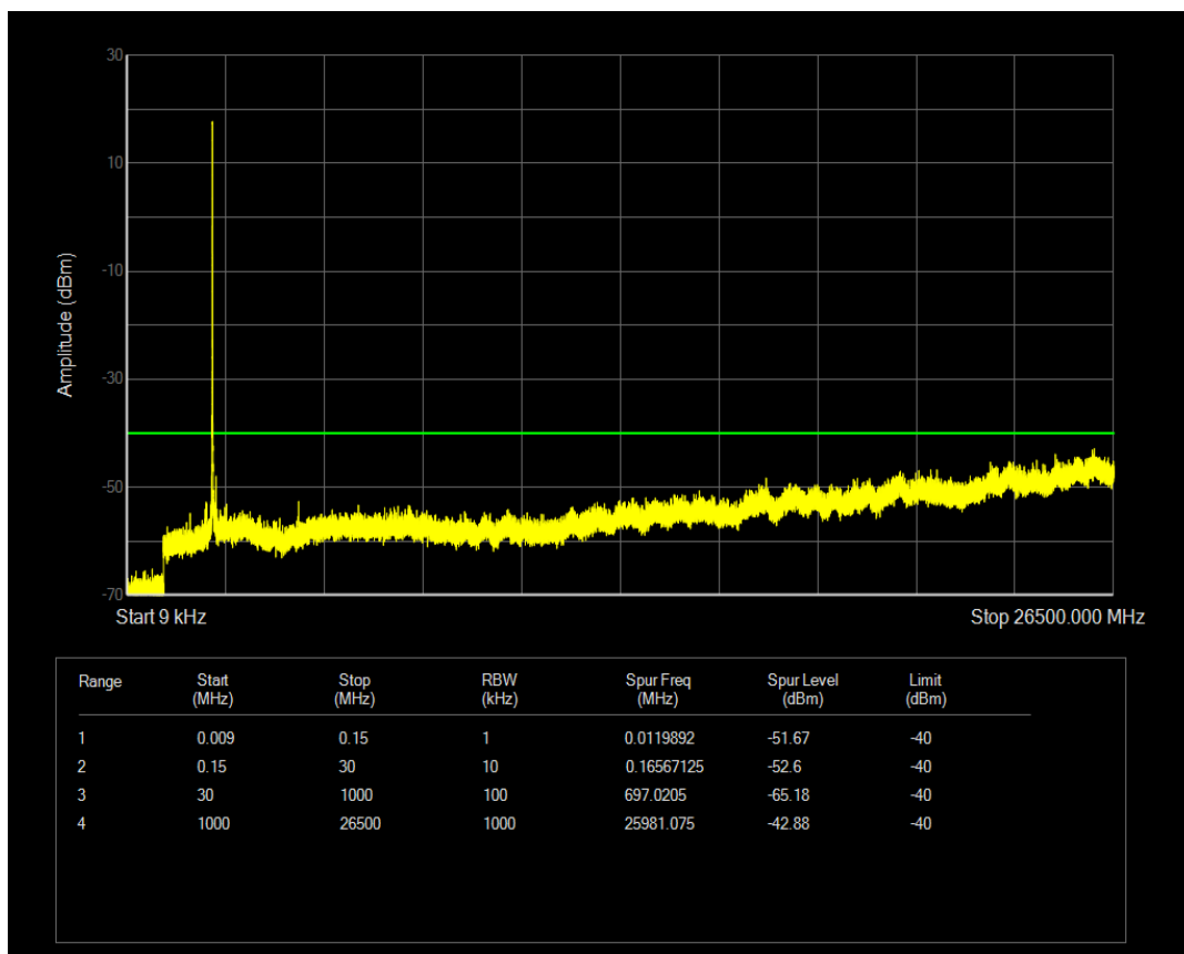
Band40a QPSK BW=5MHz Channel=38775 RB Size=1 Position=#0
