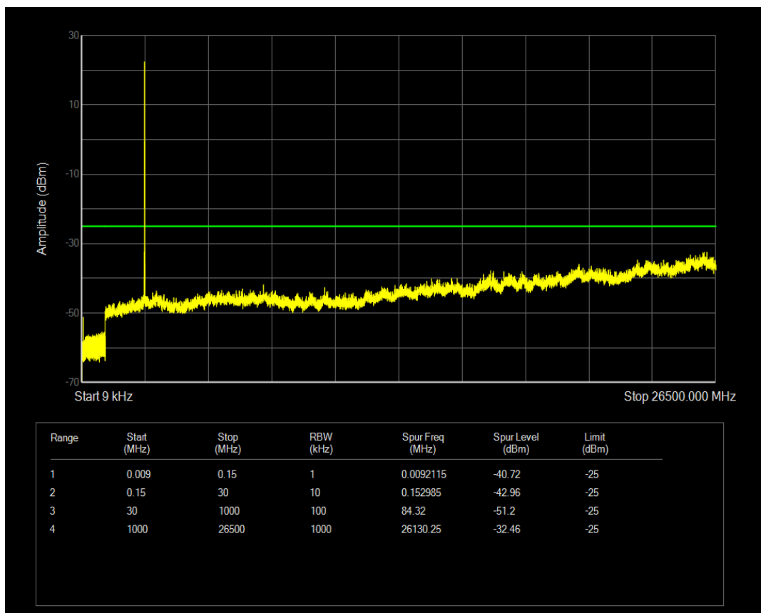
Band41 16QAM BW=10MHz Channel=41190 RB Size=1 Position=#0
