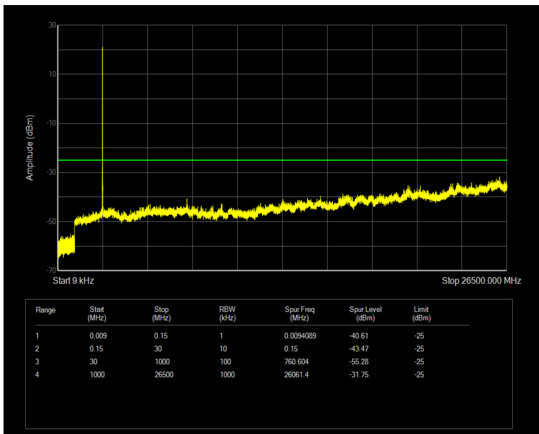
Band41 16QAM BW=5MHz Channel=41215 RB Size=1 Position=#0
