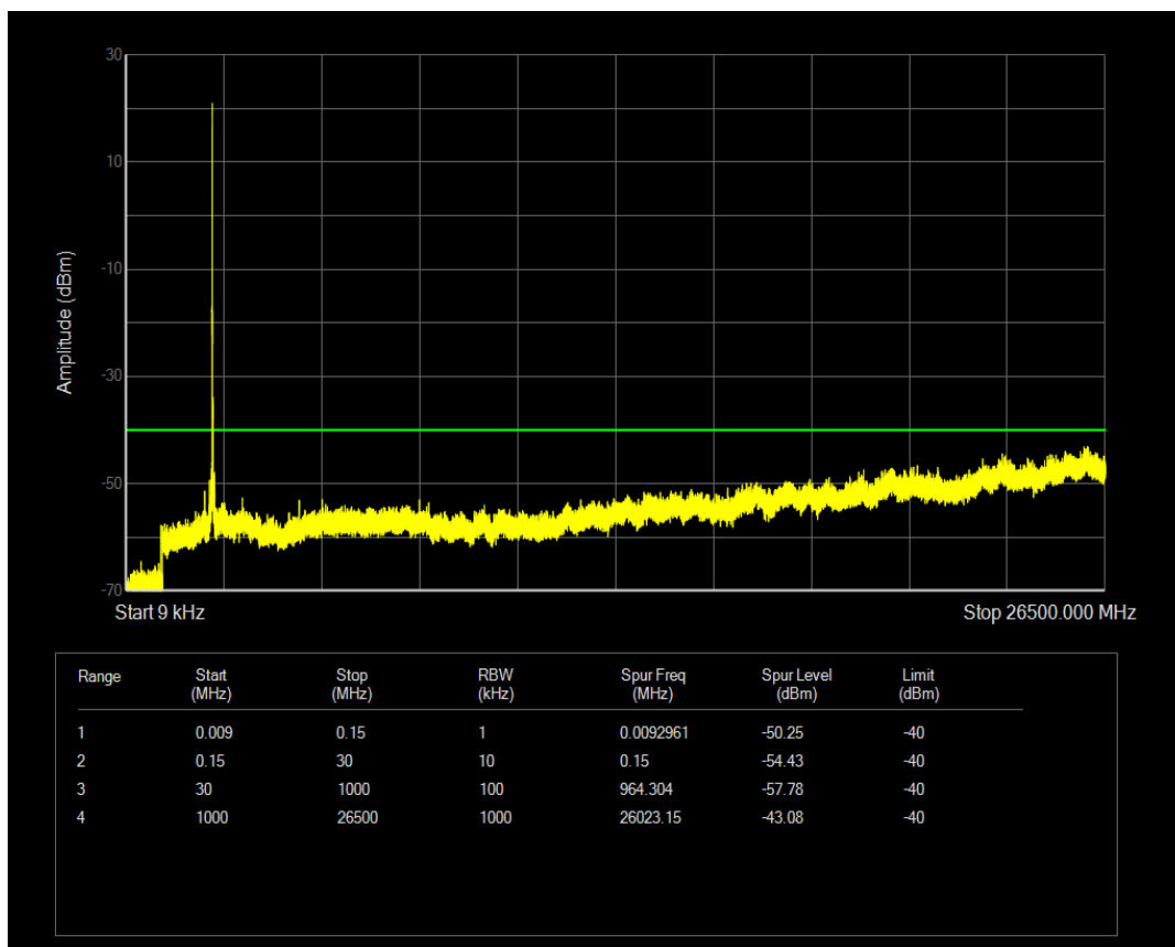
Band40b 16QAM BW=5MHz Channel=39175 RB Size=25 Position=#0
