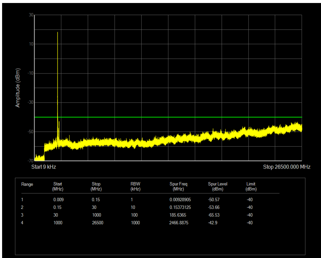
Band40a 16QAM BW=5MHz Channel=38750 RB Size=1 Position=#0
