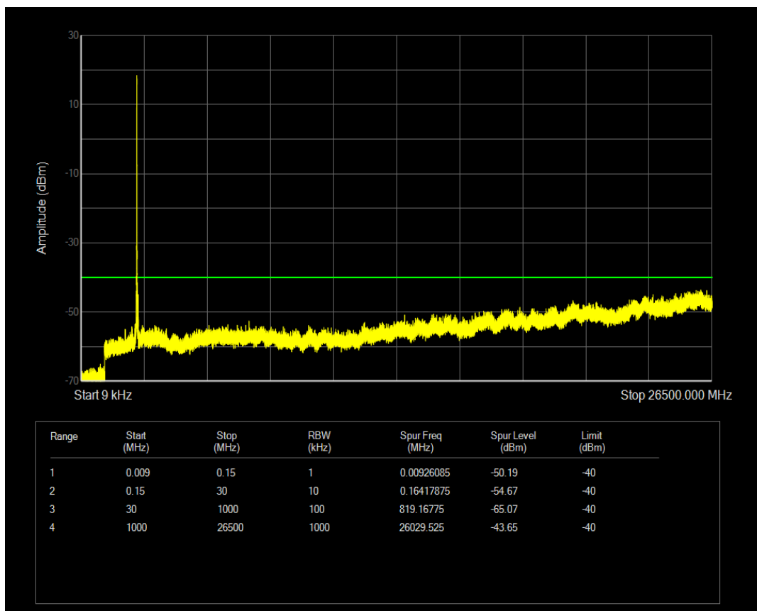
Band40b 16QAM BW=5MHz Channel=39200 RB Size=1 Position=#0
