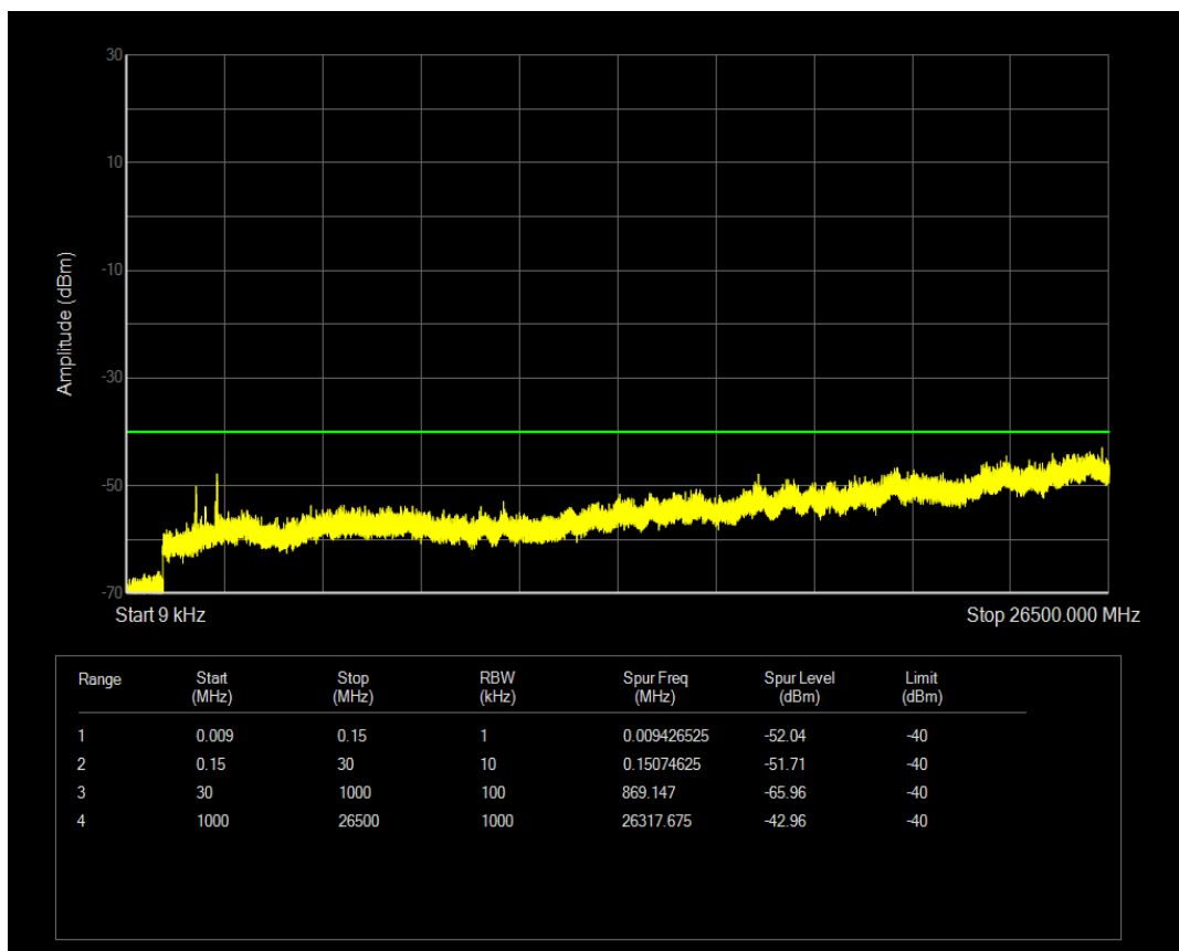
Band40b 16QAM BW=5MHz Channel=39175 RB Size=1 Position=#0
