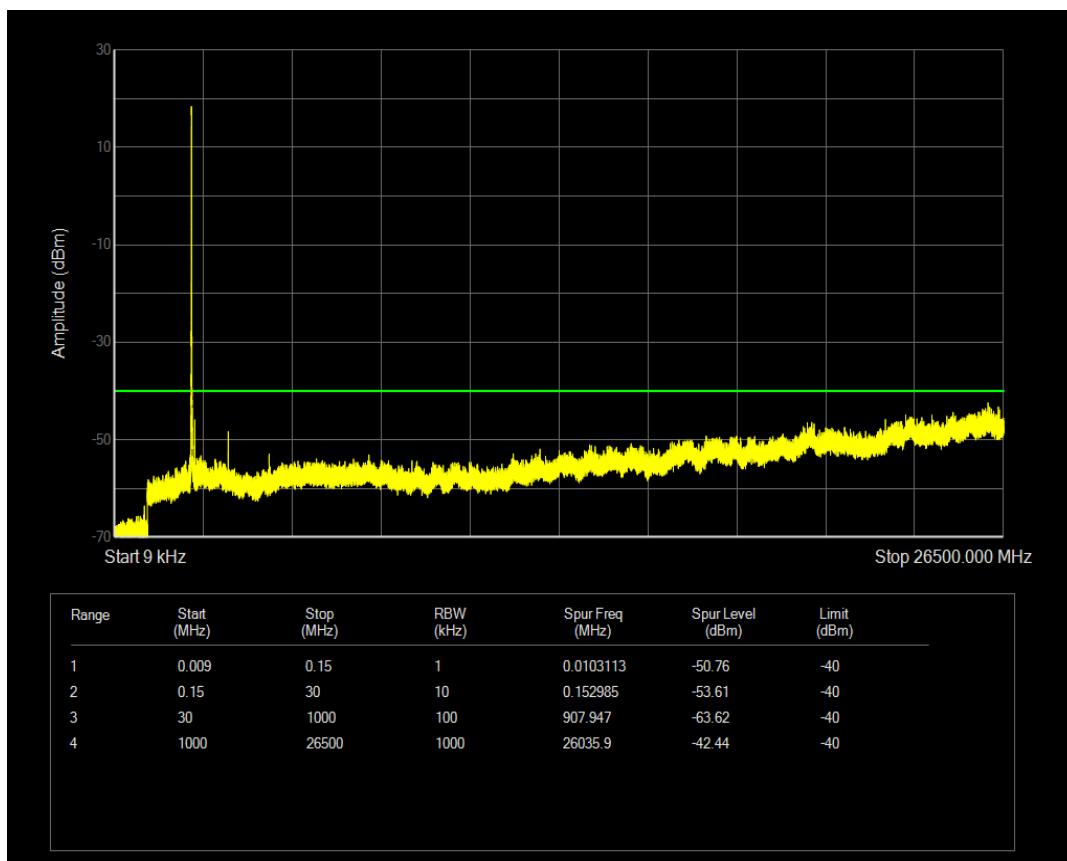
Band40a 16QAM BW=5MHz Channel=38775 RB Size=25 Position=#0
