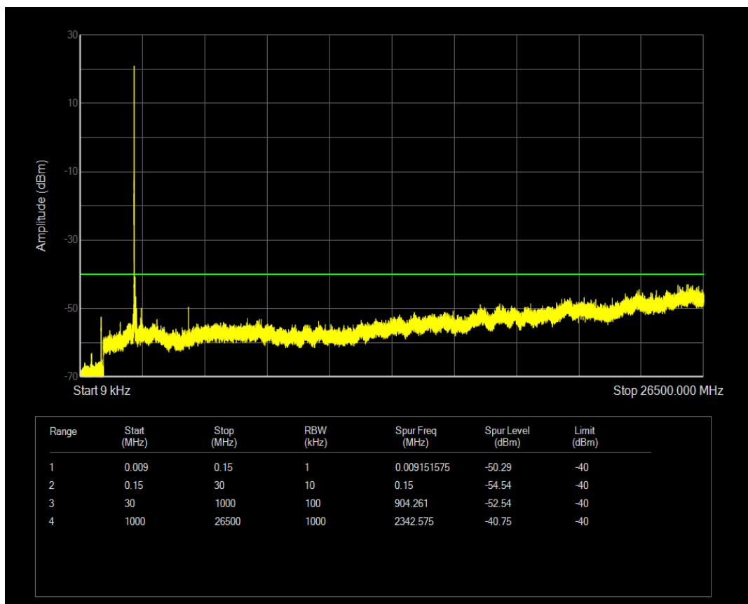
Band40a 16QAM BW=5MHz Channel=38775 RB Size=1 Position=#0
