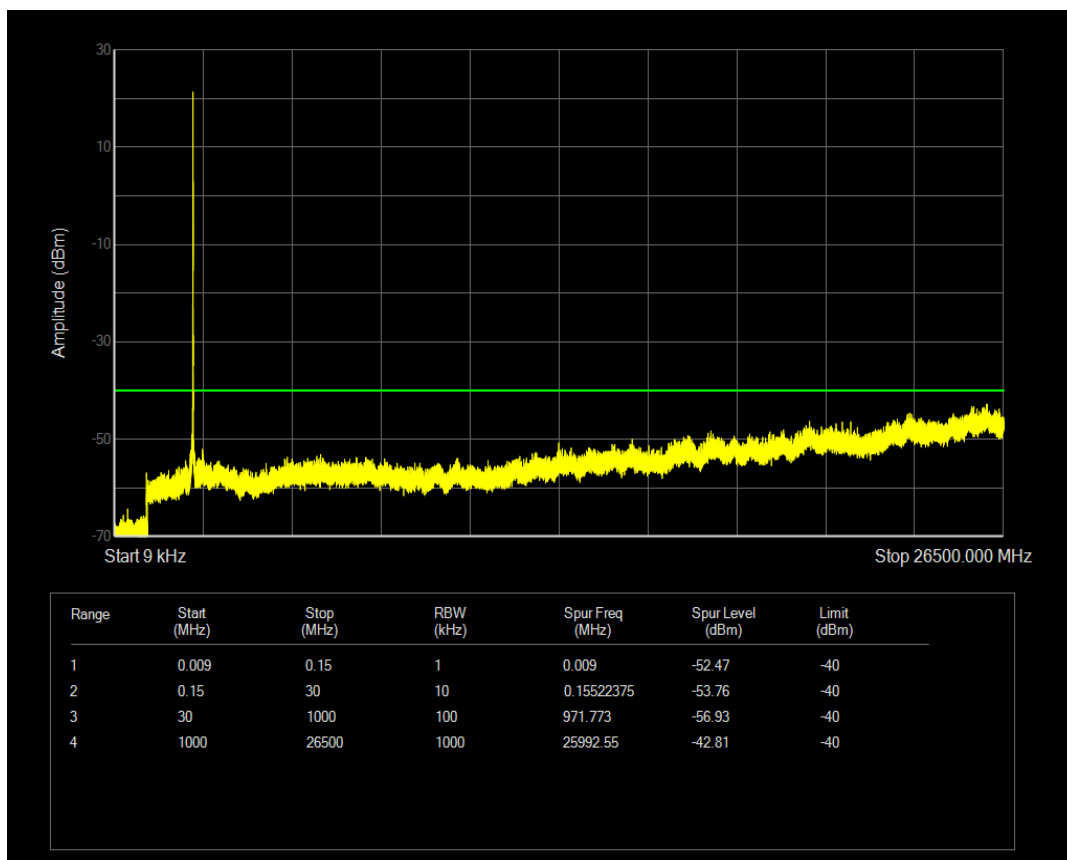
Band40b 16QAM BW=5MHz Channel=39225 RB Size=25 Position=#0
