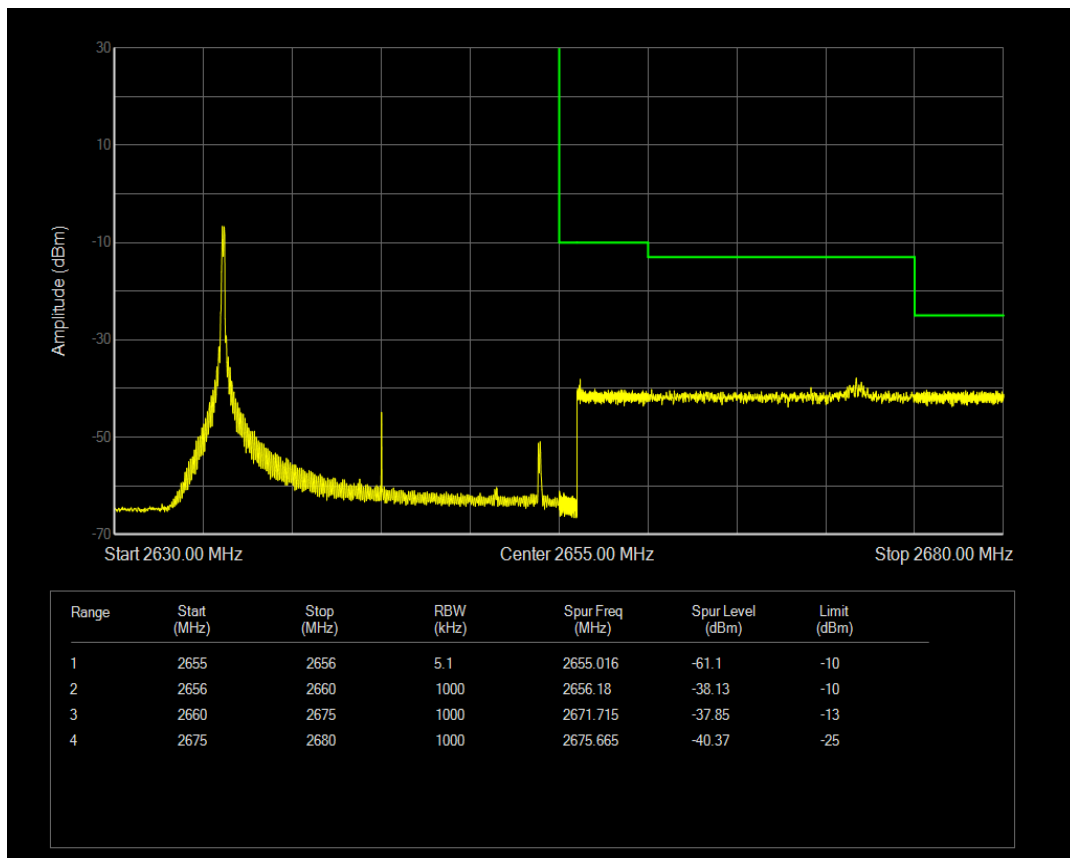
Band41 16QAM BW=20MHz Channel=41140 RB Size=1 Position=#Max
