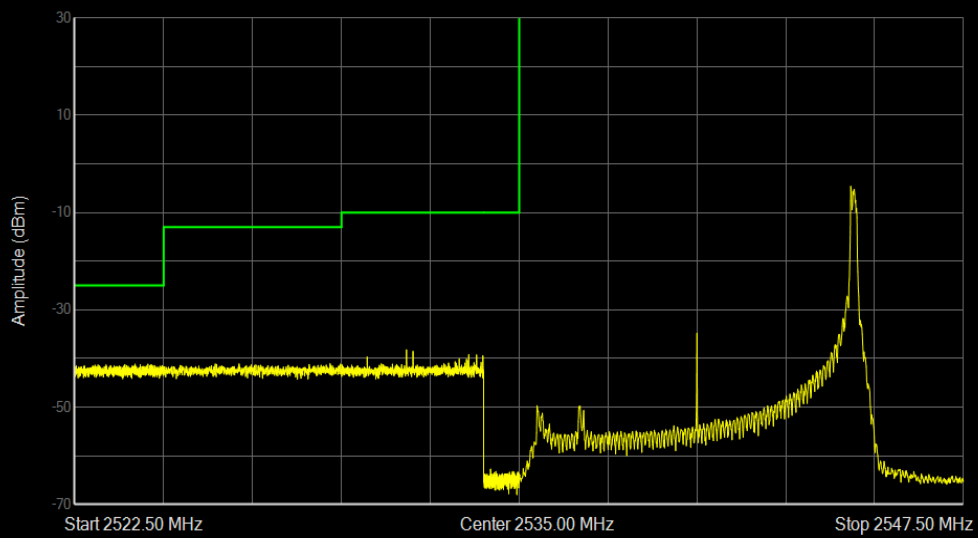
Band41 QPSK BW=10MHz Channel=40090 RB Size=1 Position=#Max
