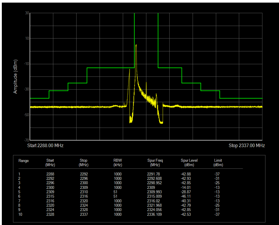
Band40a QPSK BW=5MHz Channel=38775 RB Size=1 Position=#Max
