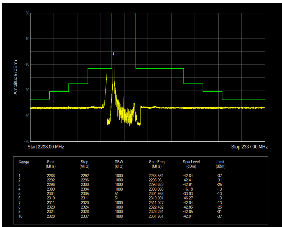
Band40a QPSK BW=5MHz Channel=38725 RB Size=1 Position=#Max
