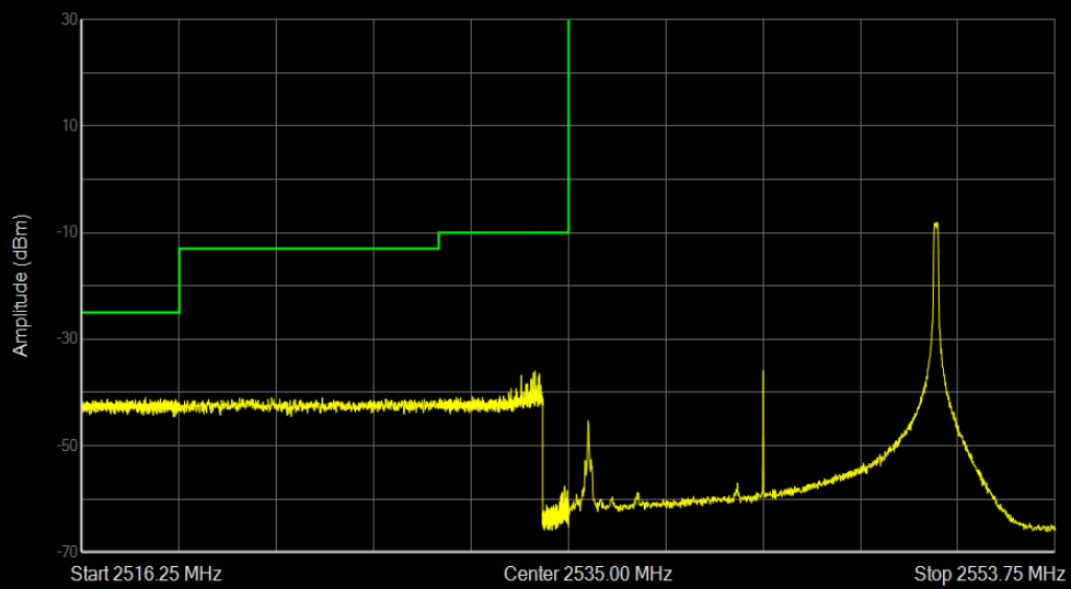
Band41 16QAM BW=15MHz Channel=40115 RB Size=1 Position=#Max
