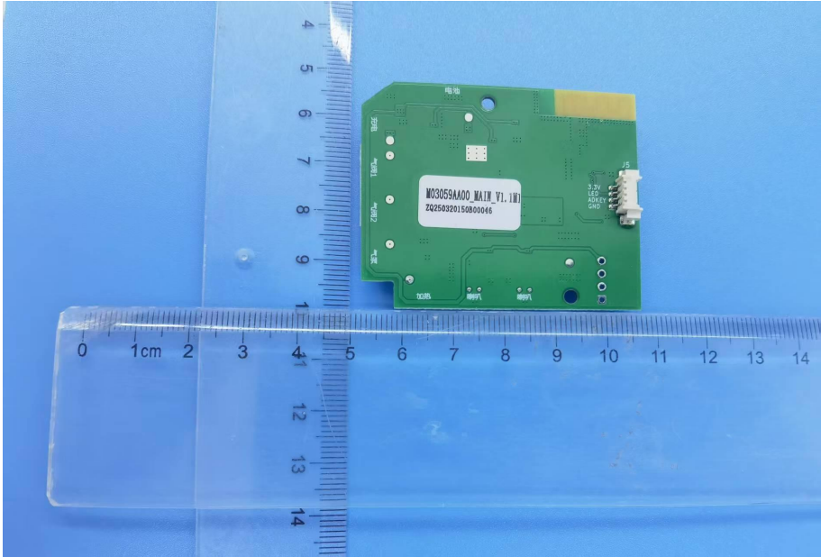
INTERNAL PHOTO OF SAMPLE PCB
