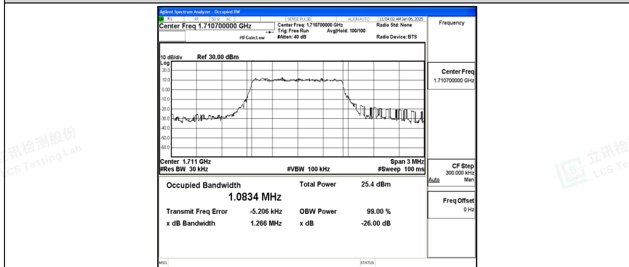
Band66-1.4MHz-16QAM-131979-6-0-Low-1.0834-1.266-PASS
