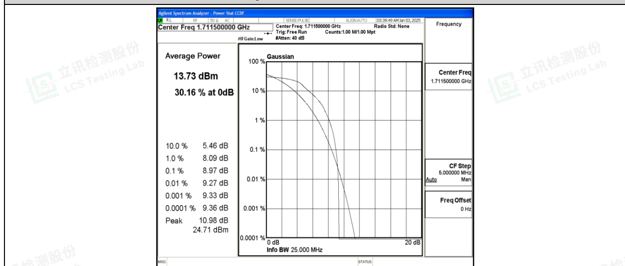
Band66-3MHz-16QAM-131987-6-0-Low-8.97-&lt;=13-PASS
