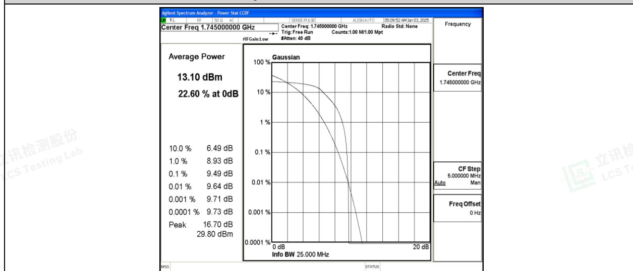
Band66-15MHz-QPSK-132322-6-0-Low-9.49-&lt;=13-PASS
