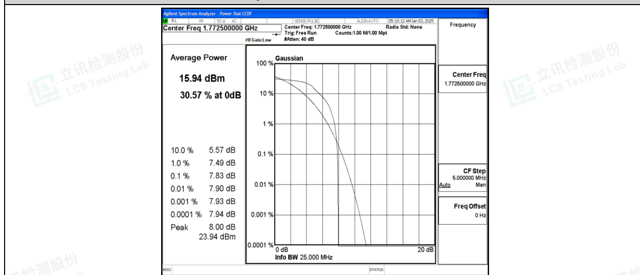
Band66-15MHz-QPSK-132597-1-0-High-7.83-&lt;=13-PASS
