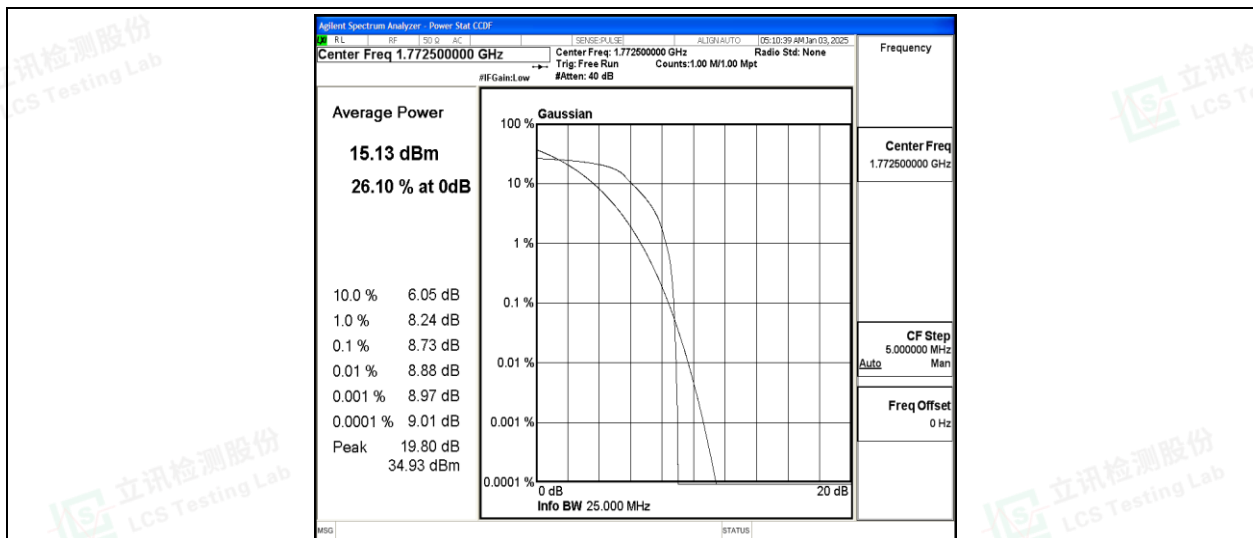
Band66-15MHz-16QAM-132597-6-0-High-8.73-&lt;=13-PASS
