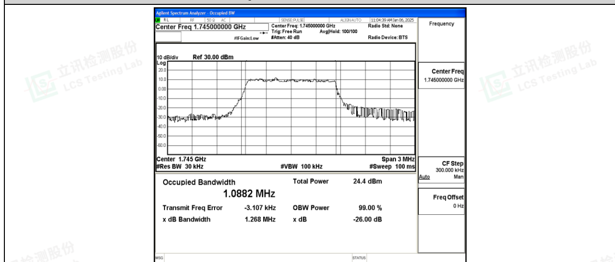
Band66-1.4MHz-16QAM-132322-6-0-Low-1.0882-1.268-PASS
