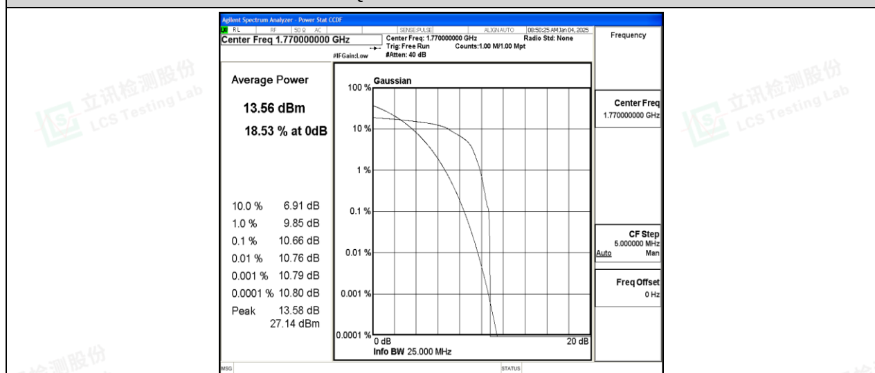
Band66-20MHz-16QAM-132572-1-0-High-10.66-&lt;=13-PASS
