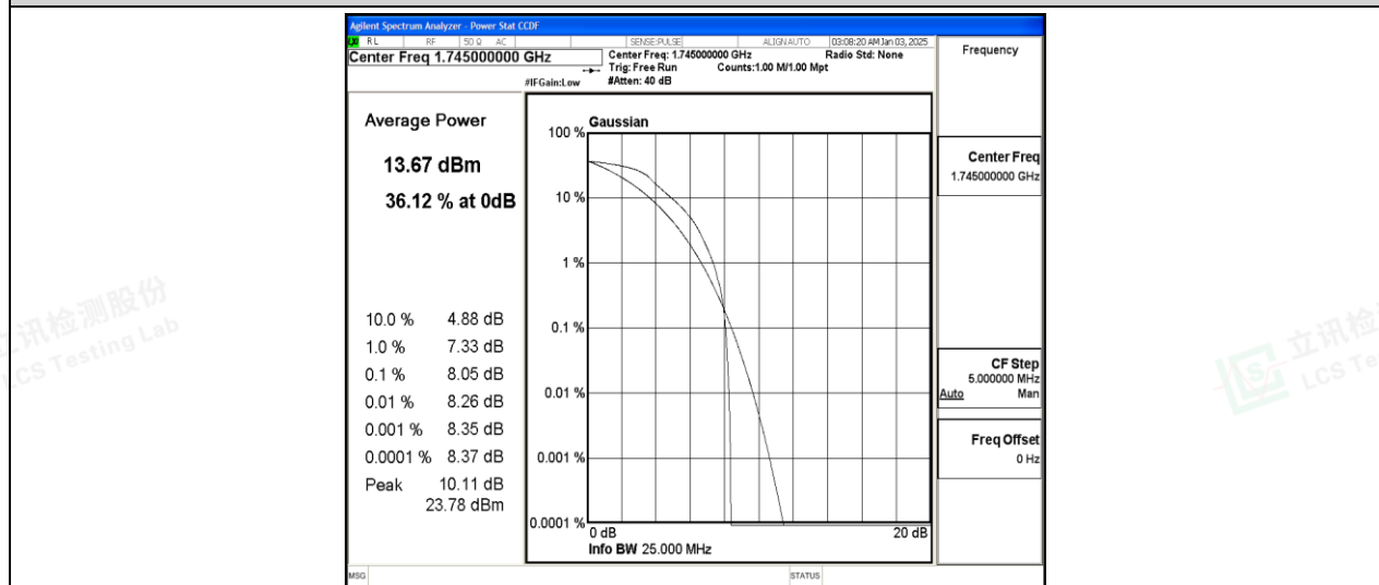
Band66-q 1.4MHz-16QAM-132322-6-0-Low-8.05-&lt;=13-PASS
