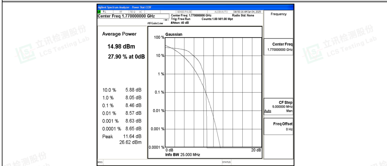
Band66-20MHz-QPSK-132572-1-0-High-8.46-&lt;=13-PASS
