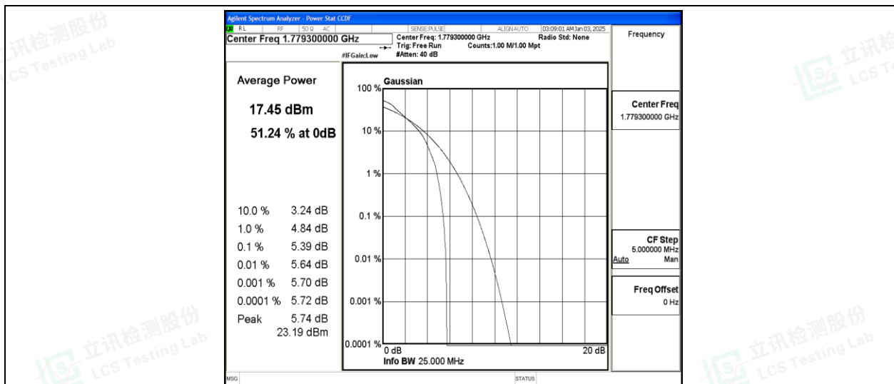
Band66-1.4MHz-16QAM-132665-6-0-High-5.39-&lt;=13-PASS
