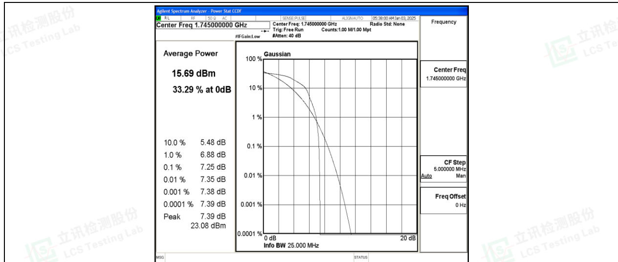
Band66-20MHz-16QAM-132322-1-0-Low-7.25-&lt;=13-PASS
