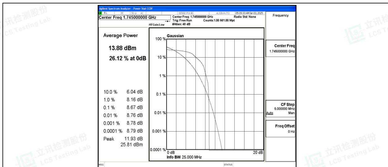
Band66-15MHz-QPSK-132322-1-0-Low-8.67-&lt;=13-PASS
