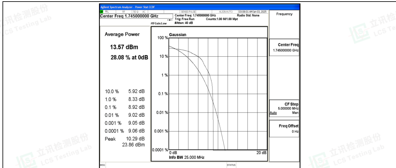
Band66-1.4MHz-16QAM-132322-1-0-Low-8.92-&lt;=13-PASS
