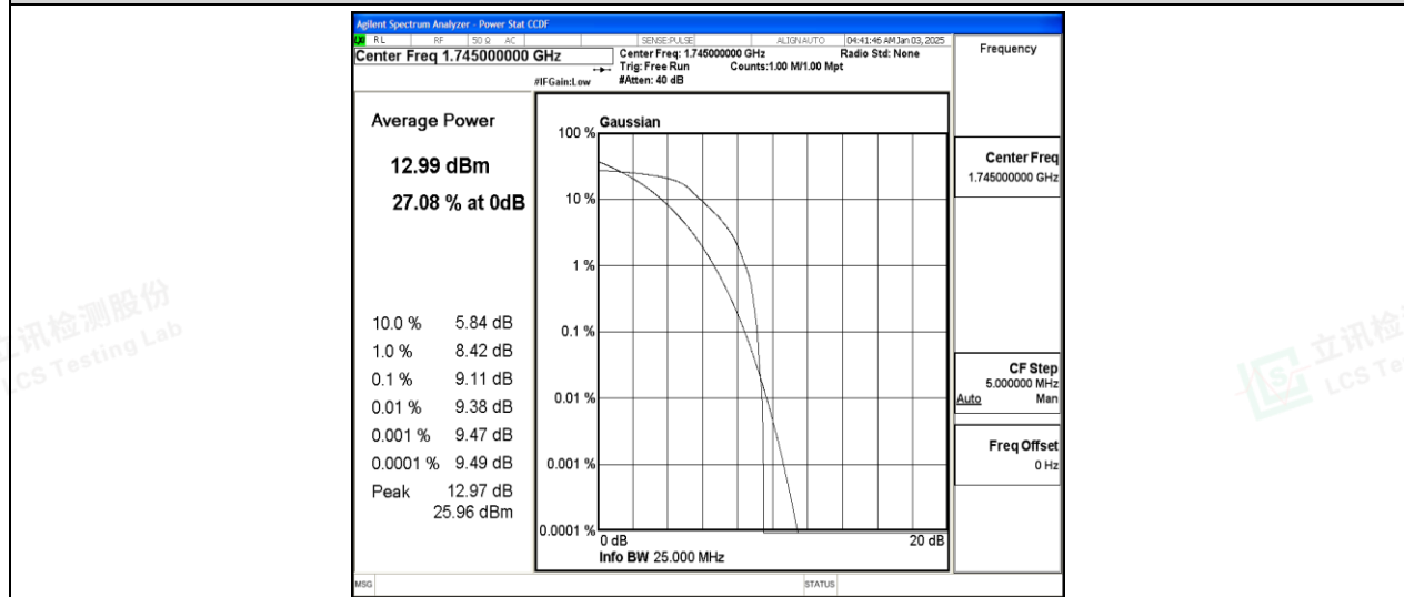
Band66-10MHz-16QAM-132322-6-0-Low-9.11-&lt;=13-PASS
