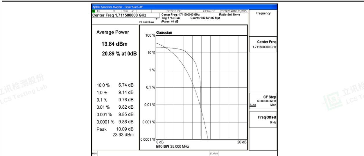
Band66-3MHz-QPSK-131987-1-0-Low-9.76-&lt;=13-PASS
