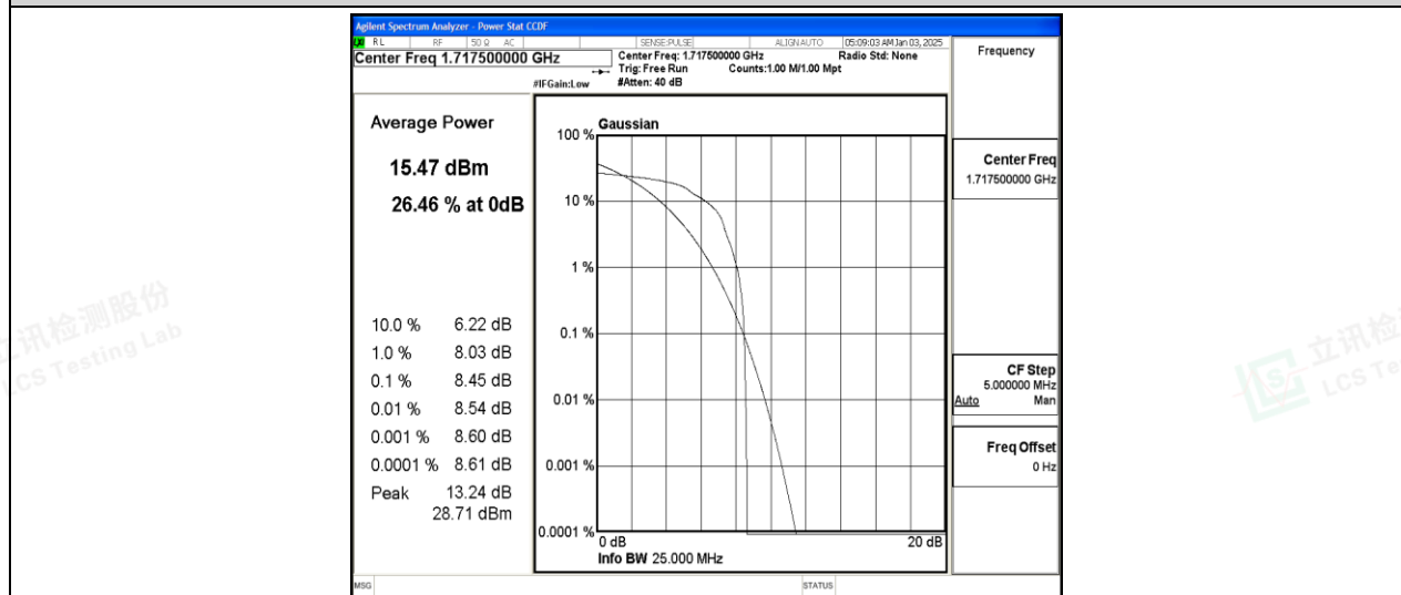
Band66-15MHz-16QAM-132047-1-0-Low-8.45-13-PASS
