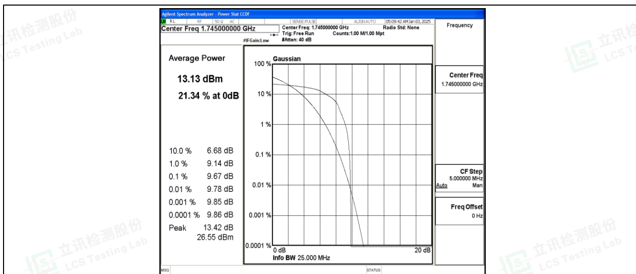
Band66-15MHz-16QAM-132322-1-0-Low-9.67-&lt;=13-PASS
