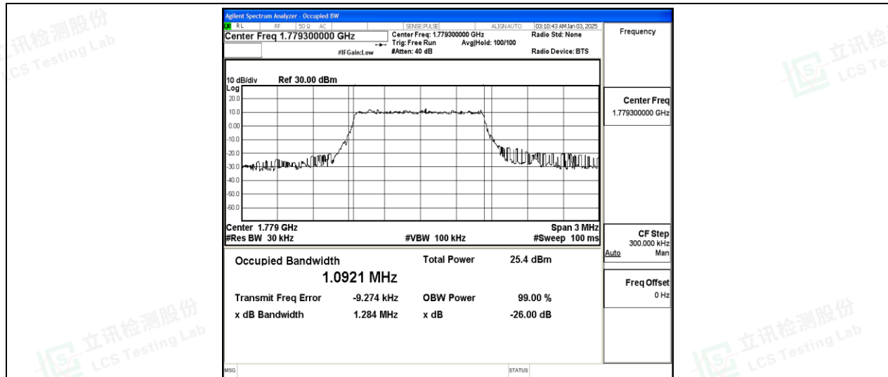
Band66-1.4MHz-QPSK-132665-6-0-High-1.0921-1.284-PASS
