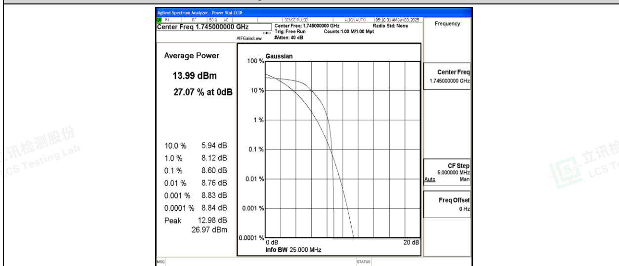
Band66-15MHz-16QAM-132322-6-0-Low-8.60-&lt;=13-PASS
