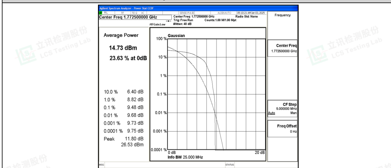
Band66-15MHz-16QAM-132597-1-0-High-9.48-&lt;=13-PASS
