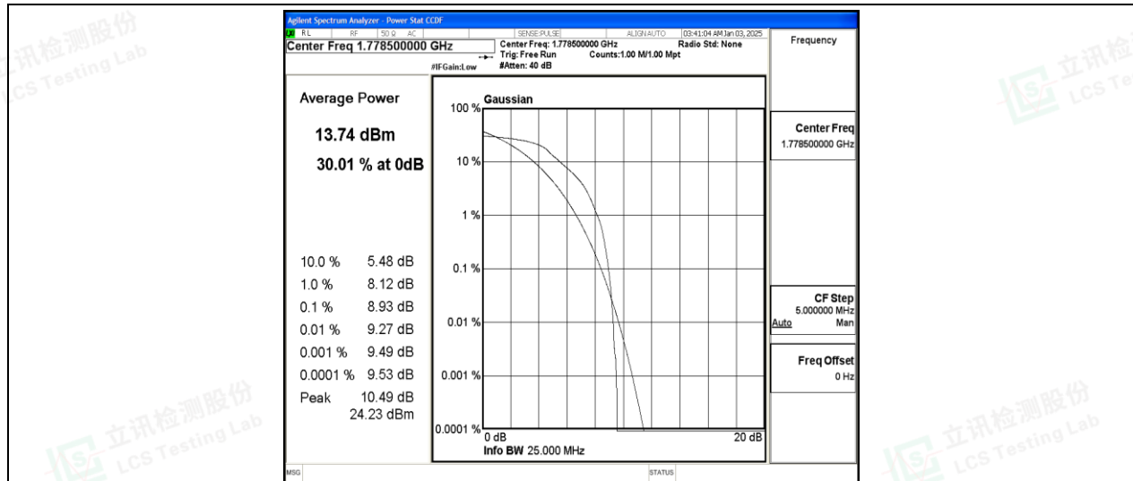
Band66-3MHz-QPSK-132657-6-0-High-8.93-&lt;=13-PASS
