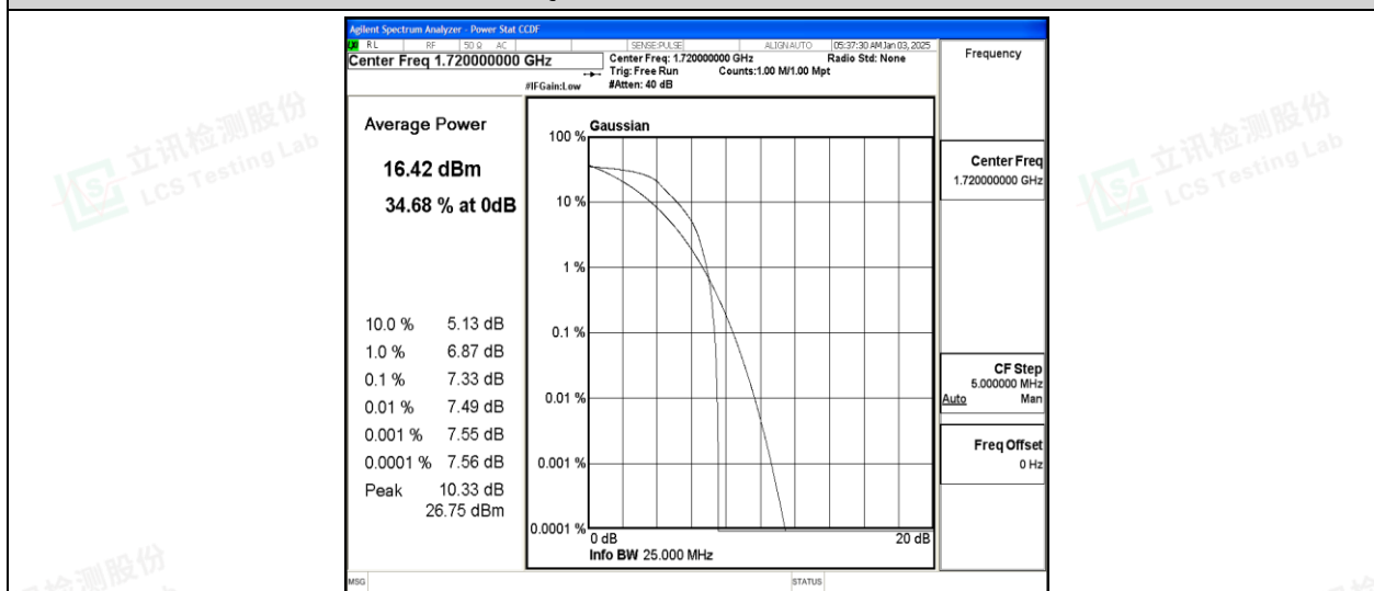
Band66-20MHz-QPSK-132072-6-0-Low-7.33-&lt;=13-PASS
