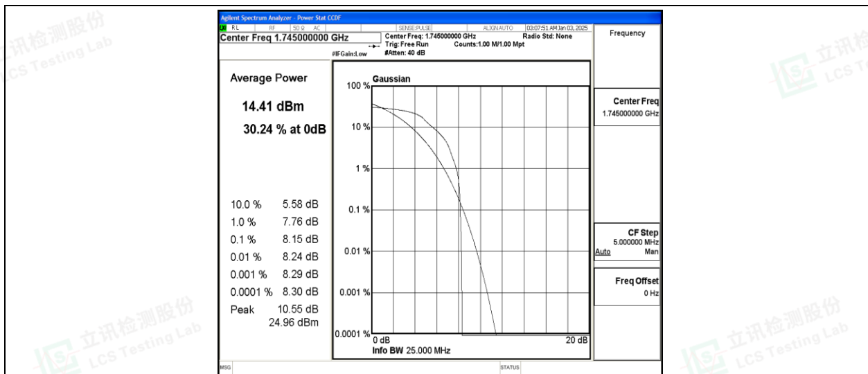
Band66-1.4MHz-QPSK-132322-1-0-Low-8.15-&lt;=13-PASS
