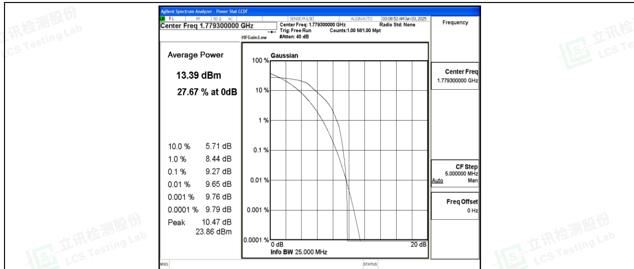
Band66-1.4MHz-QPSK-132665-6-0-High-9.27-&lt;=13-PASS
