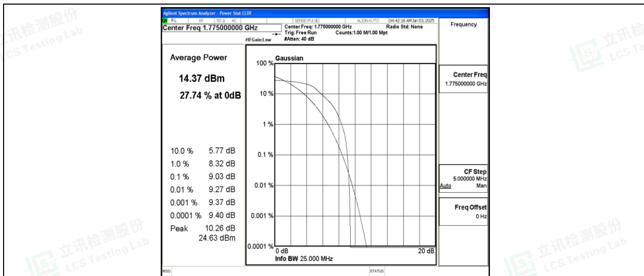
Band66-10MHz-QPSK-132622-6-0-High-9.03-&lt;=13-PASS
