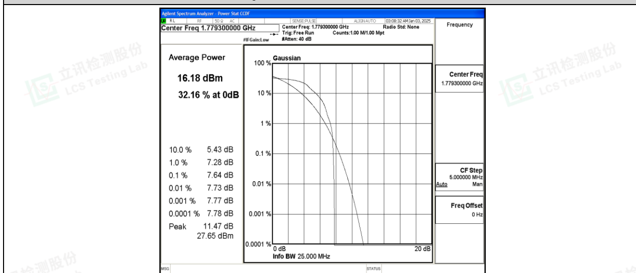
Band66-1.4MHz-QPSK-132665-1-0-High-7.64-&lt;=13-PASS
