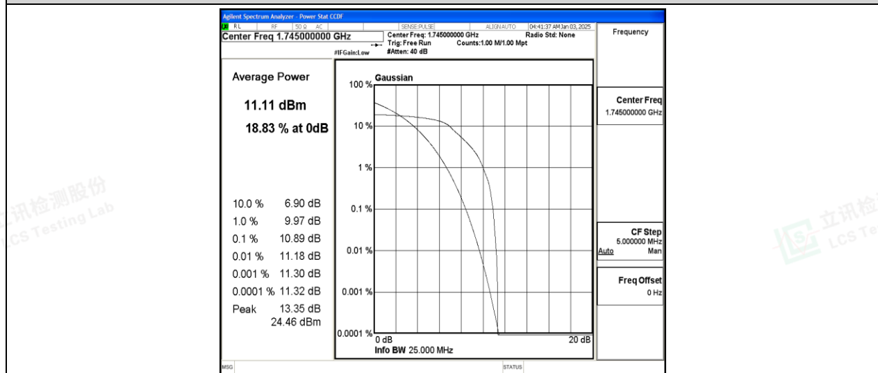
Band66-10MHz-QPSK-132322-6-0-Low-10.89-≤13-PASS
