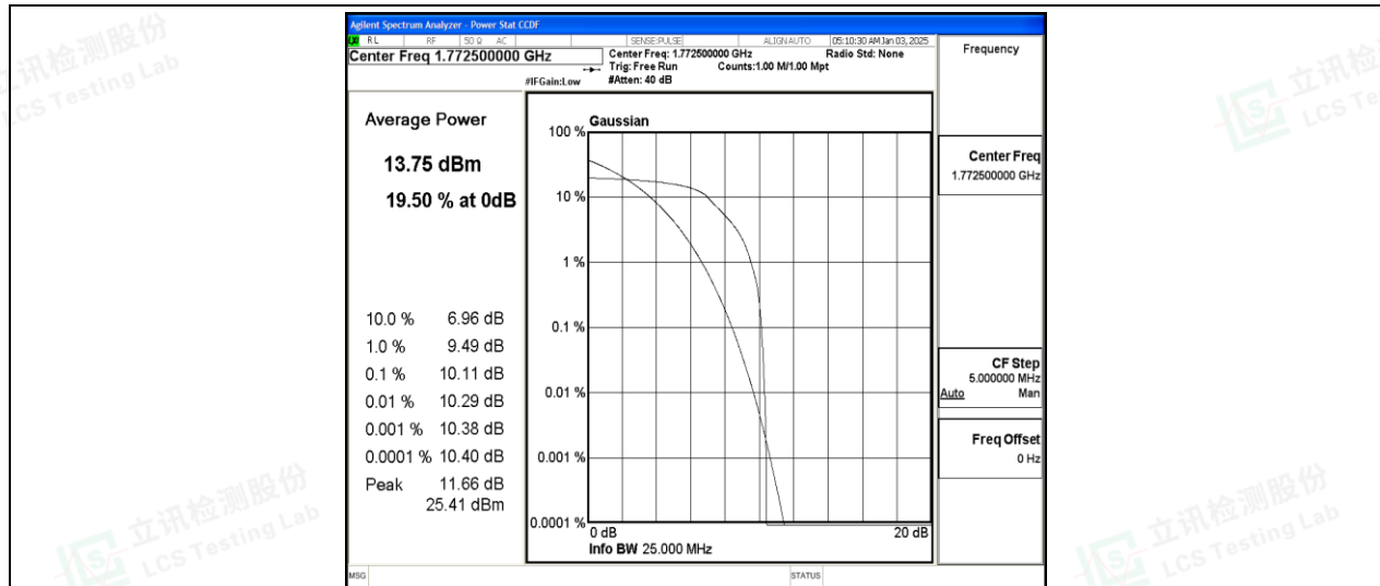
Band66-15MHz-QPSK-132597-6-0-High-10.11-13-PASS
