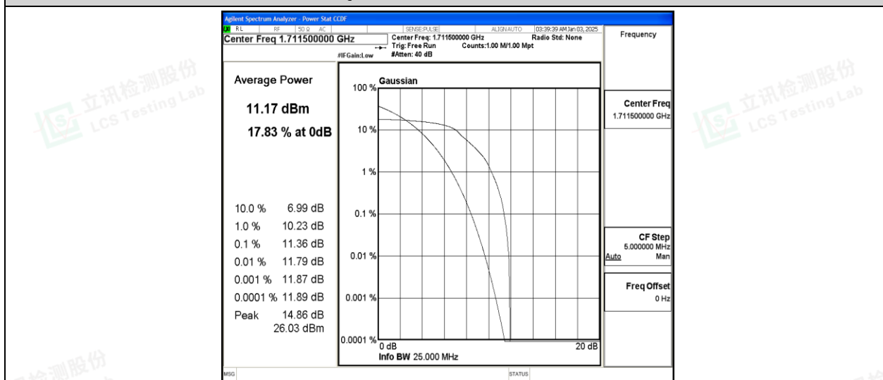
Band66-3MHz-QPSK-131987-6-0-Low-11.36-&lt;=13-PASS
