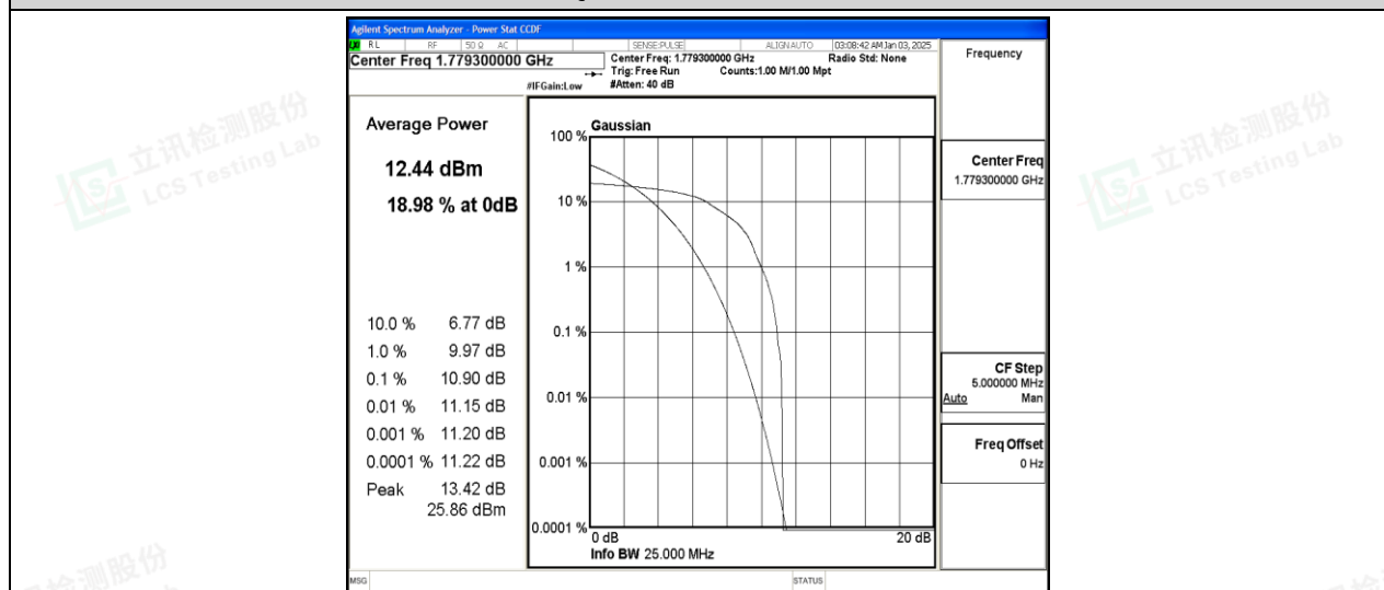
Band66-1.4MHz-16QAM-132665-1-0-High-10.90-&lt;=13-PASS
