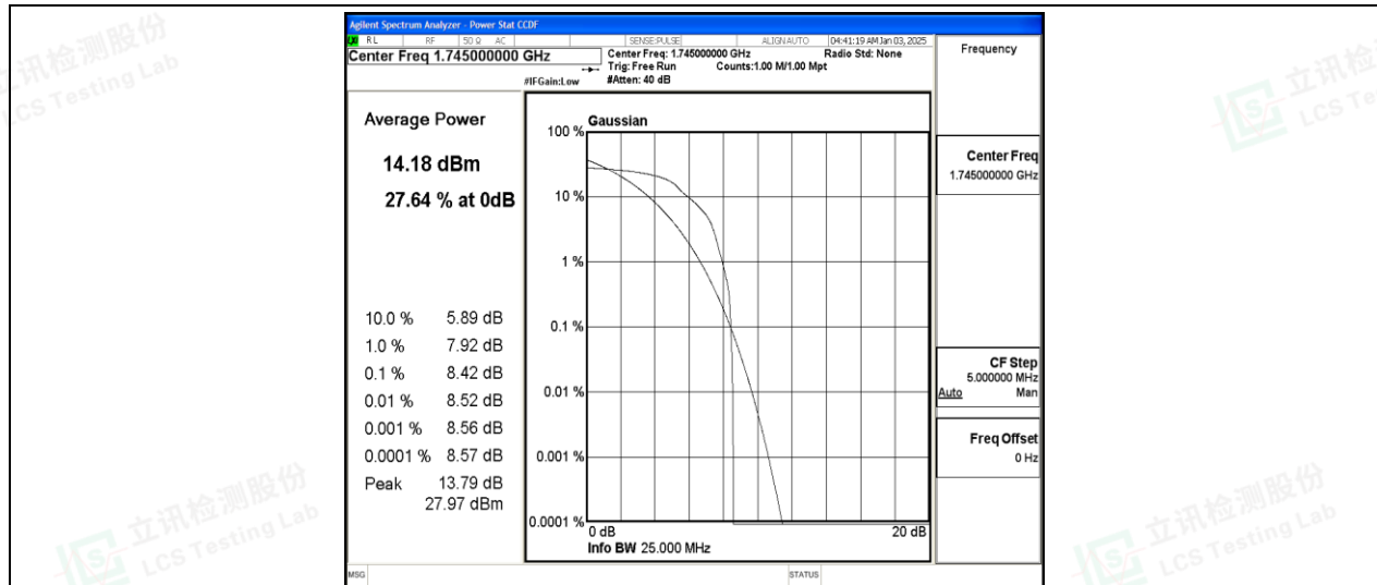
Band66-10MHz-QPSK-132322-1-0-Low-8.42-≤13-PASS
