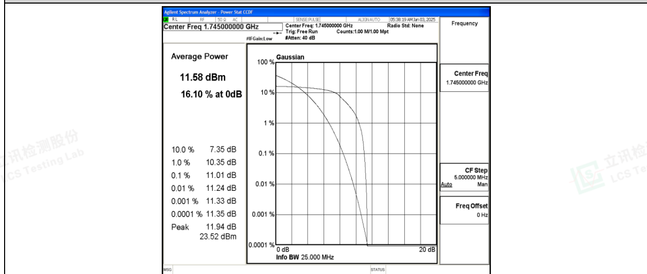
Band66-20MHz-16QAM-132322-6-0-Low-11.01-&lt;=13-PASS
