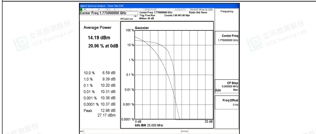
Band66-10MHz-16QAM-132622-1-0-High-10.20-&lt;=13-PASS
