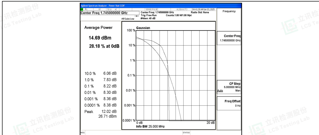
Band66-10MHz-16QAM-132322-1-0-Low-8.22-&lt;=13-PASS
