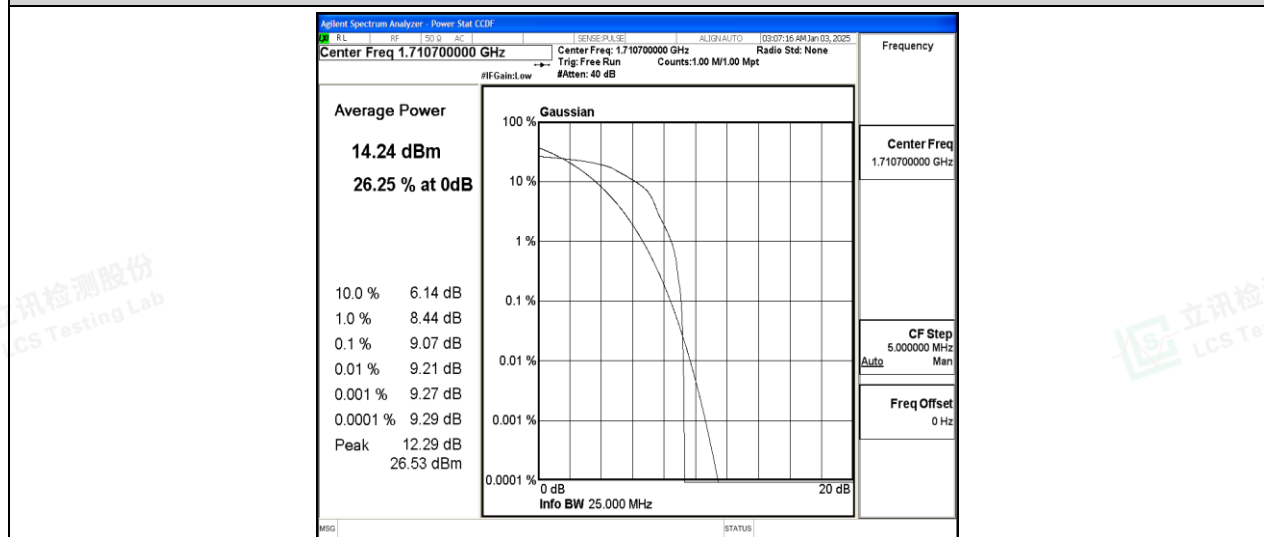
Band66-1.4MHz-16QAM-131979-1-0-Low-9.07-&lt;=13-PASS
