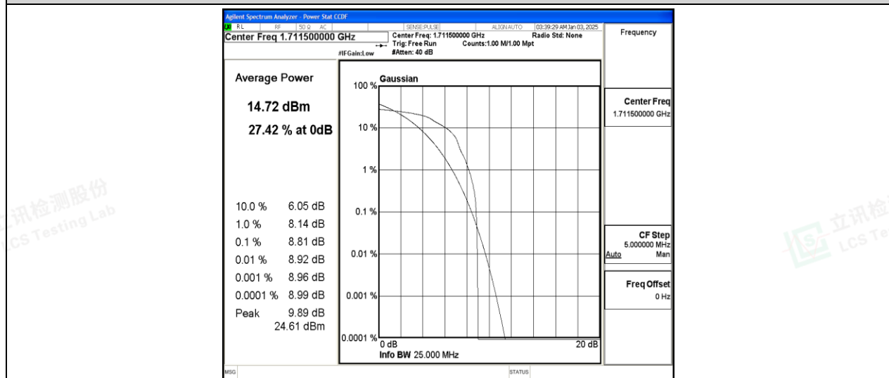
Band66-3MHz-16QAM-131987-1-0-Low-8.81-&lt;=13-PASS
