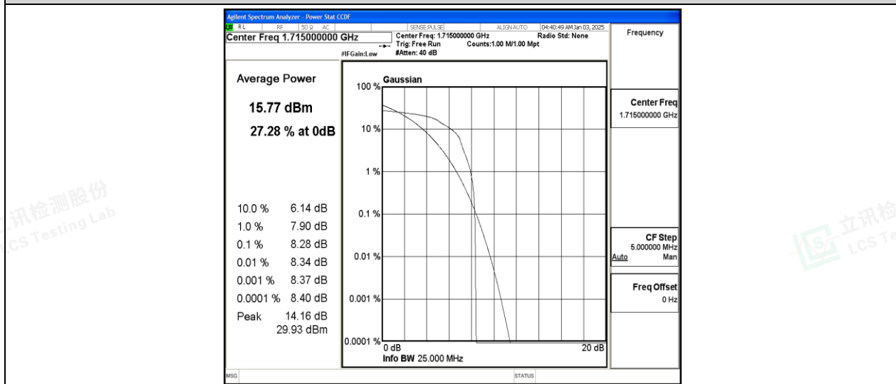
Band66-10MHz-16QAM-132022-1-0-Low-8.28-&lt;=13-PASS
