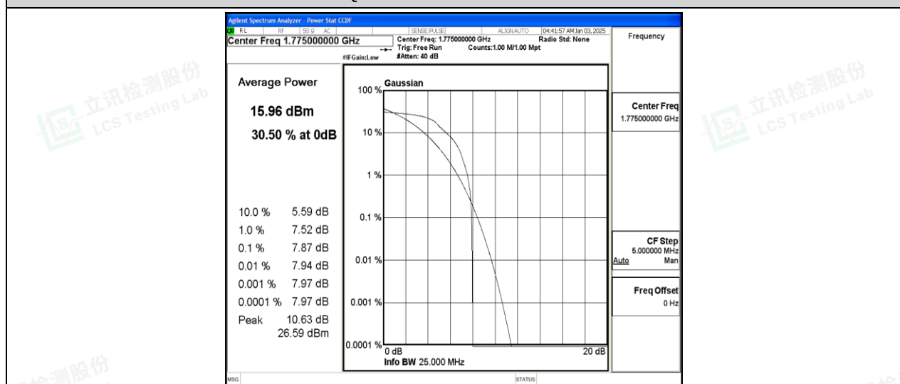
Band66-10MHz-QPSK-132622-1-0-High-7.87-≤13-PASS
