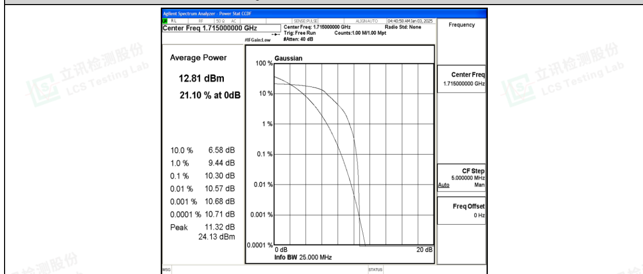
Band66-10MHz-QPSK-132022-6-0-Low-10.30-&lt;=13-PASS
