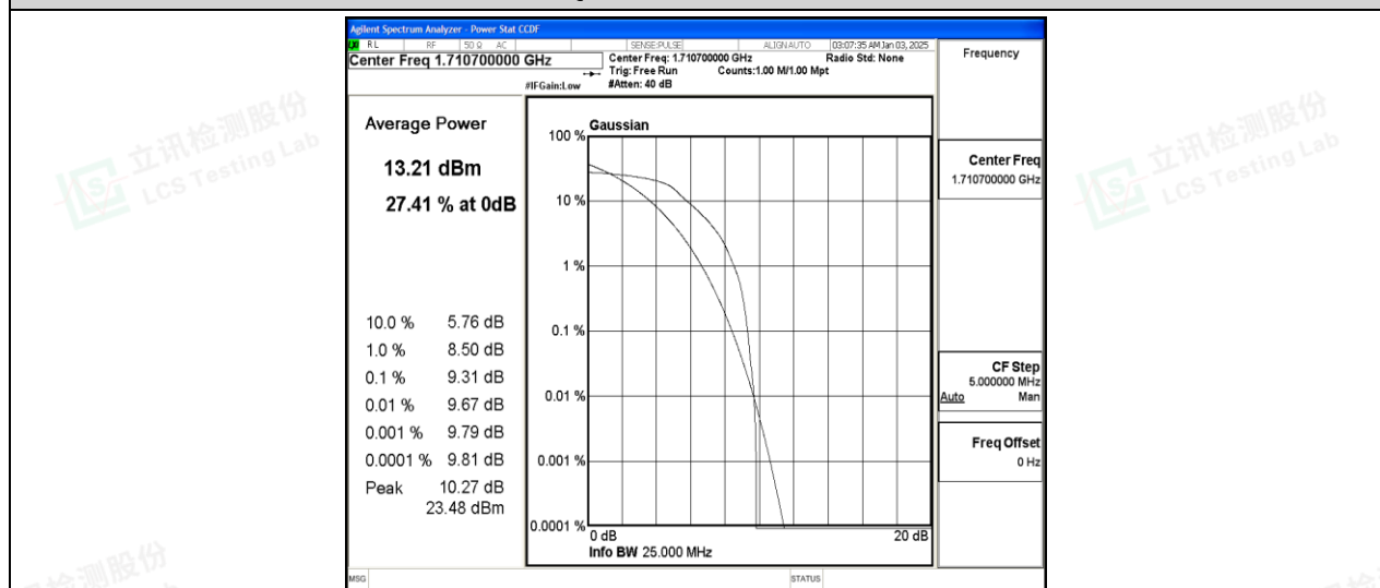
Band66-1.4MHz-16QAM-131979-6-0-Low-9.31-&lt;=13-PASS
