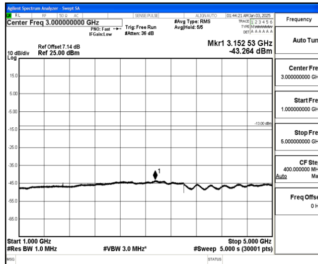
Band26-5MHz-16QAM-27015-1-0-High-1000-5000--43.26-PASS
