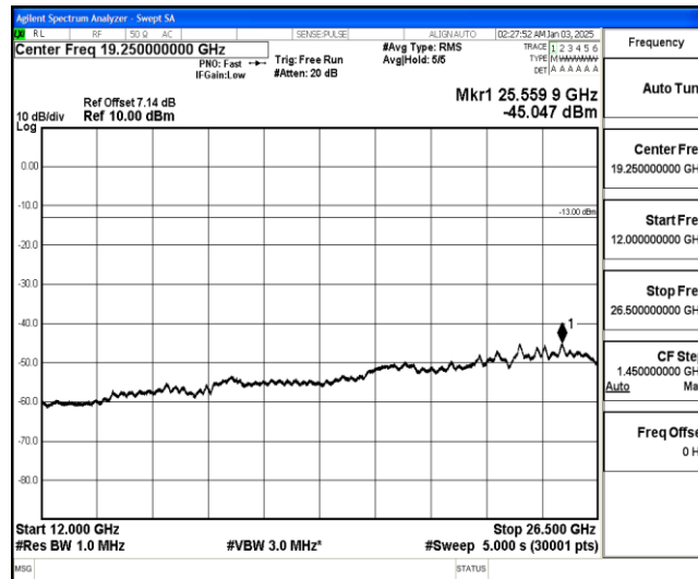
Band26-10MHz-16QAM-26915-1-0-Low-12000-26500--45.05-PASS
