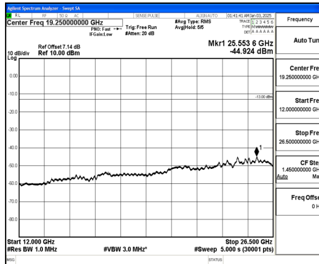
Band26-5MHz-16QAM-26915-1-0-Low-12000-26500--44.92-PASS
