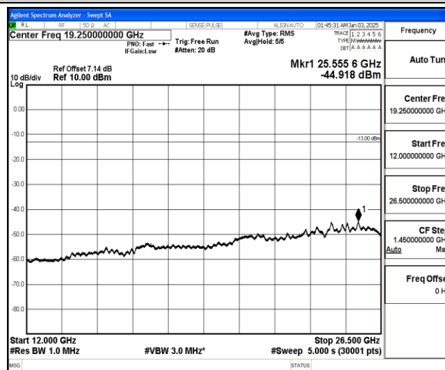
Band26-5MHz-16QAM-27015-1-0-High-12000-26500--44.92-PASS
