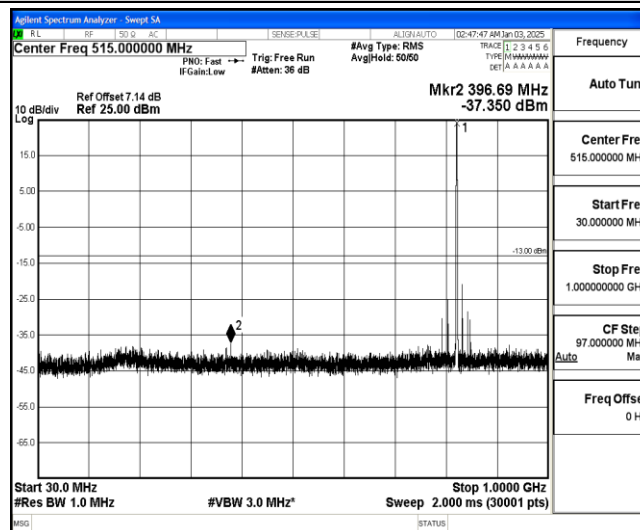
Band26-15MHz-QPSK-26865-1-0-Low-30-1000--37.35-PASS
