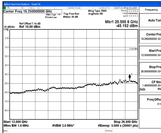
Band26-15MHz-QPSK-26965-1-0-High-12000-26500--45.15-PASS
