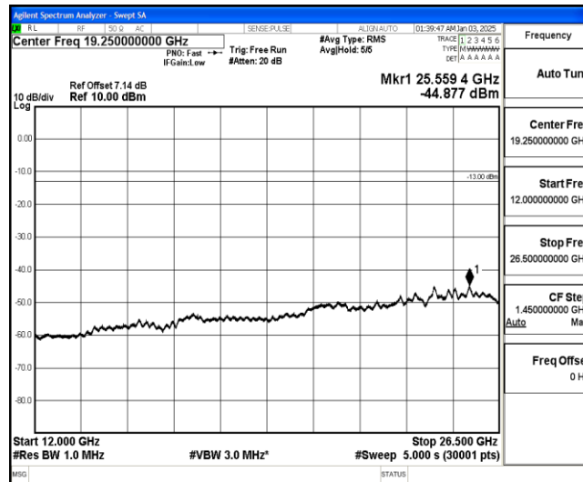
Band26-5MHz-QPSK-26915-1-0-Low-12000-26500--44.88-PASS
