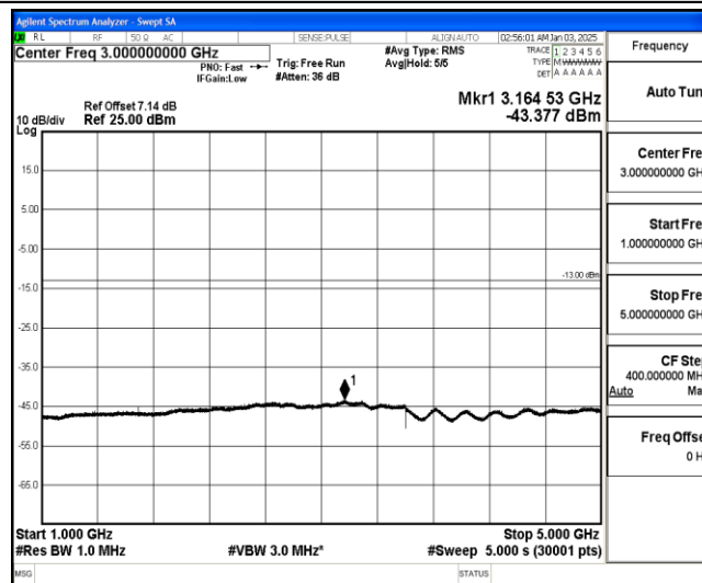
Band26-15MHz-QPSK-26965-1-0-High-1000-5000--43.38-PASS
