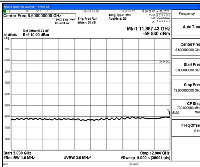
Band26-10MHz-QPSK-26740-1-0-Low-5000-12000--59.53-PASS
