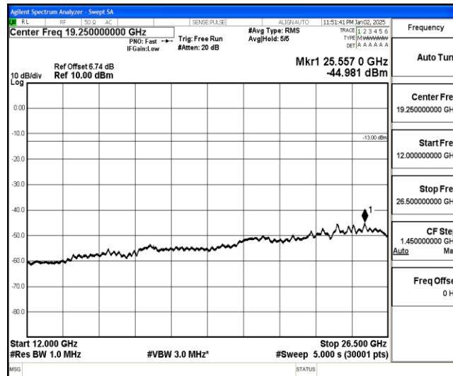
Band26-5MHz-16QAM-26715-1-0-Low-12000-26500--44.98-PASS
