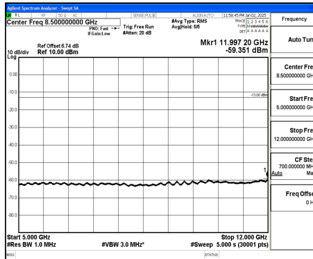
Band26-5MHz-16QAM-26765-1-0-High-5000-12000--59.35-PASS
