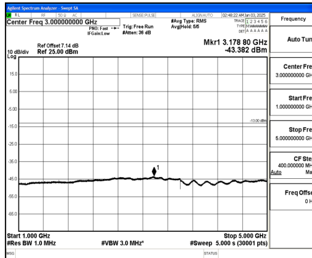
Band26-15MHz-QPSK-26865-1-0-Low-1000-5000--43.38-PASS
