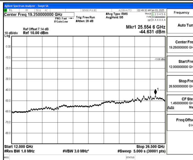
Band26-15MHz-QPSK-26865-1-0-Low-12000-26500--44.63-PASS
