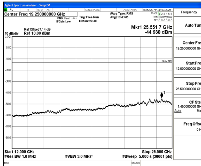
Band26-15MHz-QPSK-26915-1-0-Low-12000-26500--44.94-PASS
