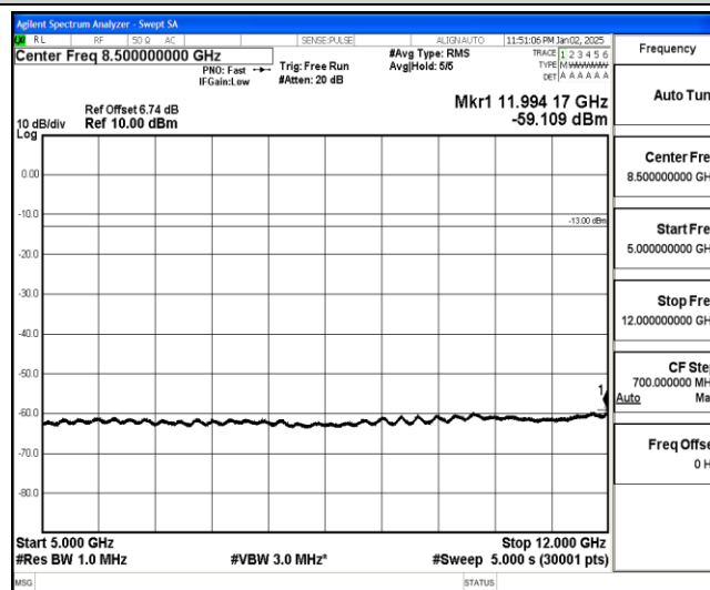
Band26-5MHz-16QAM-26715-1-0-Low-5000-12000--59.11-PASS
