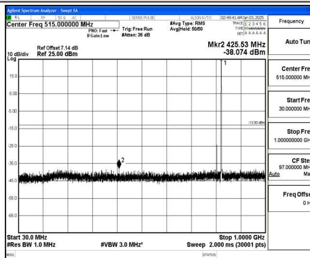
Band26-15MHz-16QAM-26865-1-0-Low-30-1000--38.07-PASS
