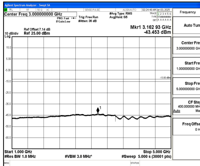
Band26-10MHz-QPSK-26915-1-0-Low-1000-5000--43.45-PASS
