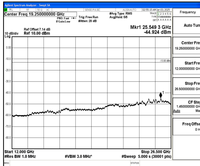
Band26-15MHz-16QAM-26915-1-0-Low-12000-26500--44.92-PASS
