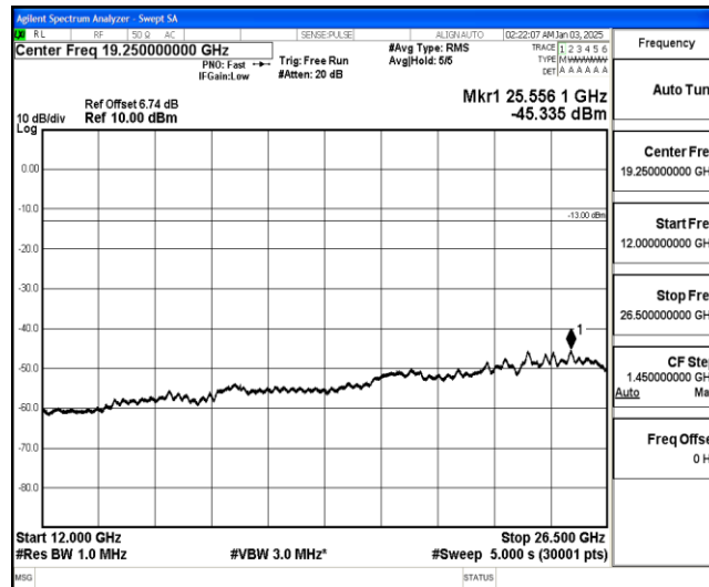
Band26-10MHz-QPSK-26840-1-0-Low-12000-26500--45.34-PASS
