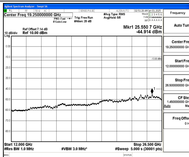
Band26-15MHz-16QAM-26865-1-0-Low-12000-26500--44.91-PASS
