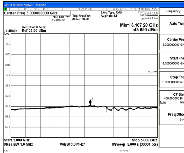
Band26-5MHz-16QAM-26715-1-0-Low-1000-5000--43.66-PASS
