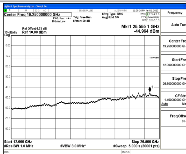
Band26-5MHz-16QAM-26765-1-0-High-12000-26500--44.96-PASS
