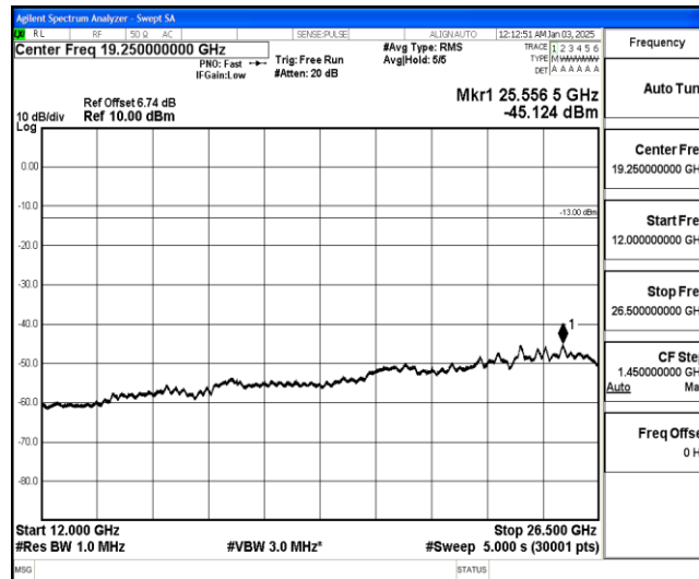
Band26-10MHz-16QAM-26740-1-0-Low-12000-26500--45.12-PASS
