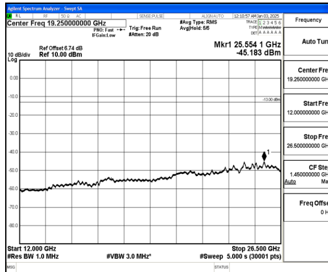
Band26-10MHz-QPSK-26740-1-0-Low-12000-26500--45.18-PASS
