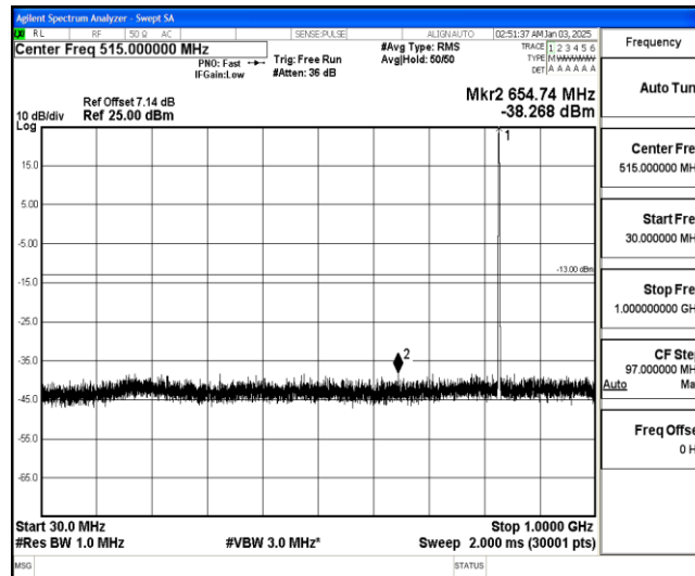
Band26-15MHz-QPSK-26915-1-0-Low-30-1000--38.27-PASS
