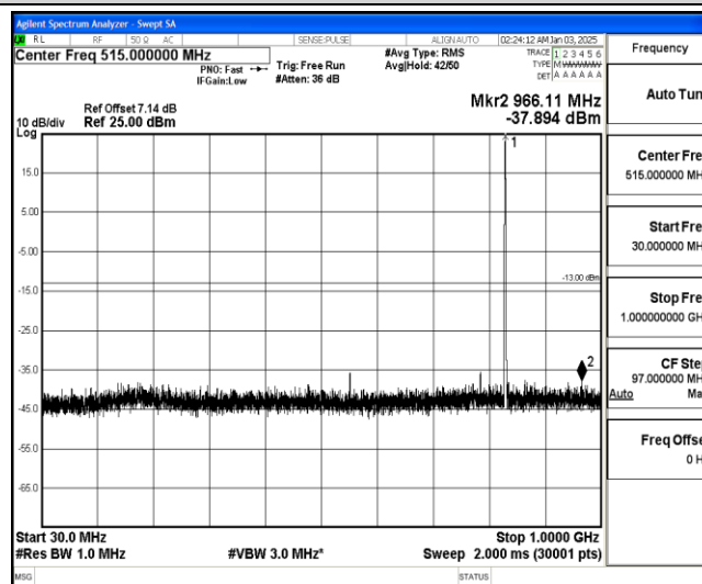
Band26-10MHz-QPSK-26915-1-0-Low-30-1000--37.89-PASS
