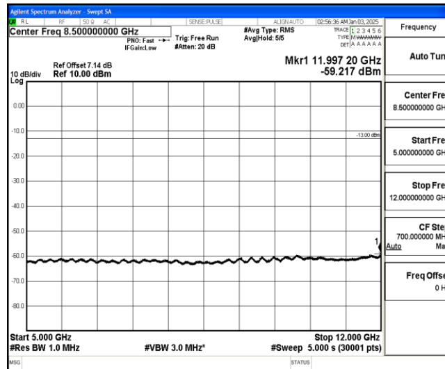
Band26-15MHz-QPSK-26965-1-0-High-5000-12000--59.22-PASS
