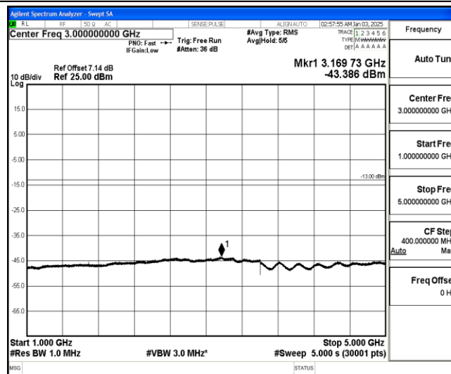
Band26-15MHz-16QAM-26965-1-0-High-1000-5000--43.39-PASS
