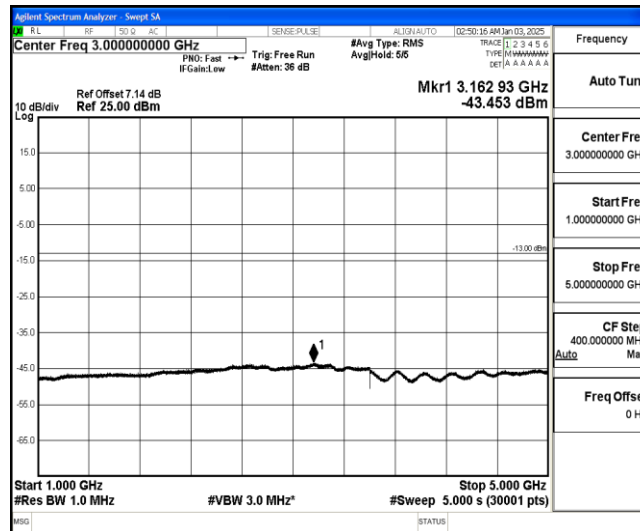
Band26-15MHz-16QAM-26865-1-0-Low-1000-5000--43.45-PASS
