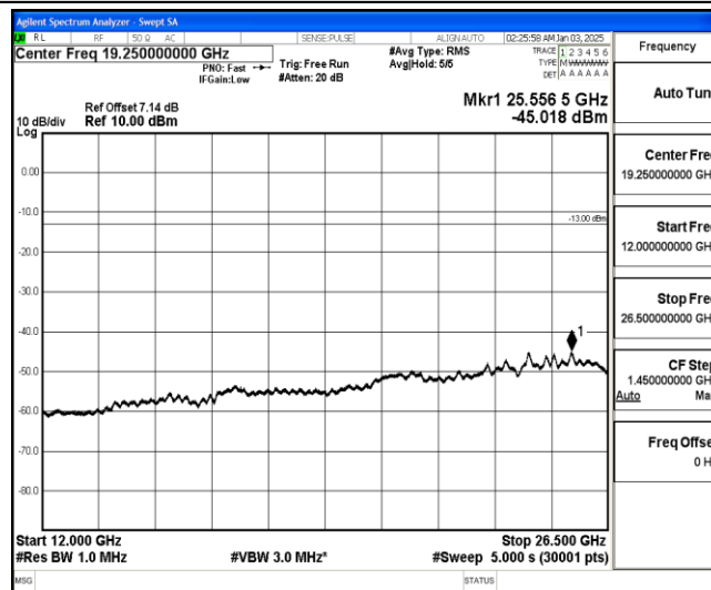
Band26-10MHz-QPSK-26915-1-0-Low-12000-26500--45.02-PASS
