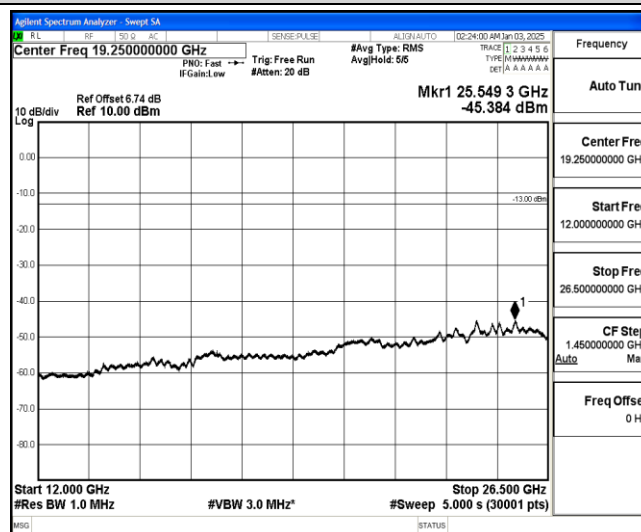
Band26-10MHz-16QAM-26840-1-0-Low-12000-26500--45.38-PASS
