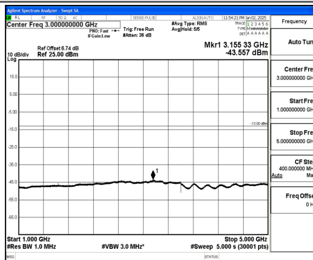
Band26-5MHz-16QAM-26740-1-0-Low-1000-5000--43.56-PASS
