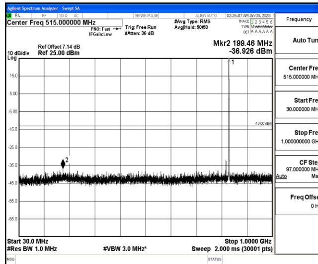
Band26-10MHz-16QAM-26915-1-0-Low-30-1000--36.93-PASS
