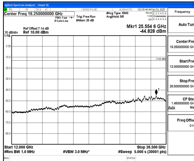
Band26-10MHz-QPSK-26990-1-0-High-12000-26500--44.83-PASS
