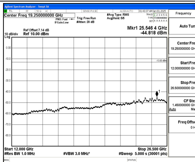
Band26-5MHz-QPSK-27015-1-0-High-12000-26500--44.82-PASS
