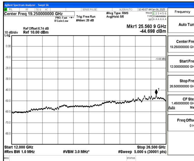
Band26-5MHz-16QAM-26815-1-0-Low-12000-26500--44.7-PASS
