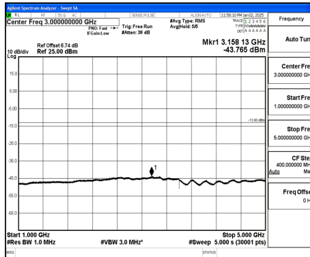
Band26-5MHz-16QAM-26765-1-0-High-1000-5000--43.77-PASS
