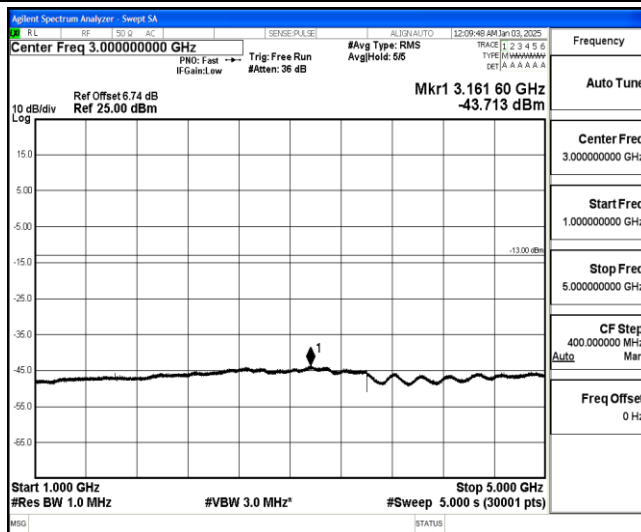
Band26-10MHz-QPSK-26740-1-0-Low-1000-5000--43.71-PASS
