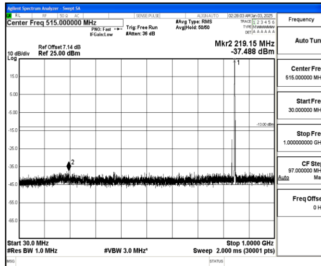
Band26-10MHz-QPSK-26990-1-0-High-30-1000--37.49-PASS
