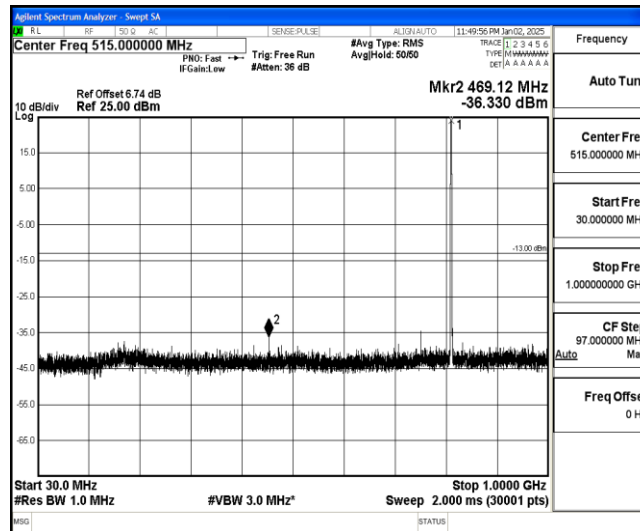
Band26-5MHz-16QAM-26715-1-0-Low-30-1000--36.33-PASS
