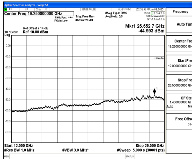
Band26-10MHz-16QAM-26990-1-0-High-12000-26500--44.99-PASS
