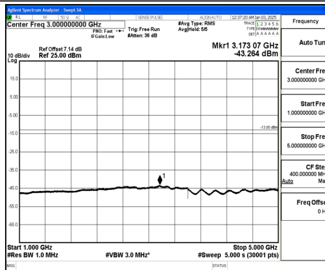
Band26-1.4MHz-16QAM-26915-1-0-Low-1000-5000--43.26-PASS
