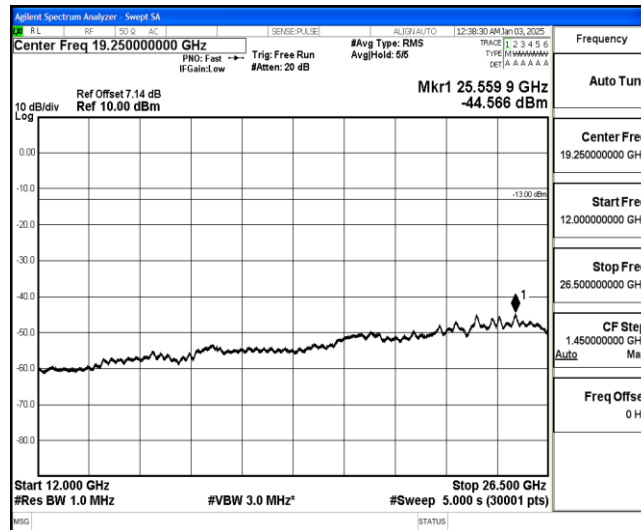
Band26-1.4MHz-16QAM-26915-1-0-Low-12000-26500--44.57-PASS
