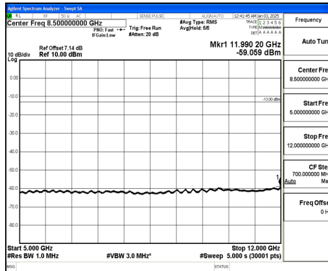
Band26-1.4MHz-16QAM-27033-1-0-High-5000-12000--59.06-PASS
