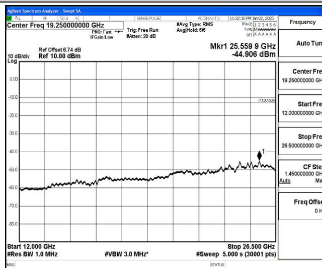
Band26-3MHz-16QAM-26775-1-0-High-12000-26500--44.91-PASS
