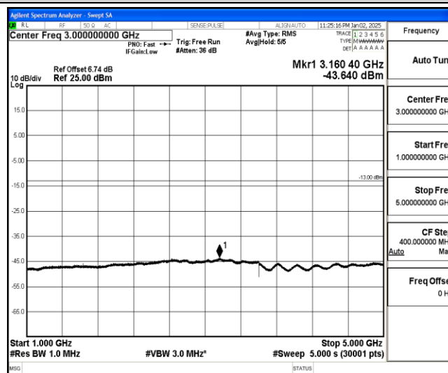
Band26-3MHz-QPSK-26740-1-0-Low-1000-5000--43.64-PASS
