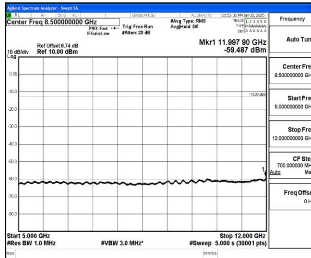
Band26-5MHz-QPSK-26740-1-0-Low-5000-12000--59.49-PASS
