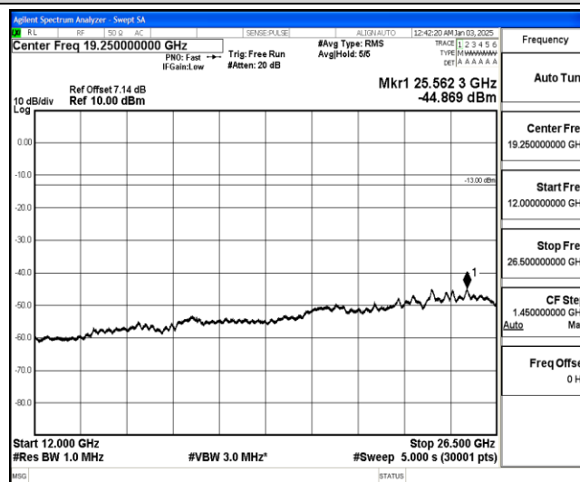
Band26-1.4MHz-16QAM-27033-1-0-High-12000-26500--44.87-PASS
