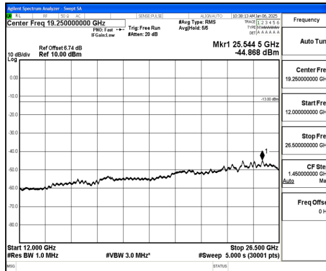
Band26-5MHz-QPSK-26815-1-0-Low-12000-26500--44.87-PASS
