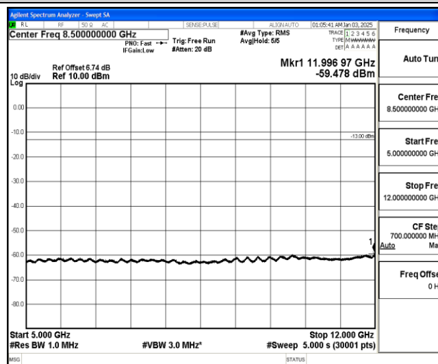
Band26-3MHz-16QAM-26805-1-0-Low-5000-12000--59.48-PASS
