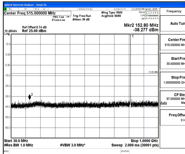
Band26-3MHz-QPSK-26705-1-0-Low-30-1000--38.28-PASS
