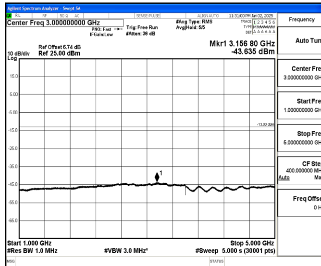
Band26-3MHz-16QAM-26775-1-0-High-1000-5000--43.64-PASS
