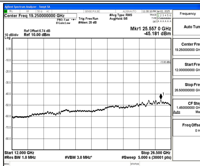
Band26-3MHz-QPSK-26775-1-0-High-12000-26500--45.18-PASS
