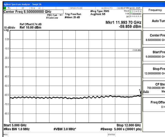
Band26-1.4MHz-16QAM-26740-1-0-Low-5000-12000--59.86-PASS
