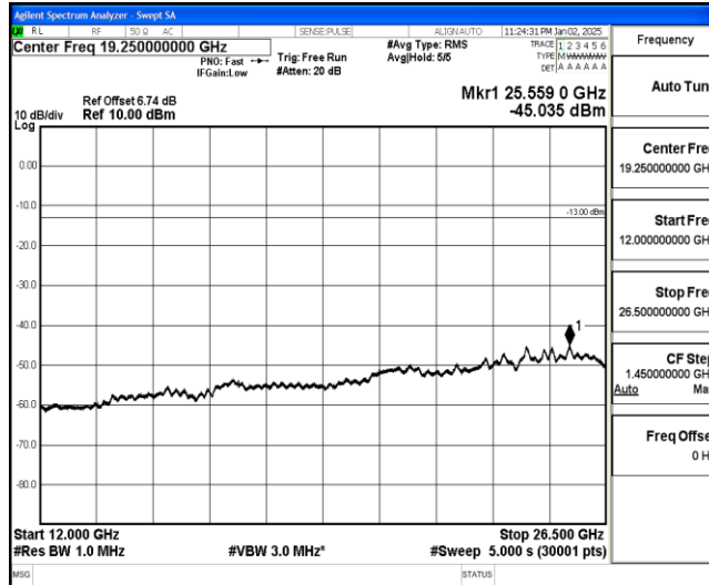
Band26-3MHz-16QAM-26705-1-0-Low-12000-26500--45.04-PASS
