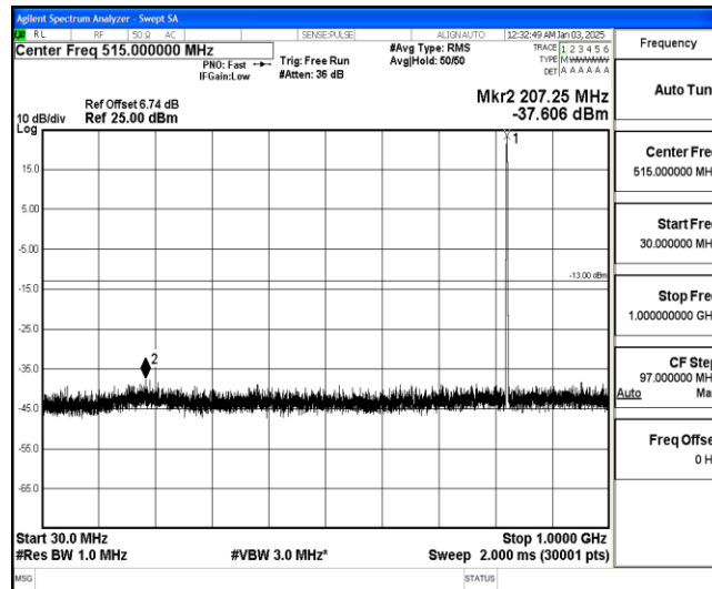
Band26-1.4MHz-16QAM-26797-1-0-Low-30-1000--37.61-PASS
