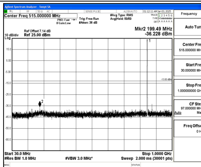
Band26-3MHz-16QAM-27025-1-0-High-30-1000--36.23-PASS
