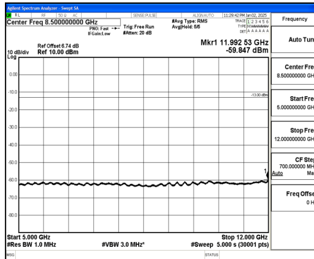
Band26-3MHz-QPSK-26775-1-0-High-5000-12000--59.85-PASS
