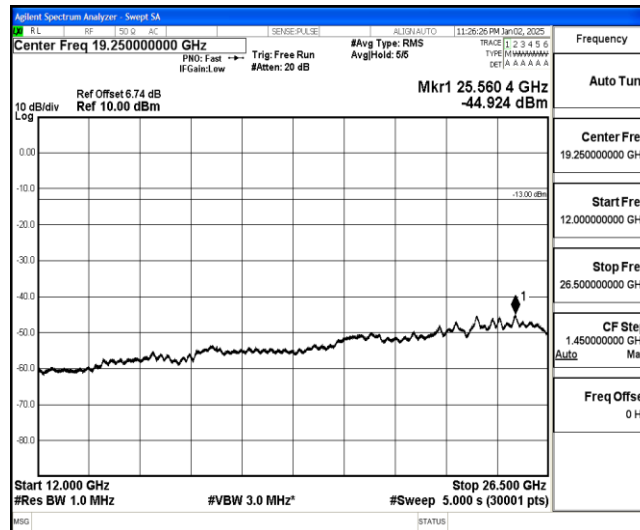
Band26-3MHz-QPSK-26740-1-0-Low-12000-26500--44.92-PASS
