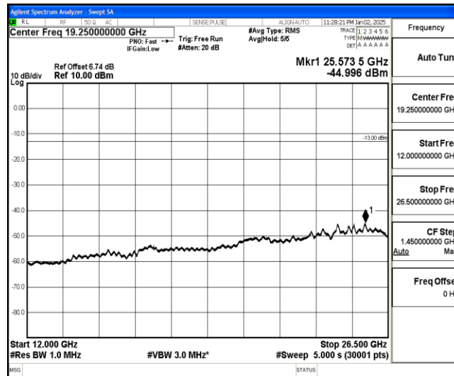
Band26-3MHz-16QAM-26740-1-0-Low-12000-26500--45-PASS
