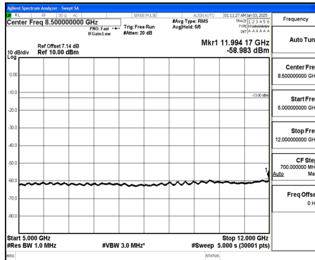
Band26-3MHz-QPSK-27025-1-0-High-5000-12000--58.98-PASS
