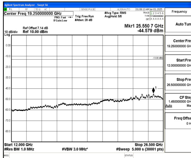
Band26-3MHz-QPSK-26915-1-0-Low-12000-26500--44.58-PASS
