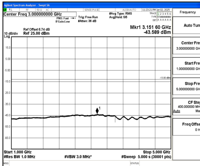
Band26-3MHz-16QAM-26705-1-0-Low-1000-5000--43.59-PASS
