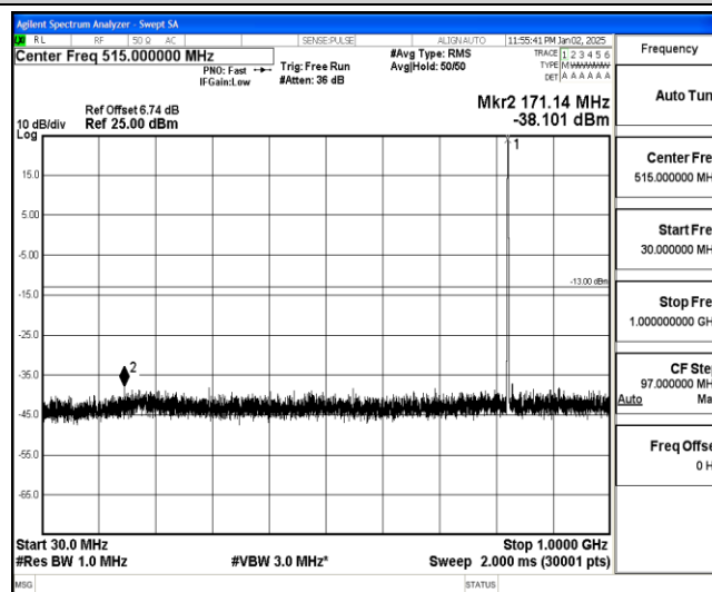
Band26-5MHz-QPSK-26765-1-0-High-30-1000--38.1-PASS
