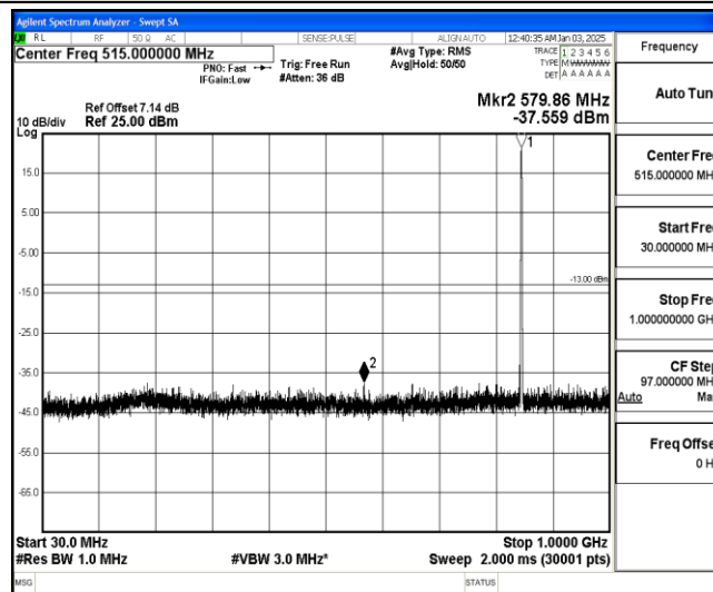
Band26-1.4MHz-16QAM-27033-1-0-High-30-1000--37.56-PASS
