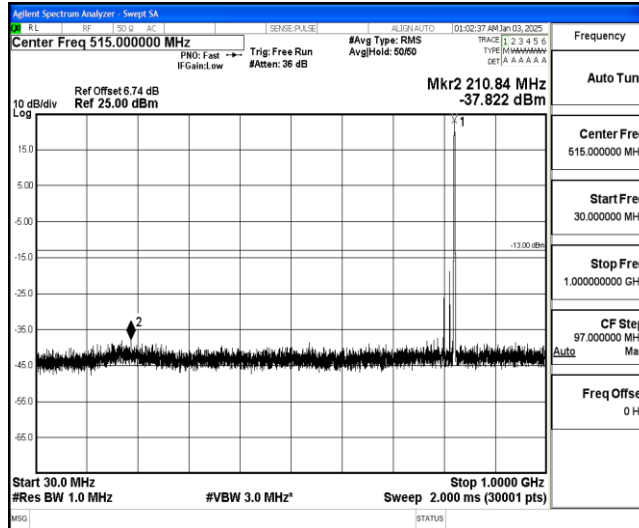
Band26-3MHz-QPSK-26805-1-0-Low-30-1000--37.82-PASS
