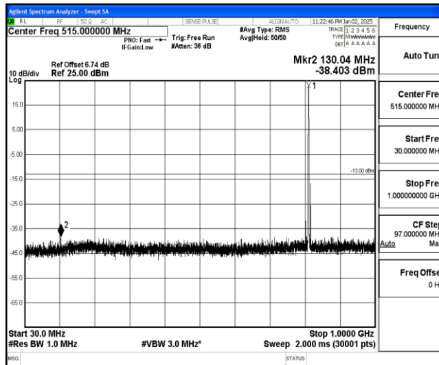
Band26-3MHz-16QAM-26705-1-0-Low-30-1000--38.4-PASS
