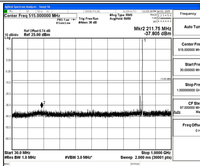
Band26-1.4MHz-16QAM-26783-1-0-High-30-1000--37.81-PASS
