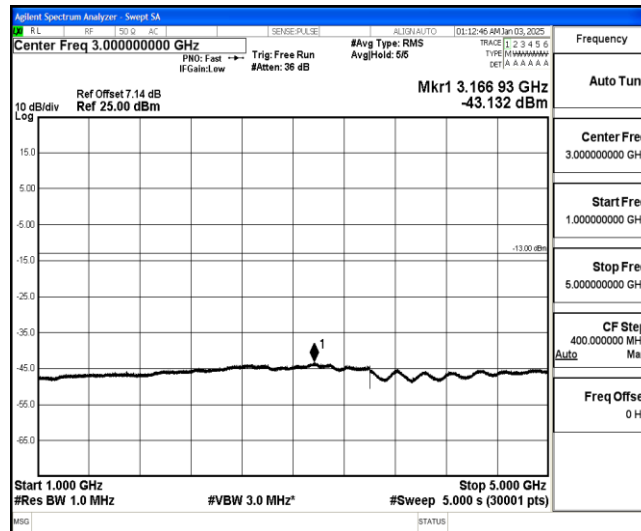
Band26-3MHz-16QAM-27025-1-0-High-1000-5000--43.13-PASS
