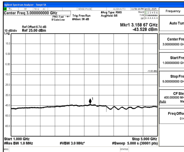
Band26-5MHz-QPSK-26765-1-0-High-1000-5000--43.53-PASS
