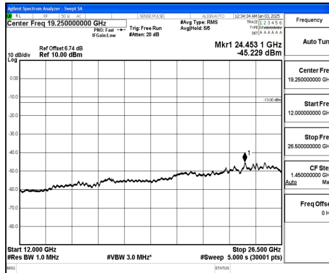
Band26-1.4MHz-16QAM-26797-1-0-Low-12000-26500--45.23-PASS
