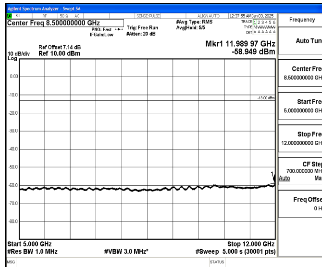
Band26-1.4MHz-16QAM-26915-1-0-Low-5000-12000--58.95-PASS
