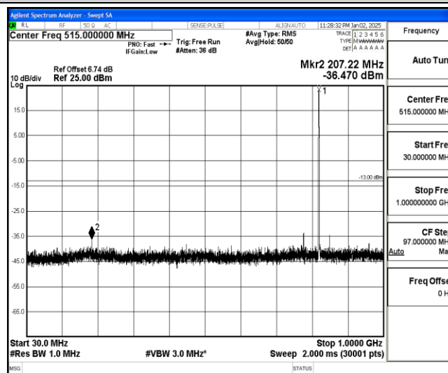
Band26-3MHz-QPSK-26775-1-0-High-30-1000--36.47-PASS
