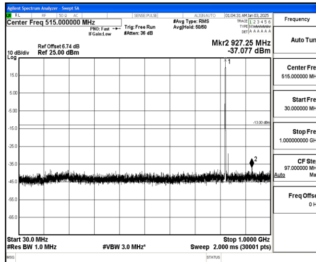
Band26-3MHz-16QAM-26805-1-0-Low-30-1000--37.08-PASS
