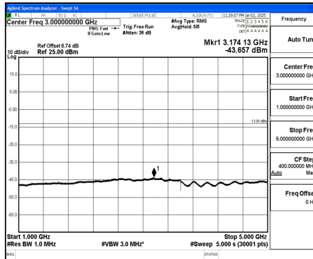
Band26-3MHz-QPSK-26775-1-0-High-1000-5000--43.66-PASS
