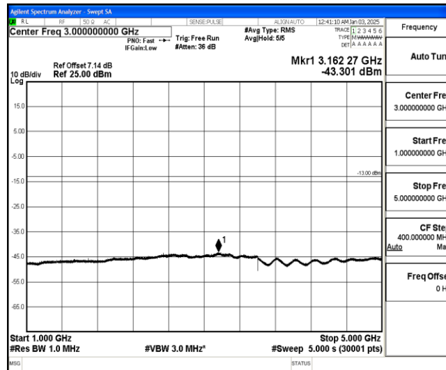
Band26-1.4MHz-16QAM-27033-1-0-High-1000-5000--43.3-PASS
