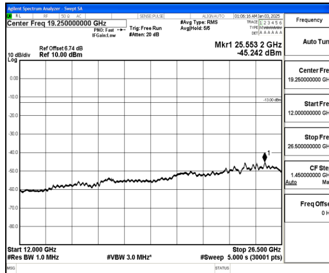
Band26-3MHz-16QAM-26805-1-0-Low-12000-26500--45.24-PASS
