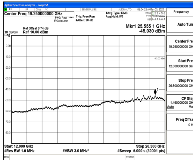
Band26-3MHz-QPSK-26805-1-0-Low-12000-26500--45.03-PASS
