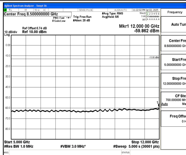
Band26-3MHz-QPSK-26705-1-0-Low-5000-12000--59.86-PASS
