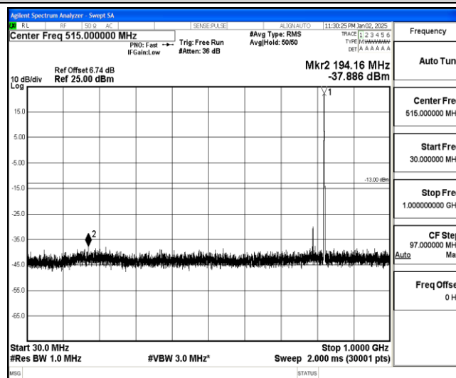
Band26-3MHz-16QAM-26775-1-0-High-30-1000--37.89-PASS
