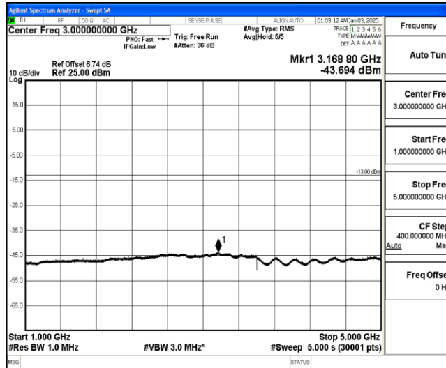
Band26-3MHz-QPSK-26805-1-0-Low-1000-5000--43.69-PASS
