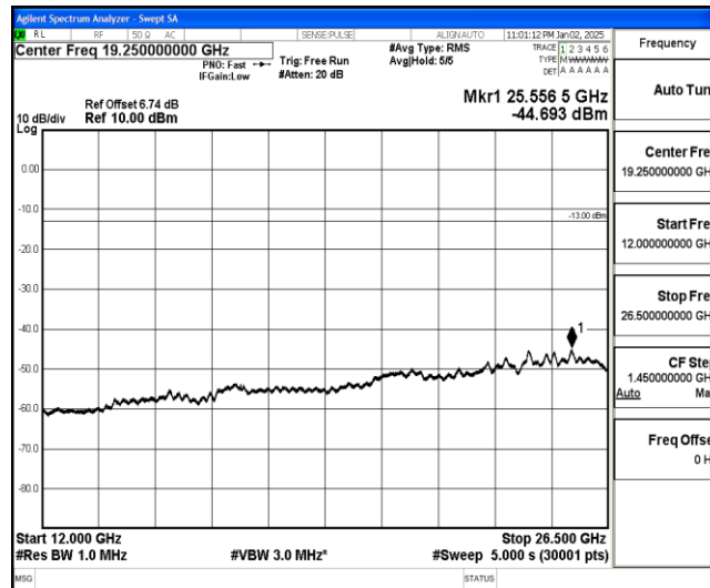
Band26-1.4MHz-16QAM-26740-1-0-Low-12000-26500--44.69-PASS
