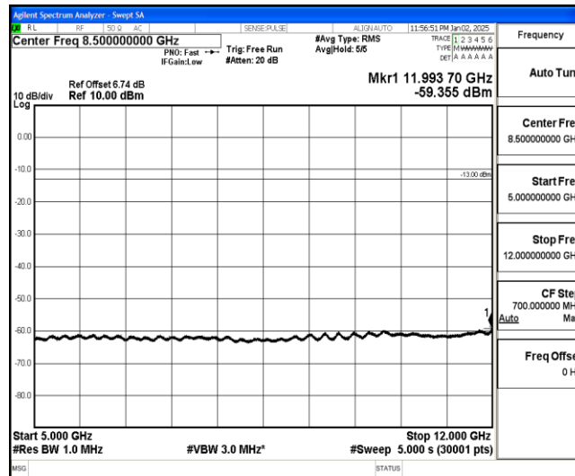
Band26-5MHz-QPSK-26765-1-0-High-5000-12000--59.36-PASS
