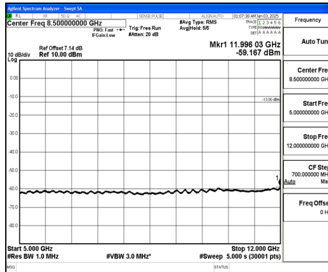
Band26-3MHz-QPSK-26915-1-0-Low-5000-12000--59.17-PASS
