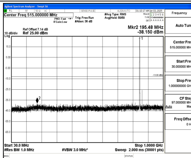
Band26-3MHz-QPSK-27025-1-0-High-30-1000--38.15-PASS
