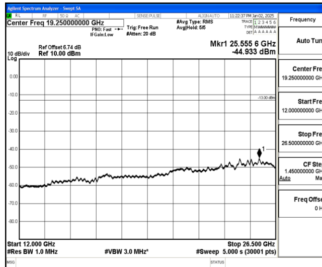
Band26-3MHz-QPSK-26705-1-0-Low-12000-26500--44.93-PASS
