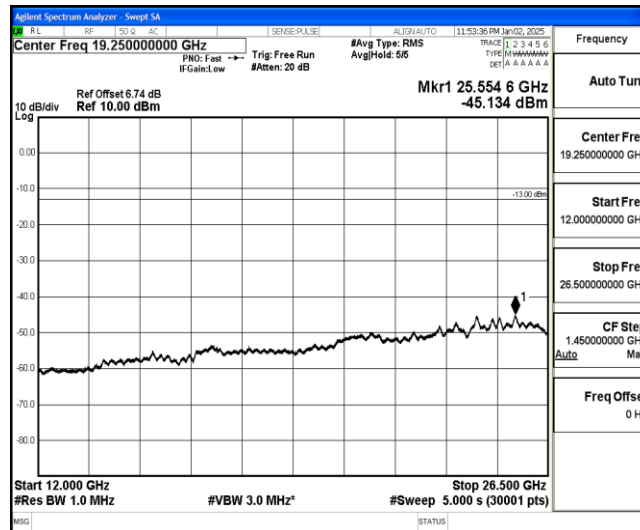
Band26-5MHz-QPSK-26740-1-0-Low-12000-26500--45.13-PASS
