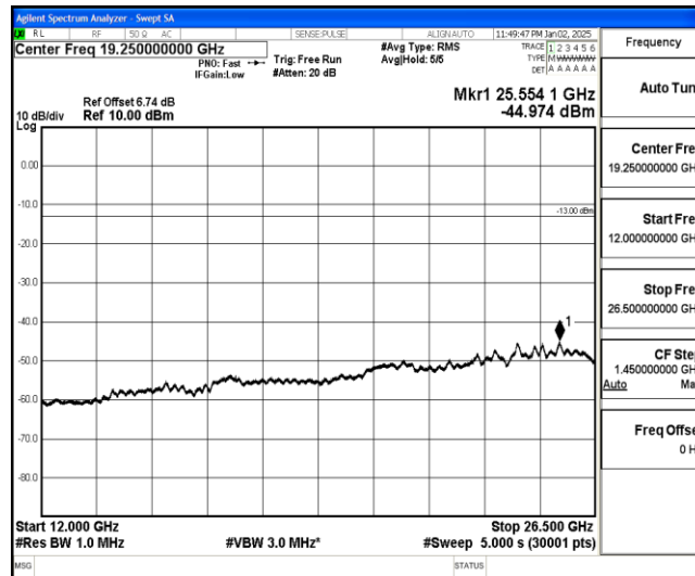
Band26-5MHz-QPSK-26715-1-0-Low-12000-26500--44.97-PASS
