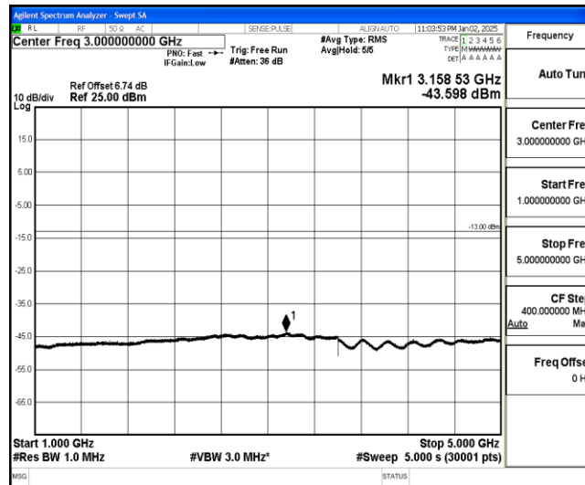
Band26-1.4MHz-16QAM-26783-1-0-High-1000-5000--43.6-PASS
