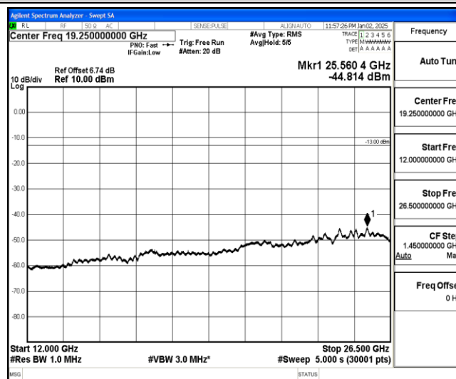
Band26-5MHz-QPSK-26765-1-0-High-12000-26500--44.81-PASS
