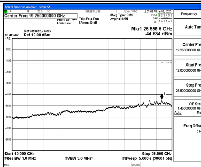
Band26-1.4MHz-16QAM-26783-1-0-High-12000-26500--44.53-PASS
