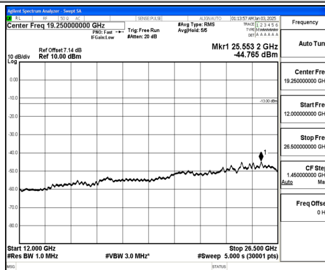
Band26-3MHz-16QAM-27025-1-0-High-12000-26500--44.77-PASS
