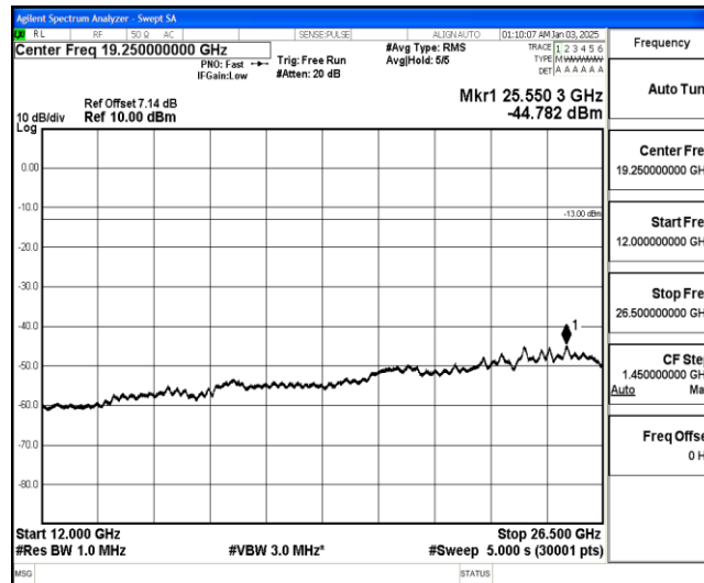
Band26-3MHz-16QAM-26915-1-0-Low-12000-26500--44.78-PASS
