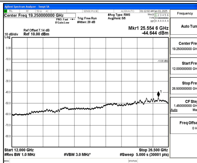
Band26-3MHz-QPSK-27025-1-0-High-12000-26500--44.64-PASS
