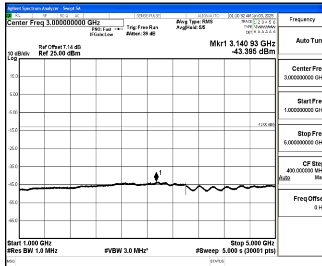
Band26-3MHz-QPSK-27025-1-0-High-1000-5000--43.4-PASS
