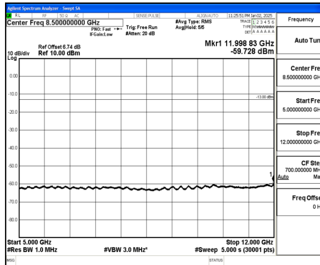
Band26-3MHz-QPSK-26740-1-0-Low-5000-12000--59.73-PASS
