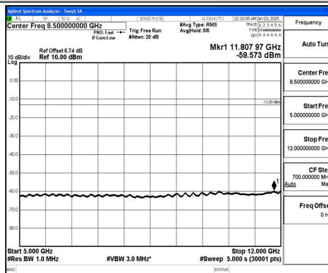
Band26-1.4MHz-QPSK-26797-1-0-Low-5000-12000--59.57-PASS
