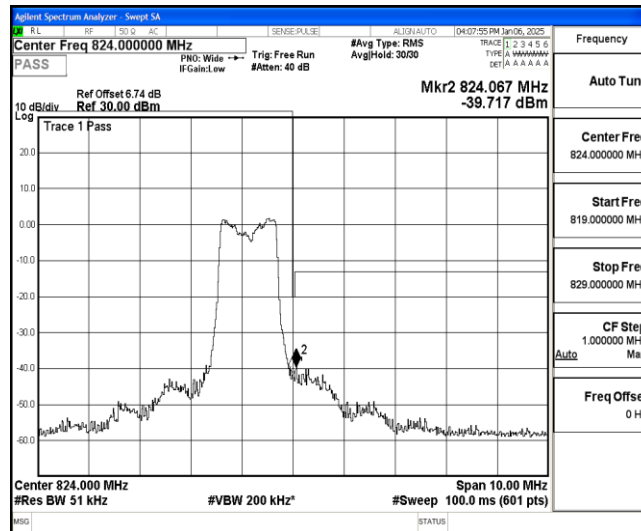
Band26-3MHz-16QAM-26775-6-0-High--41.68,-39.72-PASS
