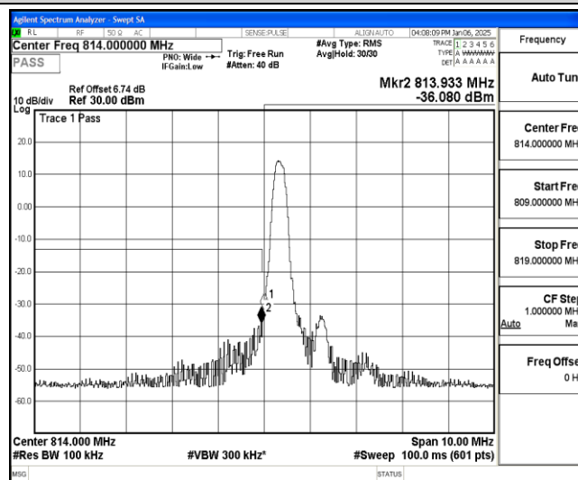
Band26-5MHz-QPSK-26715-1-0-Low--31.98,-36.08-PASS
