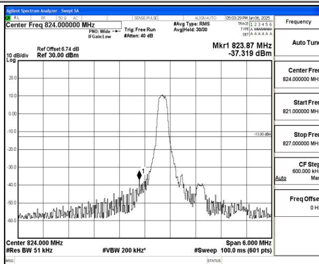
Band26-3MHz-QPSK-26805-1-0-Low--37.32-PASS
