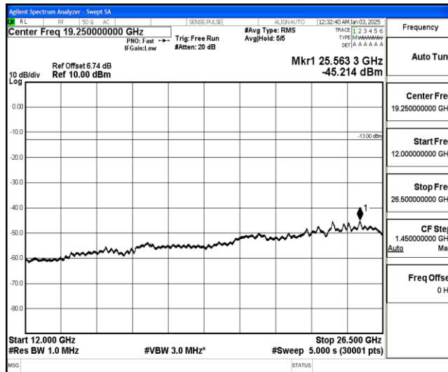
Band26-1.4MHz-QPSK-26797-1-0-Low-12000-26500--45.21-PASS
