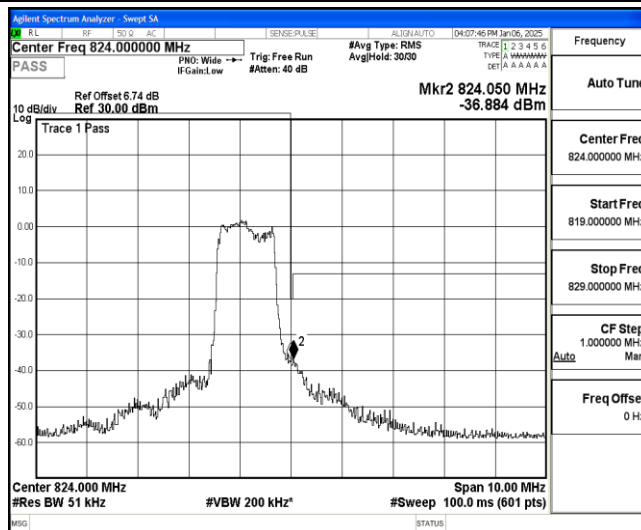
Band26-3MHz-QPSK-26775-6-0-High--37.26,-36.88-PASS
