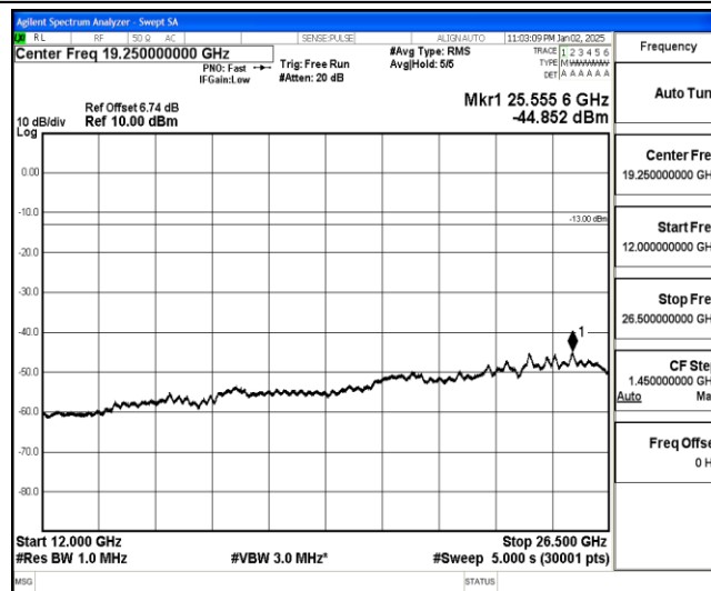
Band26-1.4MHz-QPSK-26783-1-0-High-12000-26500--44.85-PASS
