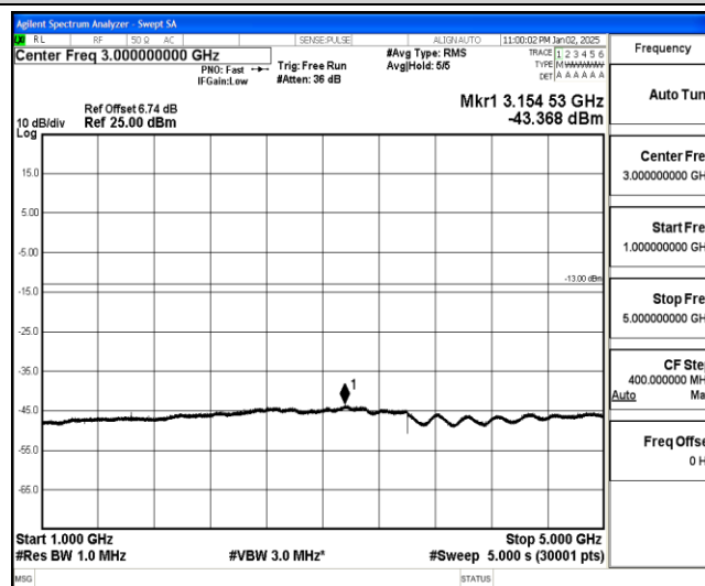
Band26-1.4MHz-16QAM-26740-1-0-Low-1000-5000--43.37-PASS
