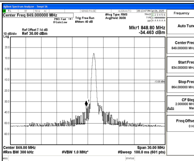
Band26-15MHz-QPSK-26865-1-0-Low--34.46-PASS
