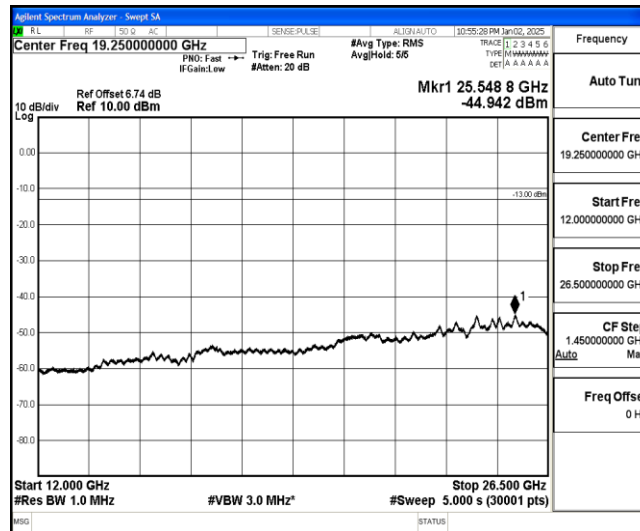
Band26-1.4MHz-QPSK-26697-1-0-Low-12000-26500--44.94-PASS
