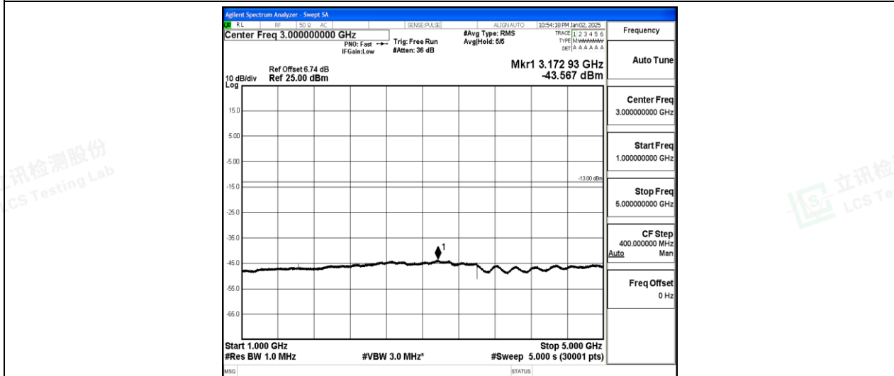
Band26-1.4MHz-QPSK-26697-1-0-Low-1000-5000--43.57-PASS
