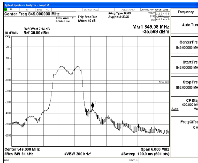
Band26-3MHz-16QAM-27025-6-0-High--35.57-PASS
