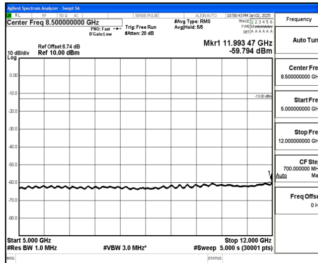
Band26-1.4MHz-QPSK-26740-1-0-Low-5000-12000--59.79-PASS
