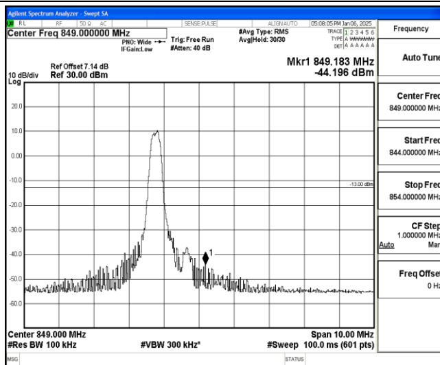
Band26-5MHz-QPSK-27015-1-0-High--44.20-PASS
