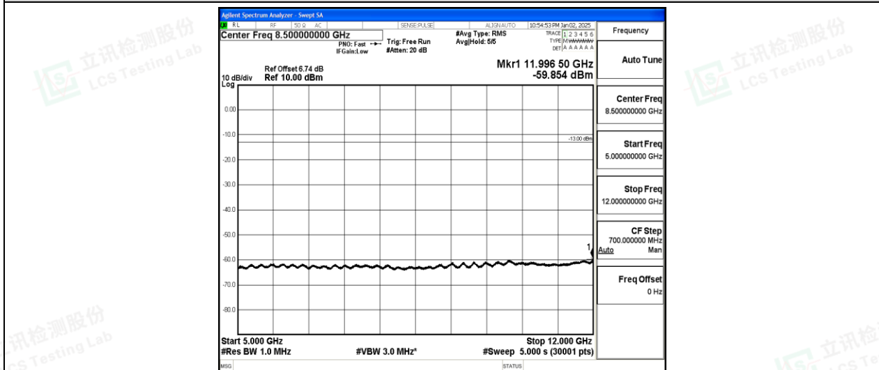
Band26-1.4MHz-QPSK-26697-1-0-Low-5000-12000--59.85-PASS
