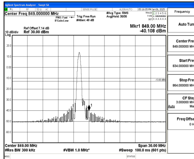
Band26-15MHz-QPSK-26965-1-0-High--40.11-PASS
