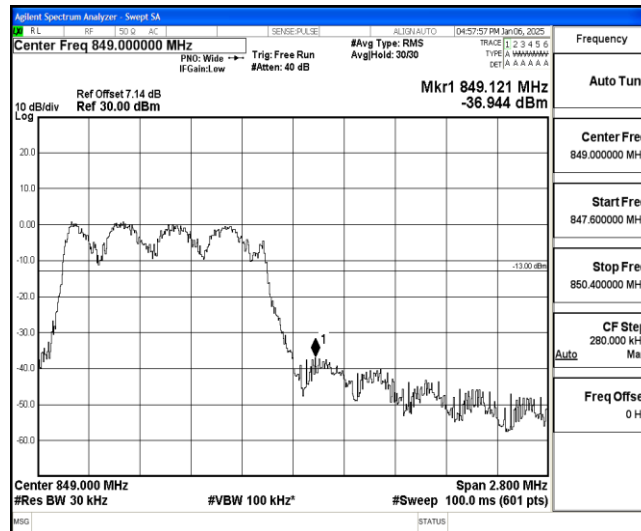
Band26-1.4MHz-16QAM-27033-6-0-High--36.94-PASS
