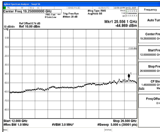
Band26-1.4MHz-QPSK-26740-1-0-Low-12000-26500--44.87-PASS
