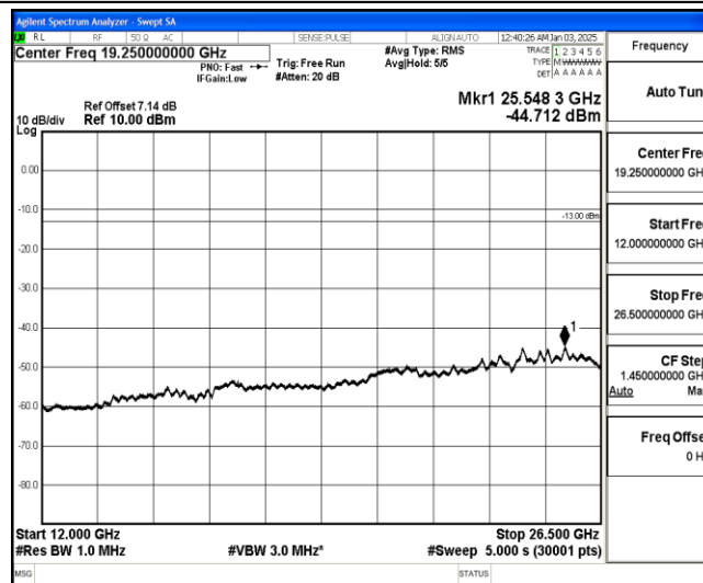
Band26-1.4MHz-QPSK-27033-1-0-High-12000-26500--44.71-PASS
