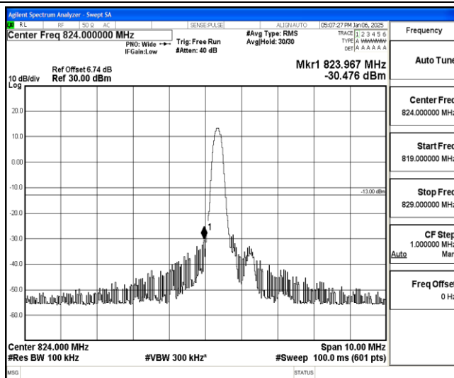
Band26-5MHz-QPSK-26815-1-0-Low--30.48-PASS
