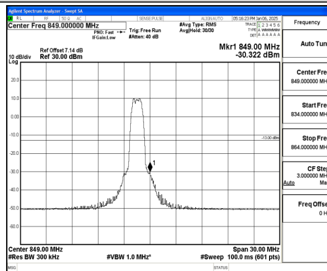
Band26-15MHz-QPSK-26965-6-0-High--30.32-PASS
