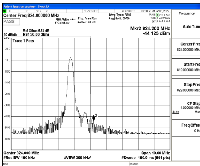
Band26-5MHz-16QAM-26765-1-0-High--46.81,-44.12-PASS
