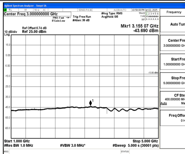
Band26-1.4MHz-QPSK-26740-1-0-Low-1000-5000--43.69-PASS
