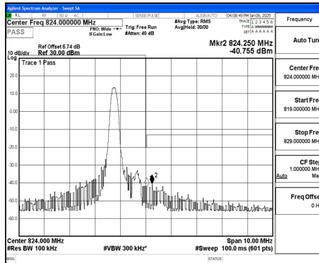
Band26-5MHz-QPSK-26765-1-0-High--42.36,-40.76-PASS
