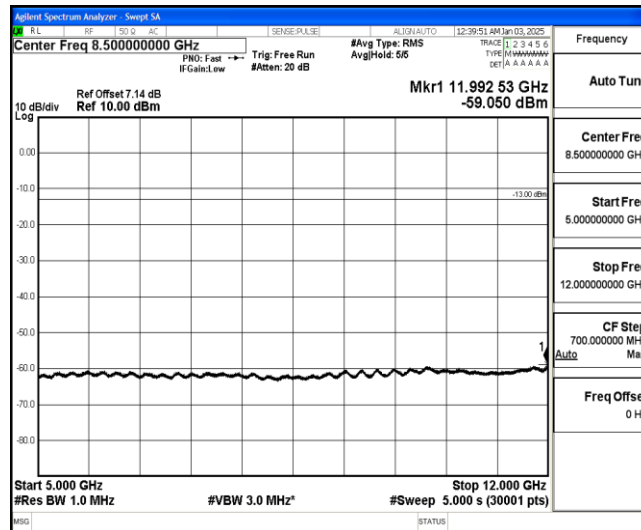
Band26-1.4MHz-QPSK-27033-1-0-High-5000-12000--59.05-PASS
