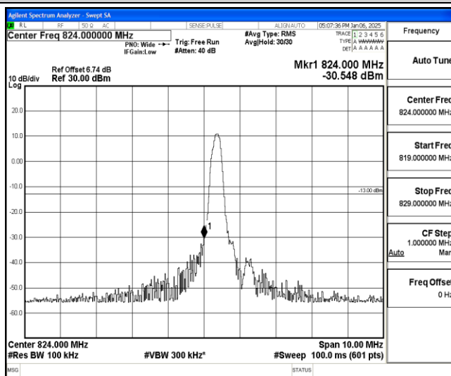
Band26-5MHz-16QAM-26815-1-0-Low--30.55-PASS
