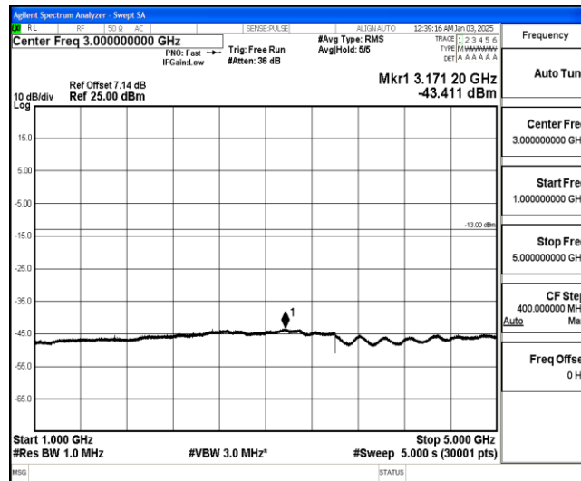
Band26-1.4MHz-QPSK-27033-1-0-High-1000-5000--43.41-PASS
