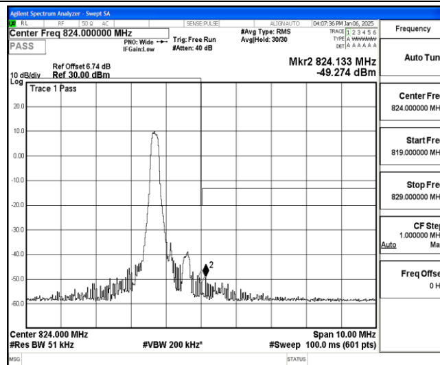
Band26-3MHz-16QAM-26775-1-0-High--51.41,-49.27-PASS
