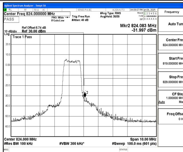
Band26-5MHz-QPSK-26765-6-0-High--31.02,-32.00-PASS
