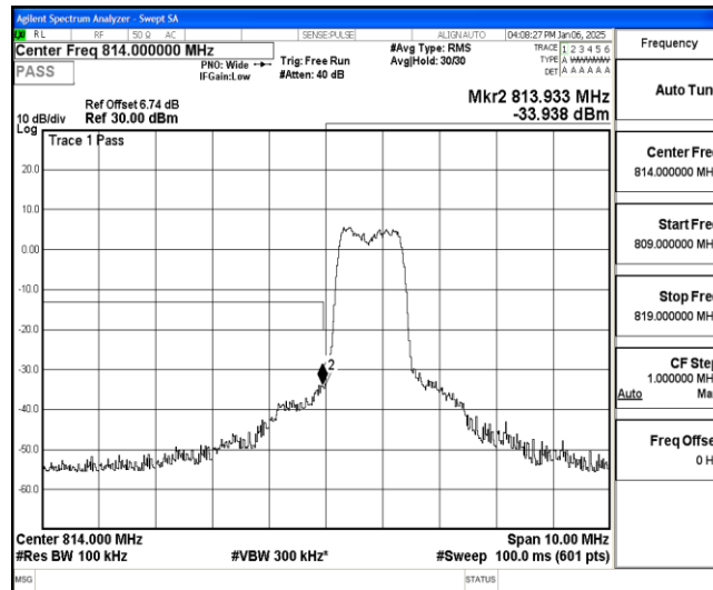
Band26-5MHz-QPSK-26715-6-0-Low--33.43,-33.94-PASS
