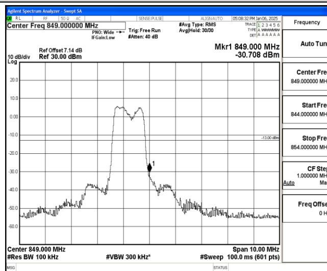
Band26-5MHz-16QAM-27015-6-0-High--30.71-PASS
