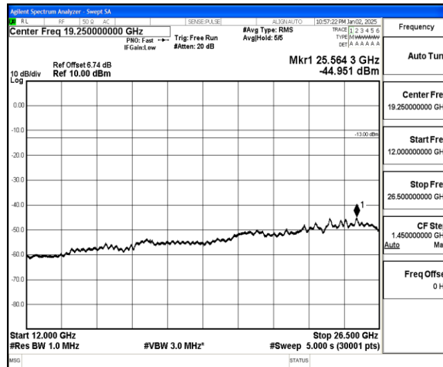
Band26-1.4MHz-16QAM-26697-1-0-Low-12000-26500--44.95-PASS
