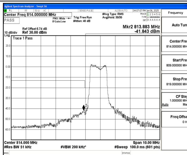
Band26-3MHz-QPSK-26705-6-0-Low--43.22,-41.84-PASS
