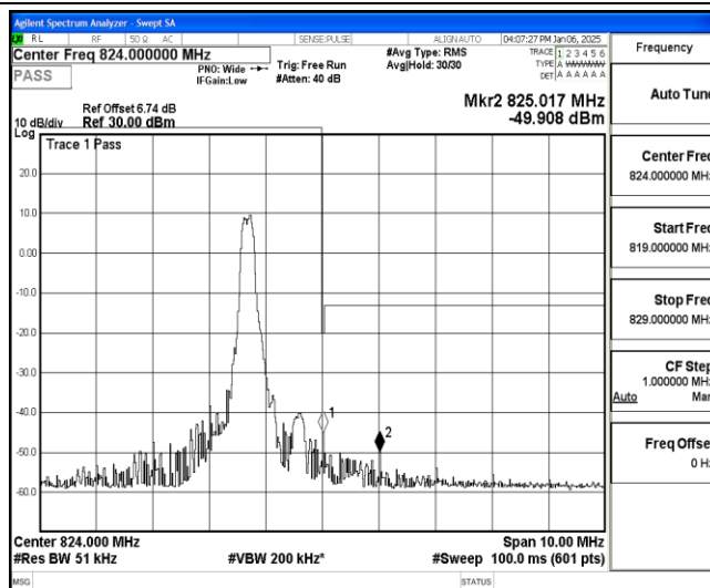
Band26-3MHz-QPSK-26775-1-0-High--44.98,-49.91-PASS
