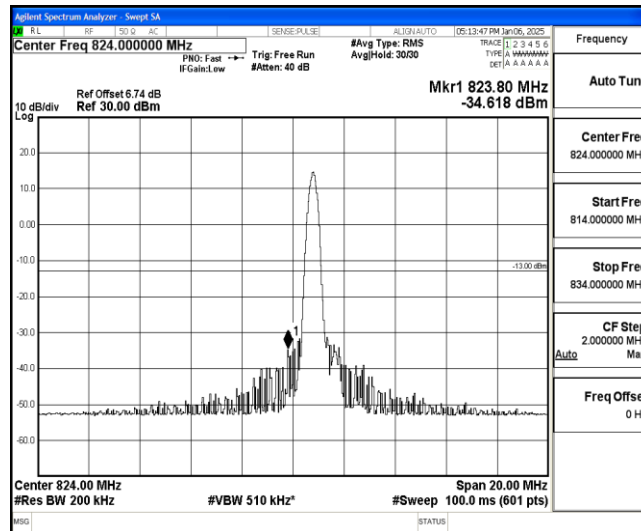
Band26-10MHz-QPSK-26840-1-0-Low--34.62-PASS
