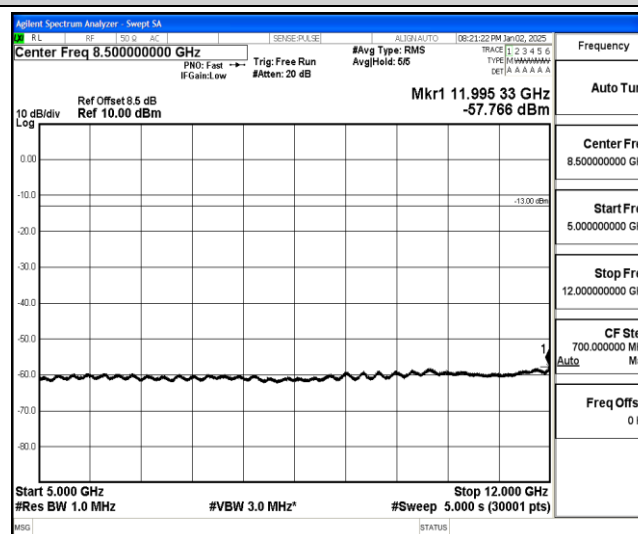
Band25-5MHz-16QAM-26365-1-0-Low-5000-12000--57.77-PASS
