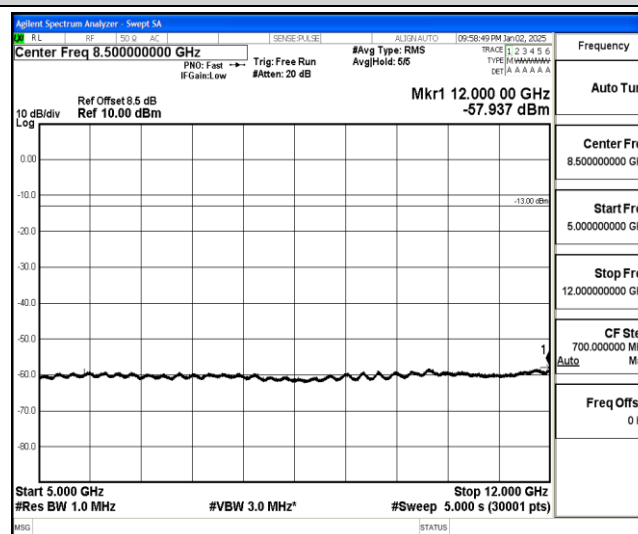
Band25-20MHz-16QAM-26365-1-0-Low-5000-12000--57.94-PASS
