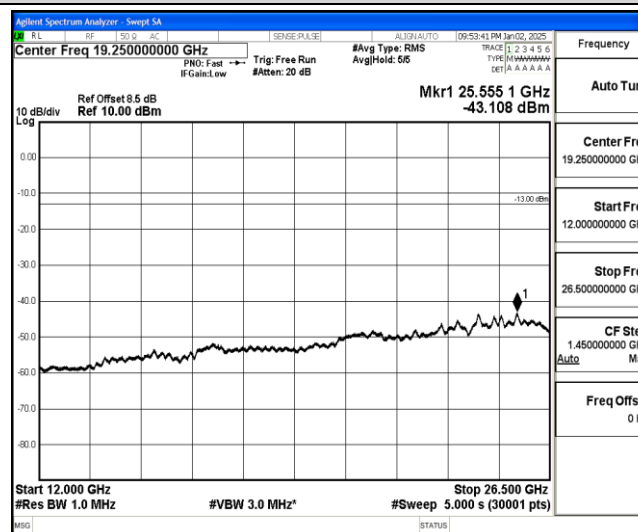
Band25-20MHz-QPSK-26140-1-0-Low-12000-26500--43.11-PASS
