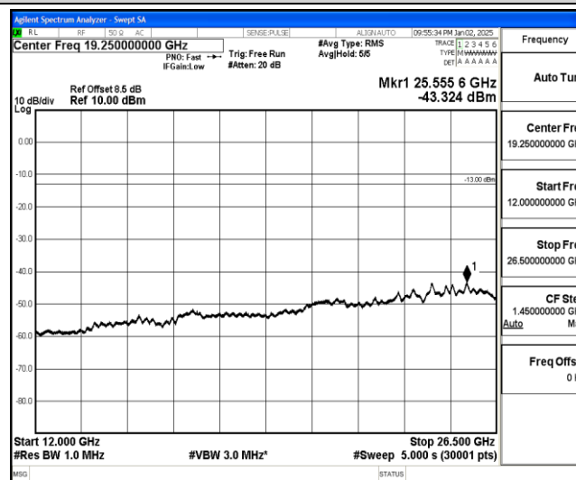
Band25-20MHz-16QAM-26140-1-0-Low-12000-26500--43.32-PASS
