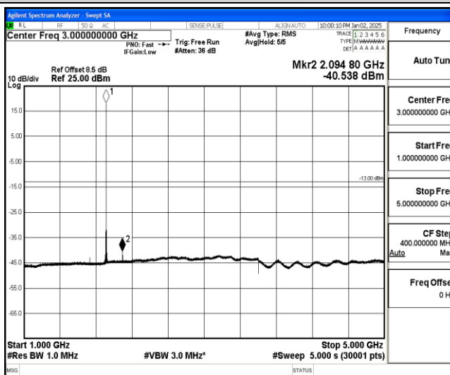
Band25-20MHz-QPSK-26590-1-0-High-1000-5000--40.54-PASS
