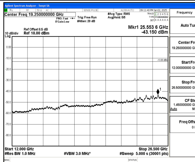
Band25-10MHz-16QAM-26640-1-0-High-12000-26500--43.15-PASS
