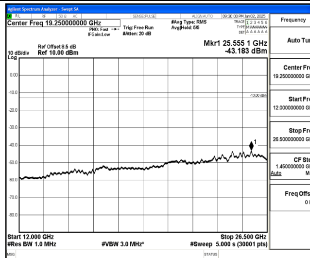
Band25-15MHz-QPSK-26365-1-0-Low-12000-26500--43.18-PASS
