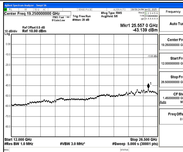
Band25-20MHz-16QAM-26365-1-0-Low-12000-26500--43.14-PASS
