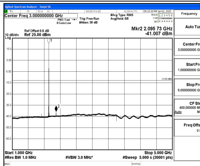
Band25-10MHz-16QAM-26640-1-0-High-1000-5000--41.01-PASS
