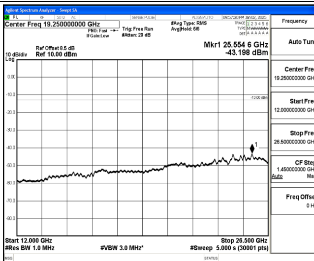
Band25-20MHz-QPSK-26365-1-0-Low-12000-26500--43.2-PASS
