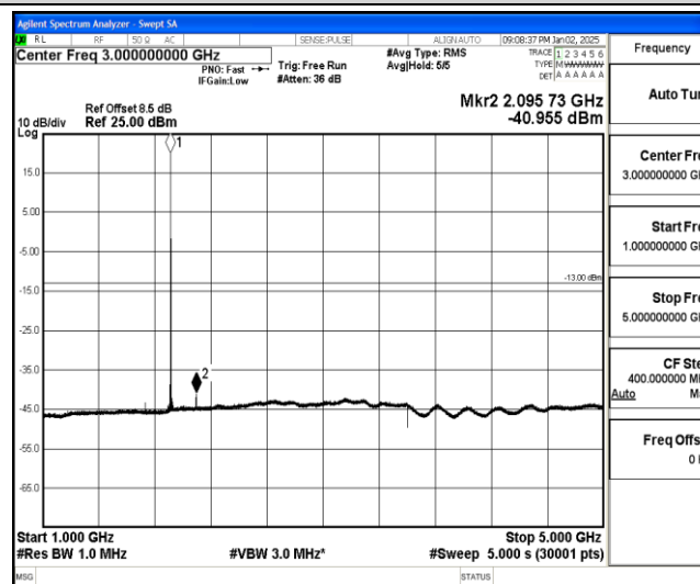
Band25-10MHz-QPSK-26640-1-0-High-1000-5000--40.96-PASS
