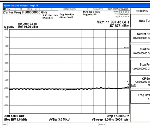
Band25-15MHz-QPSK-26365-1-0-Low-5000-12000--57.88-PASS
