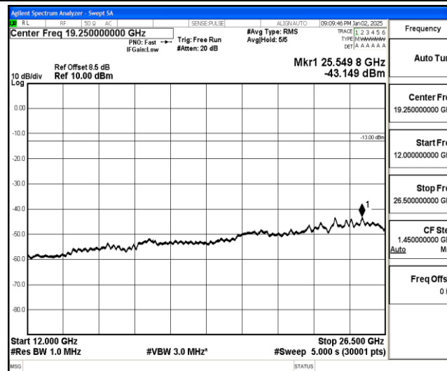
Band25-10MHz-QPSK-26640-1-0-High-12000-26500--43.15-PASS
