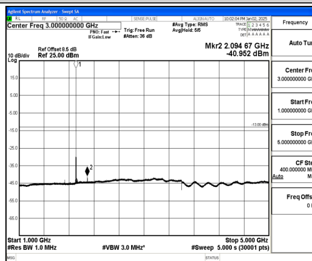
Band25-20MHz-16QAM-26590-1-0-High-1000-5000--40.95-PASS
