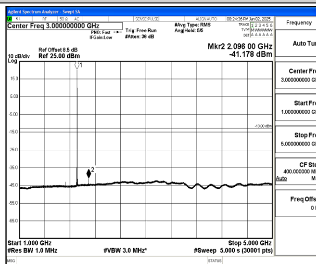
Band25-5MHz-16QAM-26665-1-0-High-1000-5000--41.18-PASS
