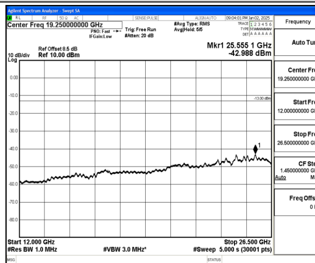
Band25-10MHz-16QAM-26090-1-0-Low-12000-26500--42.99-PASS
