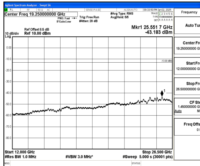
Band25-15MHz-QPSK-26615-1-0-High-12000-26500--43.18-PASS
