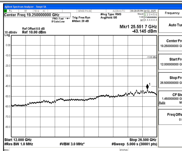
Band25-15MHz-16QAM-26115-1-0-Low-12000-26500--43.15-PASS
