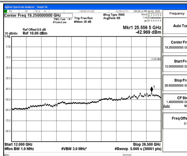
Band25-15MHz-QPSK-26115-1-0-Low-12000-26500--42.97-PASS
