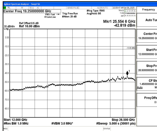
Band25-10MHz-16QAM-26365-1-0-Low-12000-26500--42.82-PASS
