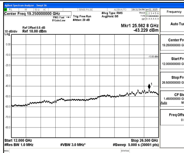
Band25-15MHz-16QAM-26365-1-0-Low-12000-26500--43.23-PASS
