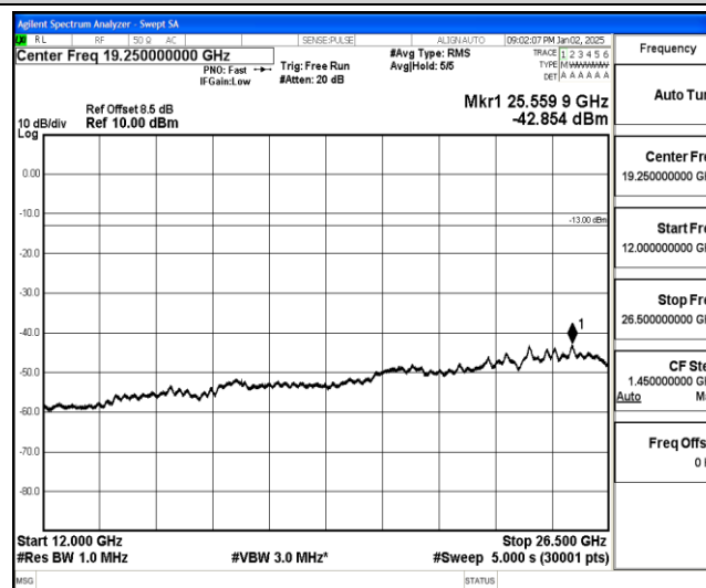
Band25-10MHz-QPSK-26090-1-0-Low-12000-26500--42.85-PASS
