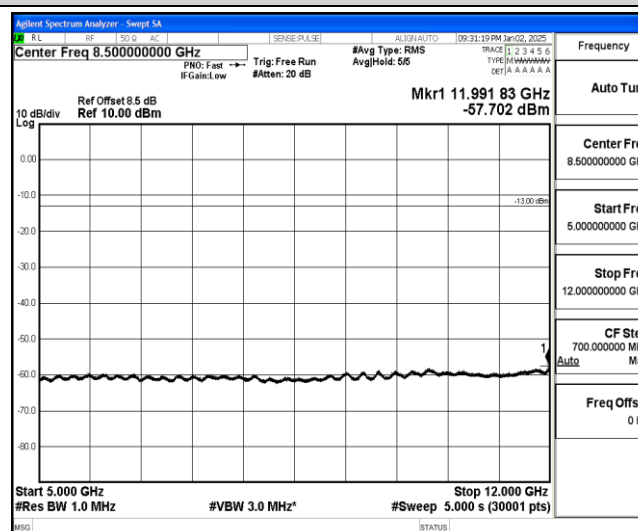
Band25-15MHz-16QAM-26365-1-0-Low-5000-12000--57.7-PASS
