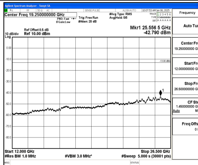
Band25-10MHz-QPSK-26365-1-0-Low-12000-26500--42.79-PASS
