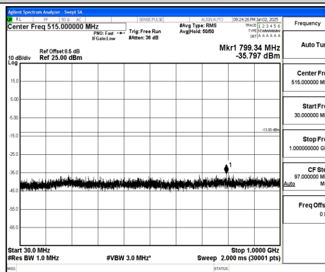
Band25-15MHz-QPSK-26115-1-0-Low-30-1000--35.8-PASS
