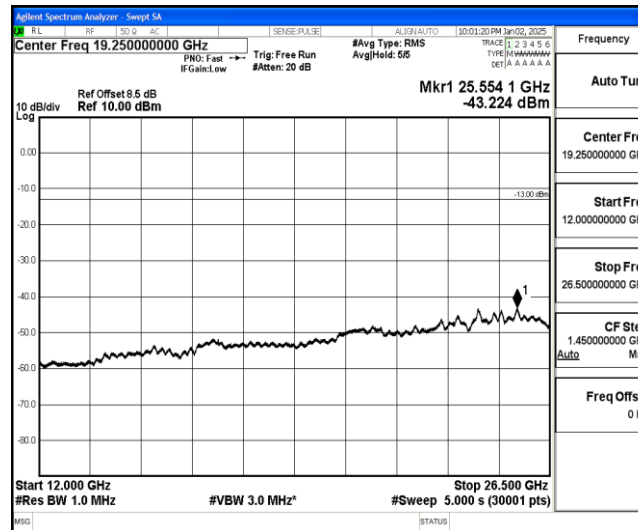
Band25-20MHz-QPSK-26590-1-0-High-12000-26500--43.22-PASS
