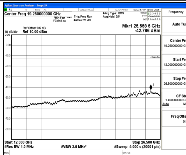
Band25-5MHz-16QAM-26365-1-0-Low-12000-26500--42.79-PASS
