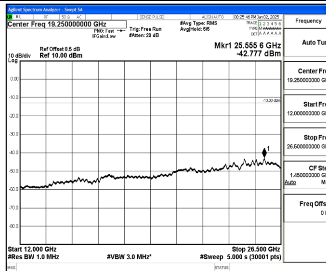
Band25-5MHz-16QAM-26665-1-0-High-12000-26500--42.78-PASS
