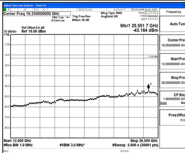
Band25-15MHz-16QAM-26615-1-0-High-12000-26500--43.16-PASS
