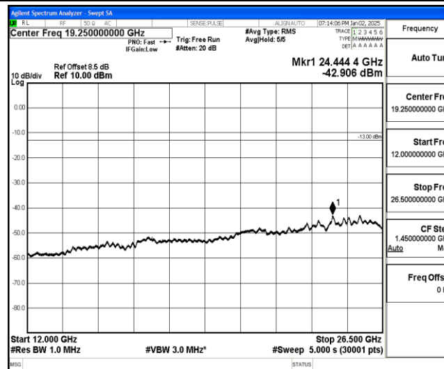
Band25-1.4MHz-16QAM-26683-1-0-High-12000-26500--42.91-PASS
