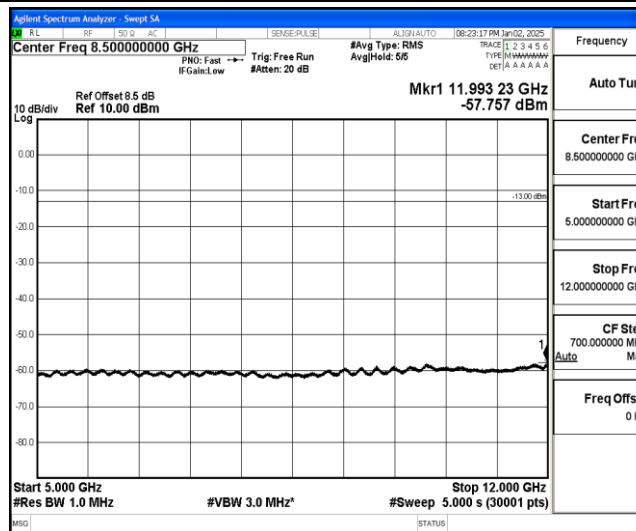
Band25-5MHz-QPSK-26665-1-0-High-5000-12000--57.76-PASS
