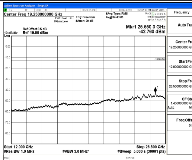
Band25-3MHz-QPSK-26365-1-0-Low-12000-26500--42.76-PASS
