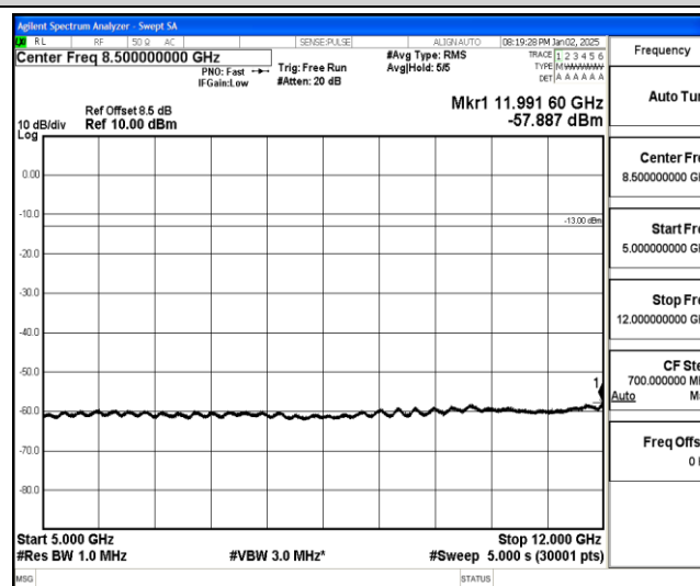
Band25-5MHz-QPSK-26365-1-0-Low-5000-12000--57.89-PASS
