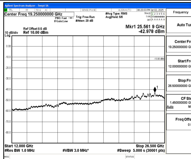
Band25-5MHz-QPSK-26365-1-0-Low-12000-26500--42.98-PASS
