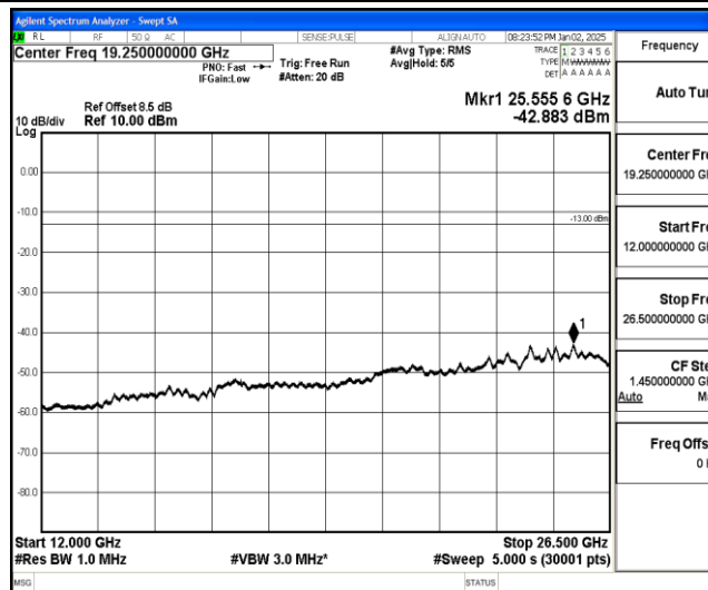
Band25-5MHz-QPSK-26665-1-0-High-12000-26500--42.88-PASS
