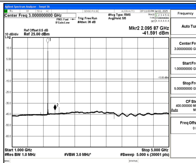
Band25-1.4MHz-QPSK-26683-1-0-High-1000-5000--41.59-PASS
