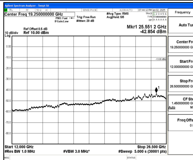
Band25-3MHz-16QAM-26365-1-0-Low-12000-26500--42.85-PASS
