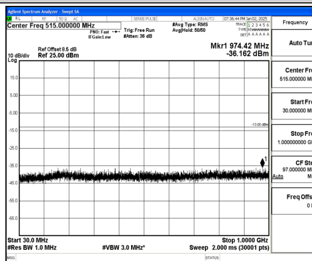
Band25-3MHz-QPSK-26055-1-0-Low-30-1000--36.16-PASS
