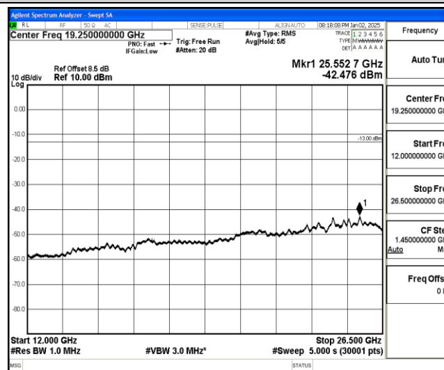
Band25-5MHz-16QAM-26065-1-0-Low-12000-26500--42.48-PASS
