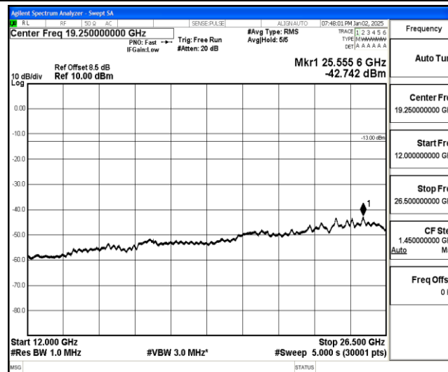
Band25-3MHz-16QAM-26675-1-0-High-12000-26500--42.74-PASS
