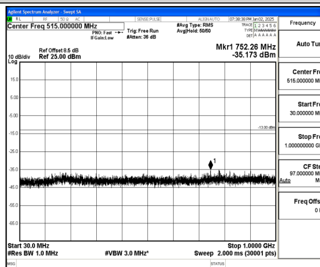
Band25-3MHz-16QAM-26055-1-0-Low-30-1000--35.17-PASS
