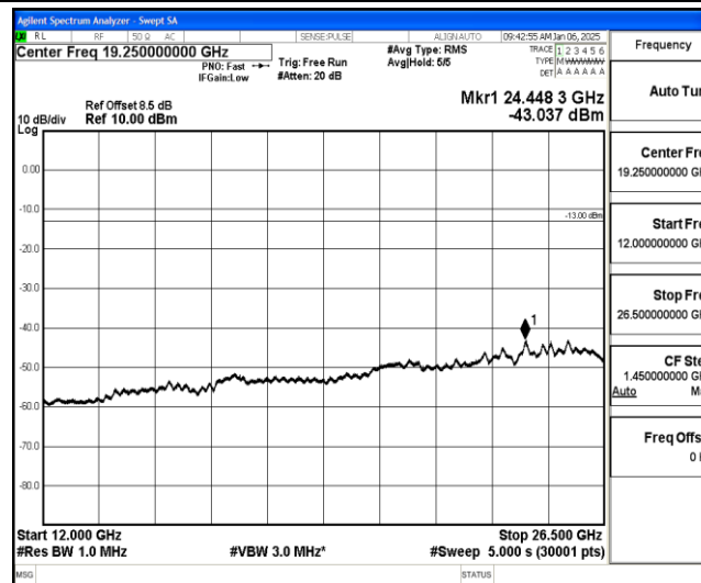
Band25-1.4MHz-16QAM-26365-1-0-Low-12000-26500--43.04-PASS
