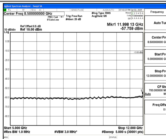
Band25-3MHz-16QAM-26365-1-0-Low-5000-12000--57.76-PASS
