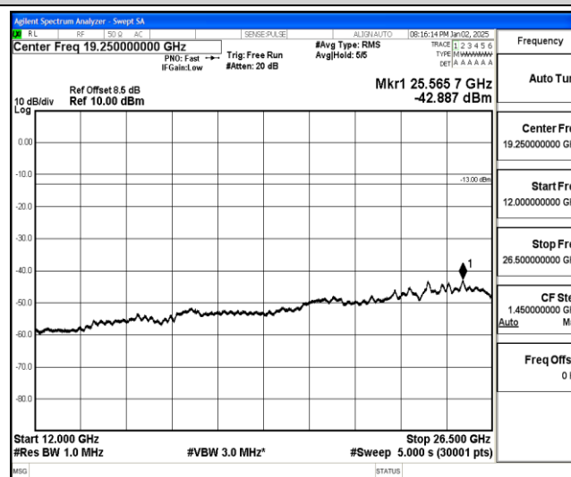
Band25-5MHz-QPSK-26065-1-0-Low-12000-26500--42.89-PASS
