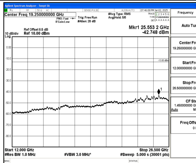
Band25-3MHz-QPSK-26675-1-0-High-12000-26500--42.75-PASS
