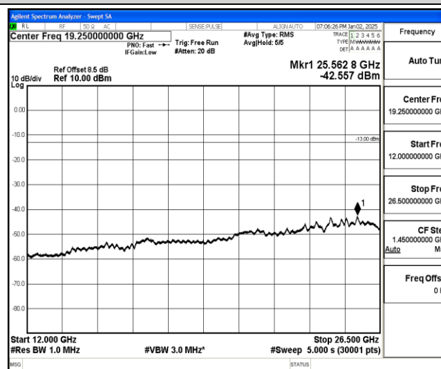
Band25-1.4MHz-16QAM-26047-1-0-Low-12000-26500--42.56-PASS
