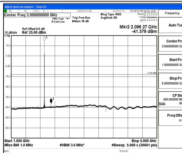
Band25-3MHz-16QAM-26675-1-0-High-1000-5000--41.38-PASS
