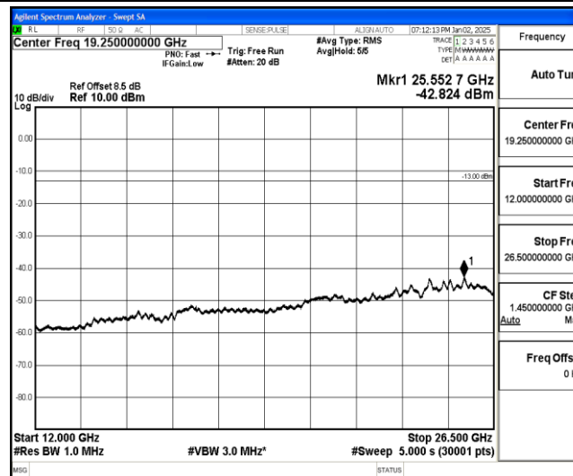
Band25-1.4MHz-QPSK-26683-1-0-High-12000-26500--42.82-PASS
