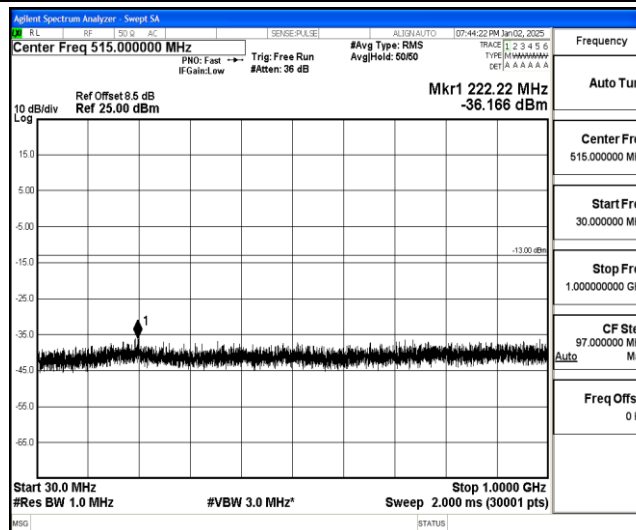
Band25-3MHz-QPSK-26675-1-0-High-30-1000--36.17-PASS
