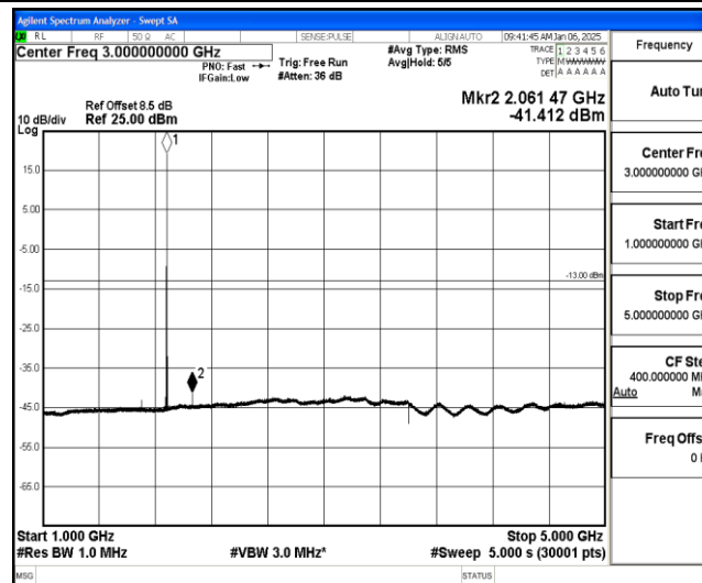
Band25-1.4MHz-16QAM-26365-1-0-Low-1000-5000--41.41-PASS
