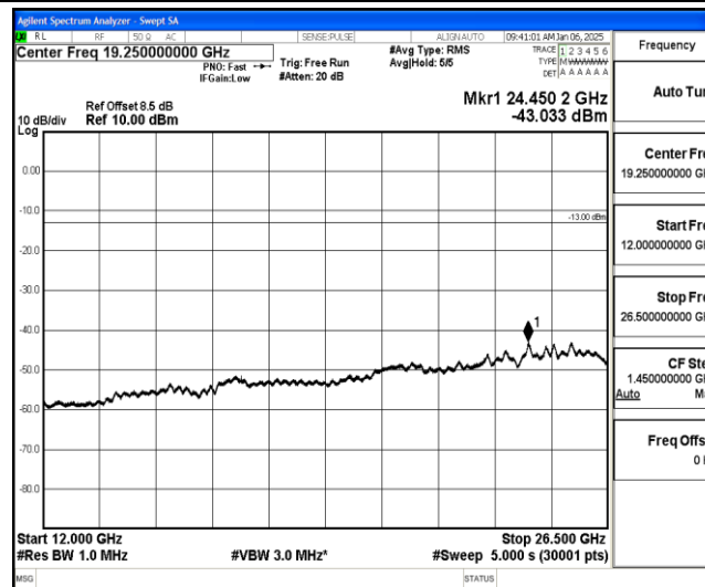
Band25-1.4MHz-QPSK-26365-1-0-Low-12000-26500--43.03-PASS
