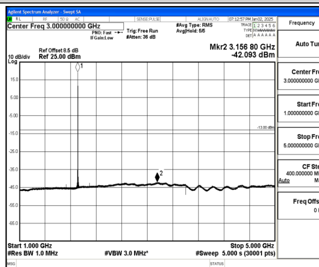
Band25-1.4MHz-16QAM-26683-1-0-High-1000-5000--42.09-PASS
