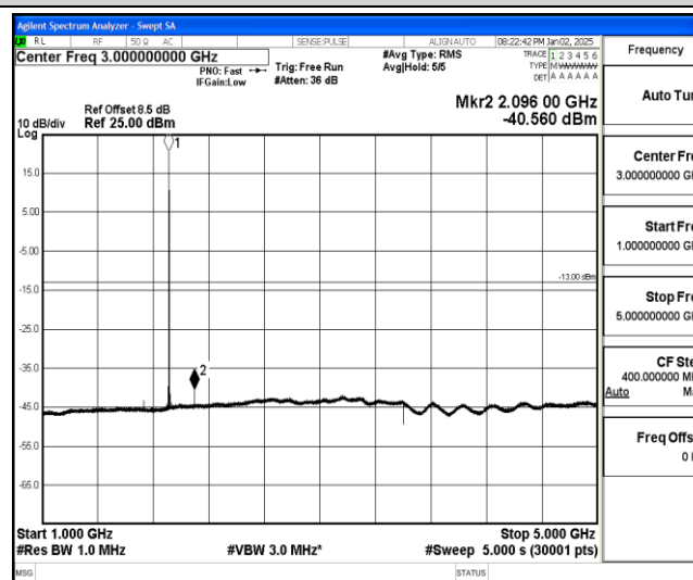
Band25-5MHz-QPSK-26665-1-0-High-1000-5000--40.56-PASS
