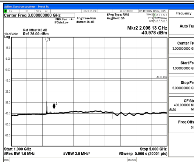
Band25-3MHz-QPSK-26675-1-0-High-1000-5000--40.98-PASS
