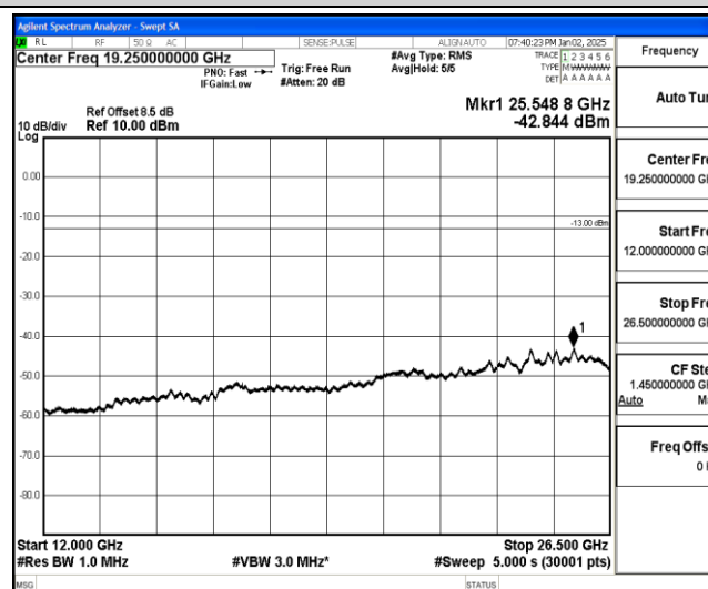
Band25-3MHz-16QAM-26055-1-0-Low-12000-26500--42.84-PASS
