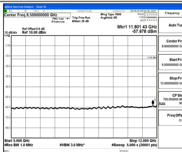
Band25-1.4MHz-QPSK-26365-1-0-Low-5000-12000--57.98-PASS
