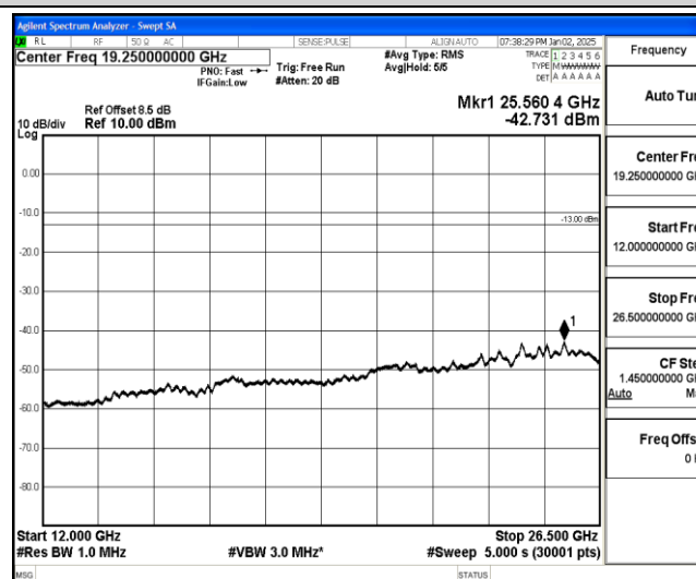
Band25-3MHz-QPSK-26055-1-0-Low-12000-26500--42.73-PASS
