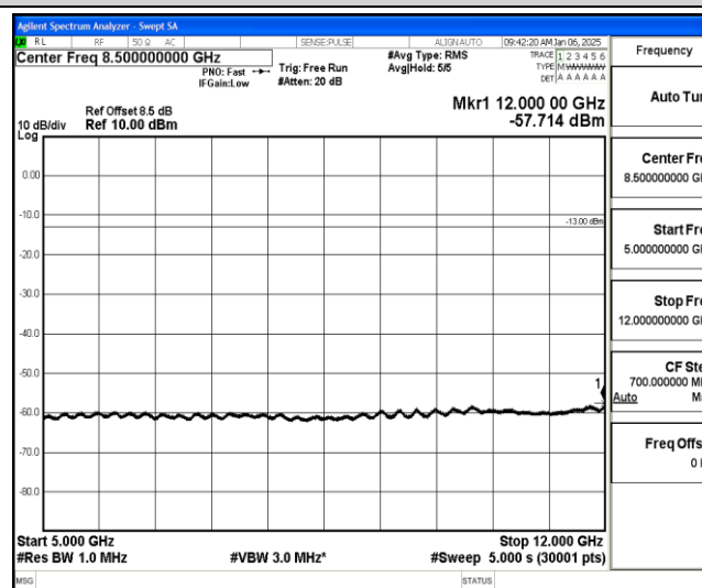
Band25-1.4MHz-16QAM-26365-1-0-Low-5000-12000--57.71-PASS
