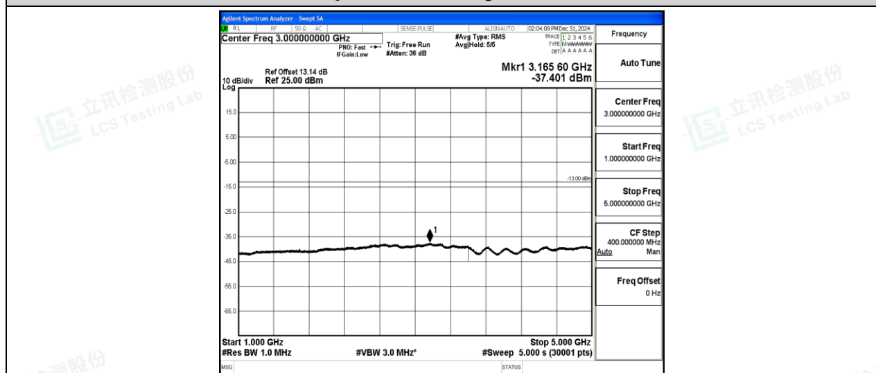
Band5-3MHz-16QAM-20635-1-0-High-1000-5000--37.4-PASS
