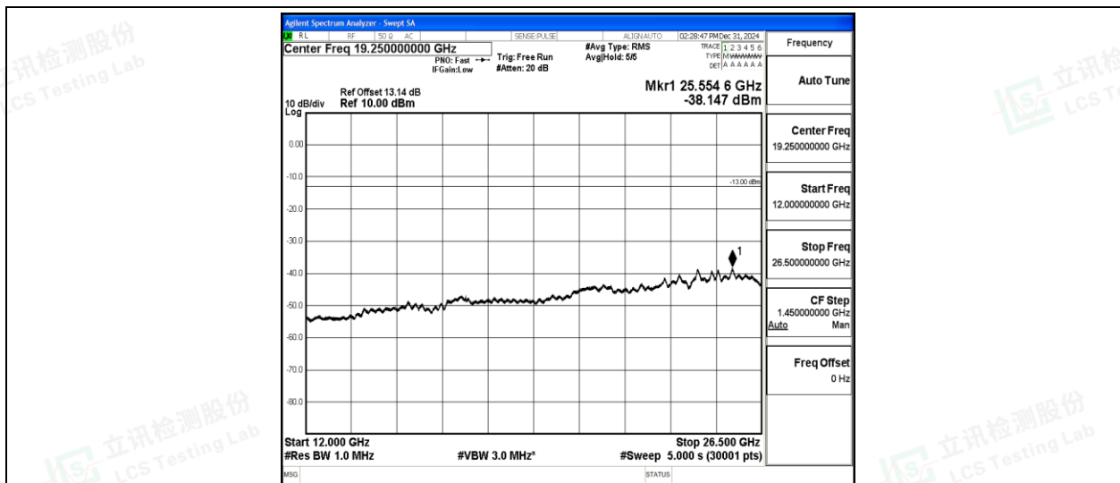
Band5-5MHz-QPSK-20525-1-0-Low-12000-26500--38.15-PASS
