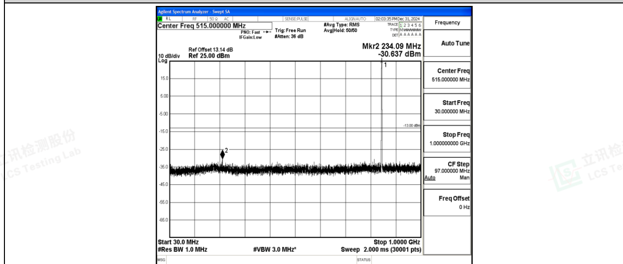
Band5-3MHz-16QAM-20635-1-0-High-30-1000--30.64-PASS
