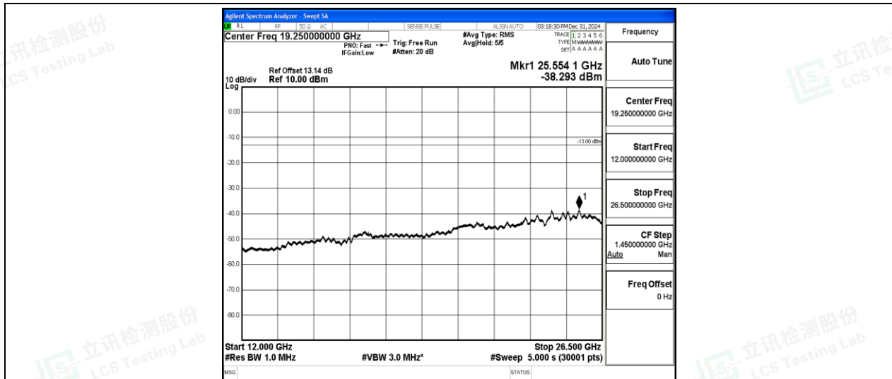
Band5-10MHz-QPSK-20525-1-0-Low-12000-26500--38.29-PASS
