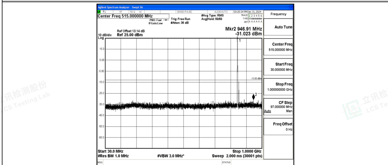
Band5-10MHz-QPSK-20600-1-0-High-30-1000--31.02-PASS
