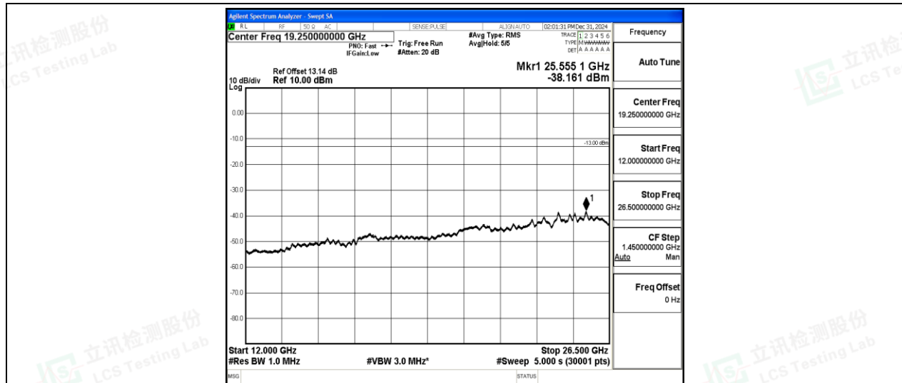
Band5-3MHz-16QAM-20525-1-0-Low-12000-26500--38.16-PASS
