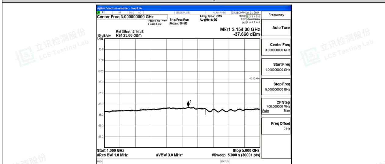
Band5-10MHz-QPSK-20600-1-0-High-1000-5000--37.67-PASS
