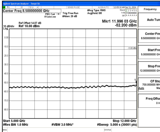
Band4-20MHz-16QAM-20050-1-0-Low-5000-12000--52.2-PASS
