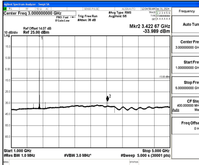
Band4-20MHz-16QAM-20050-1-0-Low-1000-5000--33.99-PASS
