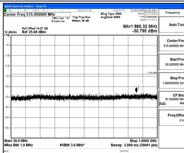
Band4-3MHz-16QAM-19965-1-0-Low-30-1000--30.8-PASS
