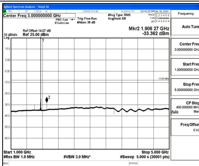
Band4-3MHz-QPSK-20385-1-0-High-1000-5000--33.36-PASS
