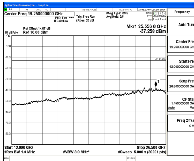
Band4-3MHz-QPSK-20385-1-0-High-12000-26500--37.26-PASS
