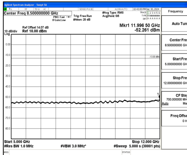
Band4-3MHz-QPSK-20385-1-0-High-5000-12000--52.26-PASS
