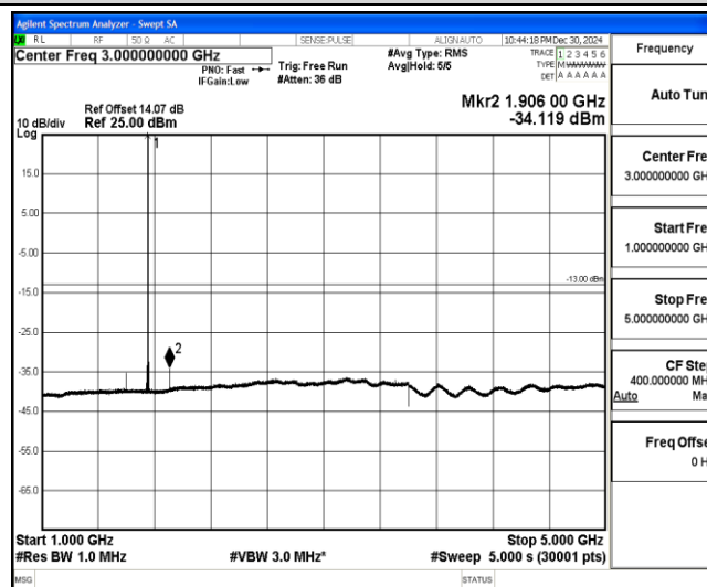
Band4-3MHz-16QAM-20385-1-0-High-1000-5000--34.12-PASS
