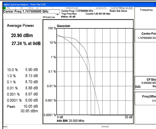
Band4-15MHz-16QAM-20325-6-0-High-8.70-&lt;=13-PASS
