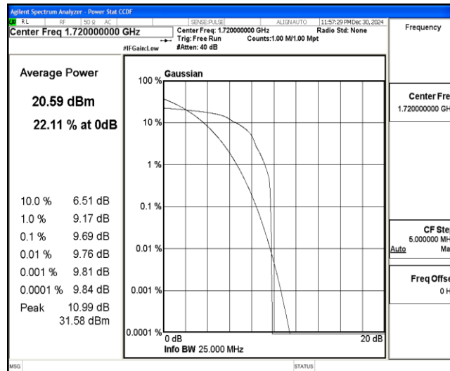
Band4-20MHz-16QAM-20050-1-0-Low-9.69-&lt;=13-PASS
