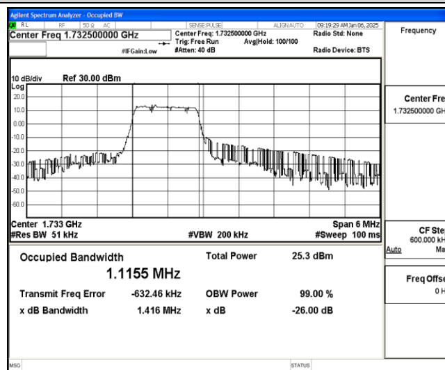
Band4-3MHz-QPSK-20175-6-0-Low-1.1155-1.416-PASS
