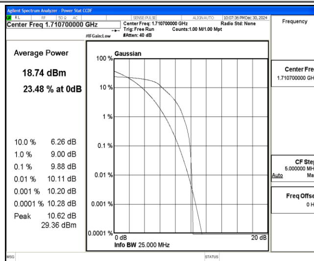
Band4-1.4MHz-16QAM-19957-6-0-Low-9.88-&lt;=13-PASS
