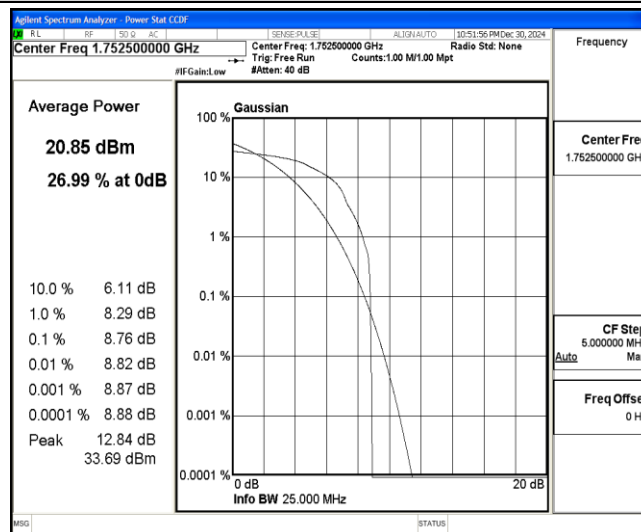
Band4-5MHz-16QAM-20375-1-0-High-8.76-&lt;=13-PASS
