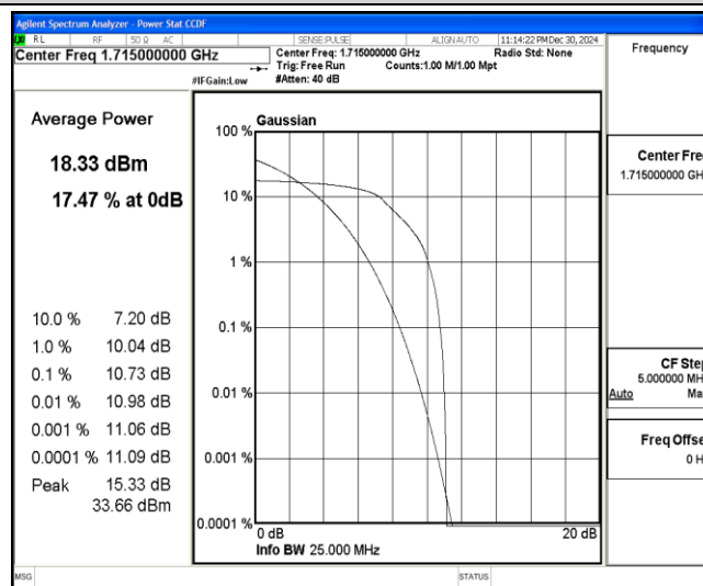
Band4-10MHz-QPSK-20000-6-0-Low-10.73-&lt;=13-PASS
