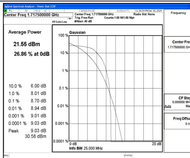
Band4-15MHz-QPSK-20025-6-0-Low-8.70-&lt;=13-PASS
