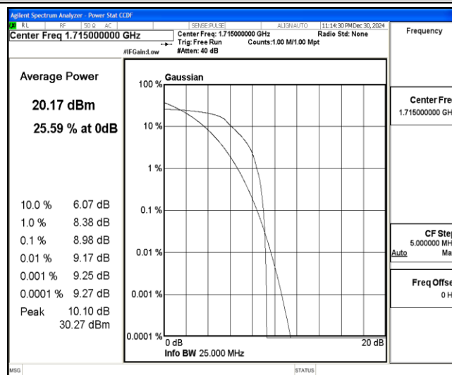
Band4-10MHz-16QAM-20000-6-0-Low-8.98-&lt;=13-PASS
