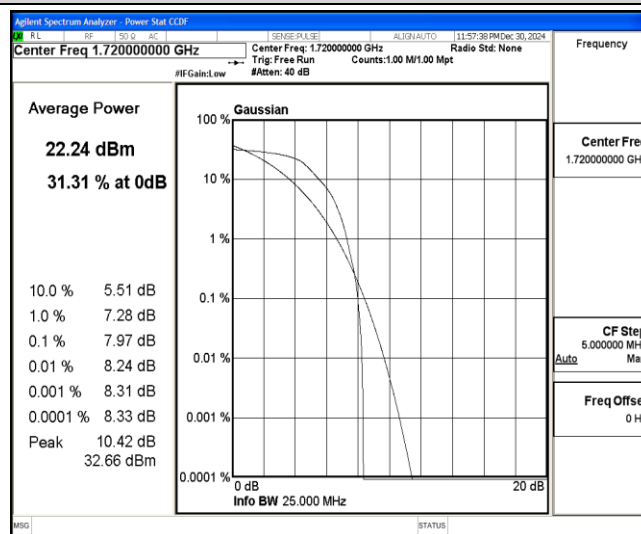
Band4-20MHz-QPSK-20050-6-0-Low-7.97-&lt;=13-PASS
