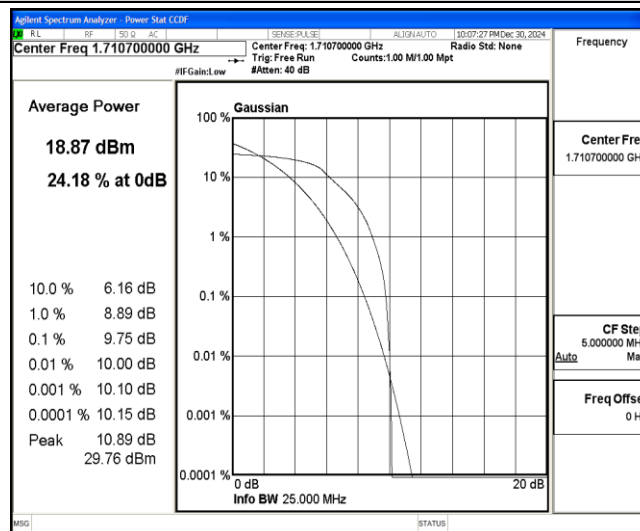
Band4-1.4MHz-QPSK-19957-6-0-Low-9.75-≤13-PASS
