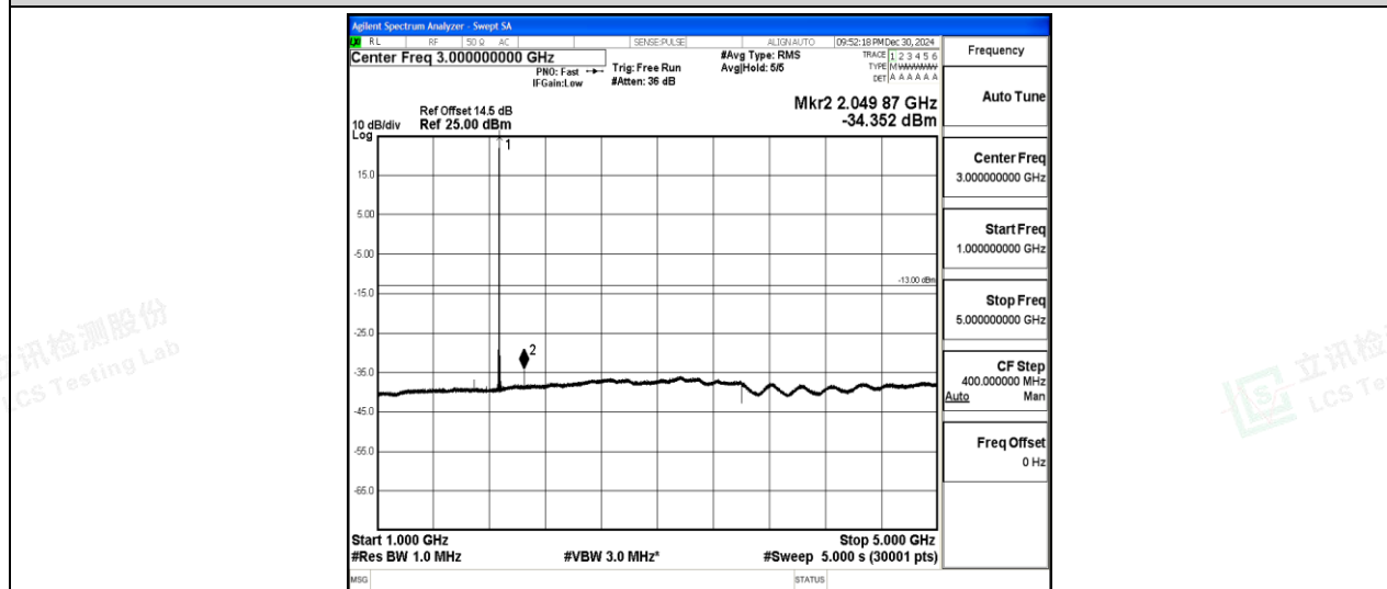
Band2-20MHz-QPSK-18900-1-0-Low-1000-5000--34.35-PASS
