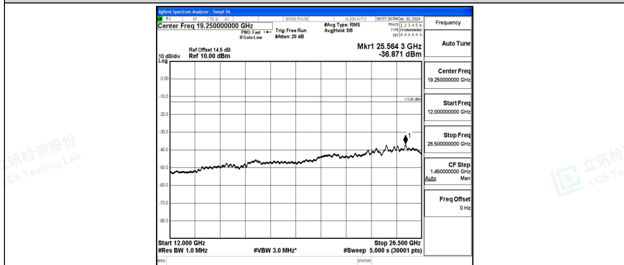
Band2-20MHz-QPSK-19100-1-0-High-12000-26500--36.87-PASS
