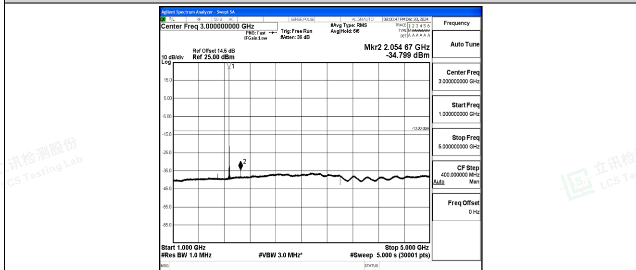
Band2-10MHz-16QAM-18900-1-0-Low-1000-5000--34.8-PASS
