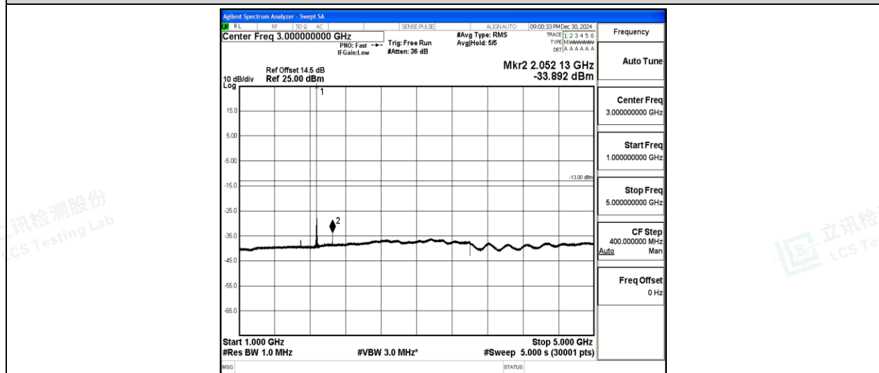
Band2-15MHz-16QAM-18900-1-0-Low-1000-5000--33.89-PASS
