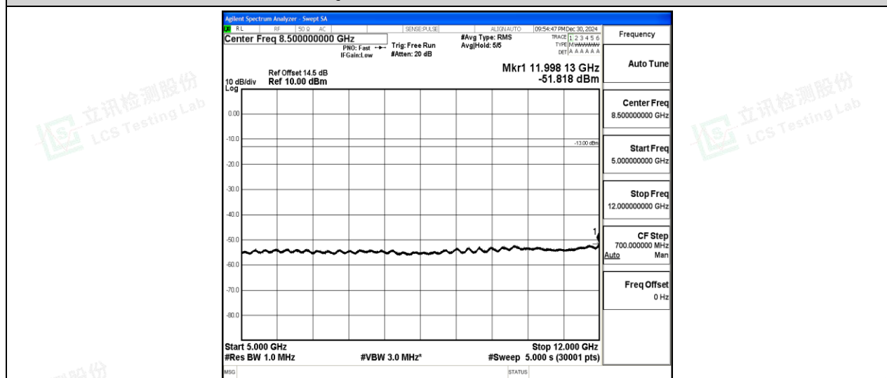
Band2-20MHz-16QAM-18900-1-0-Low-5000-12000--51.82-PASS
