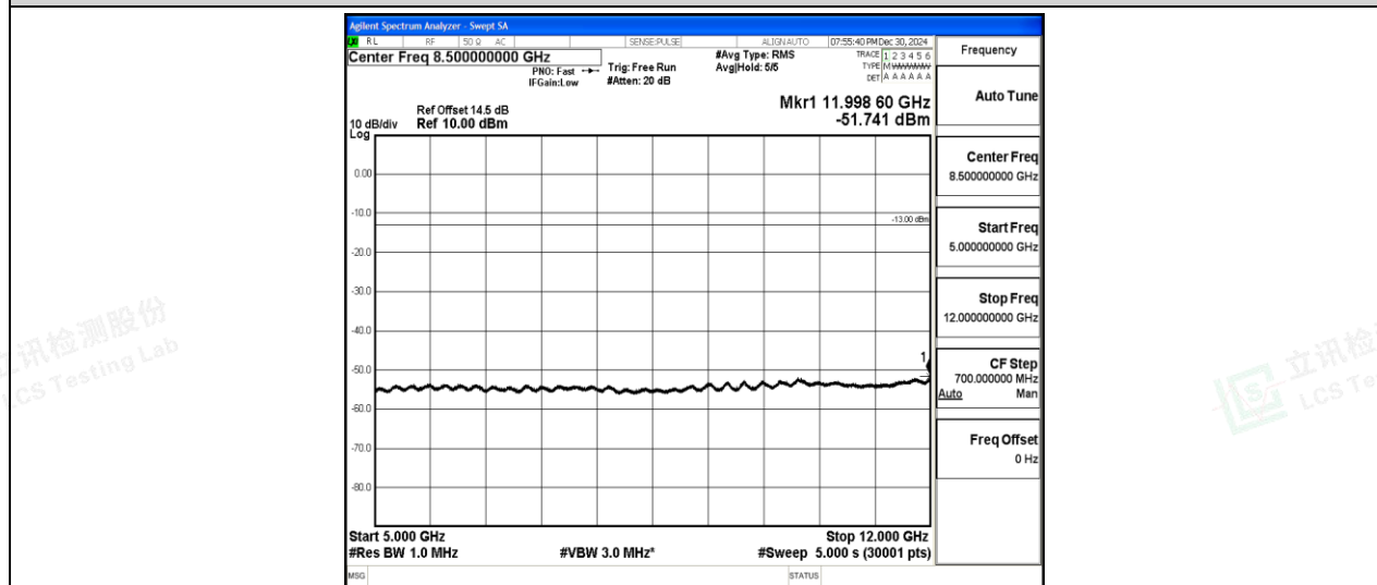
Band2-10MHz-QPSK-18650-1-0-Low-5000-12000--51.74-PASS
