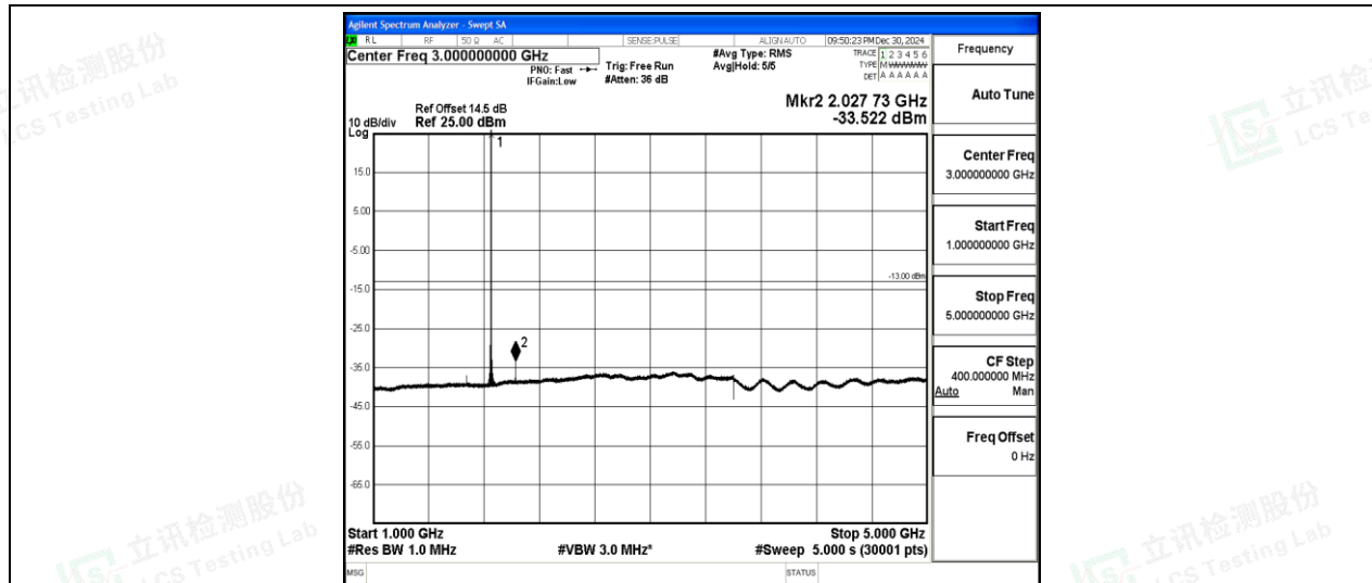
Band2-20MHz-16QAM-18700-1-0-Low-1000-5000--33.52-PASS
