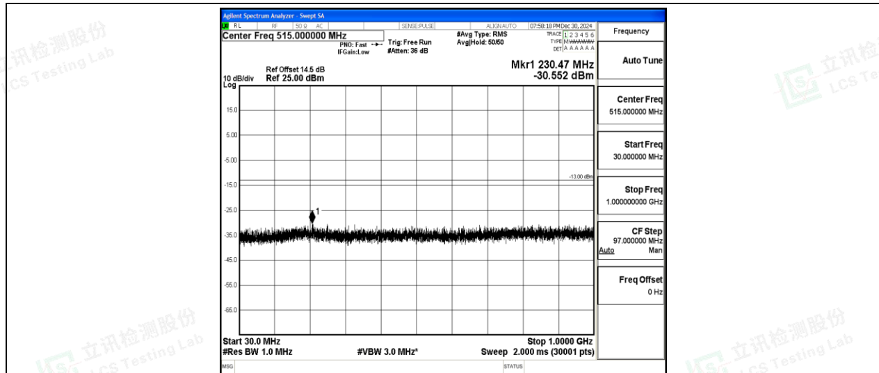
Band2-10MHz-QPSK-18900-1-0-Low-30-1000--30.55-PASS
