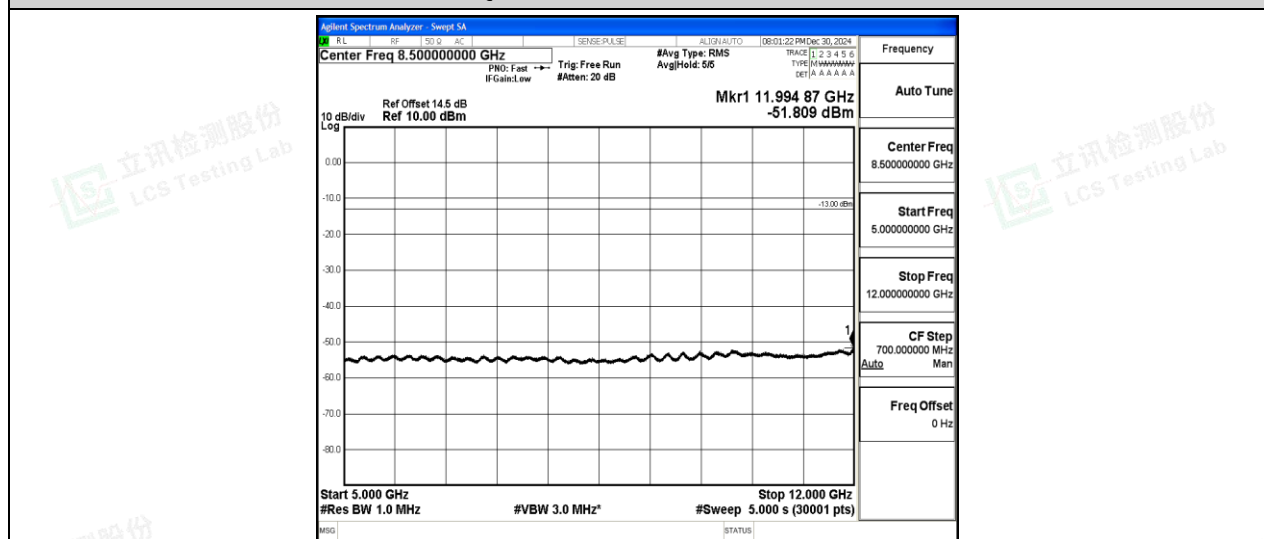
Band2-10MHz-16QAM-18900-1-0-Low-5000-12000--51.81-PASS
