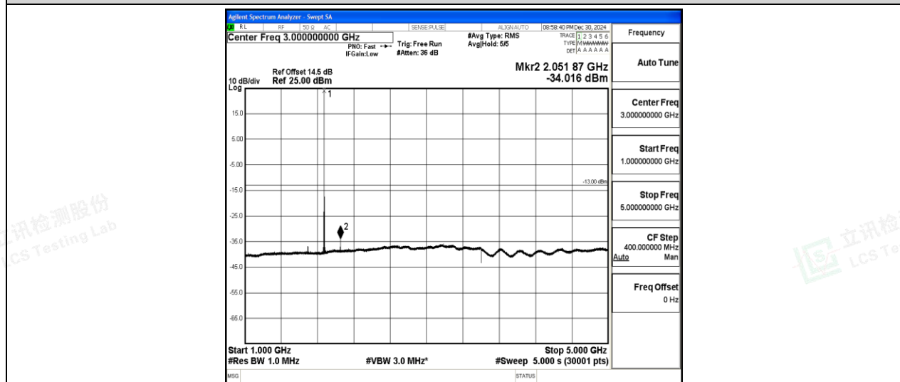
Band2-15MHz-QPSK-18900-1-0-Low-1000-5000--34.02-PASS
