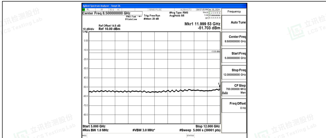
Band2-20MHz-QPSK-19100-1-0-High-5000-12000--51.7-PASS
