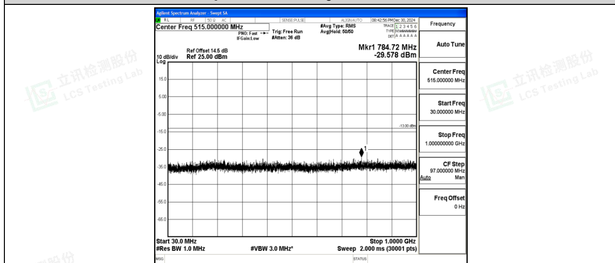
Band2-15MHz-16QAM-18675-1-0-Low-30-1000--29.58-PASS
