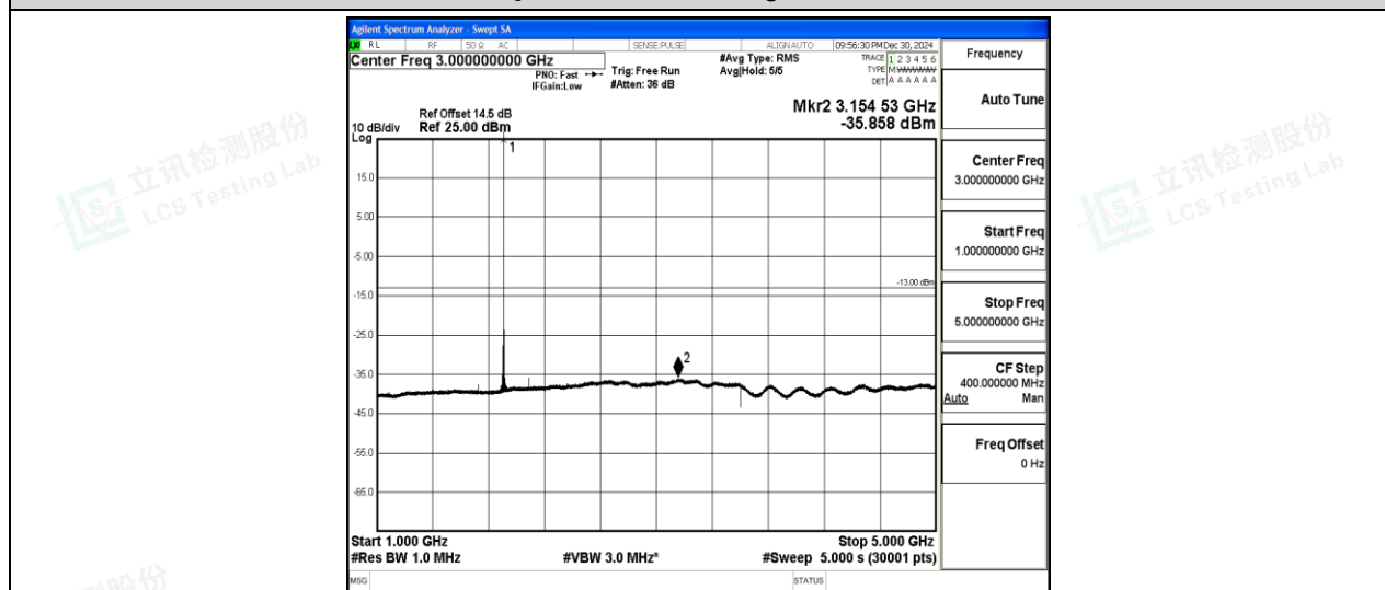
Band2-20MHz-QPSK-19100-1-0-High-1000-5000--35.86-PASS
