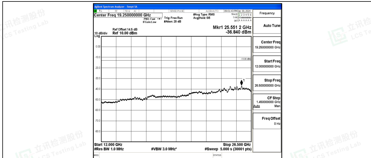
Band2-15MHz-16QAM-18900-1-0-Low-12000-26500--36.84-PASS
