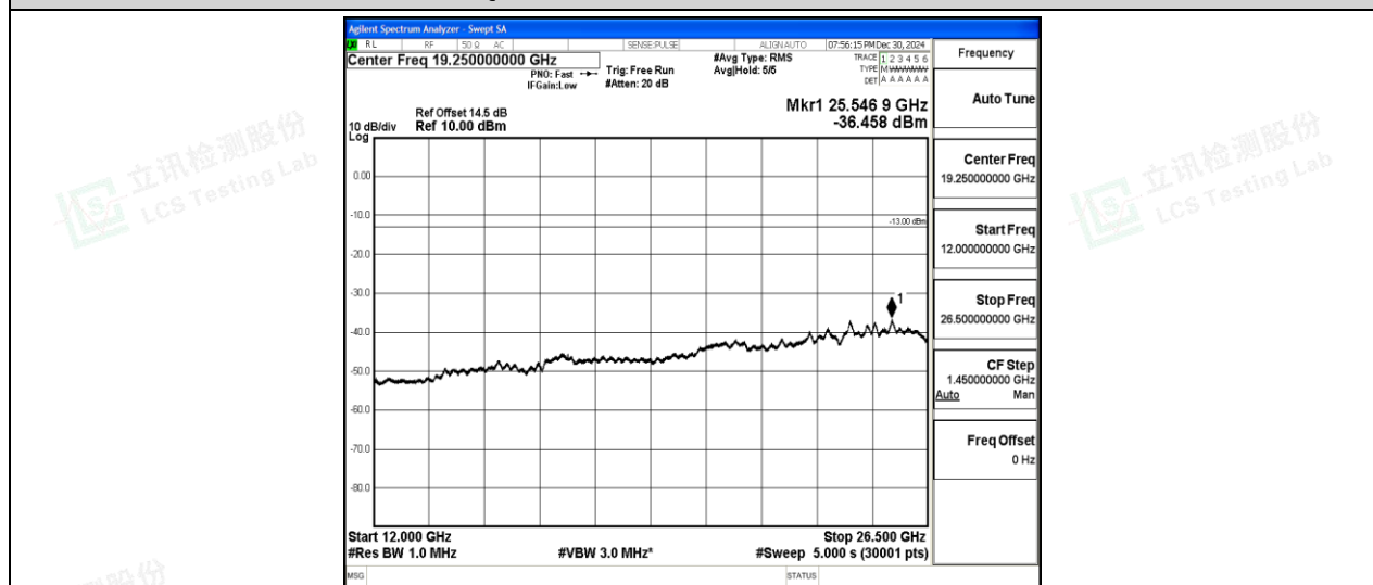
Band2-10MHz-QPSK-18650-1-0-Low-12000-26500--36.46-PASS
