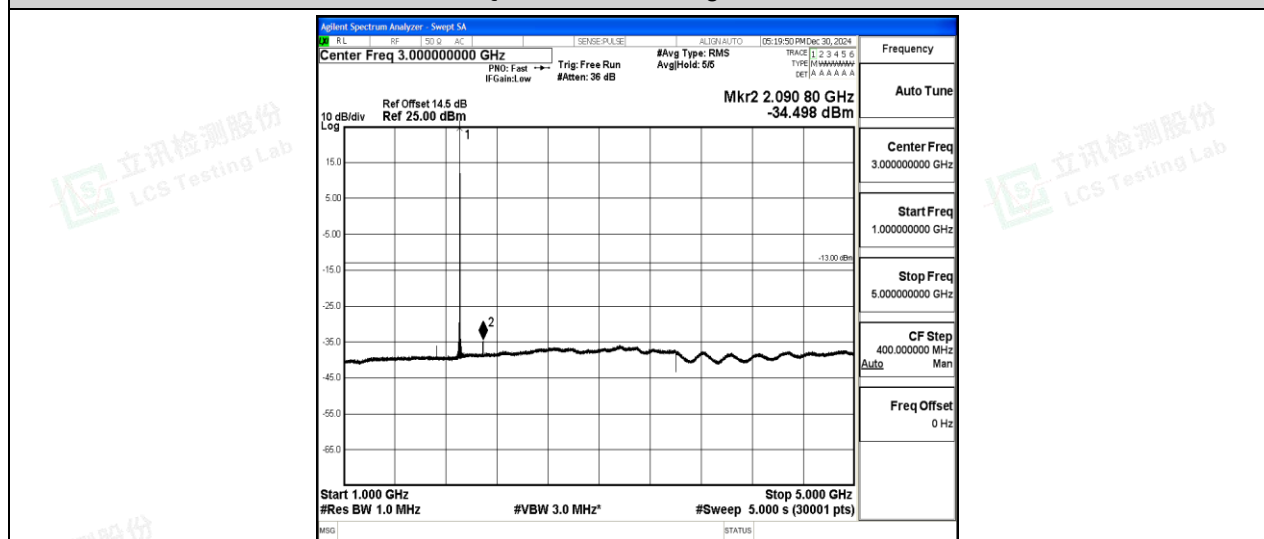
Band2-5MHz-16QAM-19175-1-0-High-1000-5000--34.5-PASS
