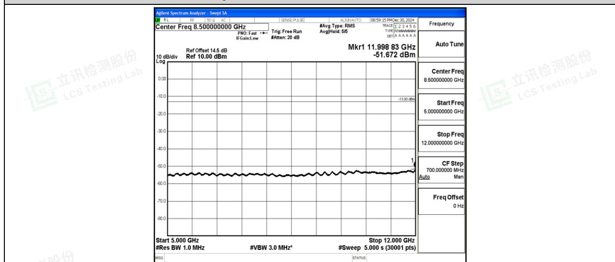
Band2-15MHz-QPSK-18900-1-0-Low-5000-12000--51.67-PASS
