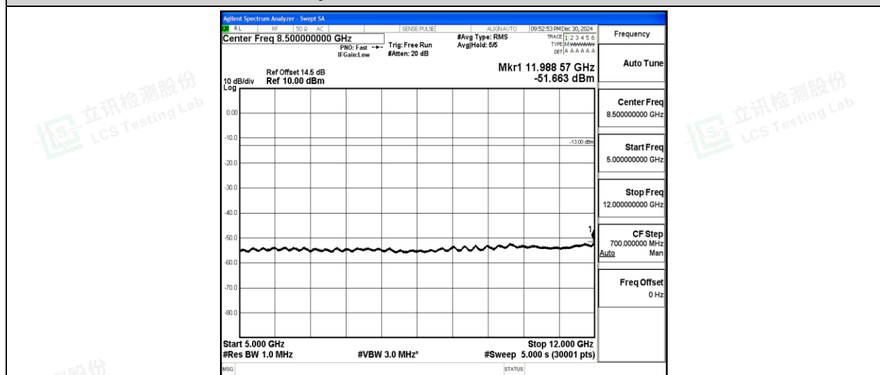
Band2-20MHz-QPSK-18900-1-0-Low-5000-12000--51.66-PASS
