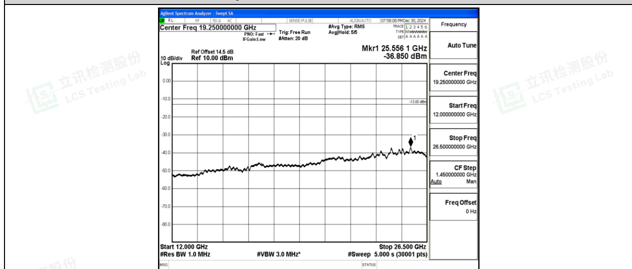
Band2-10MHz-16QAM-18650-1-0-Low-12000-26500--36.85-PASS
