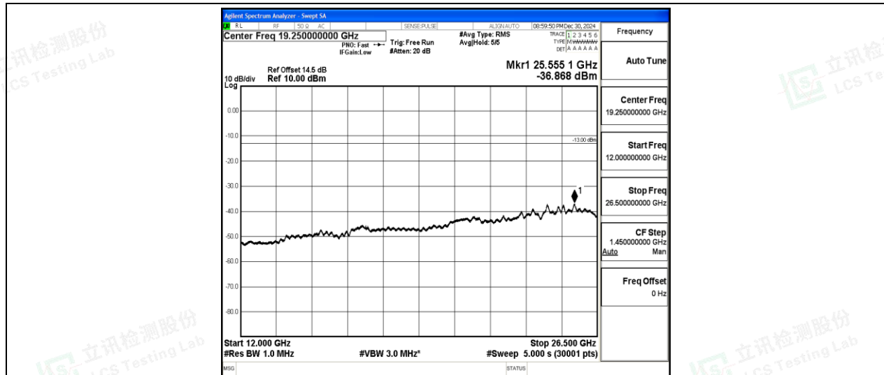
Band2-15MHz-QPSK-18900-1-0-Low-12000-26500--36.87-PASS
