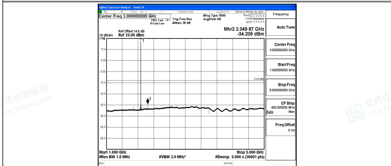
Band2-20MHz-16QAM-18900-1-0-Low-1000-5000--34.21-PASS
