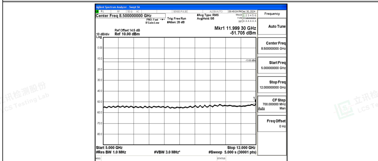
Band2-20MHz-QPSK-18700-1-0-Low-5000-12000--51.71-PASS
