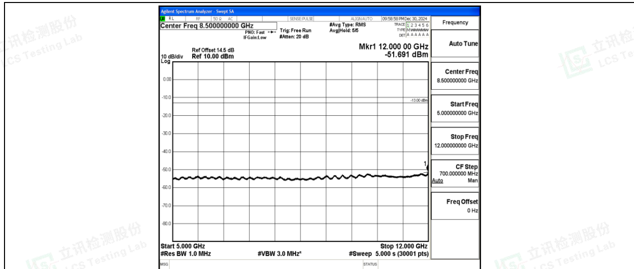
Band2-20MHz-16QAM-19100-1-0-High-5000-12000--51.69-PASS
