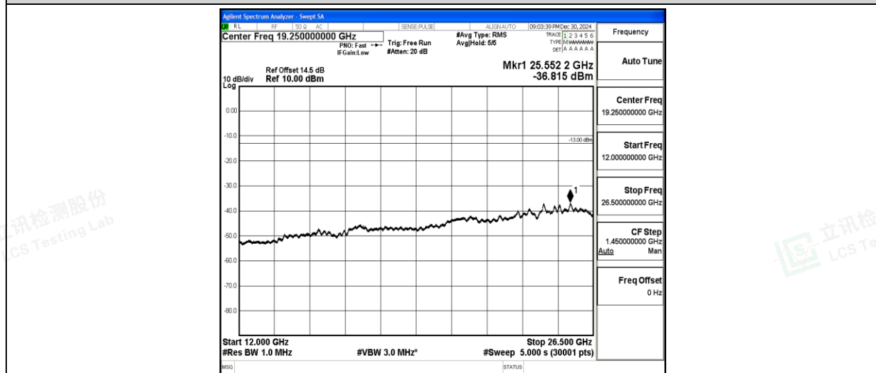
Band2-15MHz-QPSK-19125-1-0-High-12000-26500--36.82-PASS
