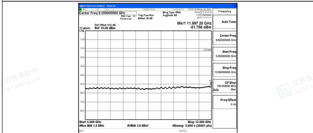
Band2-10MHz-16QAM-18650-1-0-Low-5000-12000--51.76-PASS
