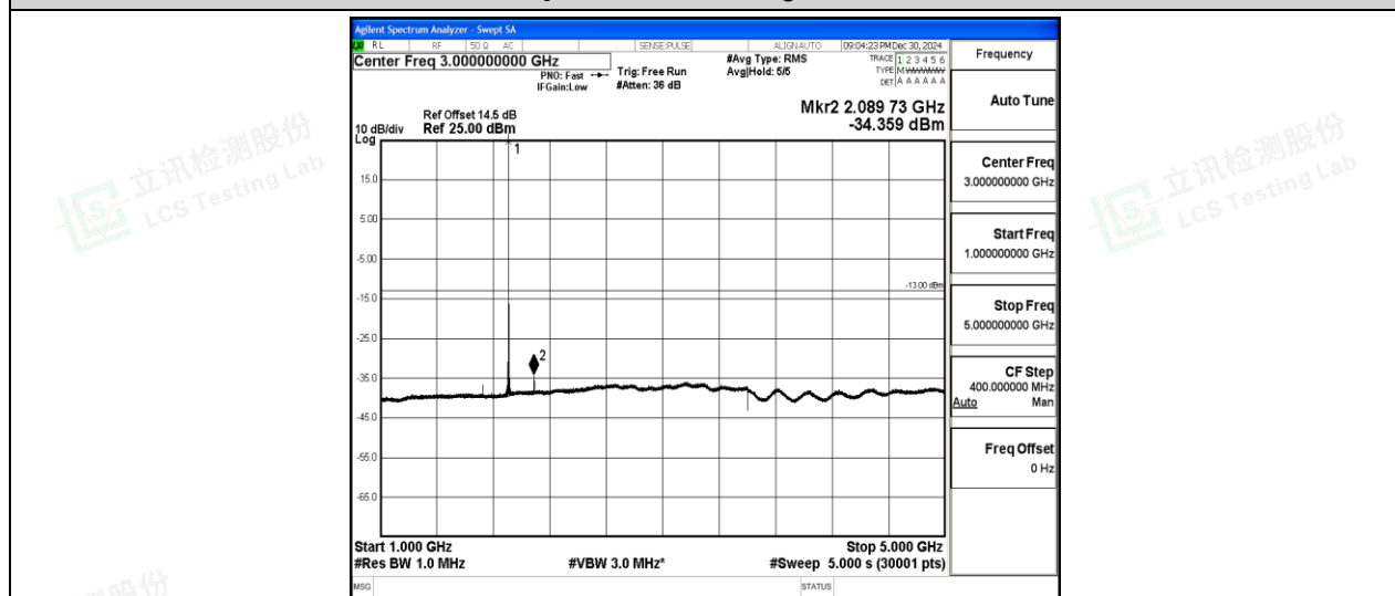
Band2-15MHz-16QAM-19125-1-0-High-1000-5000--34.36-PASS
