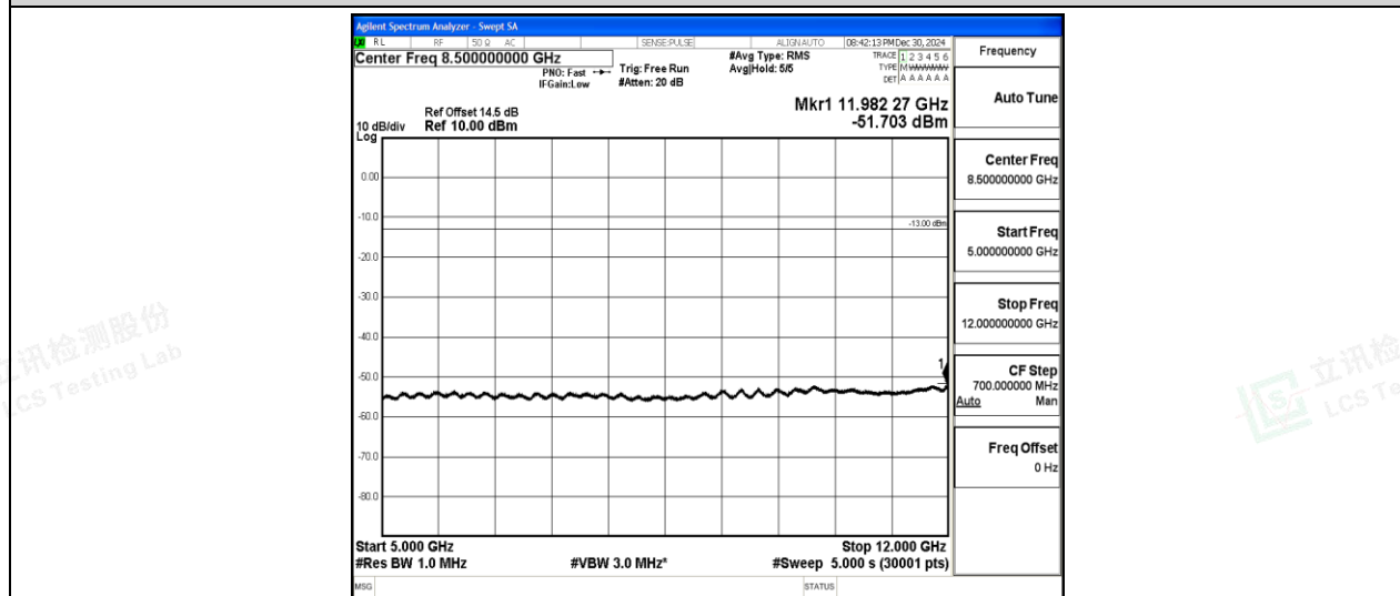
Band2-15MHz-QPSK-18675-1-0-Low-5000-12000--51.7-PASS
