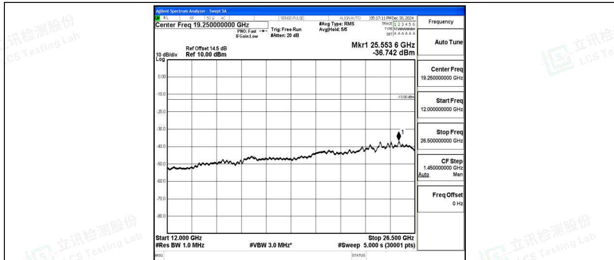
Band2-5MHz-16QAM-18900-1-0-Low-12000-26500--36.74-PASS
