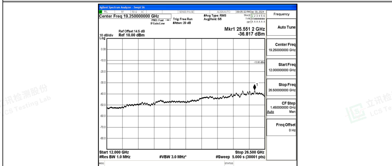
Band2-15MHz-16QAM-19125-1-0-High-12000-26500--36.82-PASS
