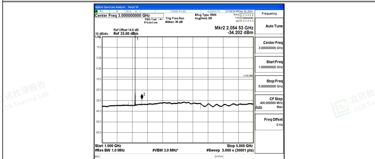
Band2-10MHz-QPSK-18900-1-0-Low-1000-5000--34.2-PASS
