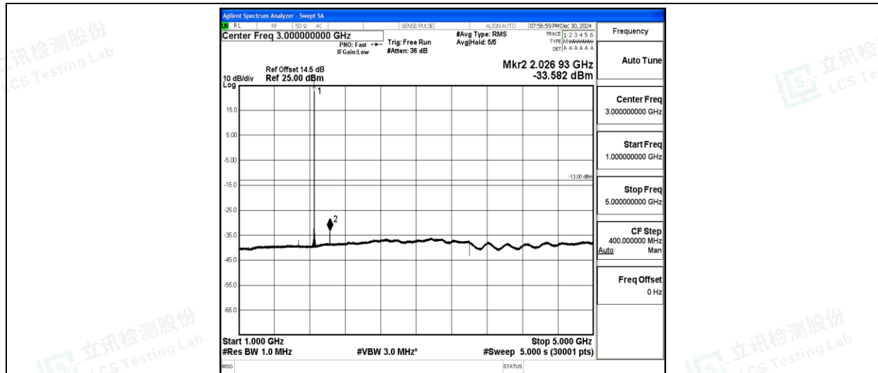
Band2-10MHz-16QAM-18650-1-0-Low-1000-5000--33.58-PASS
