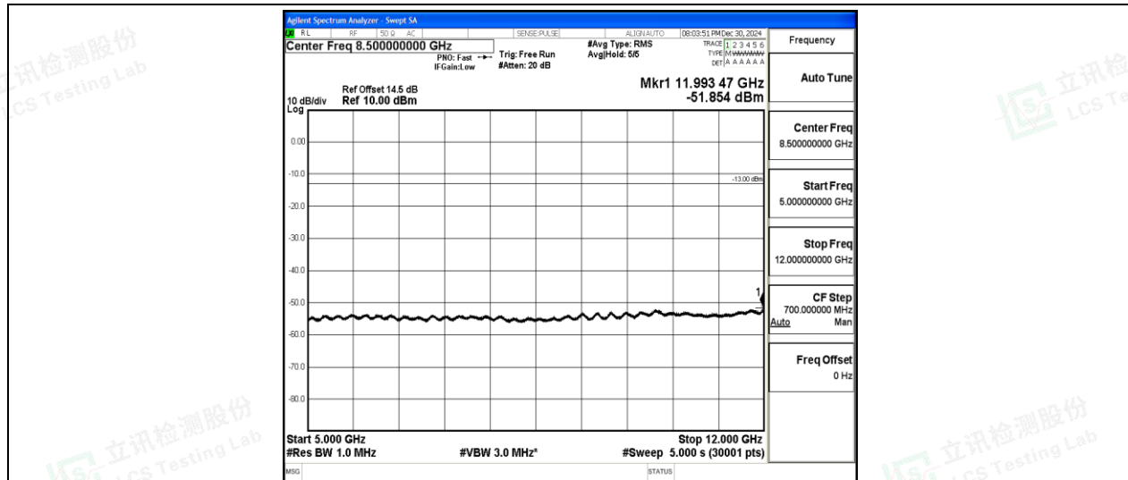
Band2-10MHz-QPSK-19150-1-0-High-5000-12000--51.85-PASS
