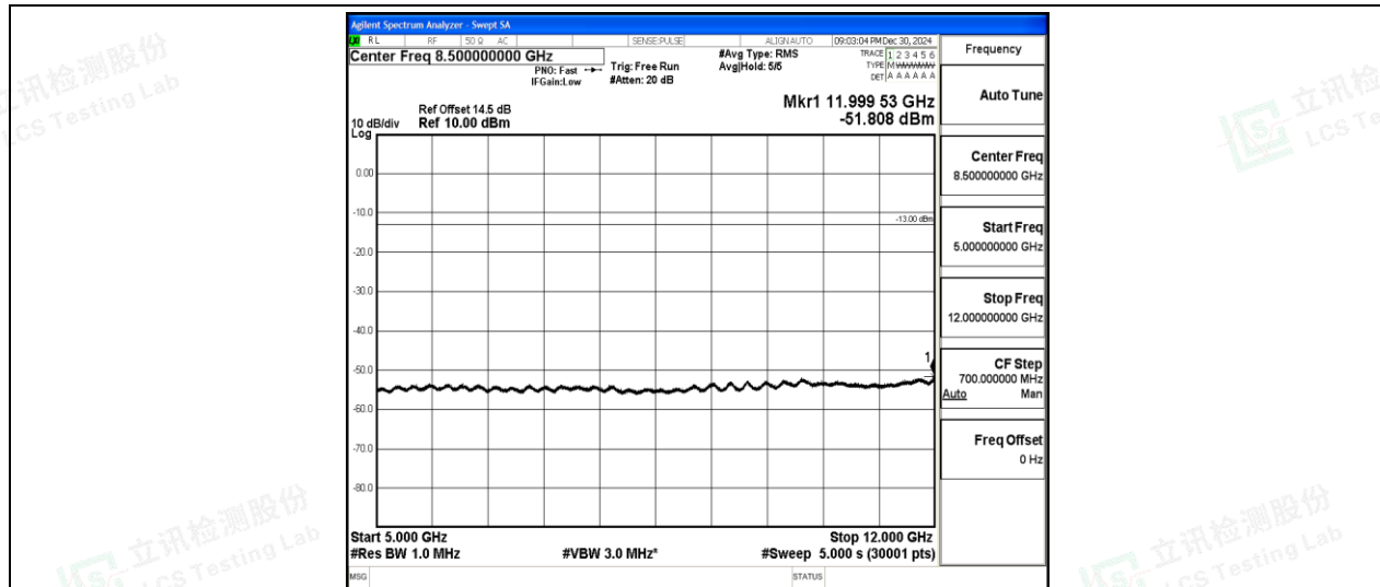
Band2-15MHz-QPSK-19125-1-0-High-5000-12000--51.81-PASS
