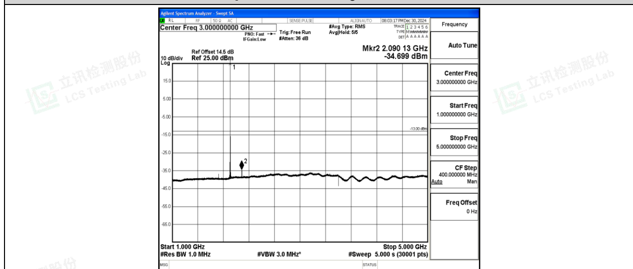
Band2-10MHz-QPSK-19150-1-0-High-1000-5000--34.7-PASS
