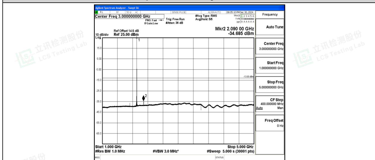
Band2-10MHz-16QAM-19150-1-0-High-1000-5000--34.69-PASS
