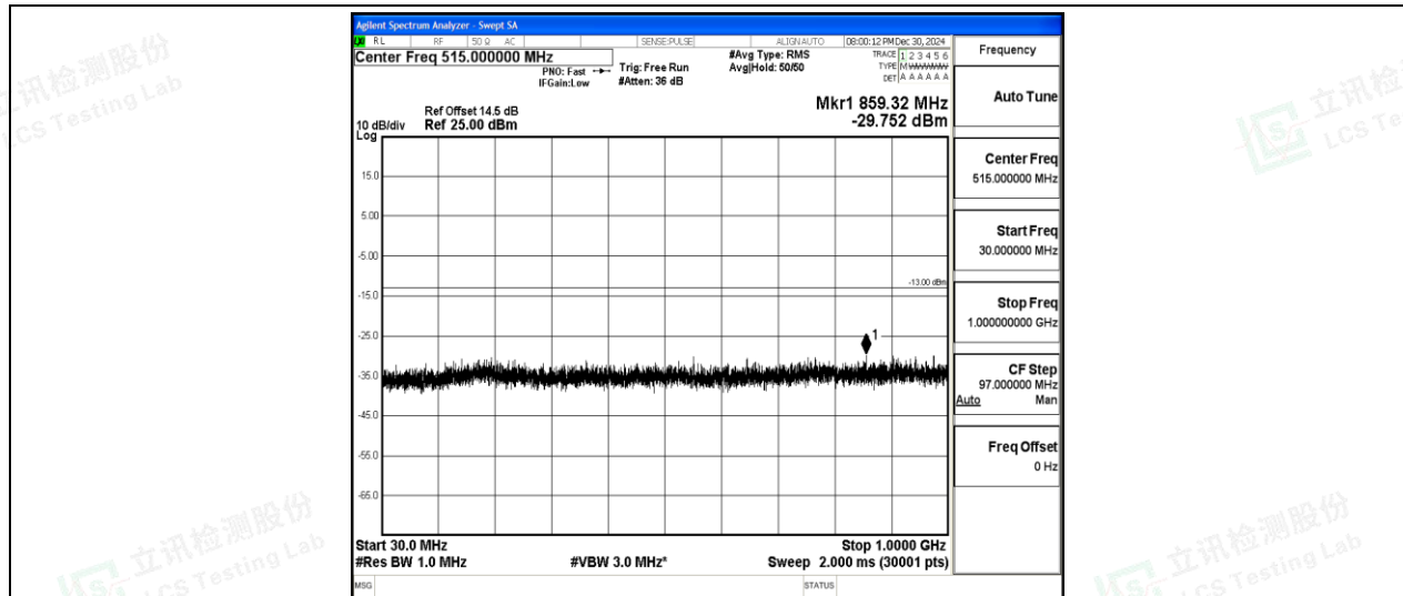
Band2-10MHz-16QAM-18900-1-0-Low-30-1000--29.75-PASS
