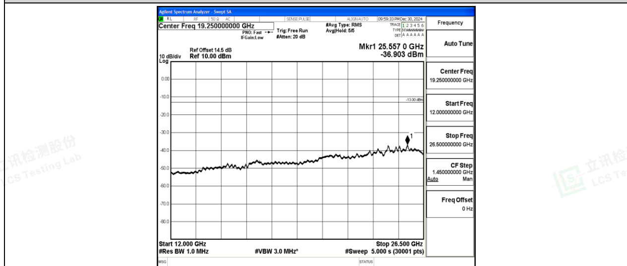
Band2-20MHz-16QAM-19100-1-0-High-12000-26500--36.9-PASS
