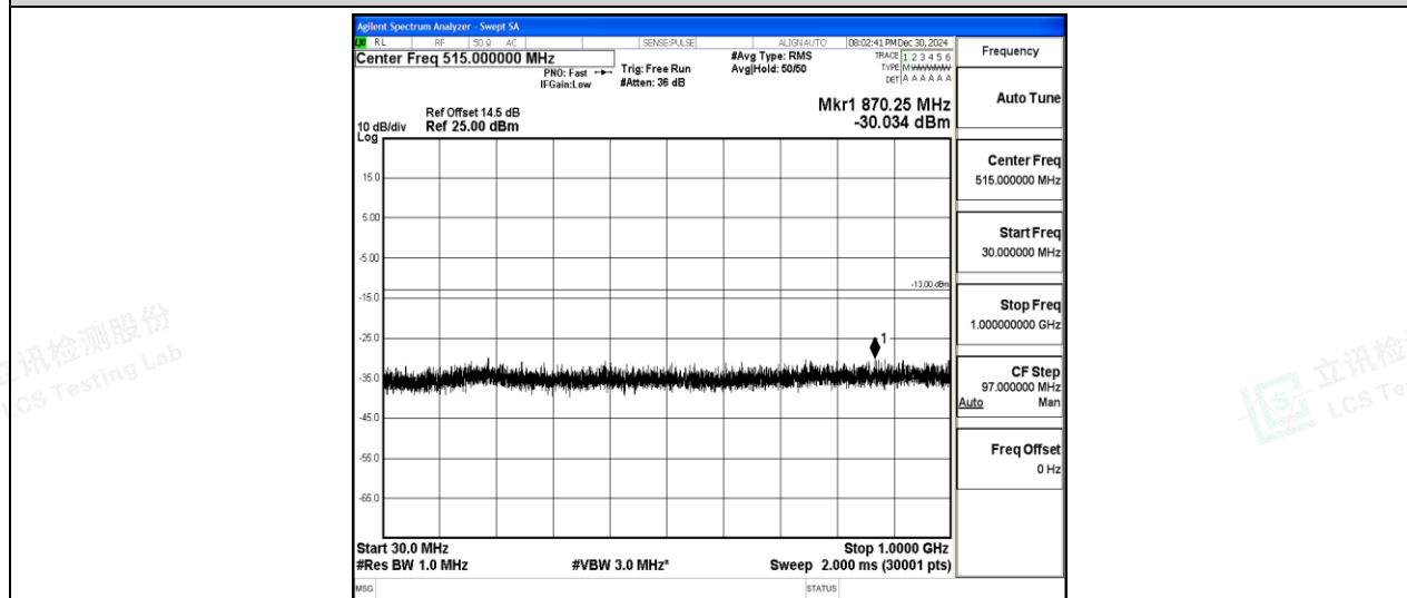
Band2-10MHz-QPSK-19150-1-0-High-30-1000--30.03-PASS
