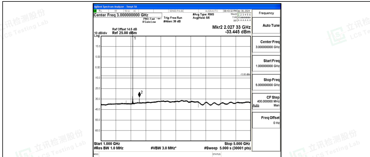
Band2-15MHz-16QAM-18675-1-0-Low-1000-5000--33.45-PASS
