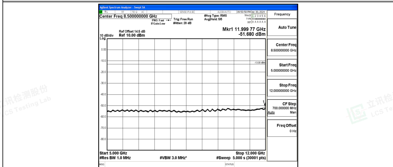
Band2-20MHz-16QAM-18700-1-0-Low-5000-12000--51.68-PASS
