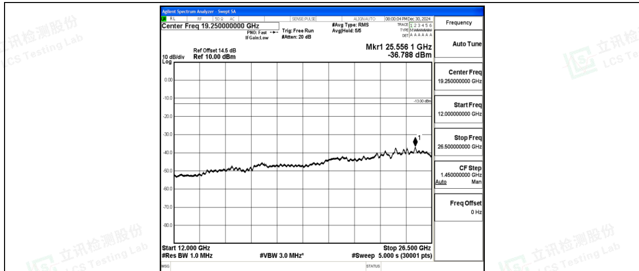
Band2-10MHz-QPSK-18900-1-0-Low-12000-26500--36.79-PASS
