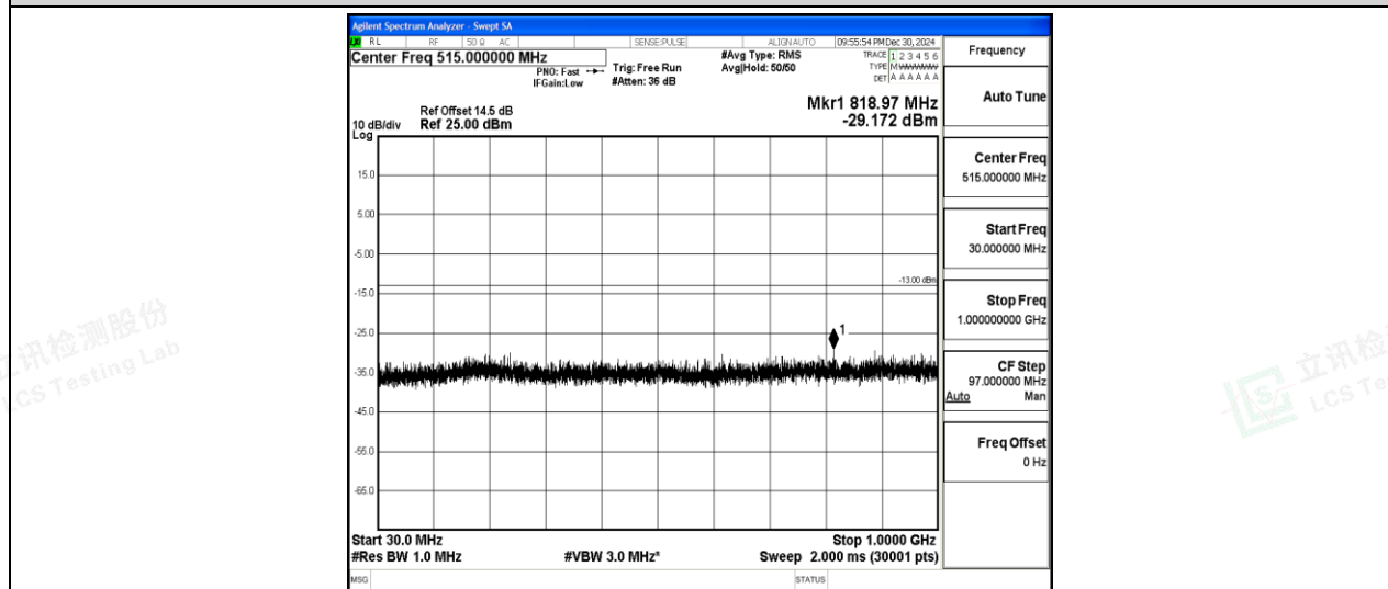
Band2-20MHz-QPSK-19100-1-0-High-30-1000--29.17-PASS
