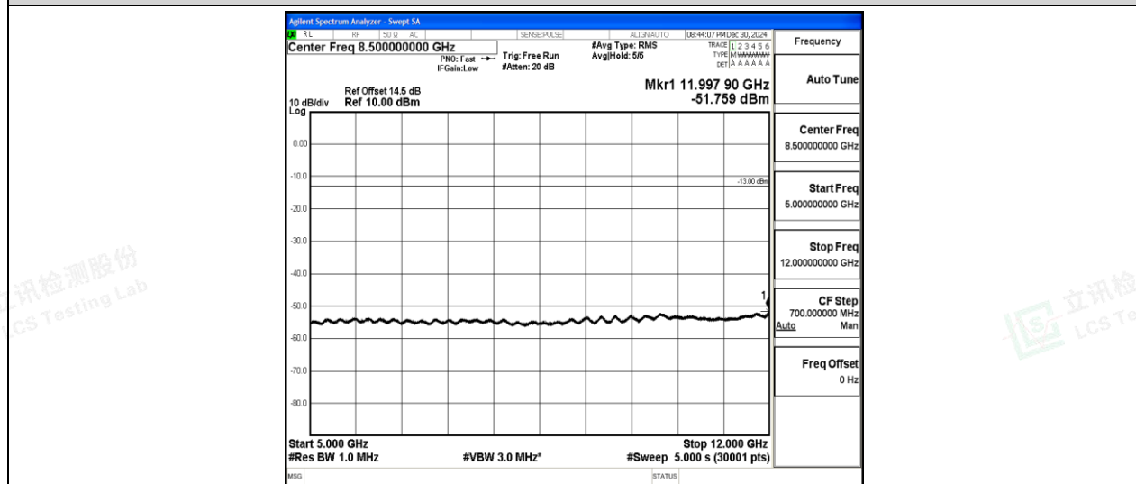
Band2-15MHz-16QAM-18675-1-0-Low-5000-12000--51.76-PASS
