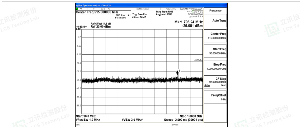
Band2-15MHz-16QAM-18900-1-0-Low-30-1000--29.08-PASS
