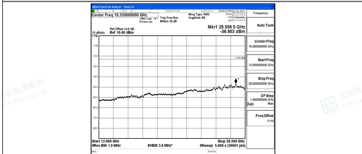
Band2-10MHz-16QAM-19150-1-0-High-12000-26500--36.95-PASS
