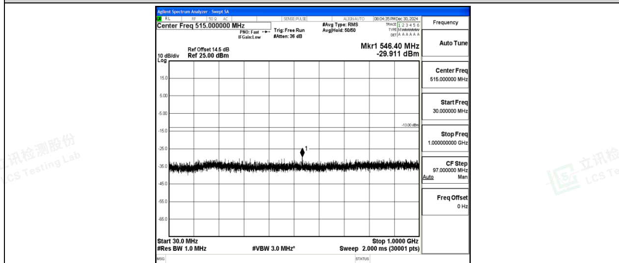
Band2-10MHz-16QAM-19150-1-0-High-30-1000--29.91-PASS
