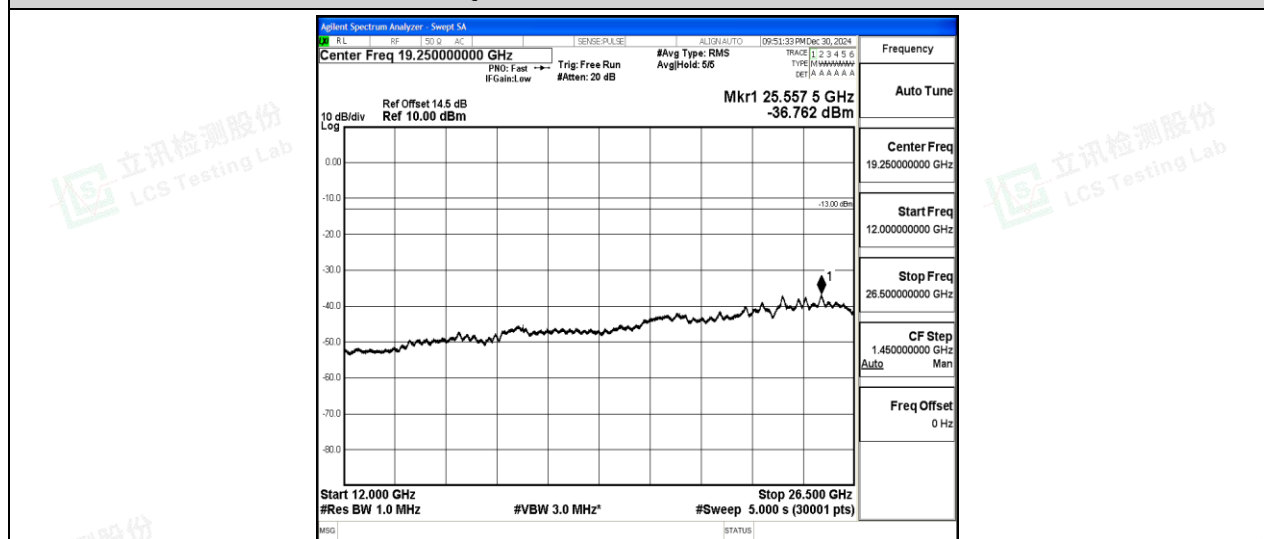
Band2-20MHz-16QAM-18700-1-0-Low-12000-26500--36.76-PASS
