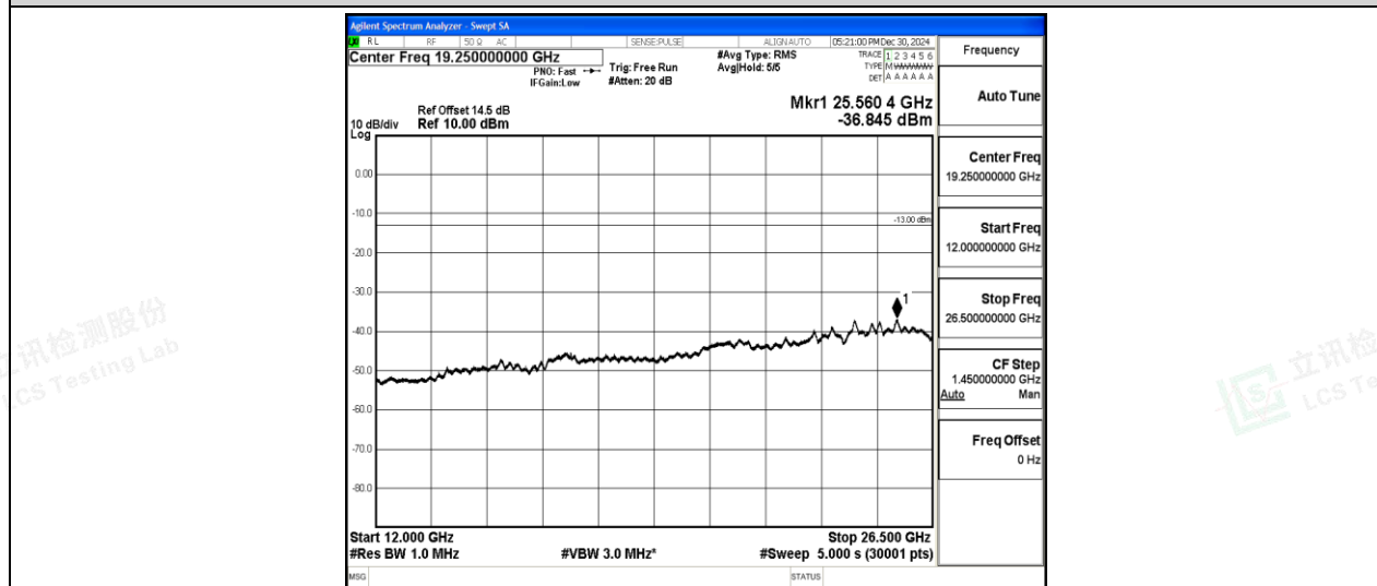
Band2-5MHz-16QAM-19175-1-0-High-12000-26500--36.85-PASS
