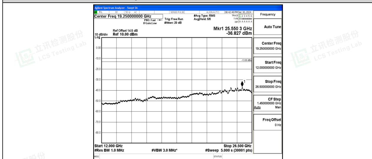
Band2-15MHz-QPSK-18675-1-0-Low-12000-26500--36.83-PASS
