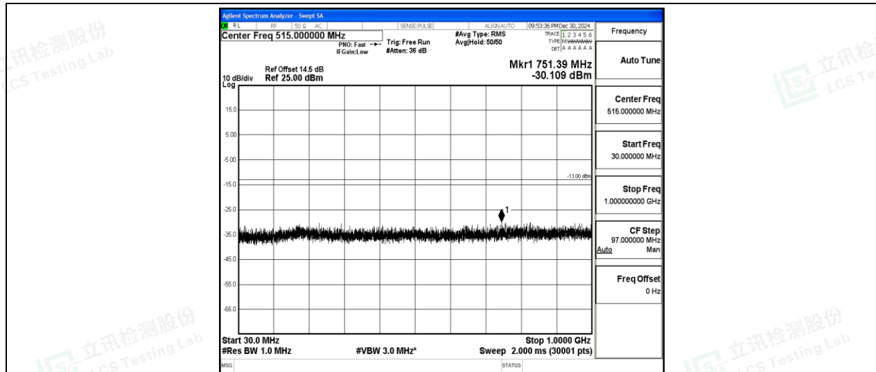
Band2-20MHz-16QAM-18900-1-0-Low-30-1000--30.11-PASS
