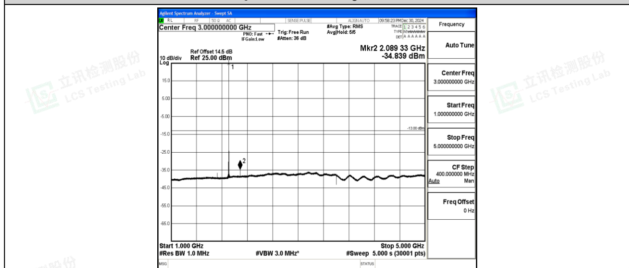
Band2-20MHz-16QAM-19100-1-0-High-1000-5000--34.84-PASS
