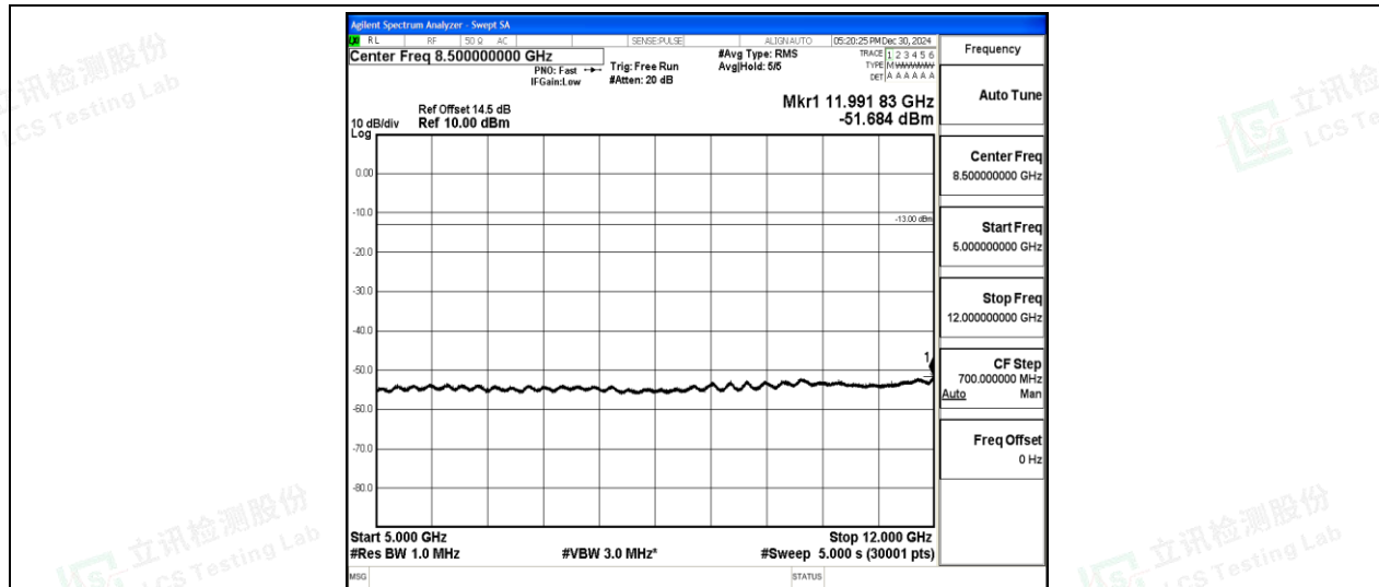
Band2-5MHz-16QAM-19175-1-0-High-5000-12000--51.68-PASS
