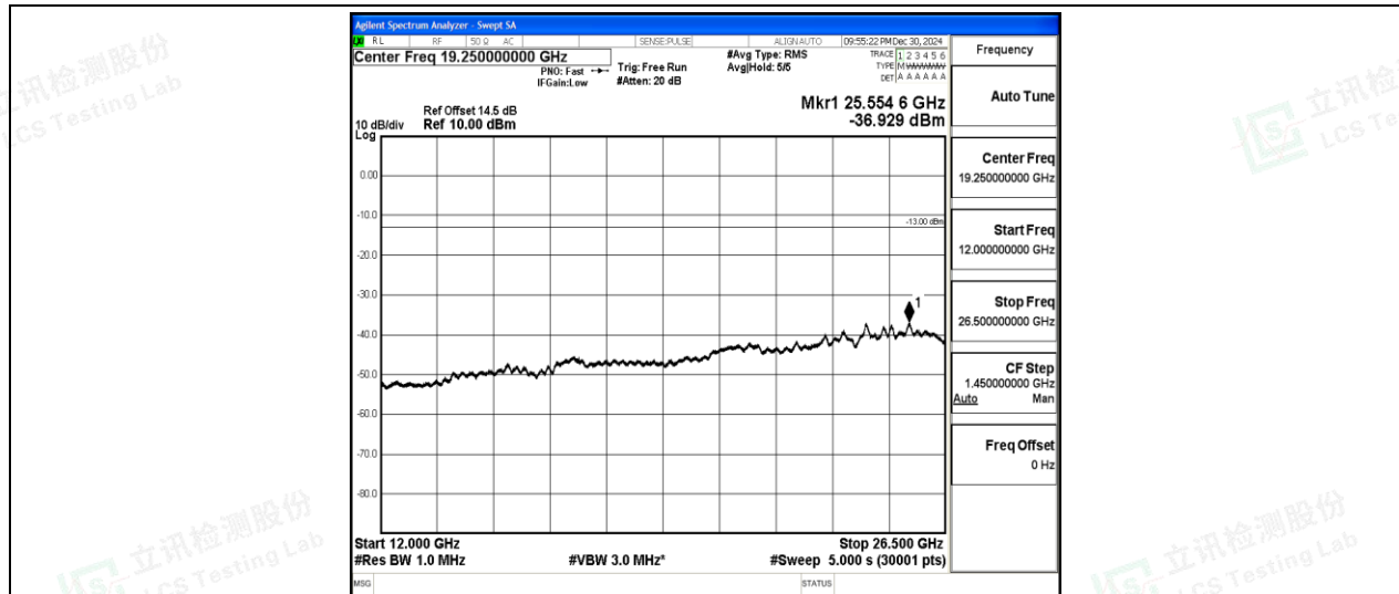
Band2-20MHz-16QAM-18900-1-0-Low-12000-26500--36.93-PASS
