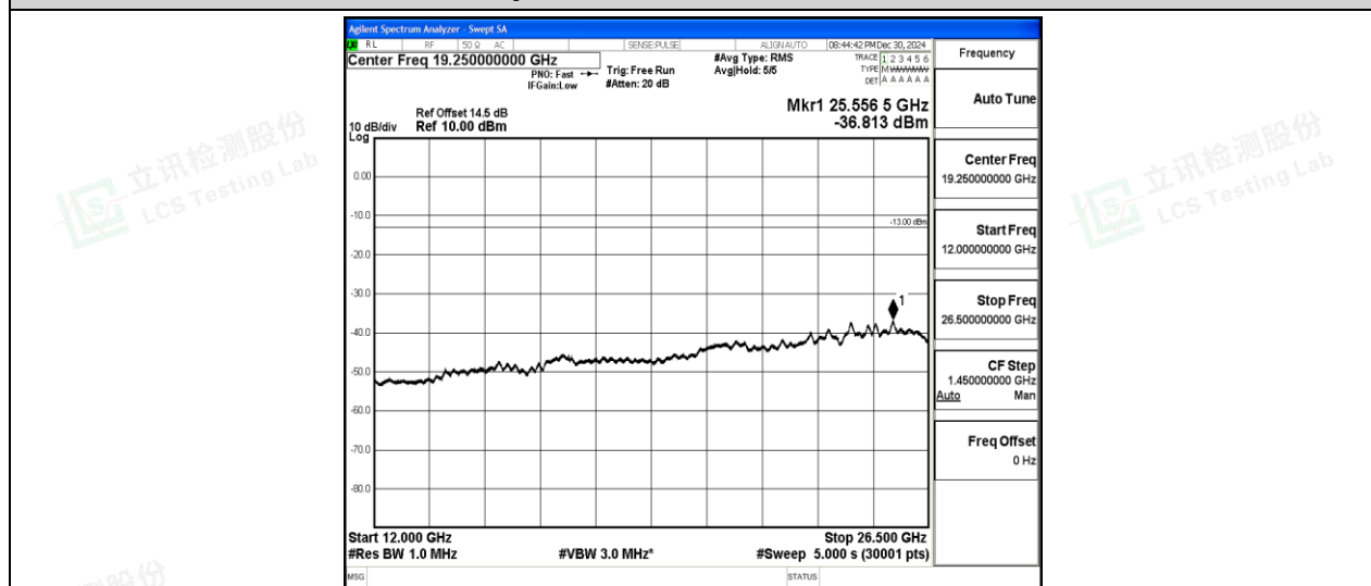
Band2-15MHz-16QAM-18675-1-0-Low-12000-26500--36.81-PASS
