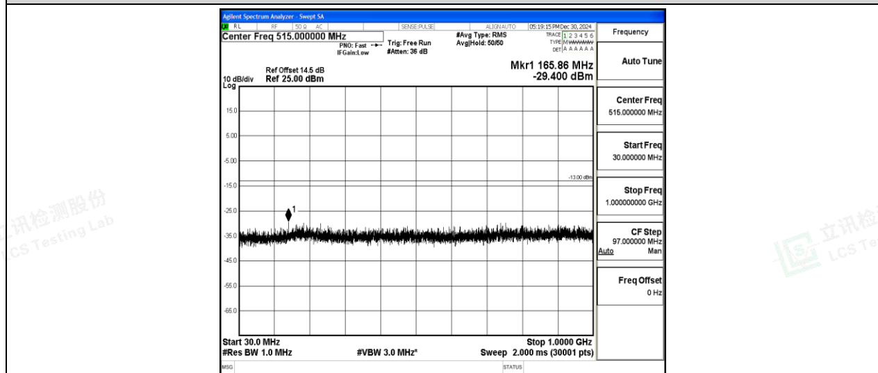
Band2-5MHz-16QAM-19175-1-0-High-30-1000--29.4-PASS
