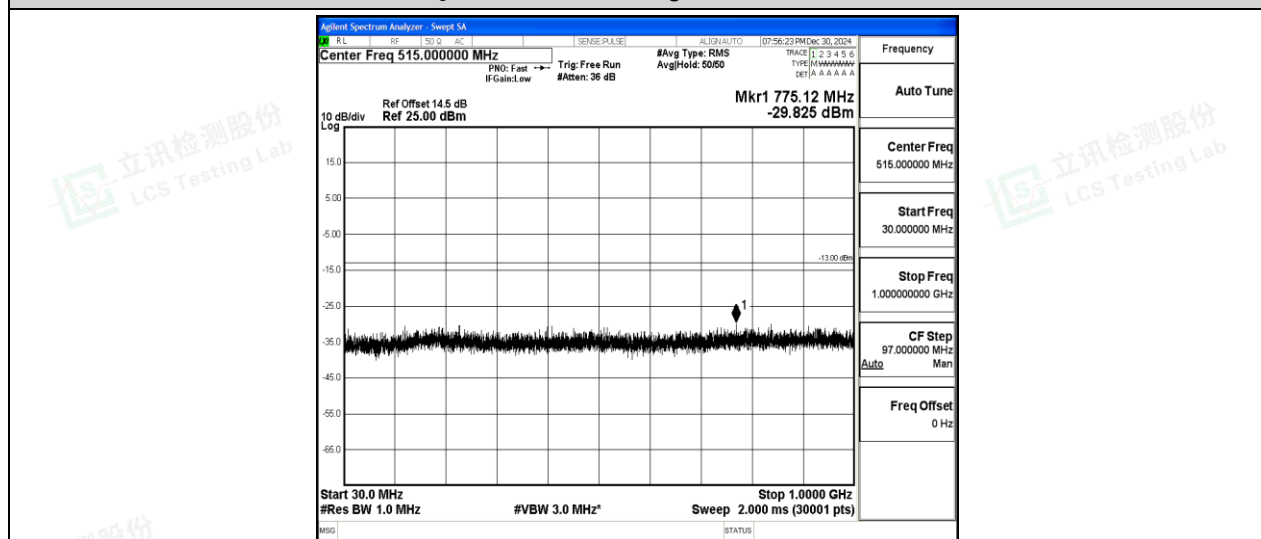
Band2-10MHz-16QAM-18650-1-0-Low-30-1000--29.83-PASS
