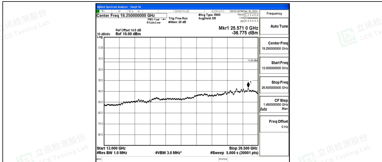
Band2-20MHz-QPSK-18900-1-0-Low-12000-26500--36.78-PASS
