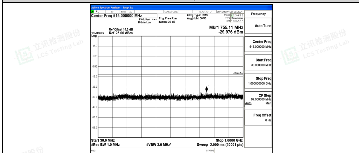
Band2-15MHz-QPSK-18675-1-0-Low-30-1000--29.98-PASS
