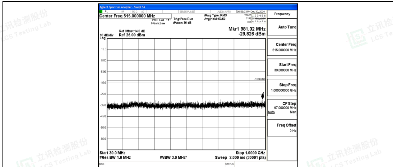
Band2-15MHz-QPSK-18900-1-0-Low-30-1000--29.83-PASS
