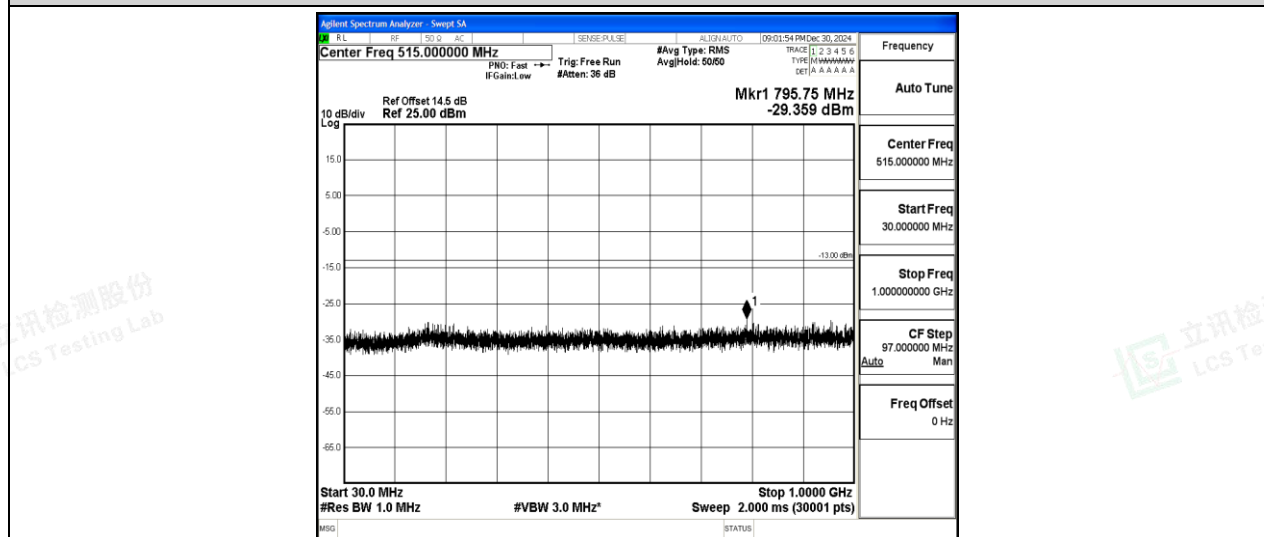
Band2-15MHz-QPSK-19125-1-0-High-30-1000--29.36-PASS
