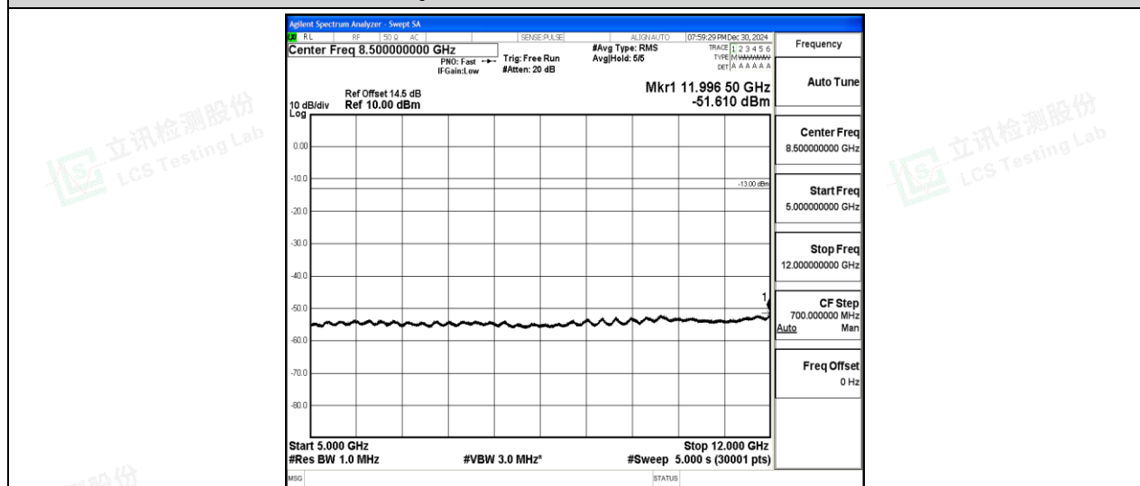
Band2-10MHz-QPSK-18900-1-0-Low-5000-12000--51.61-PASS
