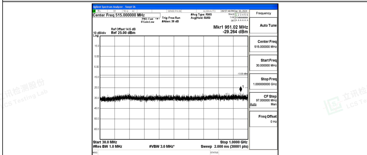
Band2-20MHz-16QAM-19100-1-0-High-30-1000--29.26-PASS
