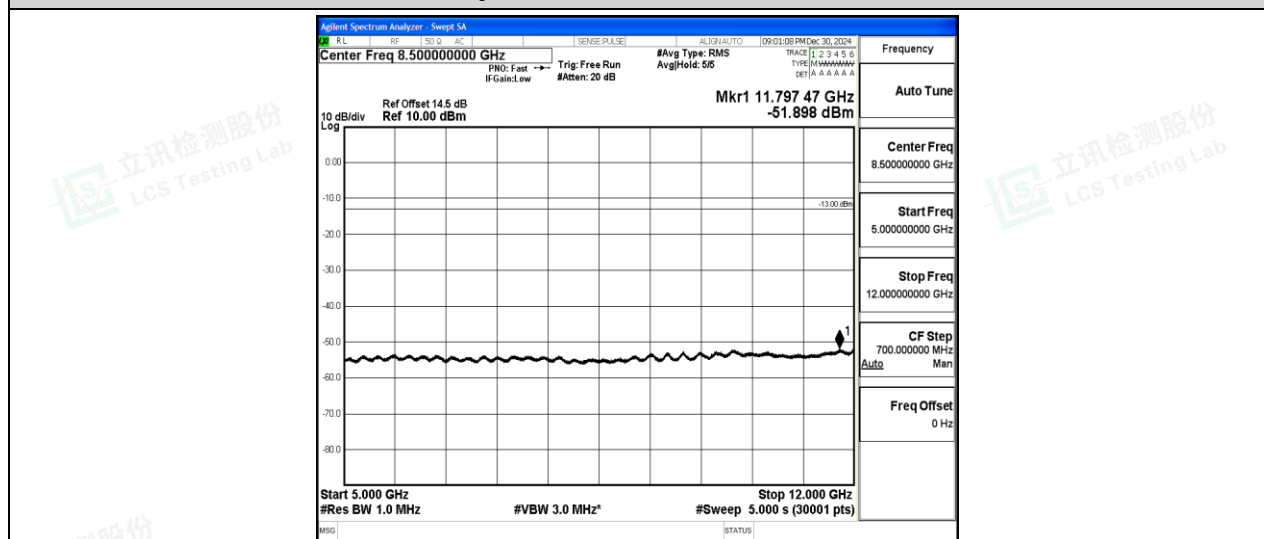
Band2-15MHz-16QAM-18900-1-0-Low-5000-12000--51.9-PASS
