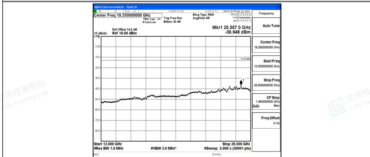
Band2-10MHz-QPSK-19150-1-0-High-12000-26500--36.95-PASS
