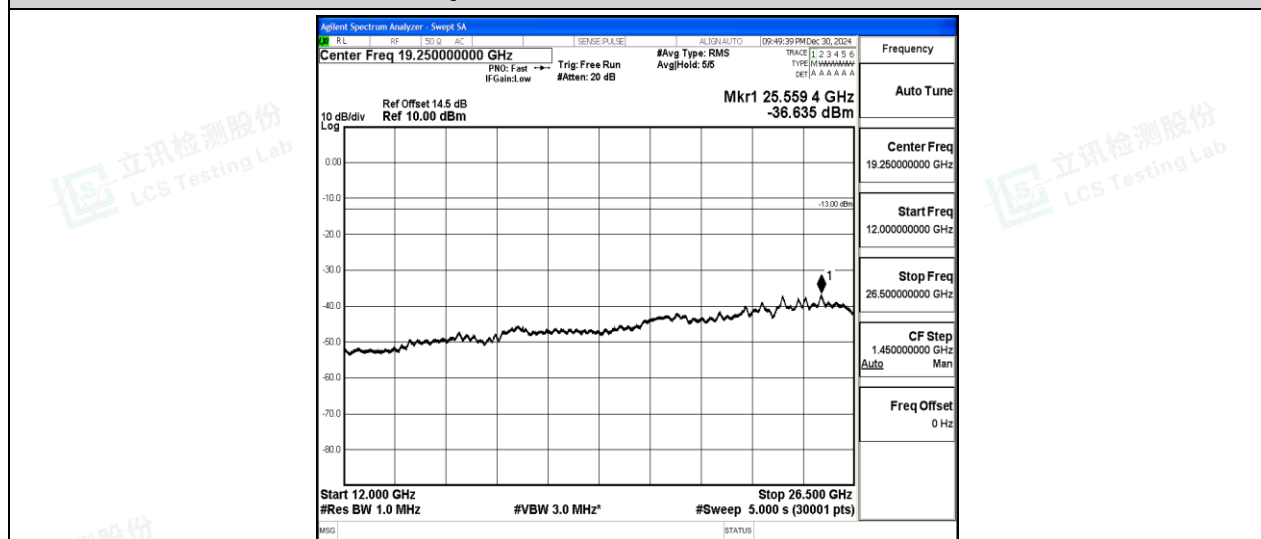
Band2-20MHz-QPSK-18700-1-0-Low-12000-26500--36.64-PASS
