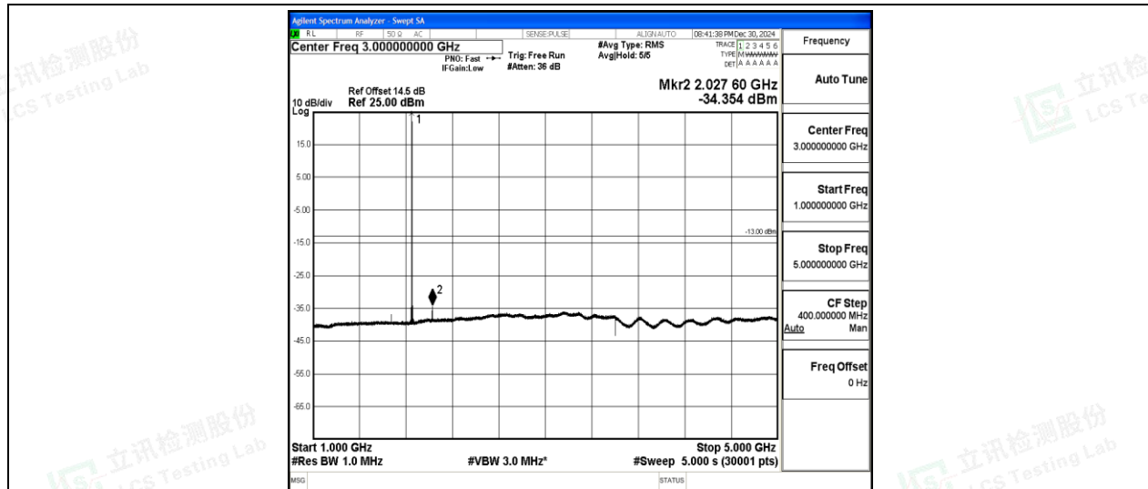
Band2-15MHz-QPSK-18675-1-0-Low-1000-5000--34.35-PASS
