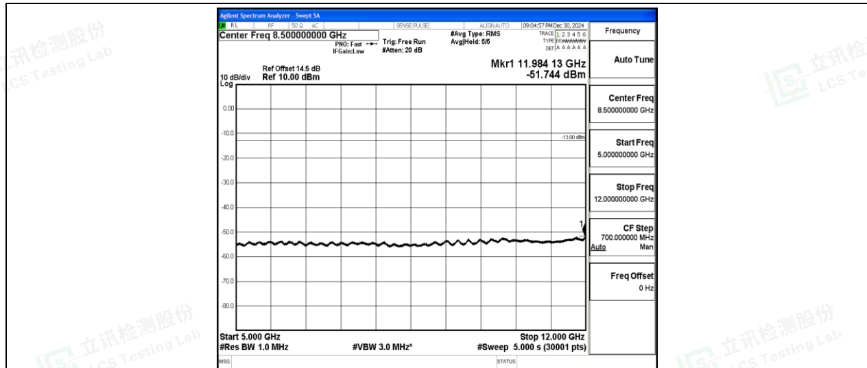
Band2-15MHz-16QAM-19125-1-0-High-5000-12000--51.74-PASS
