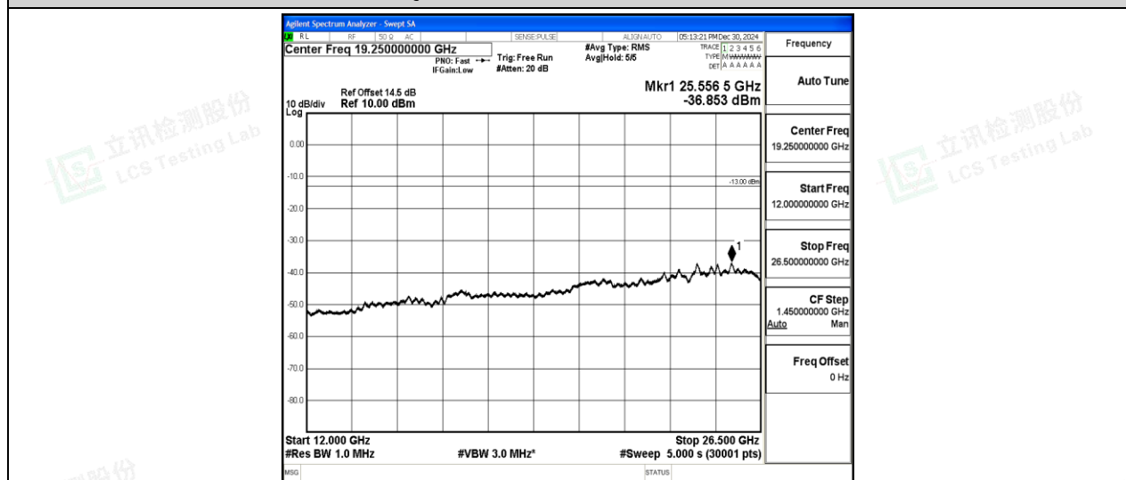
Band2-5MHz-16QAM-18625-1-0-Low-12000-26500--36.85-PASS
