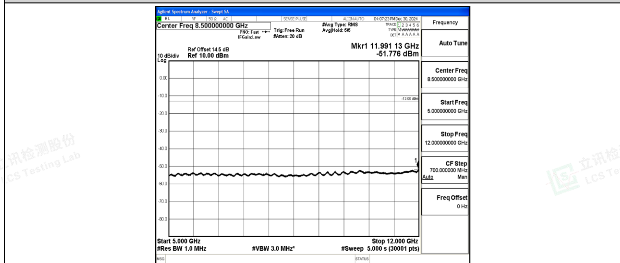
Band2-1.4MHz-16QAM-18607-1-0-Low-5000-12000--51.78-PASS
