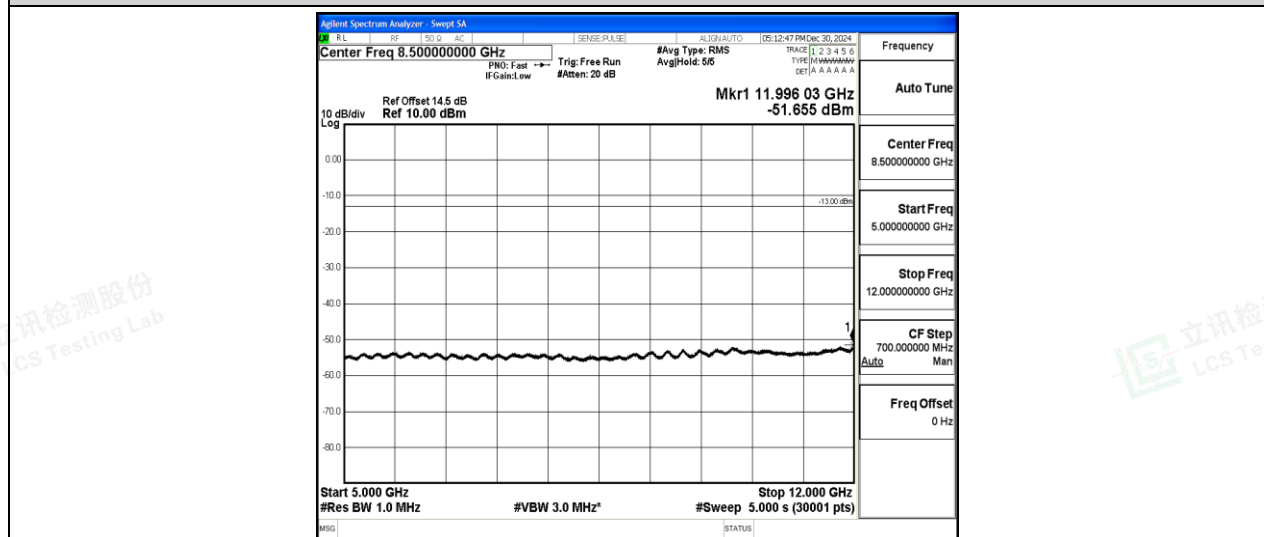
Band2-5MHz-16QAM-18625-1-0-Low-5000-12000--51.66-PASS
