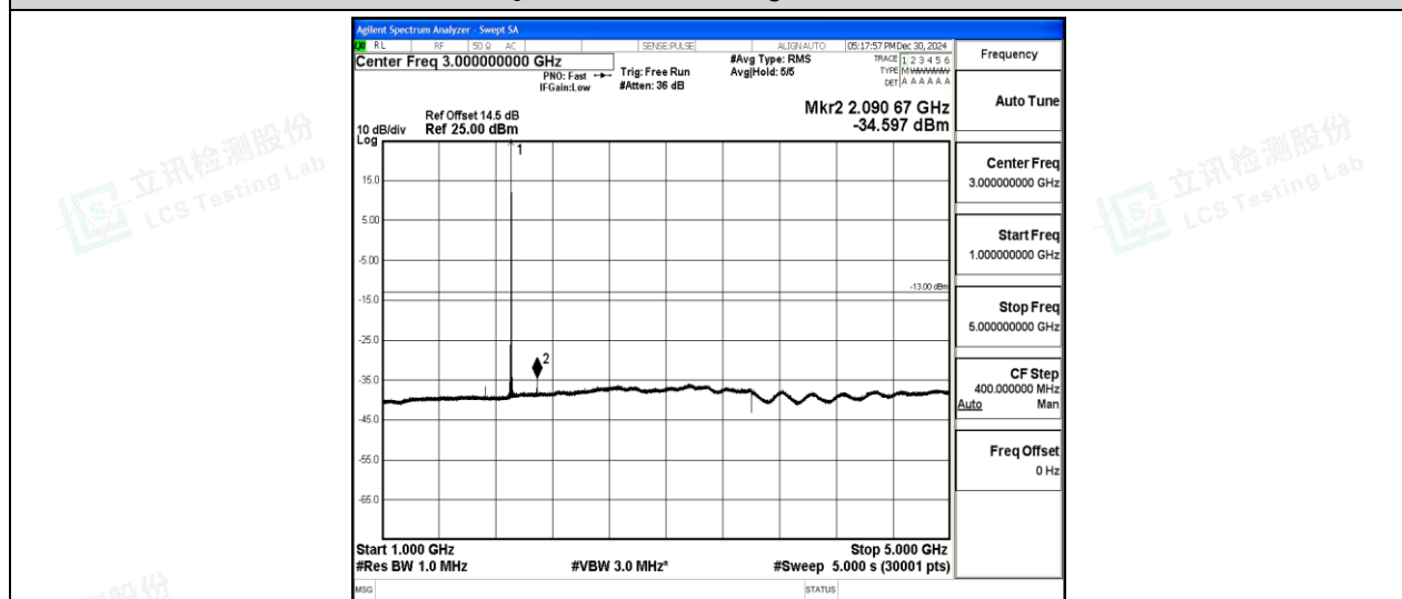
Band2-5MHz-QPSK-19175-1-0-High-1000-5000--34.6-PASS
