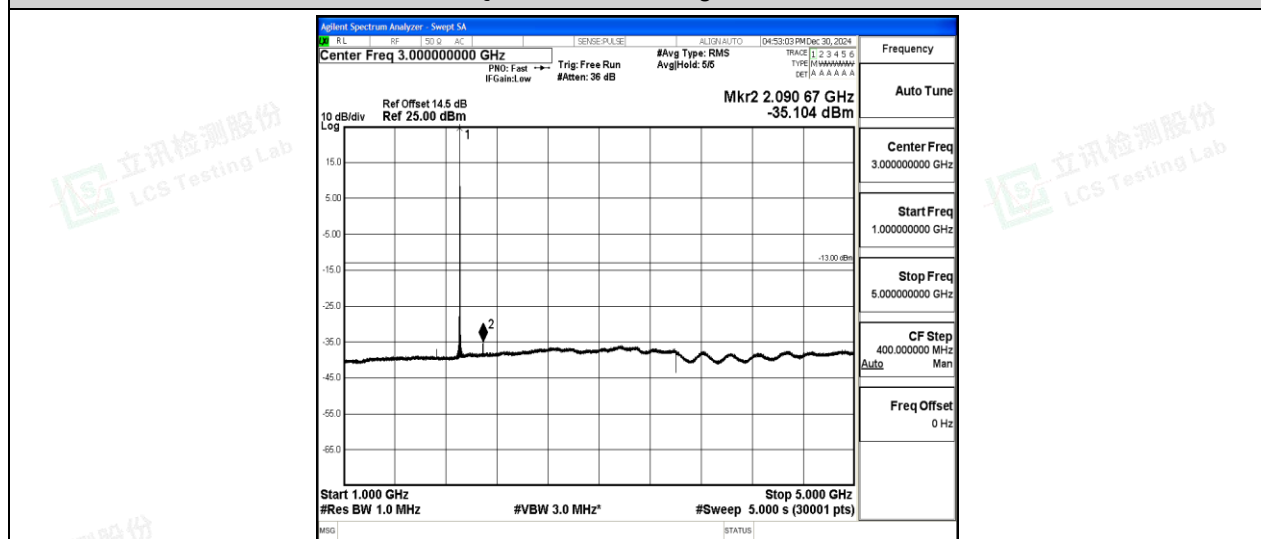
Band2-3MHz-16QAM-19185-1-0-High-1000-5000--35.1-PASS
