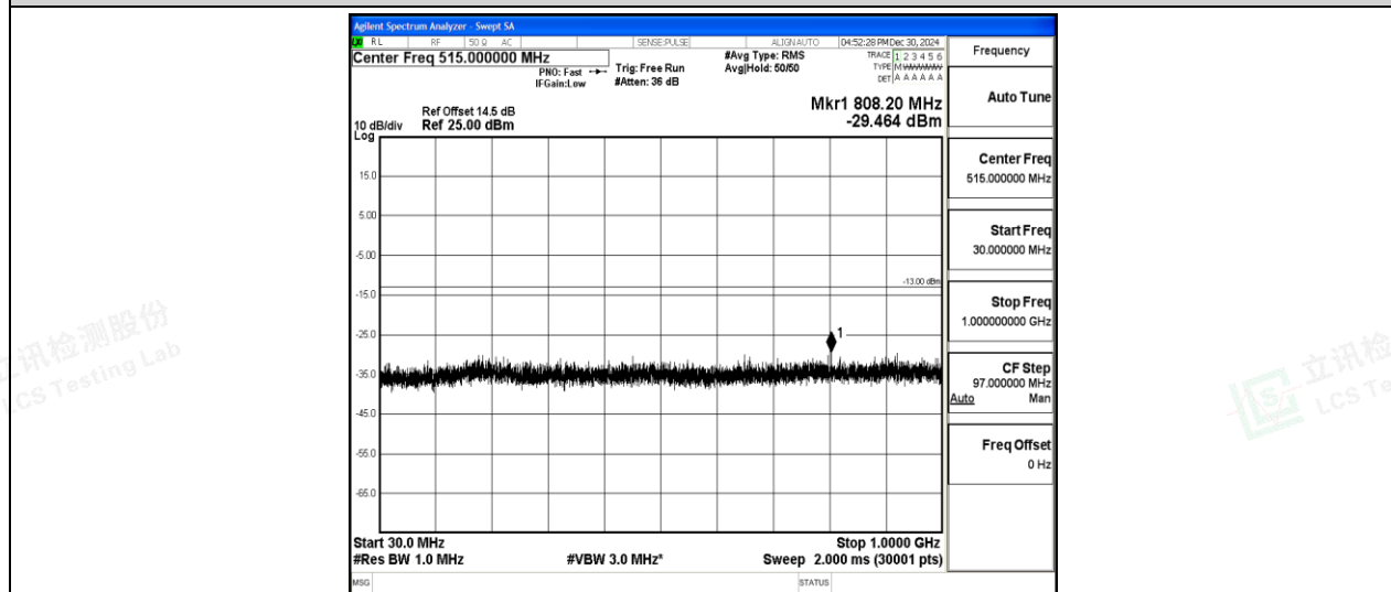
Band2-3MHz-16QAM-19185-1-0-High-30-1000--29.46-PASS
