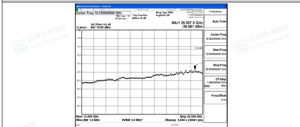
Band2-1.4MHz-16QAM-18607-1-0-Low-12000-26500--36.68-PASS
