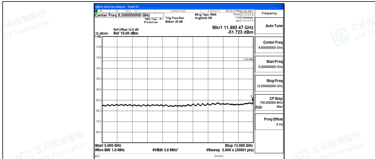
Band2-1.4MHz-QPSK-19193-1-0-High-5000-12000--51.72-PASS
