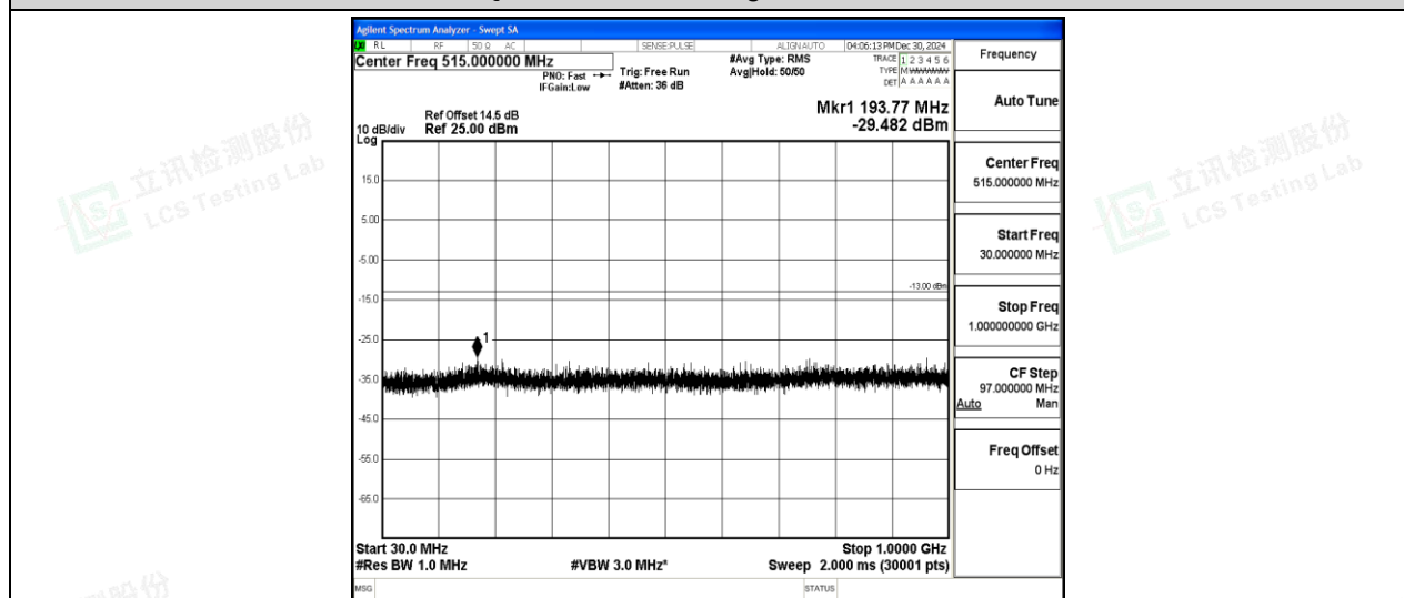
Band2-1.4MHz-16QAM-18607-1-0-Low-30-1000--29.48-PASS
