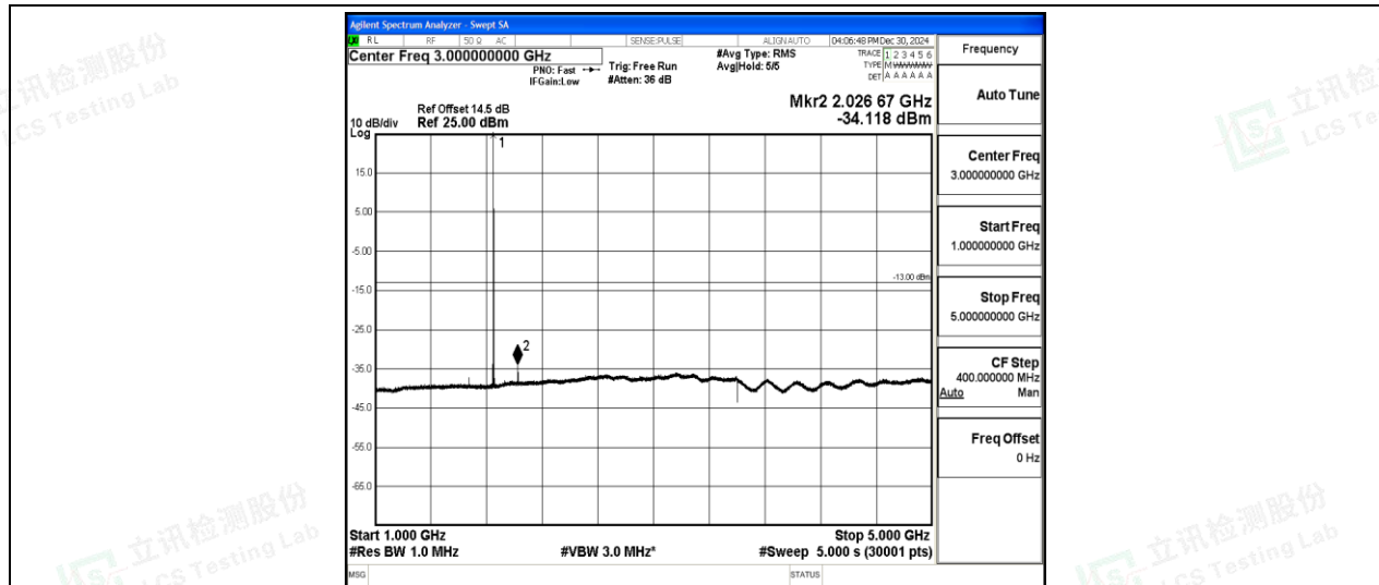
Band2-1.4MHz-16QAM-18607-1-0-Low-1000-5000--34.12-PASS
