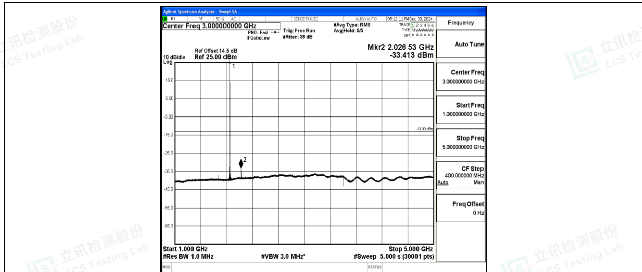
Band2-5MHz-16QAM-18625-1-0-Low-1000-5000--33.41-PASS
