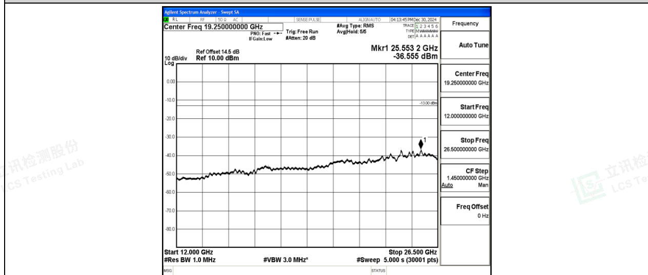
Band2-1.4MHz-QPSK-19193-1-0-High-12000-26500--36.56-PASS
