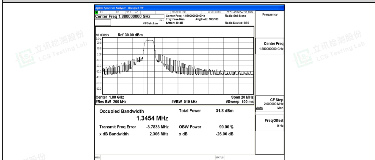
Band2-10MHz-16QAM-18900-6-0-Low-1.3454-2.306-PASS
