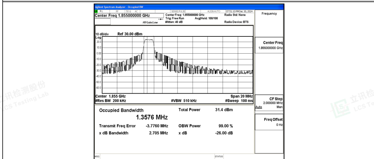
Band2-10MHz-16QAM-18650-6-0-Low-1.3576-2.705-PASS
