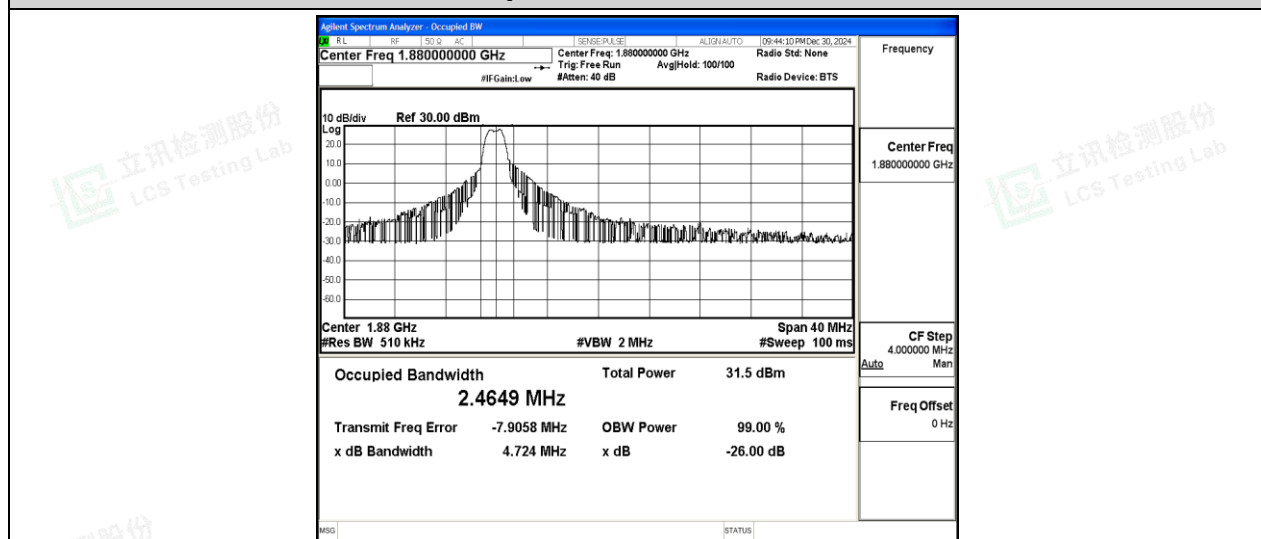
Band2-20MHz-16QAM-18900-6-0-Low-2.4649-4.724-PASS
