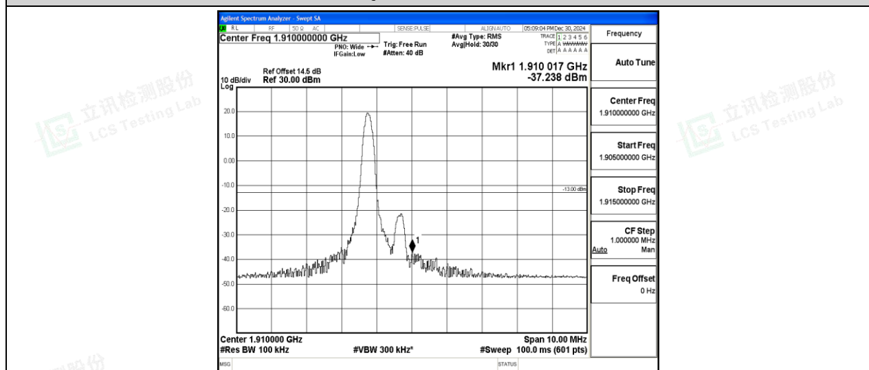
Band2-5MHz-16QAM-19175-1-0-High-37.24-PASS
