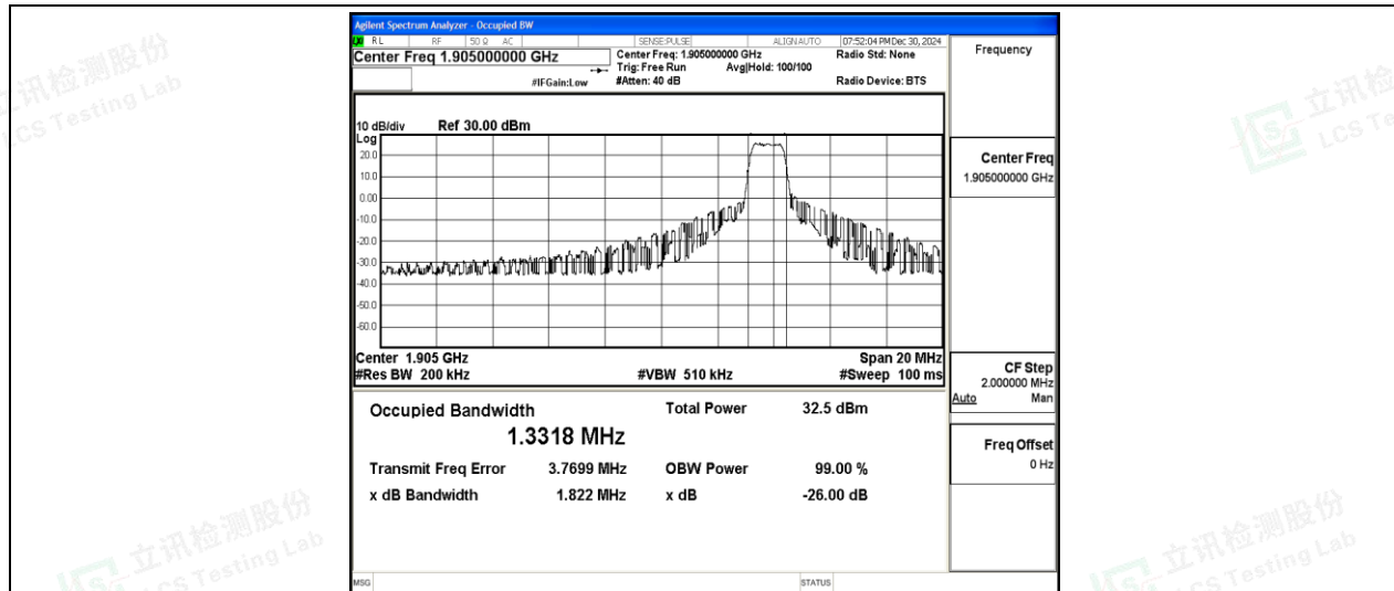
Band2-10MHz-QPSK-19150-6-0-High-1.3318-1.822-PASS
