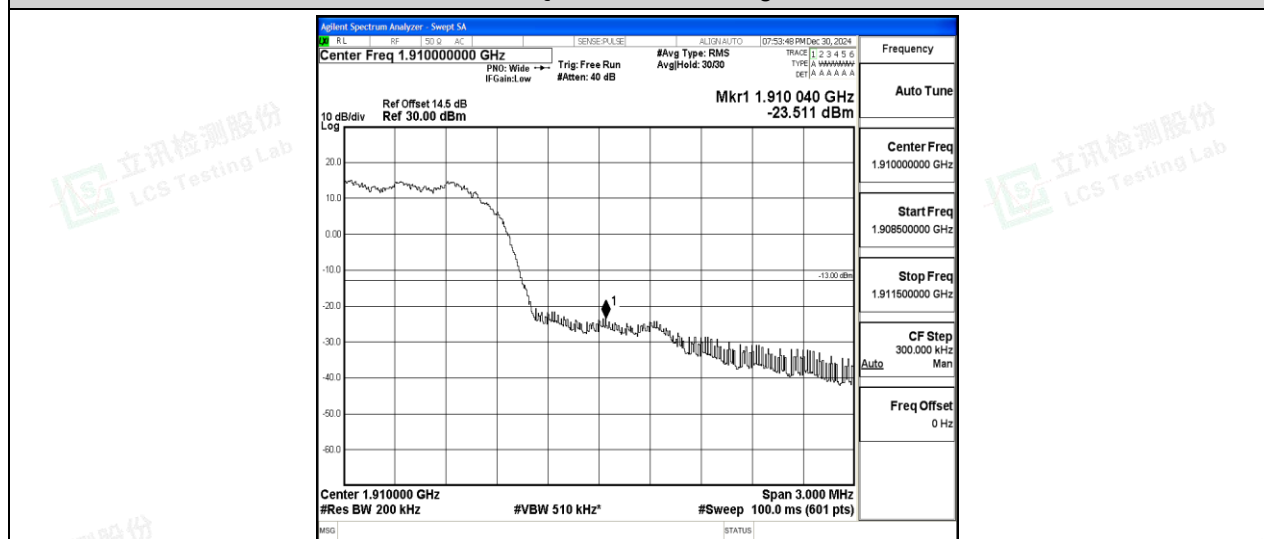
Band2-10MHz-16QAM-19150-6-0-High--23.51-PASS
