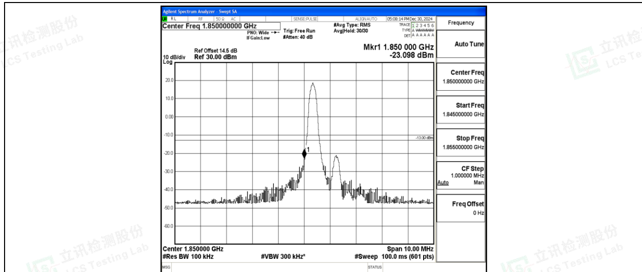
Band2-5MHz-16QAM-18625-1-0-Low-23.10-PASS
