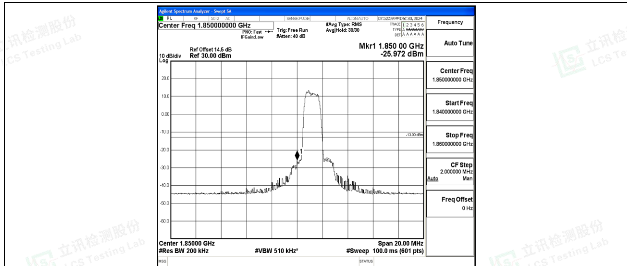
Band2-10MHz-16QAM-18650-6-0-Low--25.97-PASS
