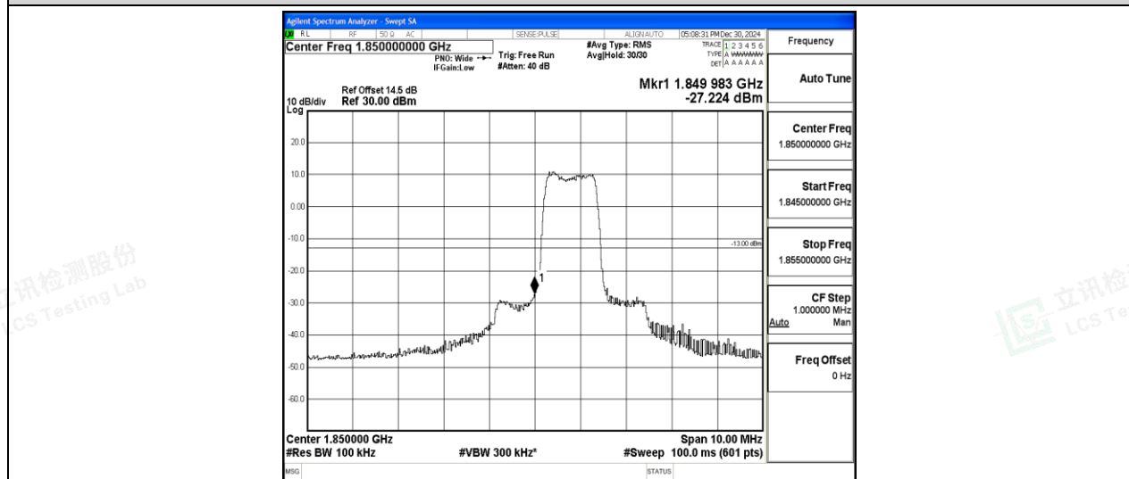
Band2-5MHz-16QAM-18625-6-0-Low-27.22-PASS
