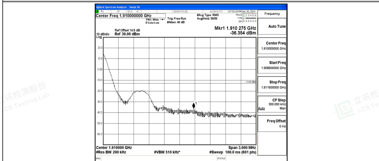
Band2-10MHz-16QAM-19150-1-0-High--36.35-PASS
