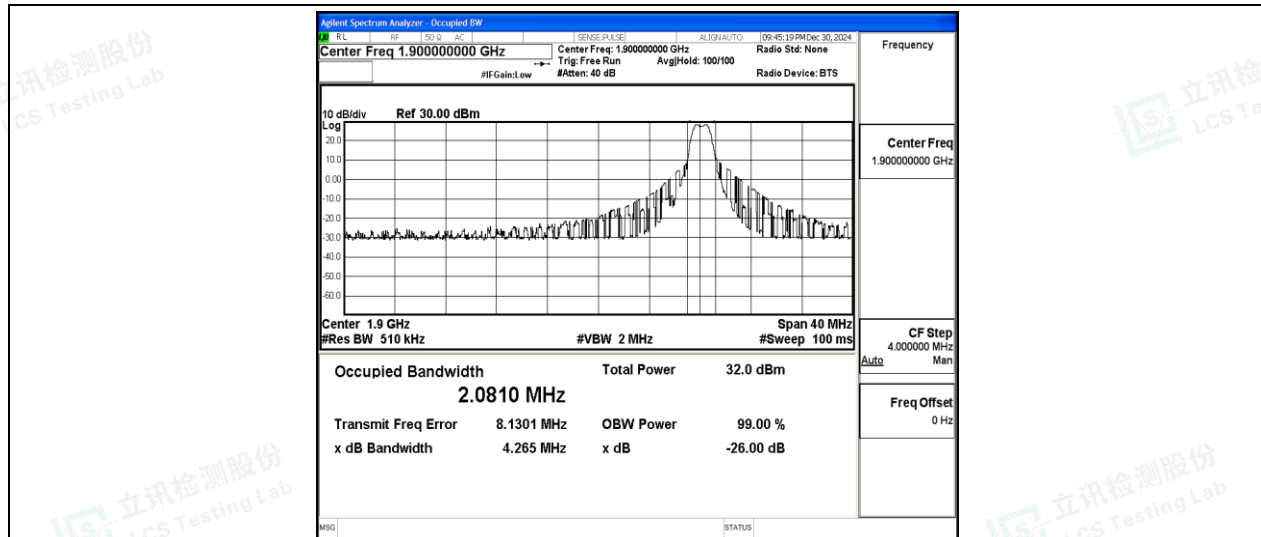
Band2-20MHz-QPSK-19100-6-0-High-2.0810-4.265-PASS
