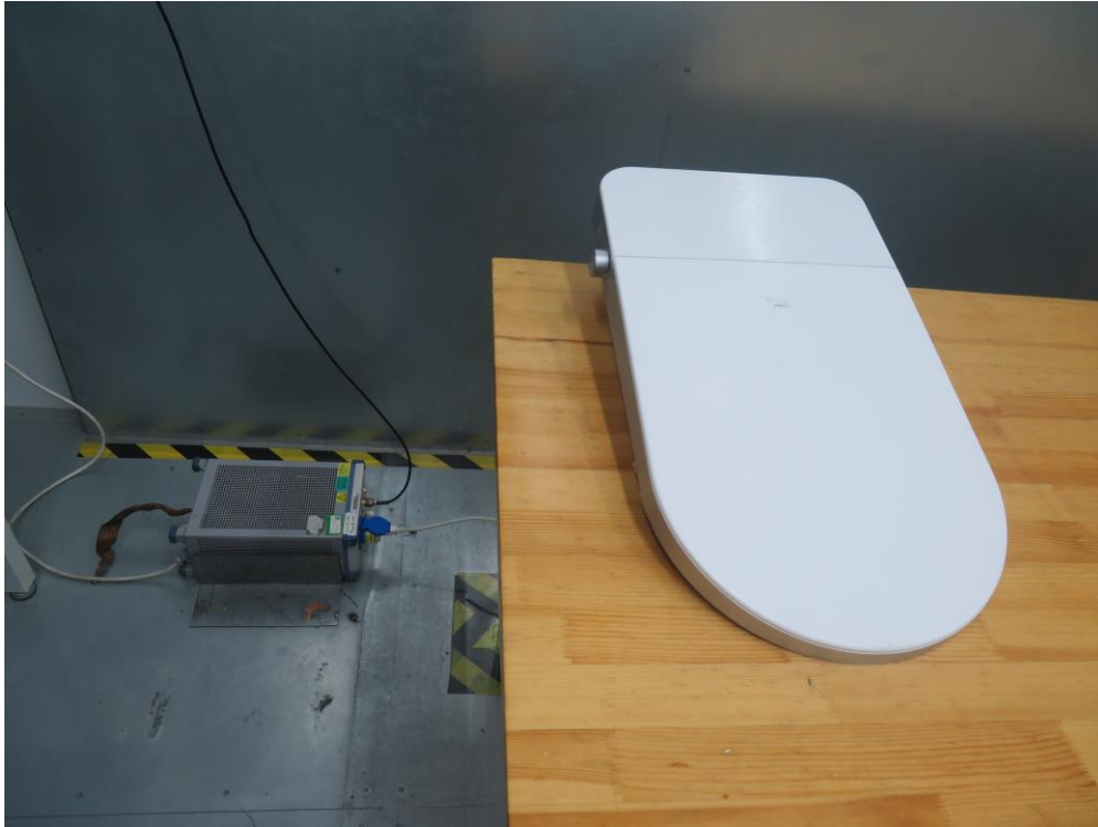
Description: Back View of Conducted Emission Test Setup for Power Port (For Radar)
