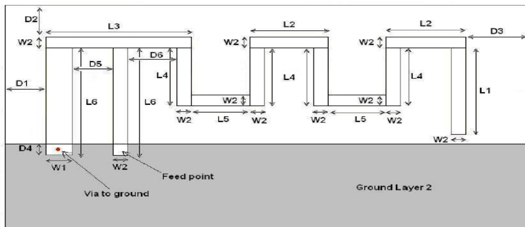
Figure 3: Antenna Dimensions
