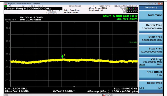
Band26(824-849)-15MHz-QPSK-26965-1RB#0-3000~100 00-PASS
