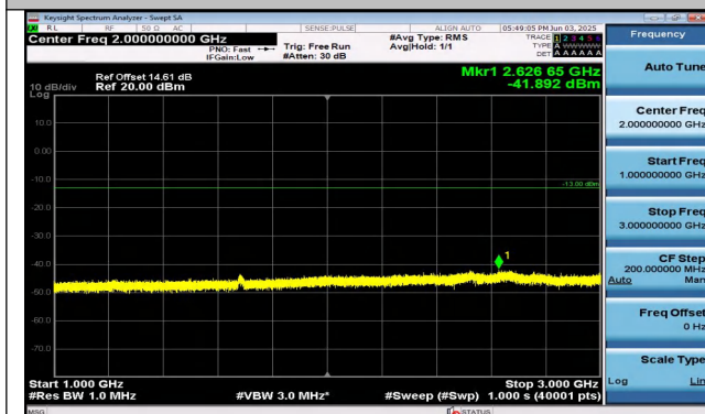
Band26(824-849)-15MHz-QPSK-26965-75RB#0-1000~3000-PASS
