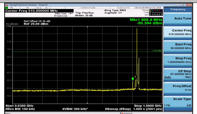
Band26(824-849)-15MHz-QPSK-26965-1RB#0-30~1000-P ASS
