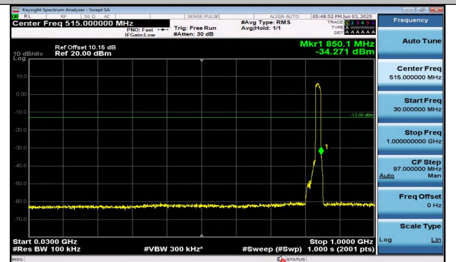
Band26(824-849)-15MHz-QPSK-26965-75RB#0-30~1000-PASS
