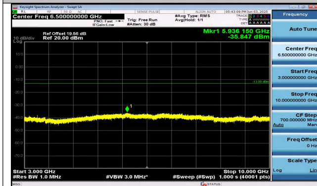
Band26(824-849)-15MHz-16QAM-26915-1RB#74-3000~1 0000-PASS
