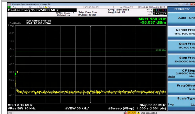
Band26(824-849)-15MHz-QPSK-26965-75RB#0-0.15~30-PASS
