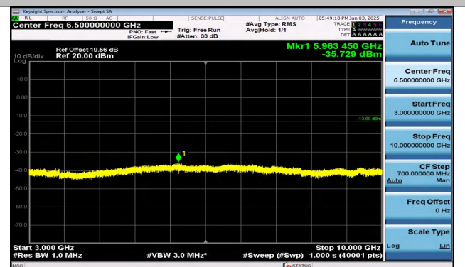
Band26(824-849)-15MHz-QPSK-26965-75RB#0-3000~10000-PASS
