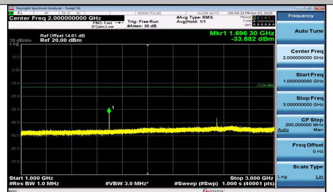
Band26(824-849)-15MHz-QPSK-26965-1RB#74-1000~30 00-PASS
