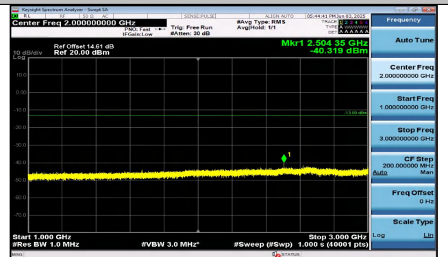
Band26(824-849)-15MHz-16QAM-26965-1RB#0-1000~3000- 00-PASS
