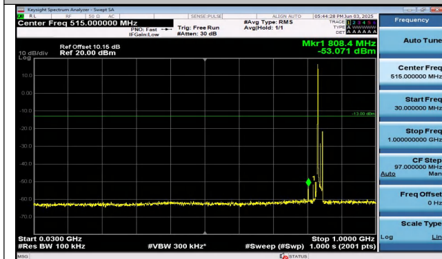
Band26(824-849)-15MHz-16QAM-26965-1RB#0-30~1000- PASS
