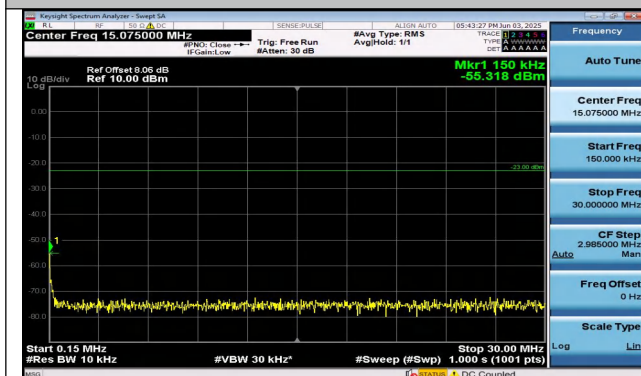
Band26(824-849)-15MHz-QPSK-26965-1RB#0-0.15~30-P ASS
