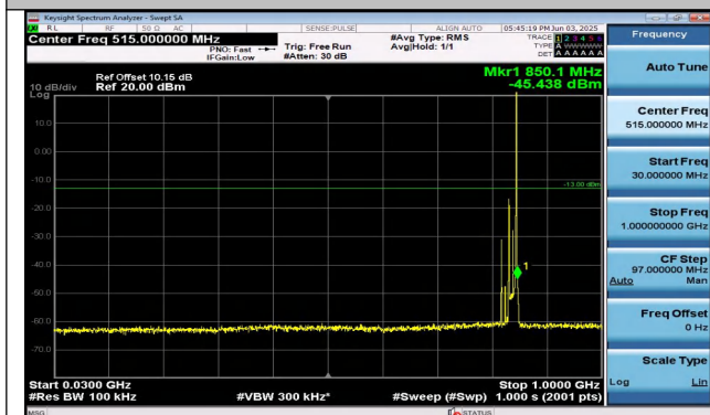
Band26(824-849)-15MHz-QPSK-26965-1RB#74-30~1000- PASS
