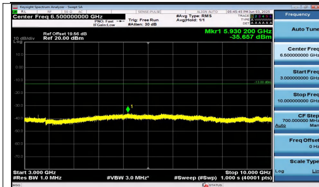
Band26(824-849)-15MHz-QPSK-26965-1RB#74-3000~10000-PASS
