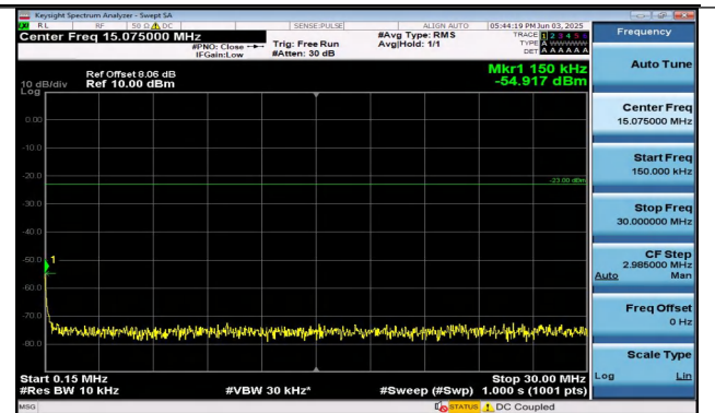
Band26(824-849)-15MHz-16QAM-26965-1RB#0-0.15~30- PASS
