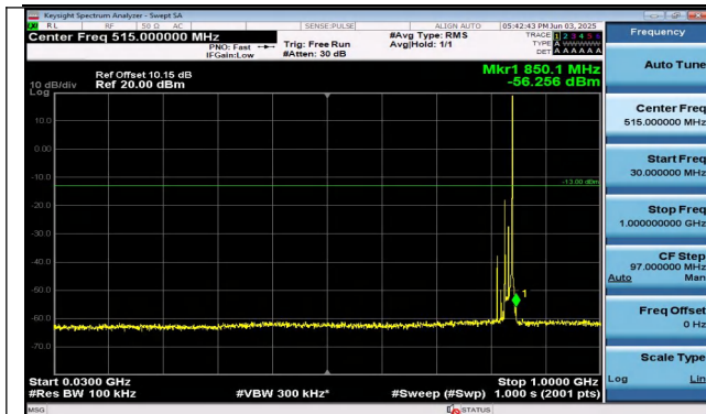
Band26(824-849)-15MHz-16QAM-26915-1RB#74-30~100 0-PASS
