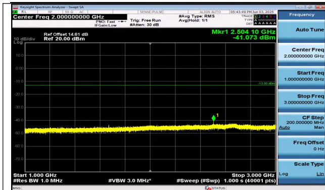
Band26(824-849)-15MHz-QPSK-26965-1RB#0-1000~300 0-PASS
