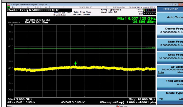
Band26(824-849)-15MHz-16QAM-26965-1RB#0-3000~10000- 000-PASS
