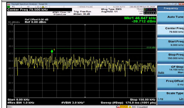
Band26(824-849)-15MHz-QPSK-26965-1RB#74-0.009~0. 15-PASS
