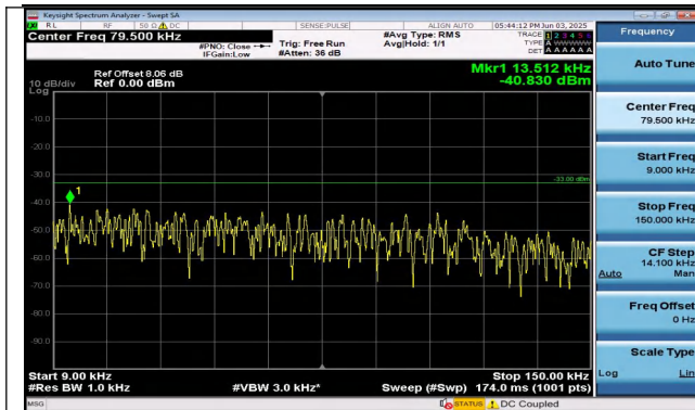
Band26(824-849)-15MHz-16QAM-26965-1RB#0-0.009~0. 15-PASS
