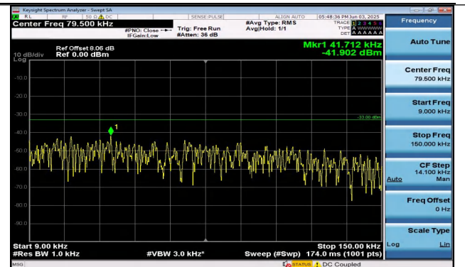
Band26(824-849)-15MHz-QPSK-26965-75RB#0-0.009~0.15-PASS
