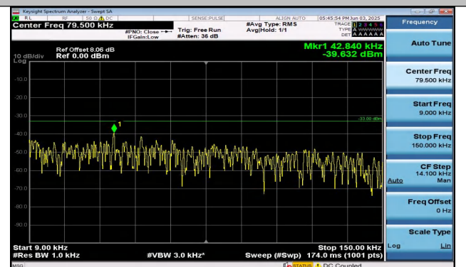
Band26(824-849)-15MHz-16QAM-26965-1RB#74-0.009~0.15- .15-PASS
