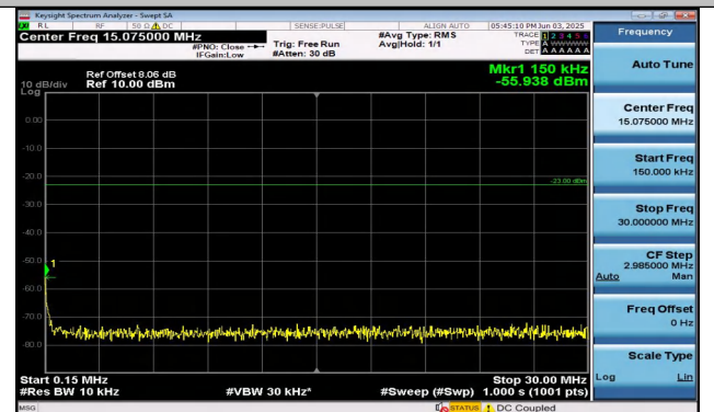
Band26(824-849)-15MHz-QPSK-26965-1RB#74-0.15~30- PASS
