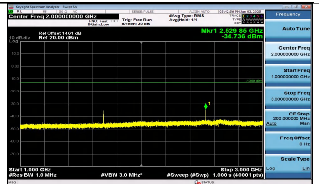
Band26(824-849)-15MHz-16QAM-26915-1RB#74-1000~3 000-PASS
