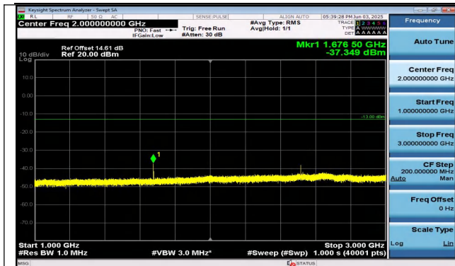
Band26(824-849)-15MHz-16QAM-26865-1RB#74-1000~3000-PASS
