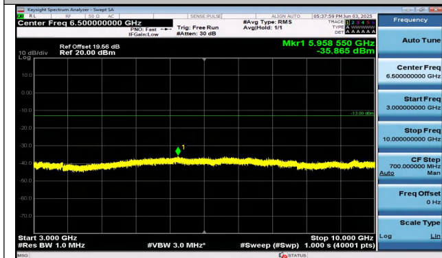
Band26(824-849)-15MHz-16QAM-26865-1RB#0-3000~10 000-PASS
