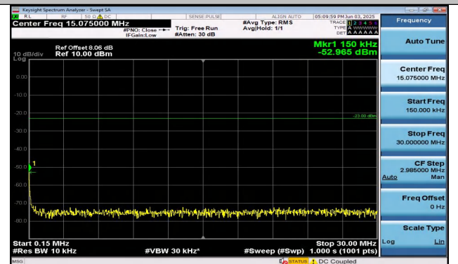
Band26(824-849)-10MHz-16QAM-26990-1RB#49-0.15~30 -PASS
