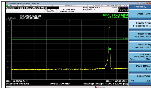
Band26(824-849)-10MHz-QPSK-26990-50RB#0-30~1000- PASS
