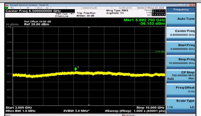
Band26(824-849)-15MHz-QPSK-26915-1RB#74-3000~10 000-PASS
