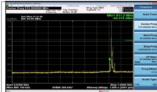
Band26(824-849)-15MHz-16QAM-26865-1RB#0-30~1000- PASS
