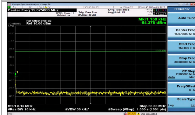
Band26(824-849)-15MHz-QPSK-26915-1RB#74-0.15~30- PASS
