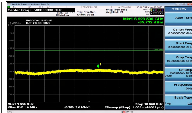
Band26(824-849)-10MHz-16QAM-26990-1RB#49-3000~1 0000-PASS
