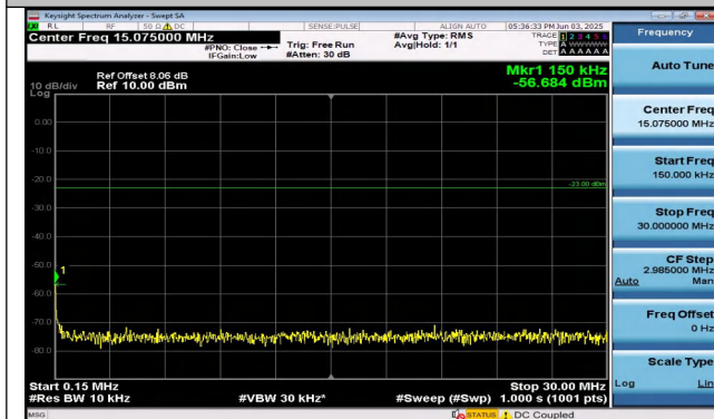
Band26(824-849)-15MHz-QPSK-26865-1RB#0-0.15~30-P ASS
