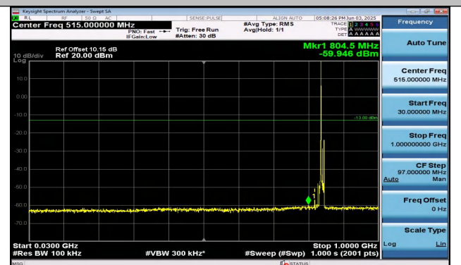
Band26(824-849)-10MHz-16QAM-26990-1RB#0-30~1000- PASS
