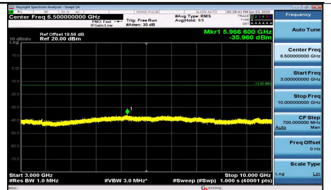
Band26(824-849)-15MHz-16QAM-26865-1RB#74-3000~10000-PASS
