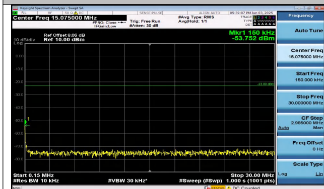
Band26(824-849)-15MHz-16QAM-26865-1RB#74-0.15~30 -PASS
