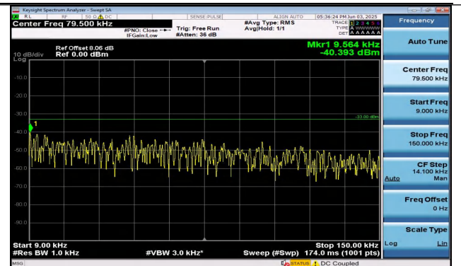
Band26(824-849)-15MHz-QPSK-26865-1RB#0-0.009~0.1 5-PASS
