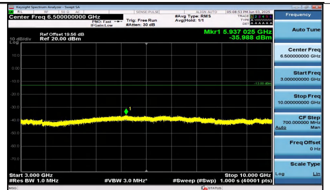
Band26(824-849)-10MHz-16QAM-26990-1RB#0-3000~10 000-PASS
