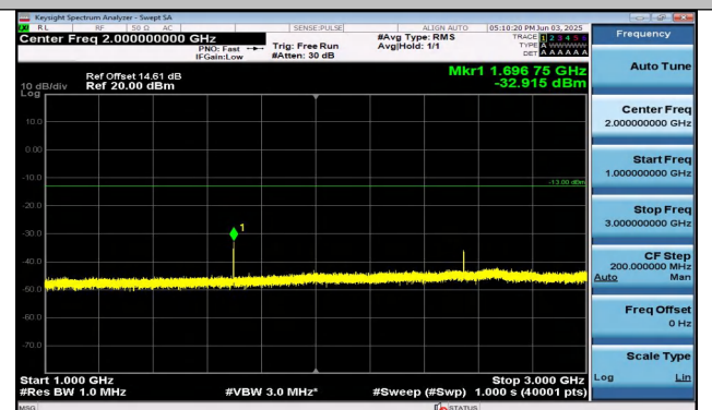
Band26(824-849)-10MHz-16QAM-26990-1RB#49-1000~3 000-PASS
