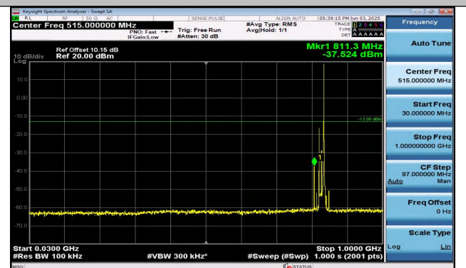
Band26(824-849)-15MHz-16QAM-26865-1RB#74-30~100 0-PASS
