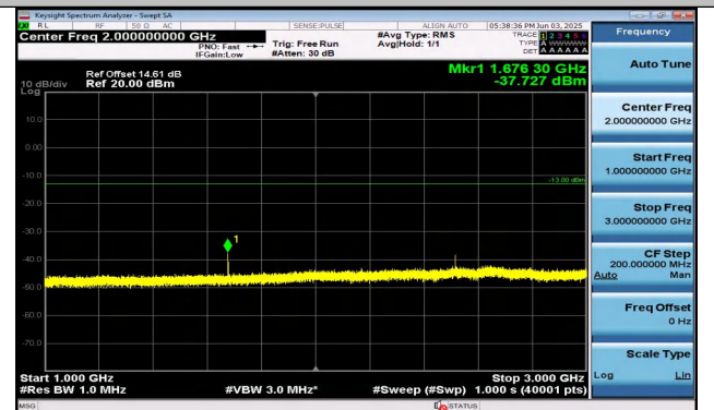
Band26(824-849)-15MHz-QPSK-26865-1RB#74-1000~30 00-PASS
