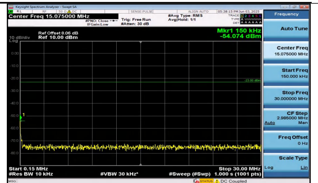
Band26(824-849)-15MHz-QPSK-26865-1RB#74-0.15~30- PASS
