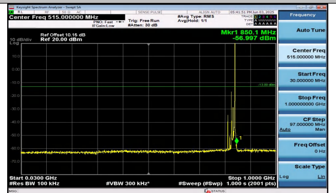
Band26(824-849)-15MHz-QPSK-26915-1RB#74-30~1000- PASS
