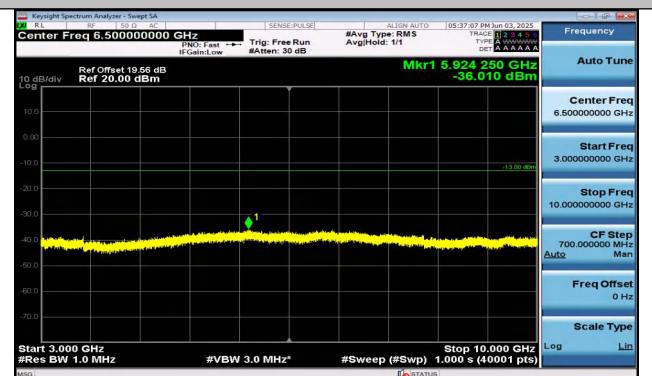
Band26(824-849)-15MHz-QPSK-26865-1RB#0-3000~100 00-PASS
