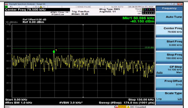
Band26(824-849)-15MHz-16QAM-26865-1RB#74-0.009~0 .15-PASS
