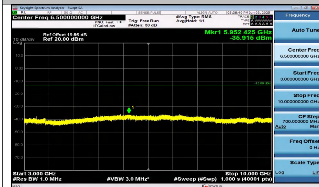
Band26(824-849)-15MHz-QPSK-26865-1RB#74-3000~10 000-PASS
