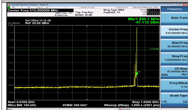
Band26(824-849)-10MHz-16QAM-26990-1RB#49-30~100 0-PASS
