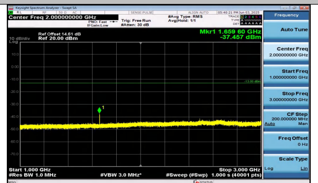
Band26(824-849)-15MHz-QPSK-26915-1RB#0-1000~3000-PASS
