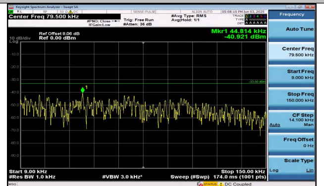
Band26(824-849)-10MHz-16QAM-26990-1RB#0-0.009~0. 15-PASS
