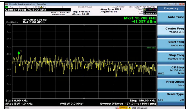
Band26(824-849)-15MHz-QPSK-26915-1RB#74-0.009~0. 15-PASS
