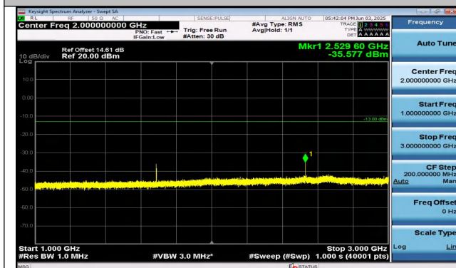
Band26(824-849)-15MHz-QPSK-26915-1RB#74-1000~30 00-PASS
