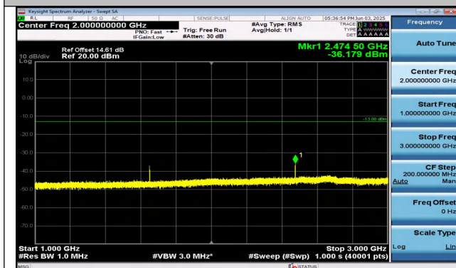
Band26(824-849)-15MHz-QPSK-26865-1RB#0-1000~300 0-PASS
