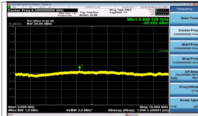
Band26(824-849)-15MHz-QPSK-26915-1RB#0-3000~100 00-PASS
