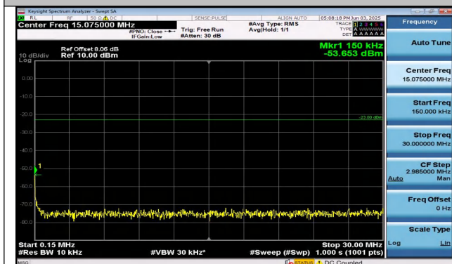
Band26(824-849)-10MHz-16QAM-26990-1RB#0-0.15~30- PASS
