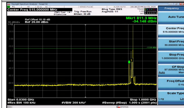
Band26(824-849)-15MHz-QPSK-26865-1RB#74-30~1000- PASS
