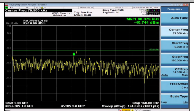
Band26(824-849)-15MHz-QPSK-26865-75RB#0-0.009~0. 15-PASS
