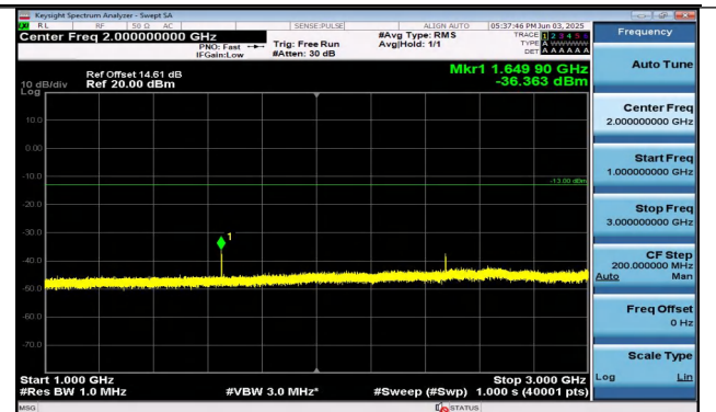
Band26(824-849)-15MHz-16QAM-26865-1RB#0-1000~30 00-PASS
