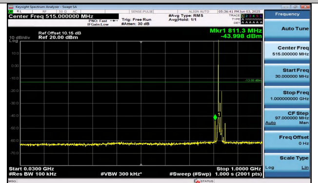
Band26(824-849)-15MHz-QPSK-26865-1RB#0-30~1000-P ASS
