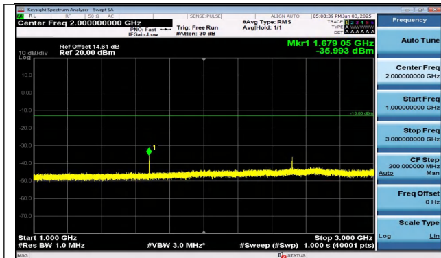
Band26(824-849)-10MHz-16QAM-26990-1RB#0-1000~30 00-PASS
