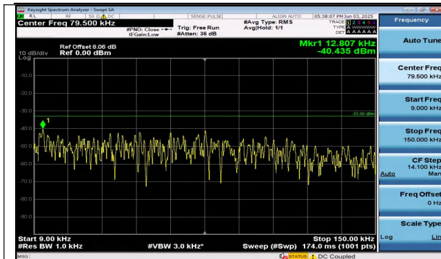
Band26(824-849)-15MHz-QPSK-26865-1RB#74-0.009~0. 15-PASS
