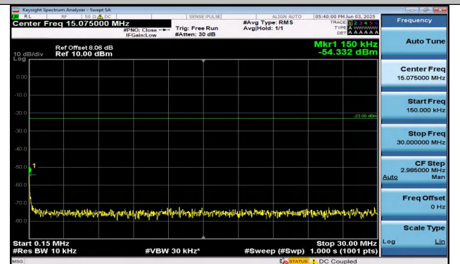
Band26(824-849)-15MHz-QPSK-26915-1RB#0-0.15~30-PASS
