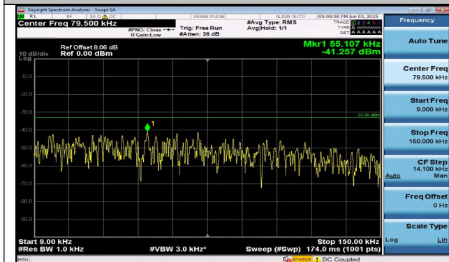
Band26(824-849)-10MHz-16QAM-26990-1RB#49-0.009~0 .15-PASS
