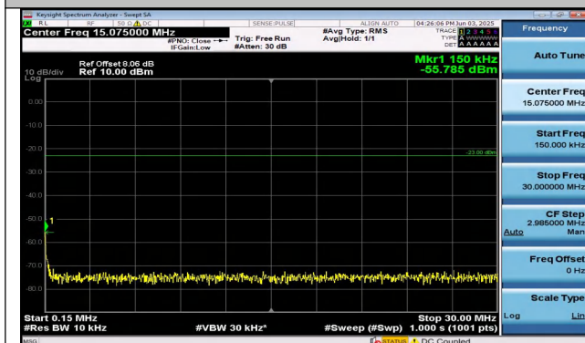
Band26(824-849)-5MHz-QPSK-27015-1RB#24-0.15~30-P
