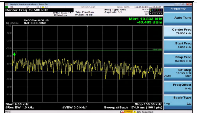
Band26(824-849)-5MHz-16QAM-27015-1RB#0-0.009~0.1 5-PASS
