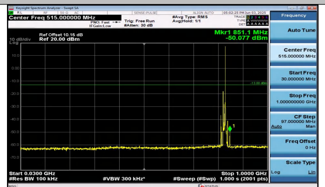
Band26(824-849)-10MHz-QPSK-26840-1RB#49-30~1000- PASS
