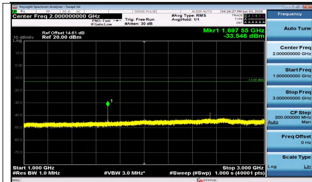
Band26(824-849)-5MHz-QPSK-27015-1RB#24-1000~300 0-PASS
