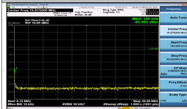
Band26(824-849)-10MHz-QPSK-26840-1RB#49-0.15~30- PASS
