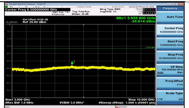
Band26(824-849)-10MHz-QPSK-26840-1RB#49-3000~10000-PASS
