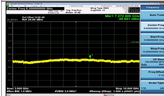
Band26(824-849)-5MHz-QPSK-27015-1RB#0-3000~1000
