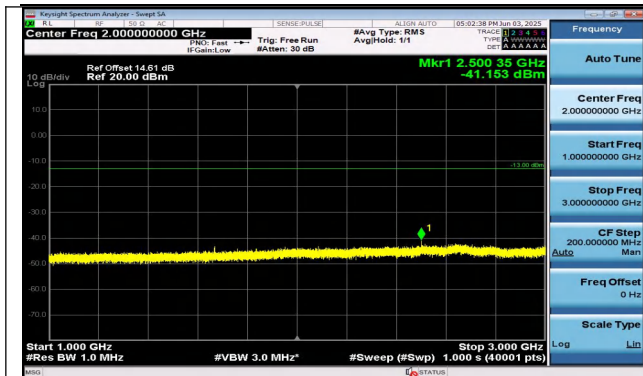
Band26(824-849)-10MHz-QPSK-26840-1RB#49-1000~3000-PASS
