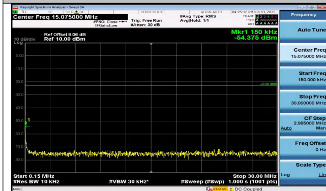
Band26(824-849)-5MHz-16QAM-27015-1RB#0-0.15~30-P ASS
