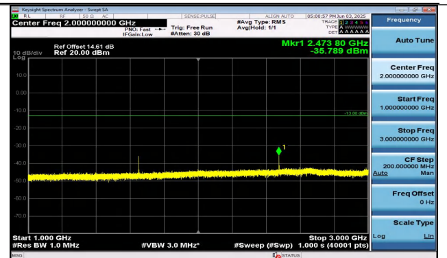
Band26(824-849)-10MHz-QPSK-26840-1RB#0-1000~300 0-PASS
