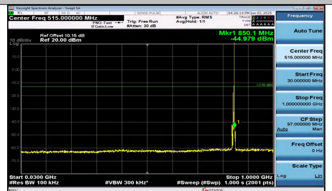
Band26(824-849)-5MHz-QPSK-27015-1RB#24-30~1000-P
