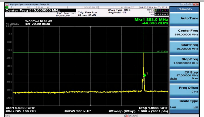
Band26(824-849)-5MHz-16QAM-27015-1RB#0-30~1000-P ASS
