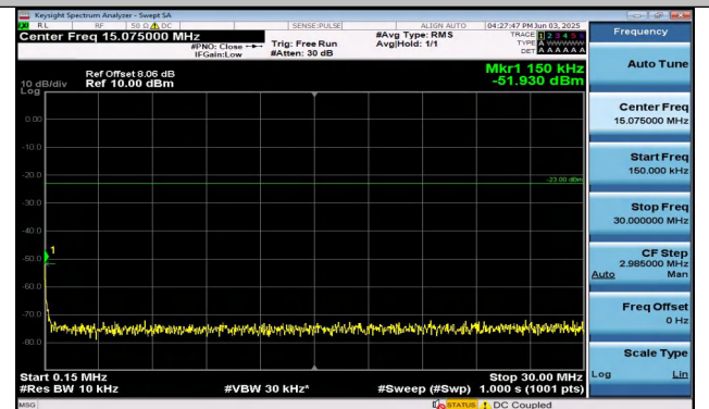
Band26(824-849)-5MHz-QPSK-27015-25RB#0-0.15~30-P ASS
