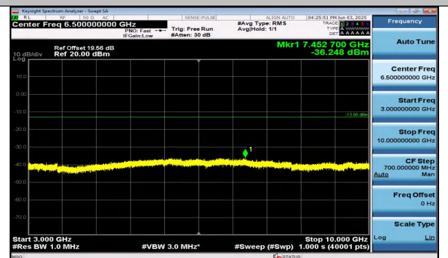
Band26(824-849)-5MHz-16QAM-27015-1RB#0-3000~100 00-PASS
