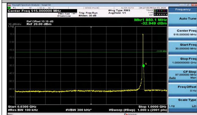
Band26(824-849)-5MHz-QPSK-27015-25RB#0-30~1000-P ASS
