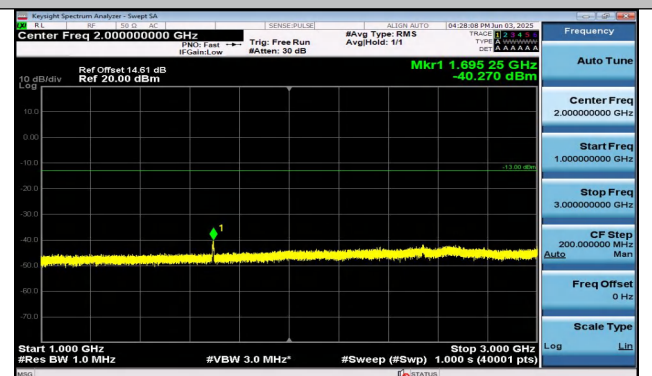
Band26(824-849)-5MHz-QPSK-27015-25RB#0-1000~300 0-PASS
