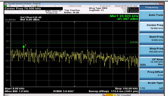
Band26(824-849)-10MHz-QPSK-26840-1RB#49-0.009~0. 15-PASS
