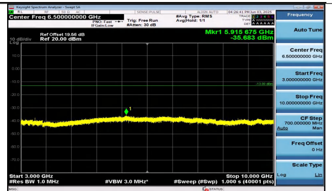
Band26(824-849)-5MHz-QPSK-27015-1RB#24-3000~100 00-PASS
