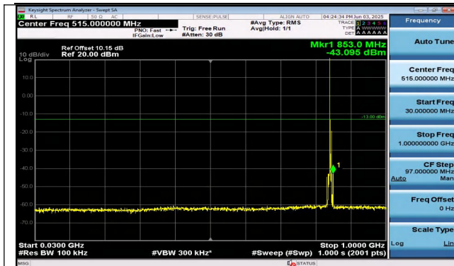
Band26(824-849)-5MHz-QPSK-27015-1RB#0-30~1000-P
