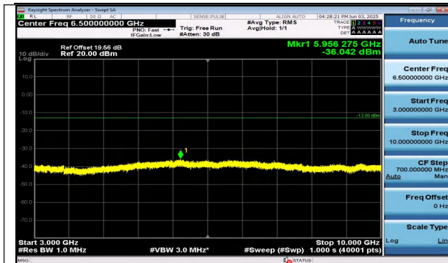
Band26(824-849)-5MHz-QPSK-27015-25RB#0-3000~100 00-PASS
