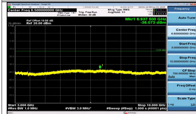
Band26(824-849)-10MHz-QPSK-26840-1RB#0-3000~100 00-PASS
