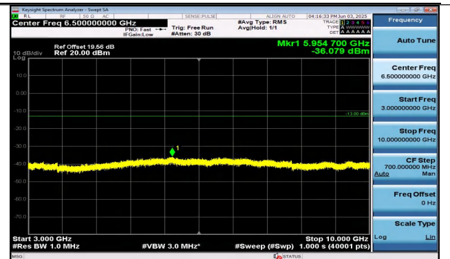
Band26(824-849)-5MHz-QPSK-26815-1RB#24-3000~100 00-PASS
