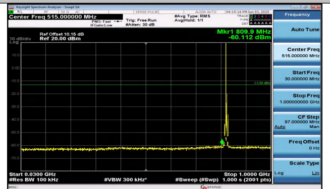
Band26(824-849)-5MHz-16QAM-26815-1RB#0-30~1000-P ASS
