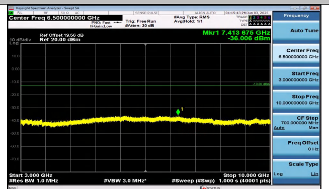
Band26(824-849)-5MHz-16QAM-26815-1RB#0-3000~100 00-PASS
