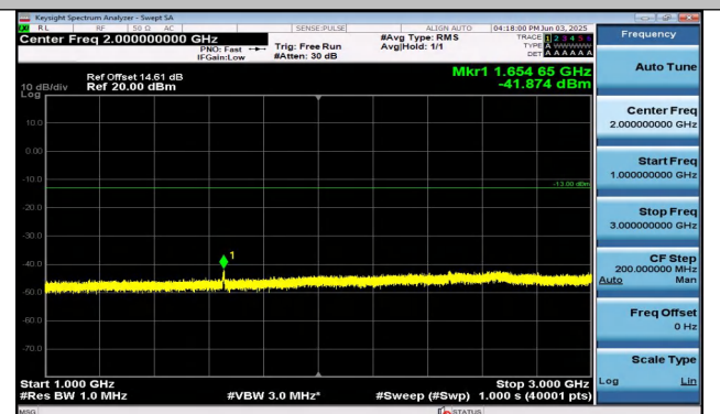
Band26(824-849)-5MHz-QPSK-26815-25RB#0-1000~300 0-PASS
