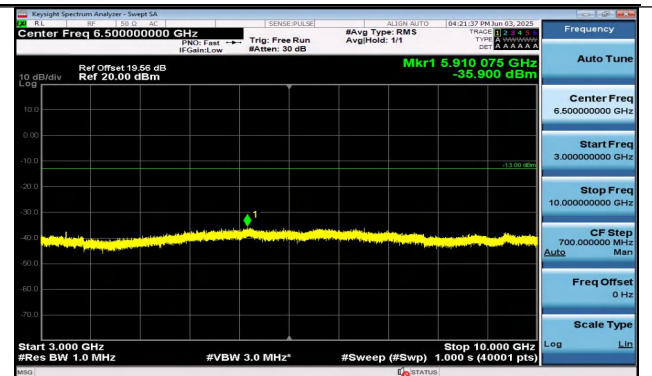
Band26(824-849)-5MHz-QPSK-26915-1RB#24-3000~100 00-PASS
