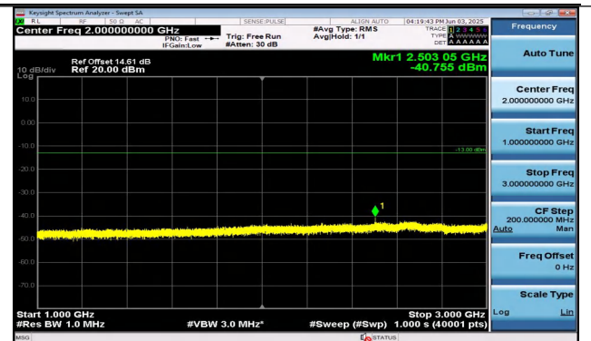
Band26(824-849)-5MHz-QPSK-26915-1RB#0-1000~3000-P PASS
