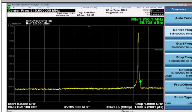
Band26(824-849)-5MHz-QPSK-26915-25RB#0-30~1000-P ASS
