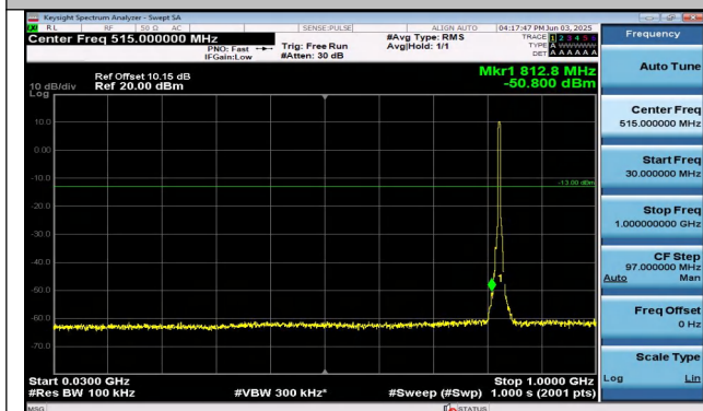
Band26(824-849)-5MHz-QPSK-26815-25RB#0-30~1000-P ASS
