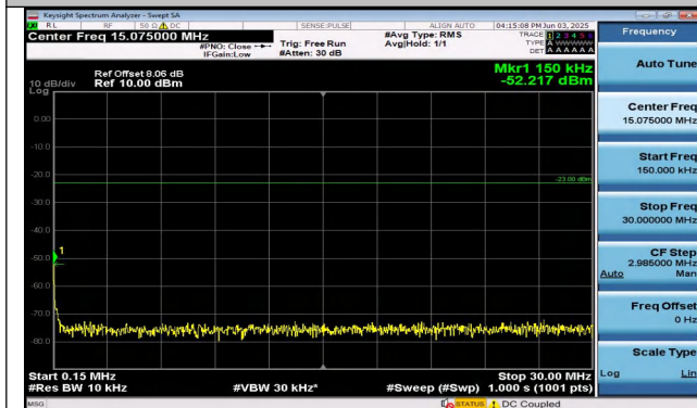
Band26(824-849)-5MHz-16QAM-26815-1RB#0-0.15~30-P ASS
