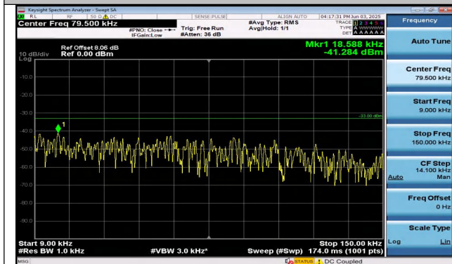
Band26(824-849)-5MHz-QPSK-26815-25RB#0-0.009~0.1 5-PASS
