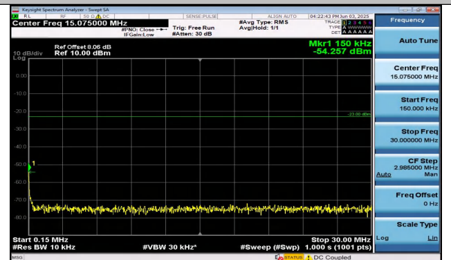
Band26(824-849)-5MHz-QPSK-26915-25RB#0-0.15~30-P ASS
