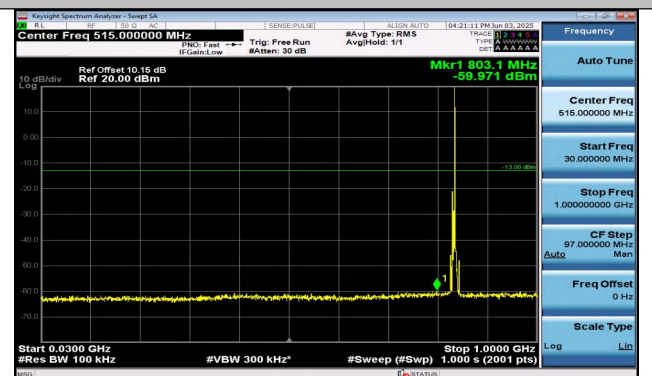
Band26(824-849)-5MHz-QPSK-26915-1RB#24-30~1000-P ASS
