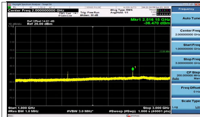
Band26(824-849)-5MHz-QPSK-26915-1RB#24-1000~300 0-PASS
