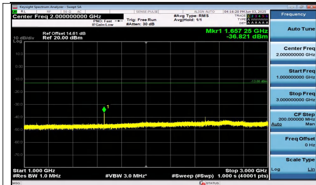
Band26(824-849)-5MHz-QPSK-26815-1RB#24-1000~300 0-PASS
