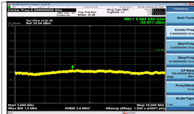
Band26(824-849)-5MHz-QPSK-26815-25RB#0-3000~100 00-PASS
