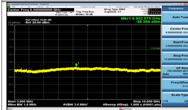
Band26(824-849)-5MHz-QPSK-26915-1RB#0-3000~1000 0-PASS
