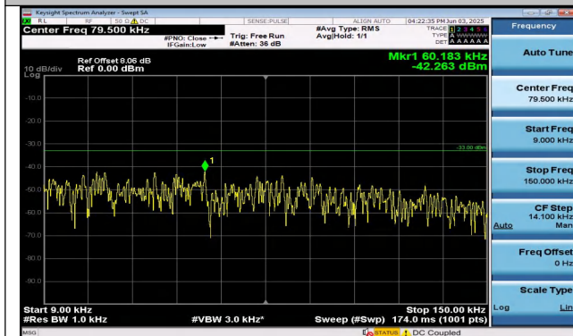
Band26(824-849)-5MHz-QPSK-26915-25RB#0-0.009~0.1 5-PASS
