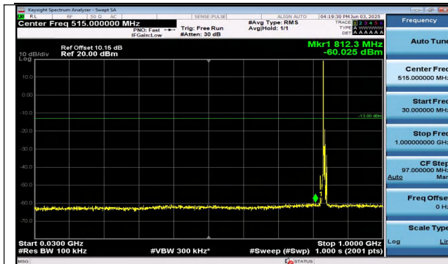
Band26(824-849)-5MHz-QPSK-26915-1RB#0-30~1000-P ASS
