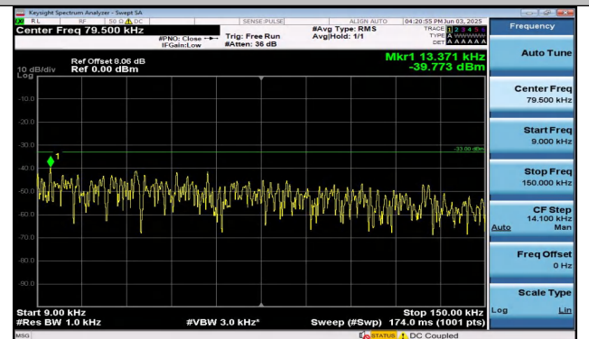
Band26(824-849)-5MHz-QPSK-26915-1RB#24-0.009~0.1 5-PASS
