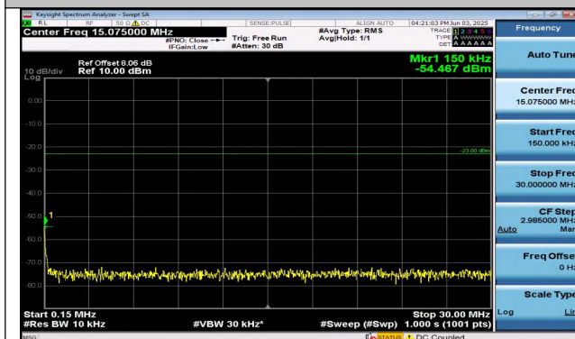
Band26(824-849)-5MHz-QPSK-26915-1RB#24-0.15~30-P ASS
