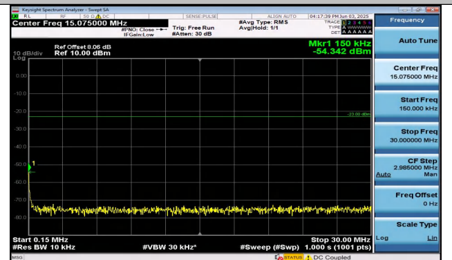
Band26(824-849)-5MHz-QPSK-26815-25RB#0-0.15~30-P ASS
