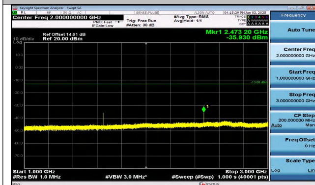
Band26(824-849)-5MHz-16QAM-26815-1RB#0-1000~300 0-PASS
