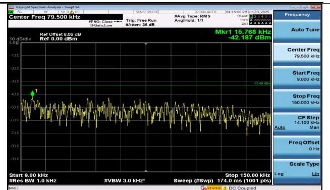
Band26(824-849)-5MHz-16QAM-26815-1RB#0-0.009~0.1 5-PASS
