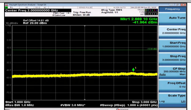
Band26(824-849)-5MHz-QPSK-26915-25RB#0-1000~300 0-PASS
