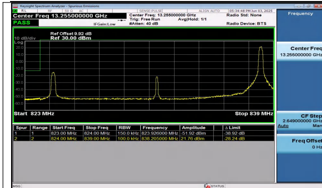
Band26(824-849)-15MHz-16QAM-26865-1RB#74-PASS
