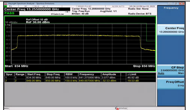
Band26(824-849)-15MHz-QPSK-26965-75RB#0-PASS
