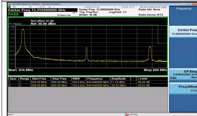
Band26(824-849)-15MHz-16QAM-26965-1RB#0-PASS
