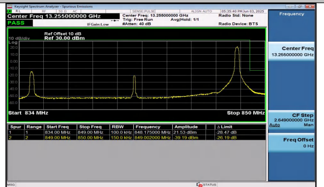
Band26(824-849)-15MHz-16QAM-26965-1RB#74-PASS
