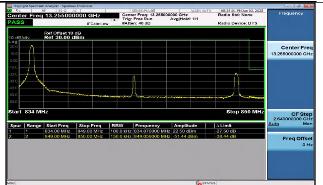
Band26(824-849)-15MHz-QPSK-26965-1RB#0-PASS
