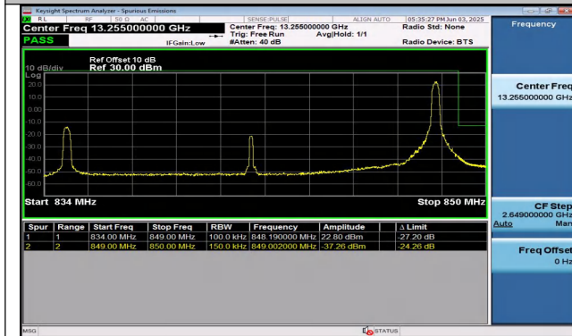
Band26(824-849)-15MHz-QPSK-26965-1RB#74-PASS
