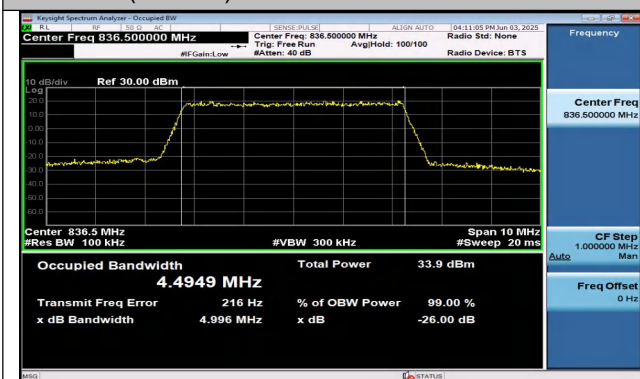
Band26(824-849)-5MHz-QPSK-26915-25RB#0-PASS
