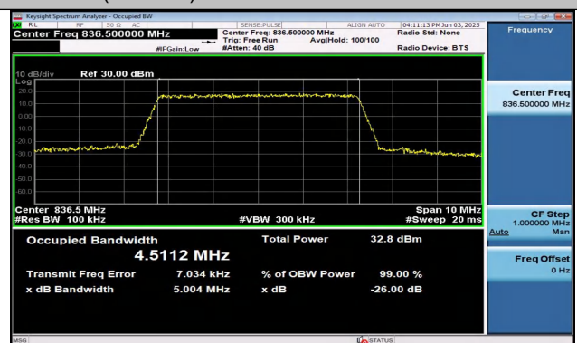
Band26(824-849)-5MHz-16QAM-26915-25RB#0-PASS
