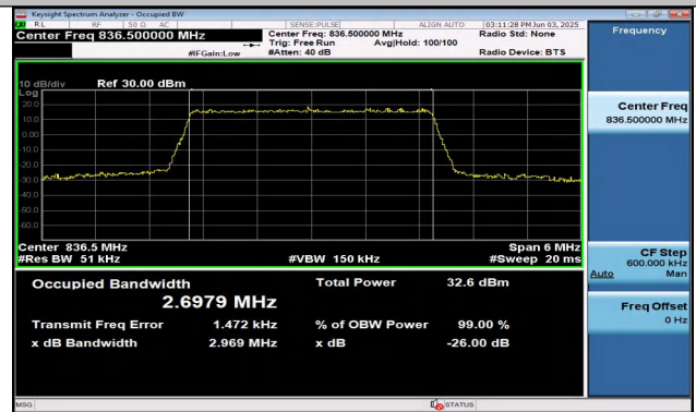
Band26(824-849)-3MHz-16QAM-26915-15RB#0-PASS
