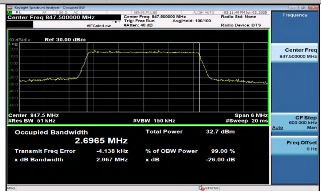
Band26(824-849)-3MHz-16QAM-27025-15RB#0-PASS
