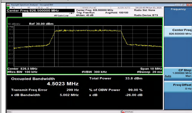
Band26(824-849)-5MHz-QPSK-26815-25RB#0-PASS
