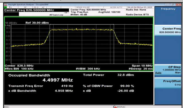
Band26(824-849)-5MHz-16QAM-26815-25RB#0-PASS
