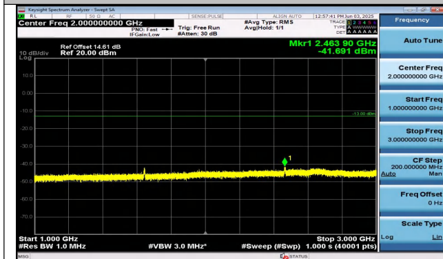
Band26(814-824)-5MHz-16QAM-26765-25RB#0-1000~30 00-PASS
