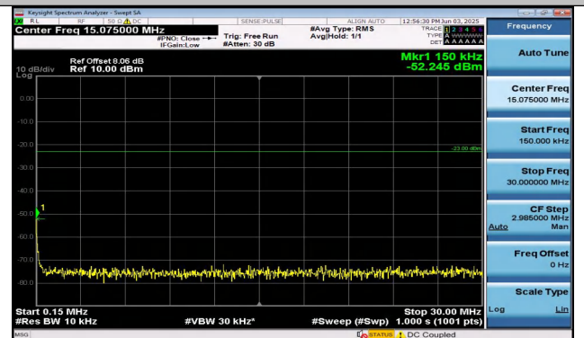
Band26(814-824)-5MHz-QPSK-26765-25RB#0-0.15~30-P ASS
