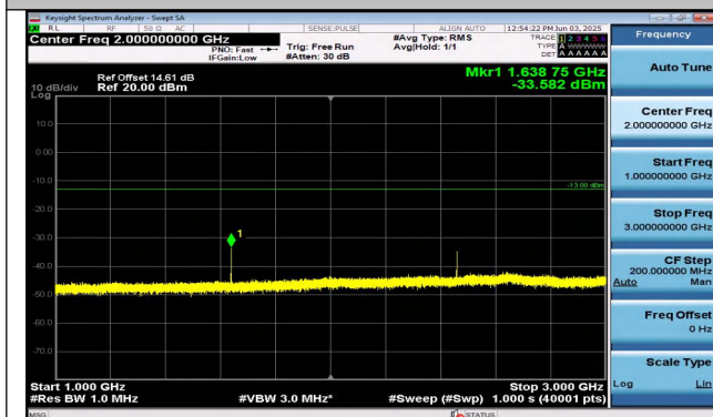
Band26(814-824)-5MHz-16QAM-26765-1RB#0-1000~300 0-PASS
