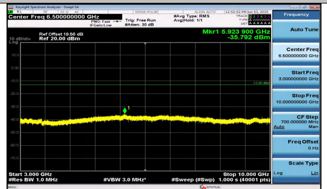
Band26(814-824)-5MHz-16QAM-26740-25RB#0-3000~10 000-PASS
