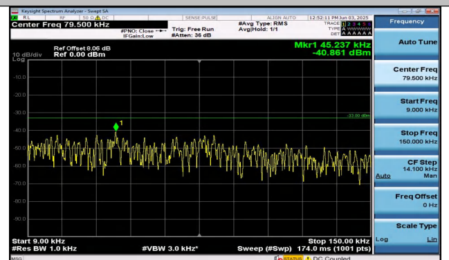
Band26(814-824)-5MHz-16QAM-26740-25RB#0-0.009~0. 15-PASS
