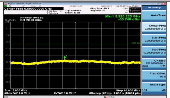
Band26(814-824)-5MHz-16QAM-26765-25RB#0-3000~10 000-PASS
