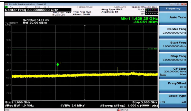
Band26(814-824)-10MHz-QPSK-26740-1RB#0-1000~300 0-PASS
