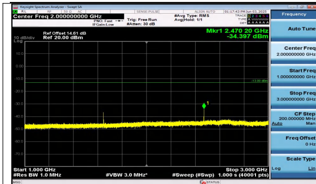
Band26(814-824)-10MHz-QPSK-26740-1RB#49-1000~300 0-PASS
