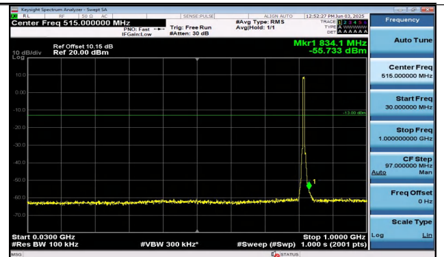
Band26(814-824)-5MHz-16QAM-26740-25RB#0-30~1000 -PASS
