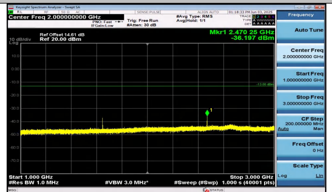
Band26(814-824)-10MHz-16QAM-26740-1RB#49-1000~3000-000-PASS
