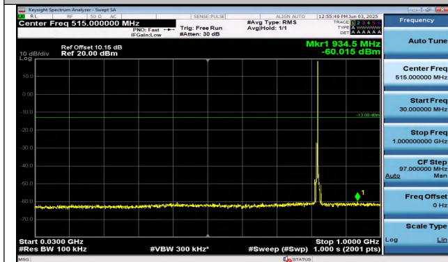
Band26(814-824)-5MHz-16QAM-26765-1RB#24-30~1000. PASS
