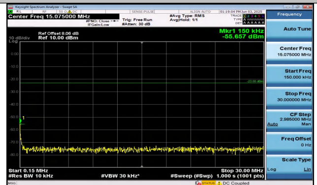
Band26(814-824)-10MHz-QPSK-26740-50RB#0-0.15~30- PASS
