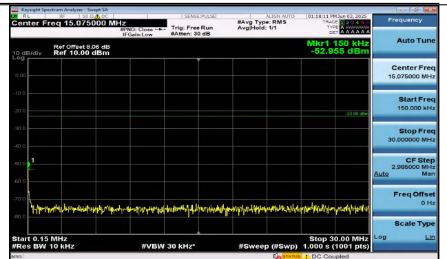
Band26(814-824)-10MHz-16QAM-26740-1RB#49-0.15~30-PASS
