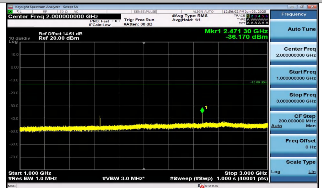
Band26(814-824)-5MHz-16QAM-26765-1RB#24-1000~30. 00-PASS
