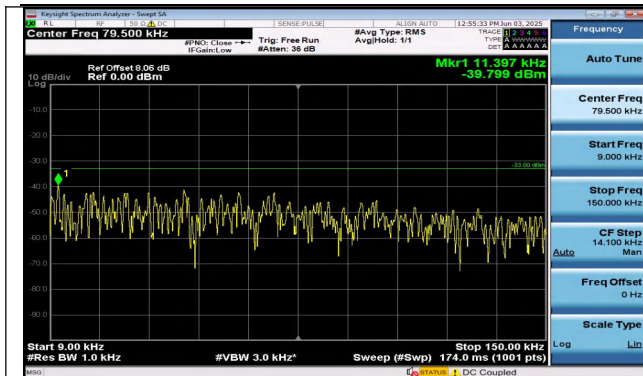
Band26(814-824)-5MHz-16QAM-26765-1RB#24-0.009~0. 15-PASS
