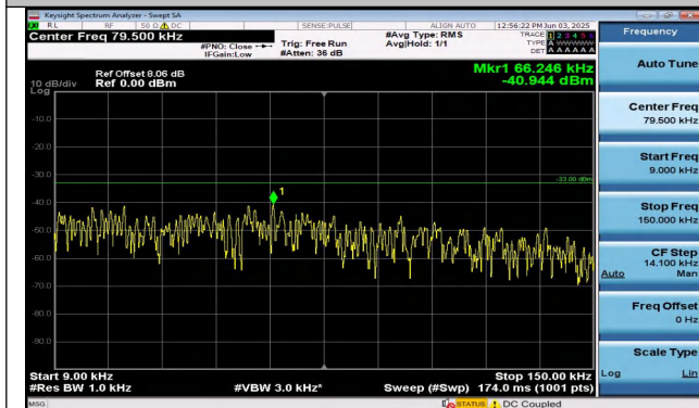
Band26(814-824)-5MHz-QPSK-26765-25RB#0-0.009~0.15 -PASS
