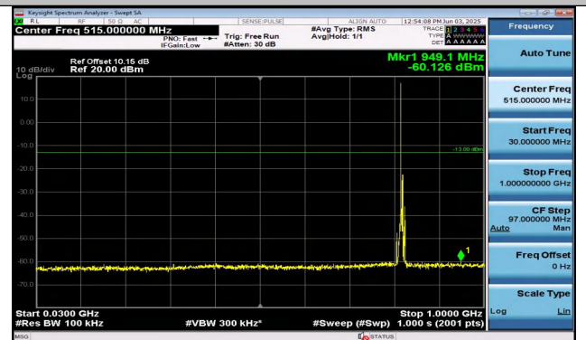
Band26(814-824)-5MHz-16QAM-26765-1RB#0-30~1000- PASS
