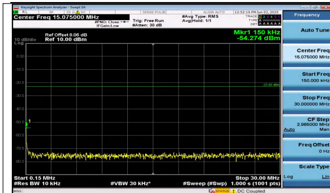
Band26(814-824)-5MHz-16QAM-26740-25RB#0-0.15~30- PASS
