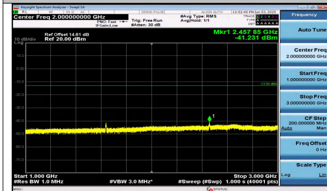
Band26(814-824)-5MHz-16QAM-26740-25RB#0-1000~30 00-PASS
