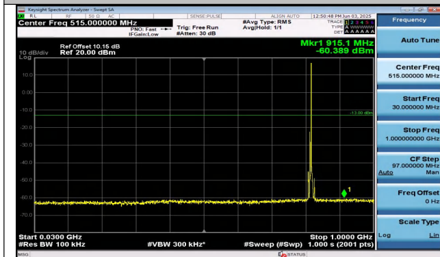
Band26(814-824)-5MHz-16QAM-26740-1RB#24-30~1000. PASS
