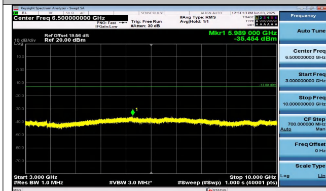
Band26(814-824)-5MHz-16QAM-26740-1RB#24-3000~10. 000-PASS
