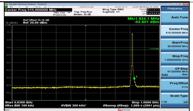
Band26(814-824)-5MHz-16QAM-26765-25RB#0-30~1000 -PASS
