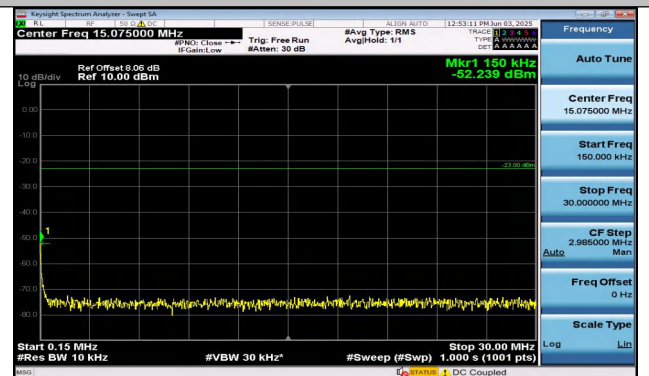
Band26(814-824)-5MHz-QPSK-26765-1RB#0-0.15~30-PA SS
