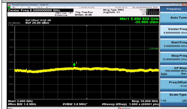
Band26(814-824)-10MHz-16QAM-26740-1RB#49-3000~10000-0000-PASS
