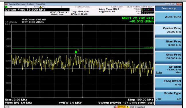
Band26(814-824)-5MHz-QPSK-26765-1RB#24-0.009~0.1 5-PASS
