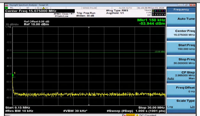
Band26(814-824)-10MHz-QPSK-26740-1RB#0-0.15~30-P ASS
