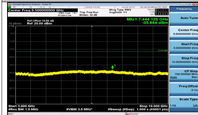
Band26(814-824)-10MHz-QPSK-26740-1RB#0-3000~1000 0-PASS
