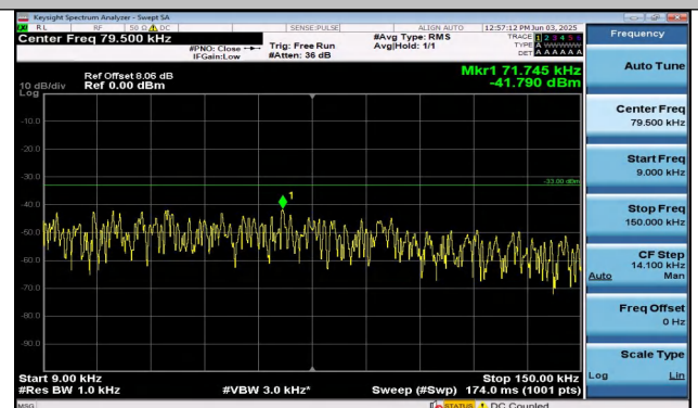
Band26(814-824)-5MHz-16QAM-26765-25RB#0-0.009~0. 15-PASS
