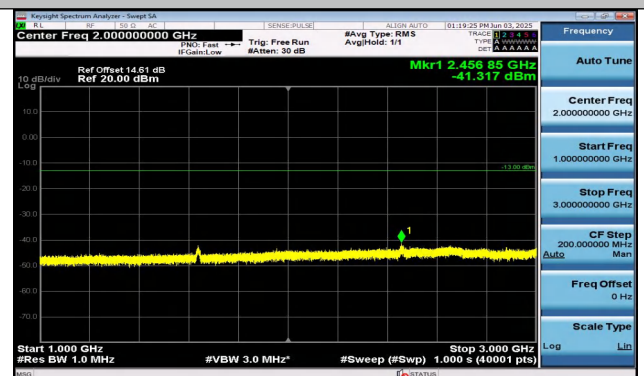
Band26(814-824)-10MHz-QPSK-26740-50RB#0-1000~30 00-PASS
