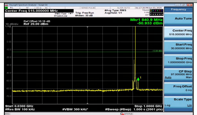
Band26(814-824)-10MHz-QPSK-26740-1RB#49-30~1000- PASS
