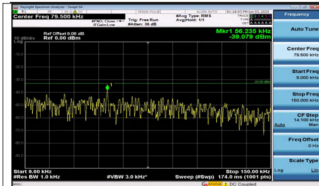
Band26(814-824)-10MHz-16QAM-26740-1RB#49-0.009~0.15-PASS
