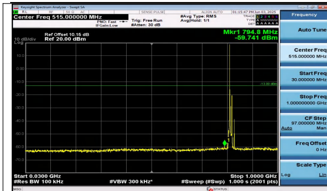
Band26(814-824)-10MHz-QPSK-26740-1RB#0-30~1000-P ASS
