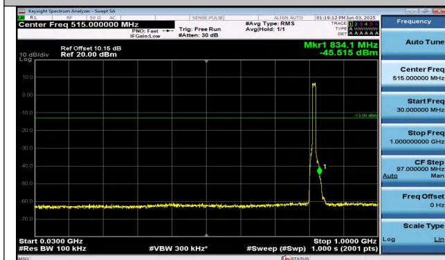
Band26(814-824)-10MHz-QPSK-26740-50RB#0-30~1000- PASS
