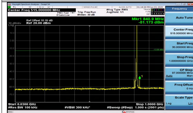
Band26(814-824)-10MHz-16QAM-26740-1RB#49-30~100-0-PASS
