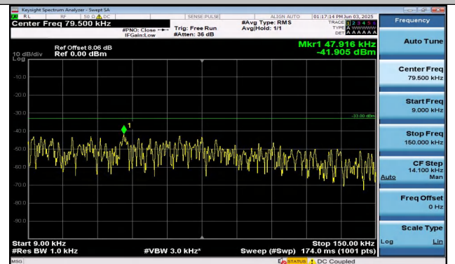
Band26(814-824)-10MHz-QPSK-26740-1RB#49-0.009~0. 15-PASS
