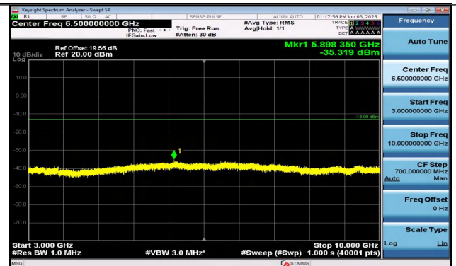
Band26(814-824)-10MHz-QPSK-26740-1RB#49-3000~10 000-PASS
