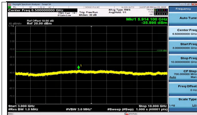
Band26(814-824)-5MHz-QPSK-26765-25RB#0-3000~1000 0-PASS
