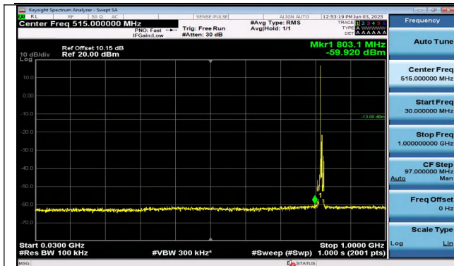
Band26(814-824)-5MHz-QPSK-26765-1RB#0-30~1000-PA SS
