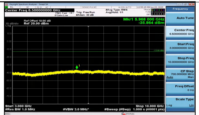
Band26(814-824)-5MHz-QPSK-26765-1RB#24-3000~100 00-PASS
