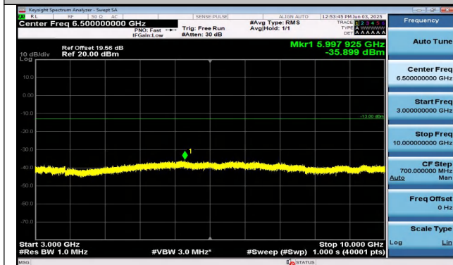
Band26(814-824)-5MHz-QPSK-26765-1RB#0-3000~10000 -PASS
