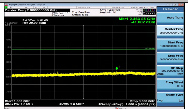
Band26(814-824)-5MHz-QPSK-26765-25RB#0-1000~300 0-PASS
