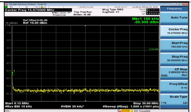
Band26(814-824)-5MHz-16QAM-26765-1RB#24-0.15~30. PASS
