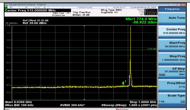
Band26(814-824)-5MHz-QPSK-26765-1RB#24-30~1000- PASS
