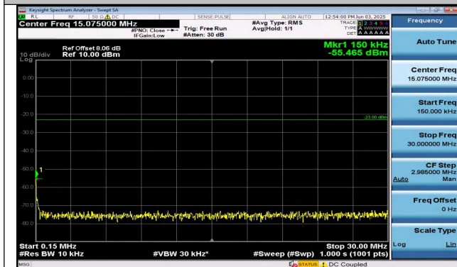
Band26(814-824)-5MHz-16QAM-26765-1RB#0-0.15~30-P ASS
