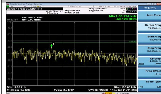
Band26(814-824)-10MHz-QPSK-26740-1RB#0-0.009~0.15 -PASS
