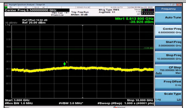
Band26(814-824)-5MHz-16QAM-26765-1RB#0-3000~100 00-PASS
