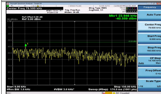
Band26(814-824)-5MHz-QPSK-26765-1RB#0-0.009~0.15- PASS
