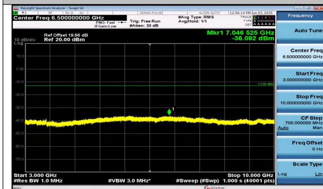
Band26(814-824)-5MHz-16QAM-26765-1RB#24-3000~10. 000-PASS
