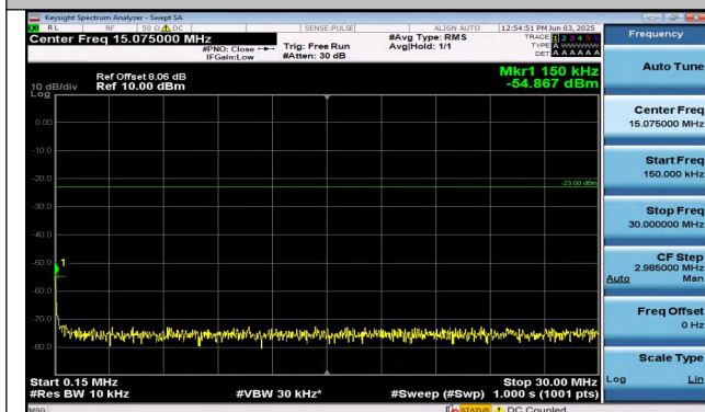
Band26(814-824)-5MHz-QPSK-26765-1RB#24-0.15~30-P ASS
