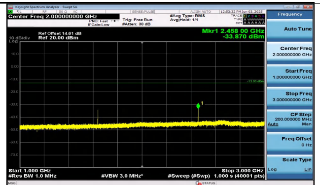
Band26(814-824)-5MHz-QPSK-26765-1RB#0-1000~3000- PASS
