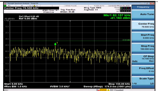
Band26(814-824)-5MHz-16QAM-26765-1RB#0-0.009~0.1 5-PASS
