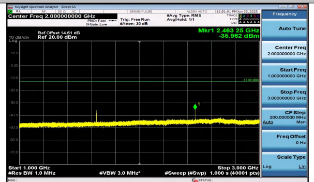
Band26(814-824)-5MHz-16QAM-26740-1RB#24-1000~30. 00-PASS
