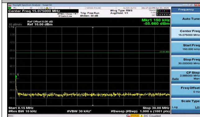
Band26(814-824)-10MHz-QPSK-26740-1RB#49-0.15~30- PASS
