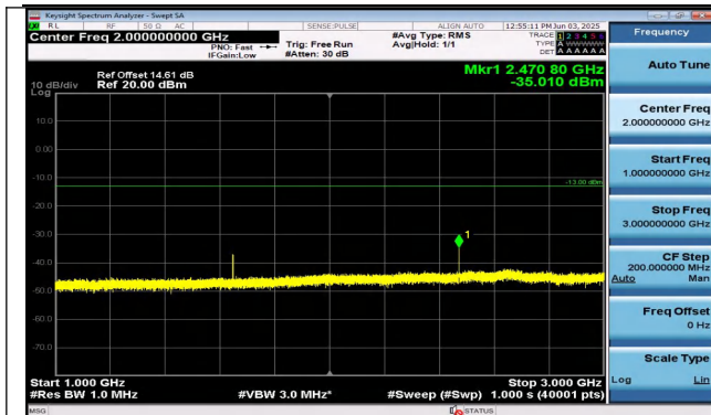
Band26(814-824)-5MHz-QPSK-26765-1RB#24-1000~3000 -PASS
