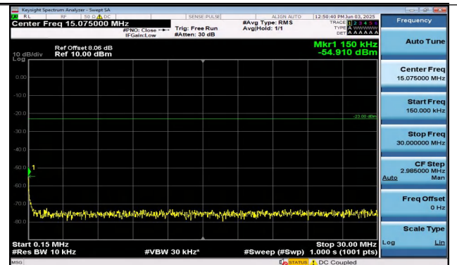
Band26(814-824)-5MHz-16QAM-26740-1RB#24-0.15~30. PASS
