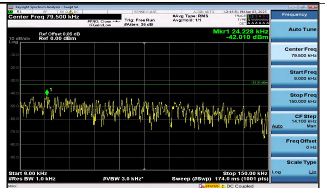
Band26(814-824)-5MHz-16QAM-26740-1RB#0-0.009~0.1 5-PASS
