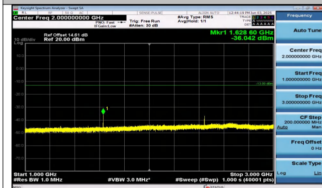
Band26(814-824)-5MHz-16QAM-26715-1RB#0-1000~300 0-PASS
