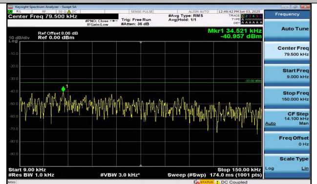
Band26(814-824)-5MHz-QPSK-26740-1RB#24-0.009~0.1 5-PASS
