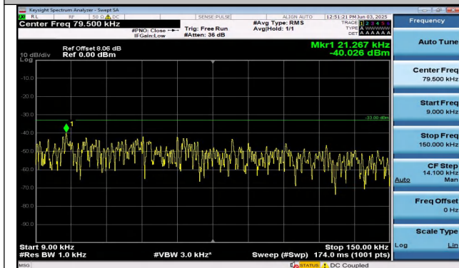
Band26(814-824)-5MHz-QPSK-26740-25RB#0-0.009~0.15 -PASS
