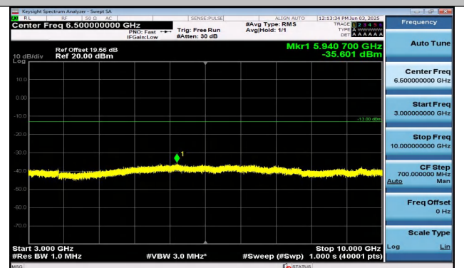
Band26(814-824)-3MHz-16QAM-26775-1RB#0-3000~100 00-PASS
