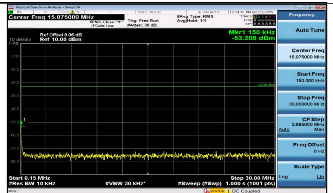
Band26(814-824)-3MHz-16QAM-26775-1RB#14-0.15~30- PASS
