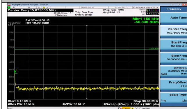
Band26(814-824)-5MHz-QPSK-26715-1RB#24-0.15~30-P ASS
