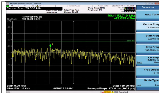
Band26(814-824)-5MHz-16QAM-26715-1RB#24-0.009~0. 15-PASS
