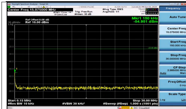
Band26(814-824)-3MHz-16QAM-26775-15RB#0-0.15~30- PASS
