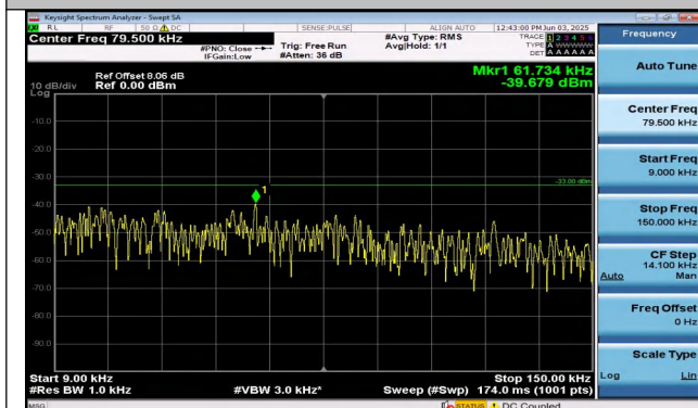
Band26(814-824)-5MHz-QPSK-26715-1RB#0-0.009~0.15- PASS
