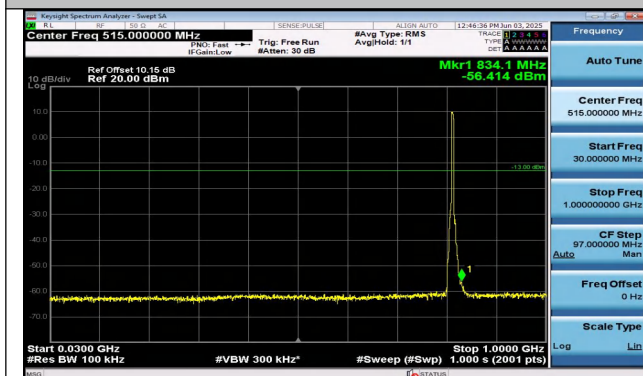
Band26(814-824)-5MHz-QPSK-26715-25RB#0-30~1000-P ASS
