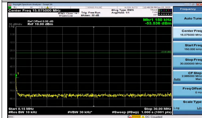
Band26(814-824)-5MHz-16QAM-26740-1RB#0-0.15~30-P ASS
