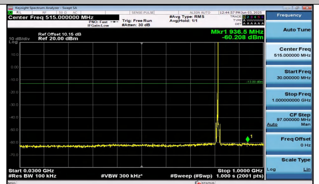
Band26(814-824)-5MHz-QPSK-26715-1RB#24-30~1000- PASS
