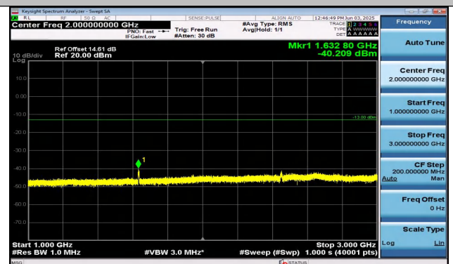
Band26(814-824)-5MHz-QPSK-26715-25RB#0-1000~300 0-PASS
