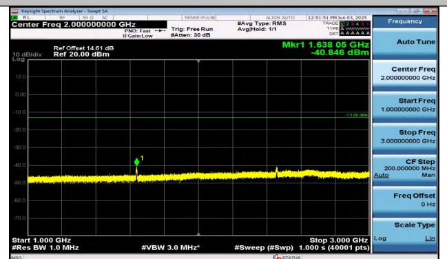
Band26(814-824)-5MHz-QPSK-26740-25RB#0-1000~300 0-PASS
