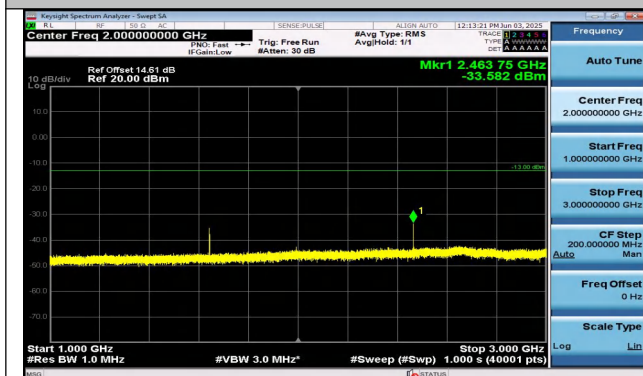
Band26(814-824)-3MHz-16QAM-26775-1RB#0-1000~300 0-PASS
