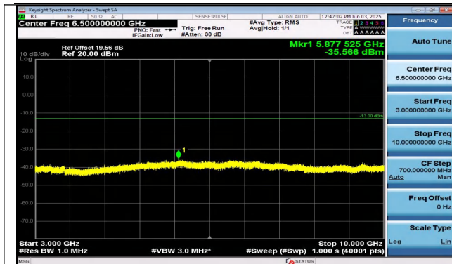
Band26(814-824)-5MHz-QPSK-26715-25RB#0-3000~1000 0-PASS
