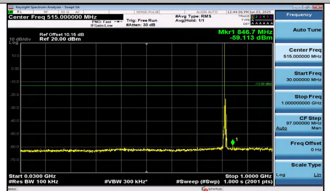
Band26(814-824)-5MHz-16QAM-26715-1RB#0-30~1000- PASS
