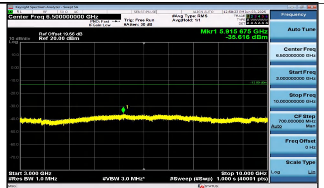
Band26(814-824)-5MHz-QPSK-26740-1RB#24-3000~100 00-PASS
