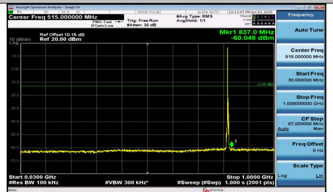
Band26(814-824)-3MHz-16QAM-26775-1RB#0-30~1000- PASS
