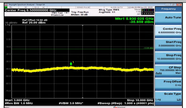
Band26(814-824)-5MHz-16QAM-26715-1RB#0-3000~100 00-PASS
