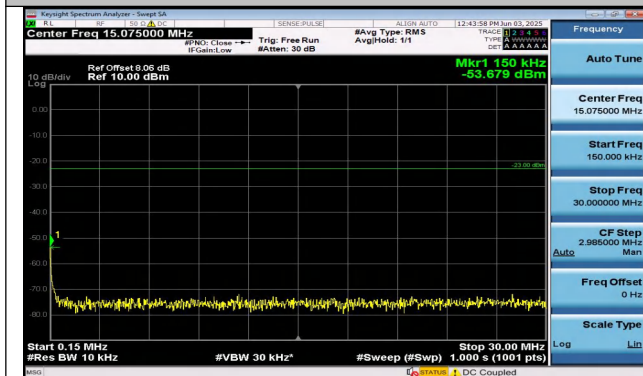
Band26(814-824)-5MHz-16QAM-26715-1RB#0-0.15~30-P ASS
