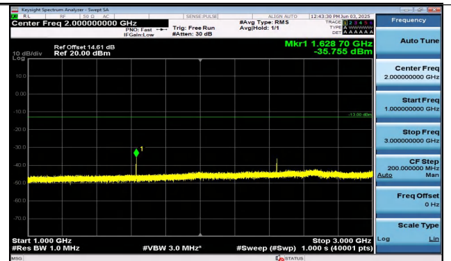
Band26(814-824)-5MHz-QPSK-26715-1RB#0-1000~3000- PASS
