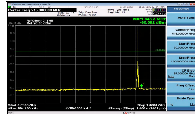
Band26(814-824)-5MHz-QPSK-26740-1RB#0-30~1000-PA SS
