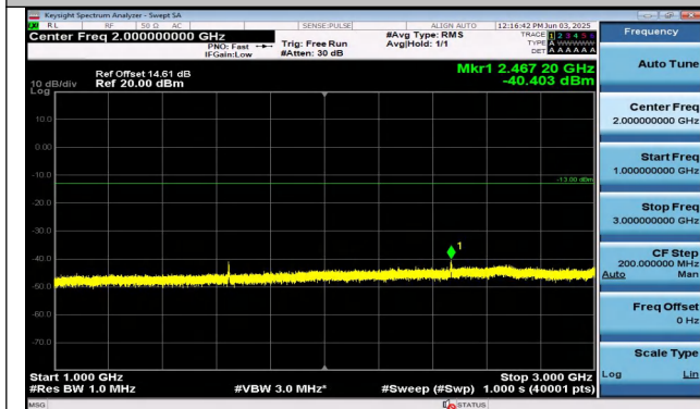
Band26(814-824)-3MHz-16QAM-26775-15RB#0-1000~30 00-PASS
