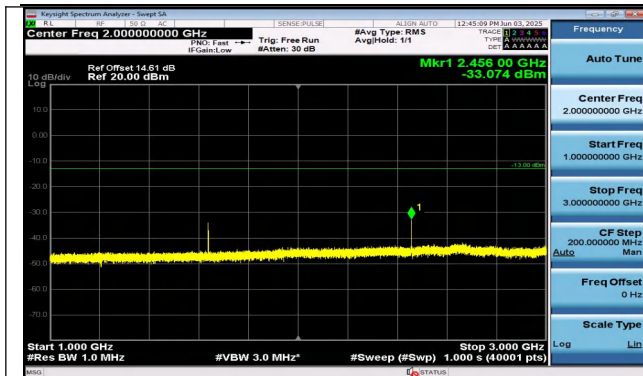
Band26(814-824)-5MHz-QPSK-26715-1RB#24-1000~3000 -PASS
