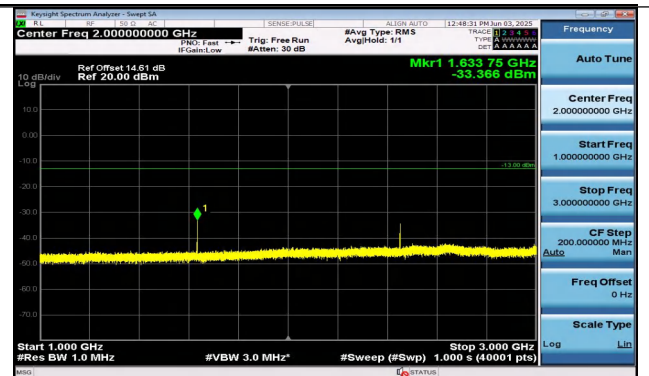
Band26(814-824)-5MHz-QPSK-26740-1RB#0-1000~3000- PASS
