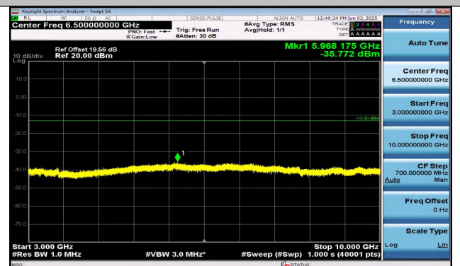
Band26(814-824)-5MHz-16QAM-26740-1RB#0-3000~100 00-PASS
