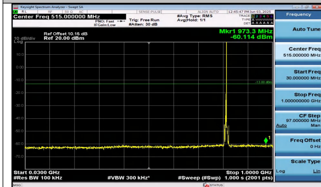
Band26(814-824)-5MHz-16QAM-26715-1RB#24-30~1000- PASS
