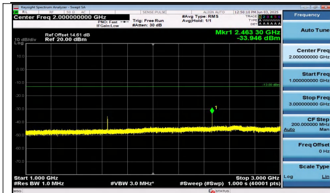
Band26(814-824)-5MHz-QPSK-26740-1RB#24-1000~3000 -PASS
