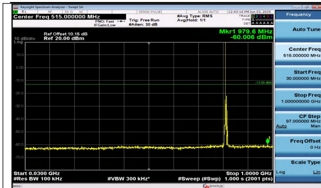
Band26(814-824)-5MHz-QPSK-26715-1RB#0-30~1000-PA SS
