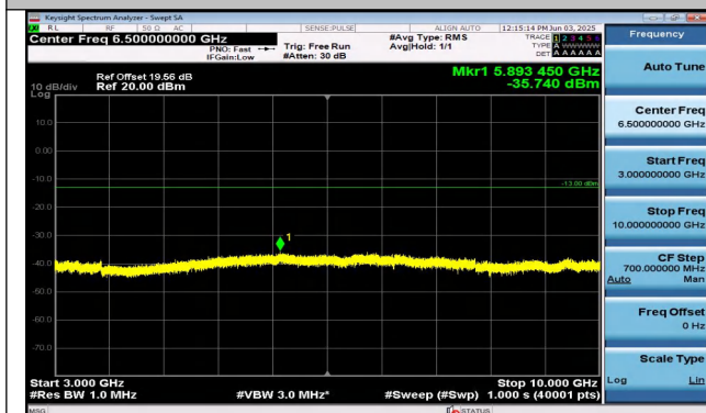
Band26(814-824)-3MHz-16QAM-26775-1RB#14-3000~10 000-PASS
