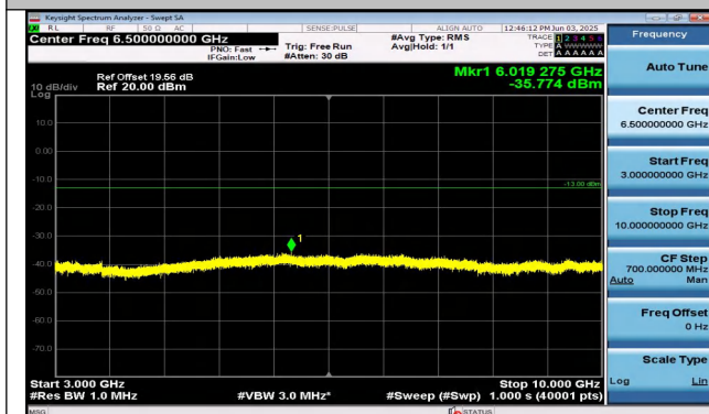
Band26(814-824)-5MHz-16QAM-26715-1RB#24-3000~10 000-PASS
