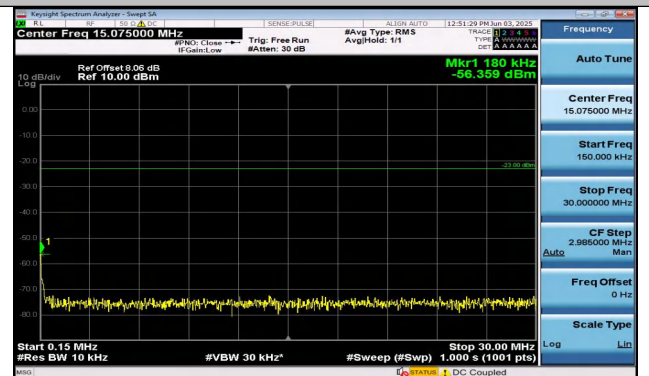
Band26(814-824)-5MHz-QPSK-26740-25RB#0-0.15~30-P ASS
