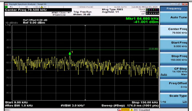
Band26(814-824)-5MHz-QPSK-26715-1RB#24-0.009~0.1 5-PASS
