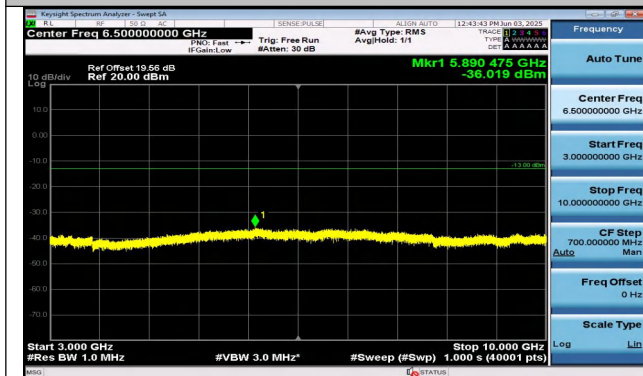
Band26(814-824)-5MHz-QPSK-26715-1RB#0-3000~10000- -PASS
