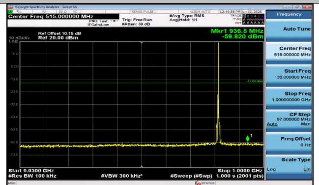
Band26(814-824)-5MHz-QPSK-26740-1RB#24-30~1000- PASS
