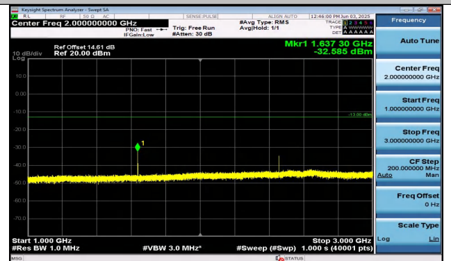
Band26(814-824)-5MHz-16QAM-26715-1RB#24-1000~30 00-PASS
