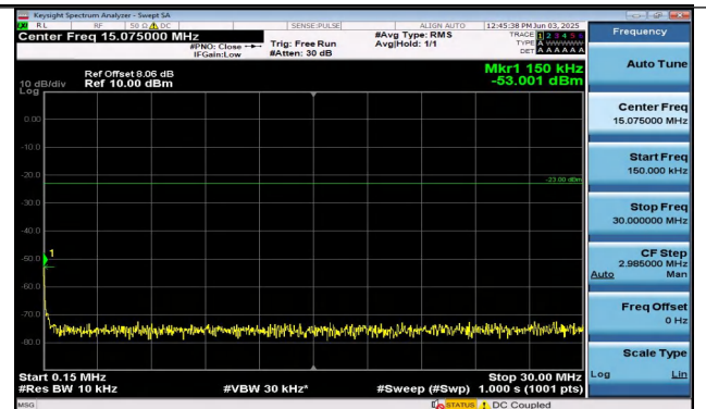
Band26(814-824)-5MHz-16QAM-26715-1RB#24-0.15~30- PASS
