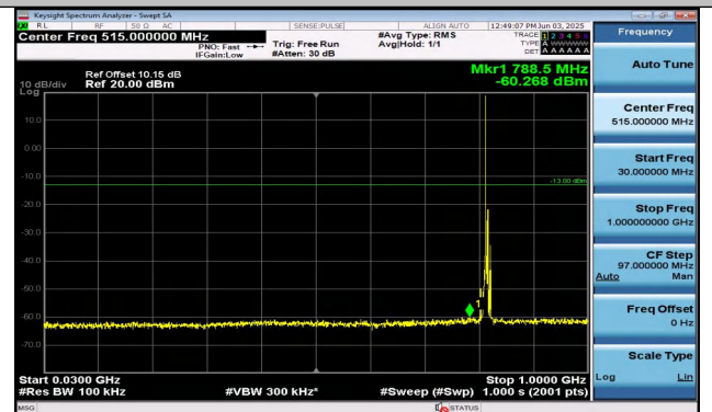
Band26(814-824)-5MHz-16QAM-26740-1RB#0-30~1000- PASS
