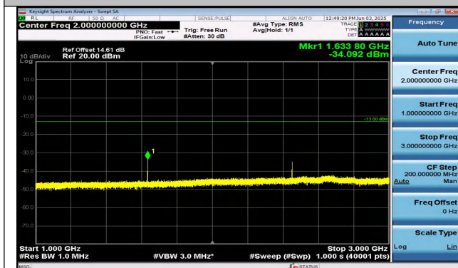
Band26(814-824)-5MHz-16QAM-26740-1RB#0-1000~300 0-PASS
