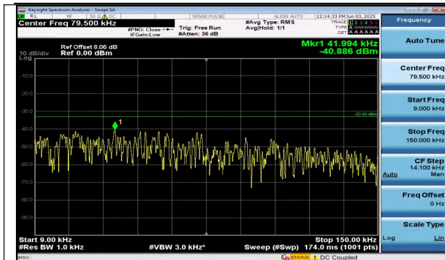
Band26(814-824)-3MHz-16QAM-26775-1RB#14-0.009~0. 15-PASS
