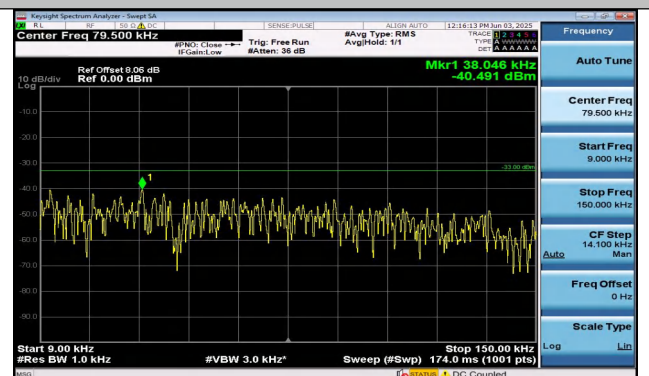
Band26(814-824)-3MHz-16QAM-26775-15RB#0-0.009~0. 15-PASS
