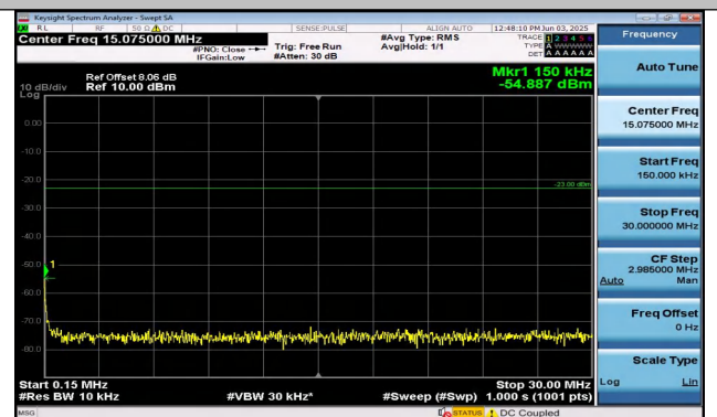
Band26(814-824)-5MHz-QPSK-26740-1RB#0-0.15~30-PA SS
