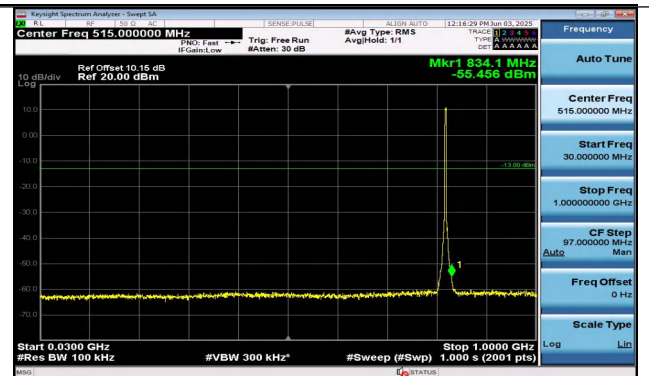
Band26(814-824)-3MHz-16QAM-26775-15RB#0-30~1000 -PASS
