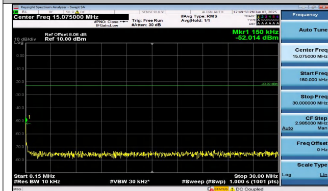
Band26(814-824)-5MHz-QPSK-26740-1RB#24-0.15~30-P ASS
