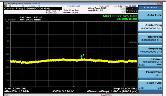
Band26(814-824)-5MHz-16QAM-26715-25RB#0-3000~10 000-PASS
