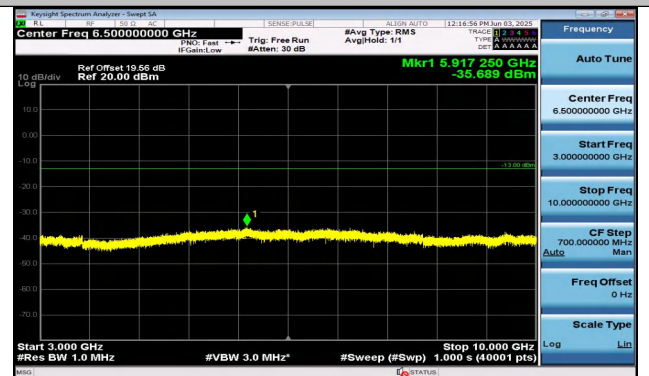
Band26(814-824)-3MHz-16QAM-26775-15RB#0-3000~10 000-PASS
