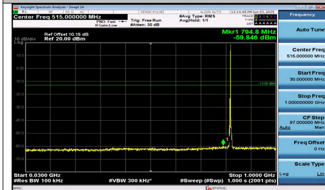
Band26(814-824)-3MHz-16QAM-26775-1RB#14-30~1000- PASS
