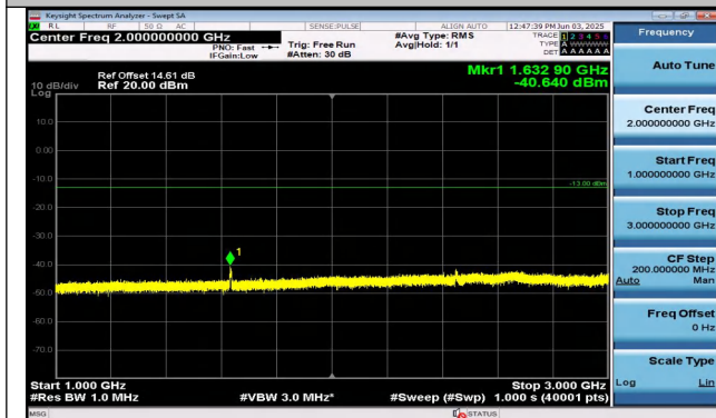
Band26(814-824)-5MHz-16QAM-26715-25RB#0-1000~30 00-PASS
