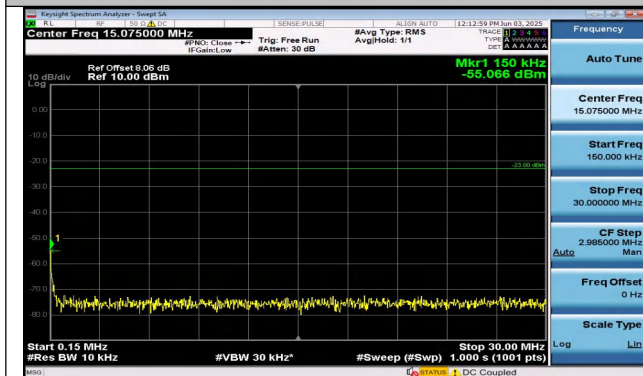
Band26(814-824)-3MHz-16QAM-26775-1RB#0-0.15~30-P ASS
