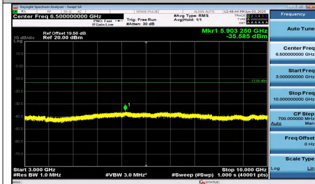
Band26(814-824)-5MHz-QPSK-26740-1RB#0-3000~10000- -PASS
