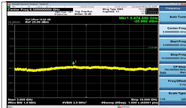
Band26(814-824)-3MHz-QPSK-26775-15RB#0-3000~1000 0-PASS
