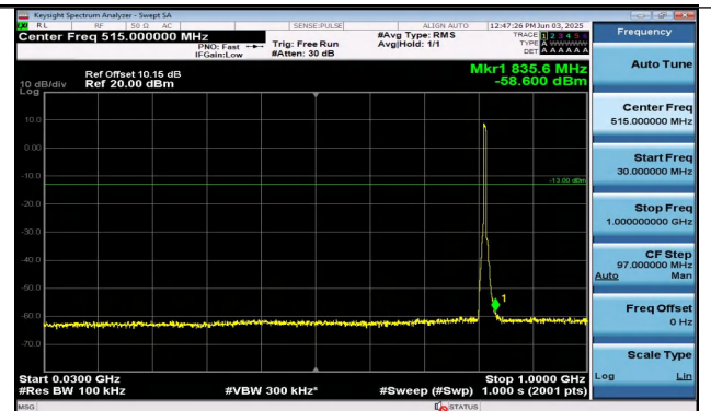
Band26(814-824)-5MHz-16QAM-26715-25RB#0-30~1000 -PASS
