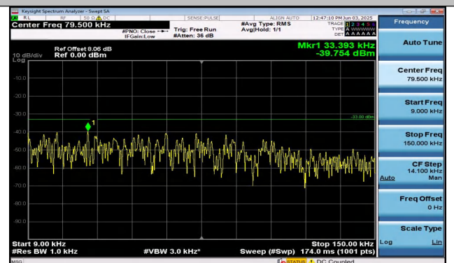
Band26(814-824)-5MHz-16QAM-26715-25RB#0-0.009~0. 15-PASS
