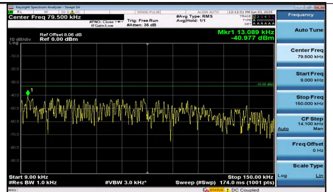
Band26(814-824)-3MHz-16QAM-26775-1RB#0-0.009~0.1 5-PASS
