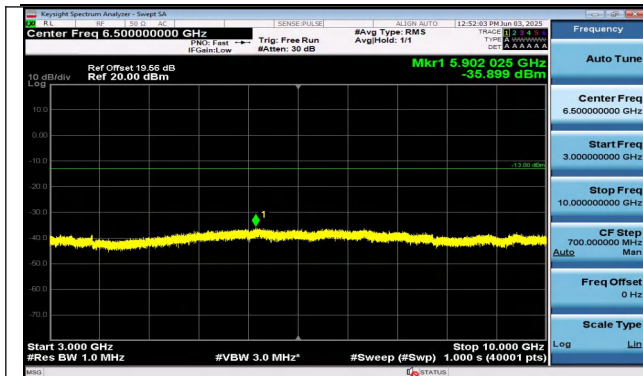
Band26(814-824)-5MHz-QPSK-26740-25RB#0-3000~1000 0-PASS
