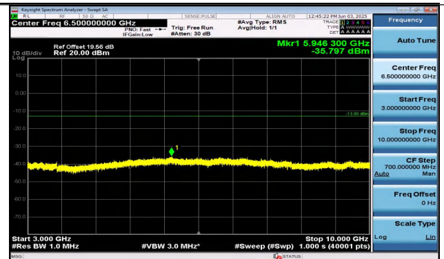
Band26(814-824)-5MHz-QPSK-26715-1RB#24-3000~100 00-PASS
