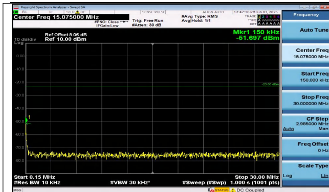
Band26(814-824)-5MHz-16QAM-26715-25RB#0-0.15~30- PASS
