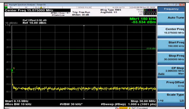
Band26(814-824)-5MHz-QPSK-26715-1RB#0-0.15~30-PA SS
