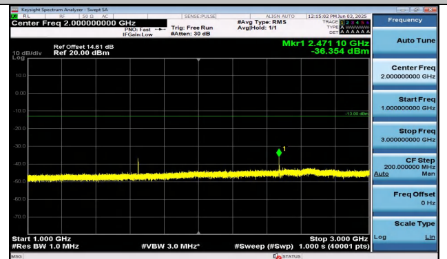
Band26(814-824)-3MHz-16QAM-26775-1RB#14-1000~30 00-PASS
