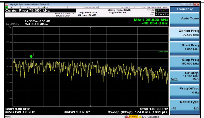
Band26(814-824)-5MHz-16QAM-26715-1RB#0-0.009~0.1 5-PASS
