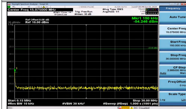
Band26(814-824)-3MHz-16QAM-26740-1RB#0-0.15~30-P ASS
