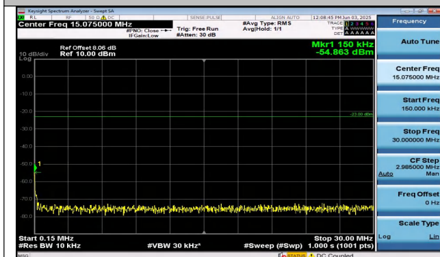
Band26(814-824)-3MHz-QPSK-26740-1RB#14-0.15~30-P ASS
