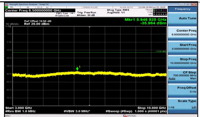
Band26(814-824)-3MHz-QPSK-26740-1RB#14-3000~100 00-PASS
