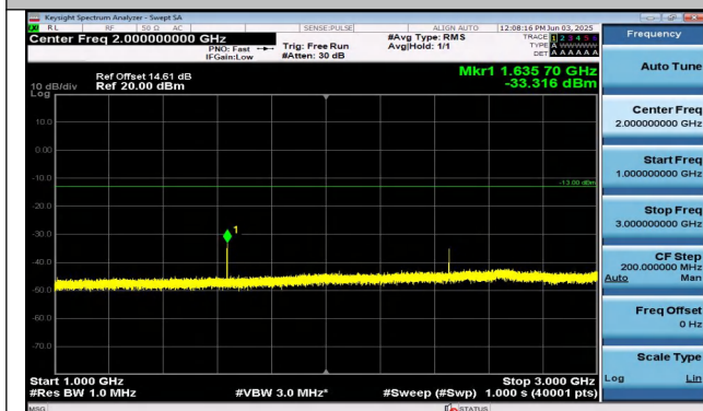
Band26(814-824)-3MHz-16QAM-26740-1RB#0-1000~300 0-PASS
