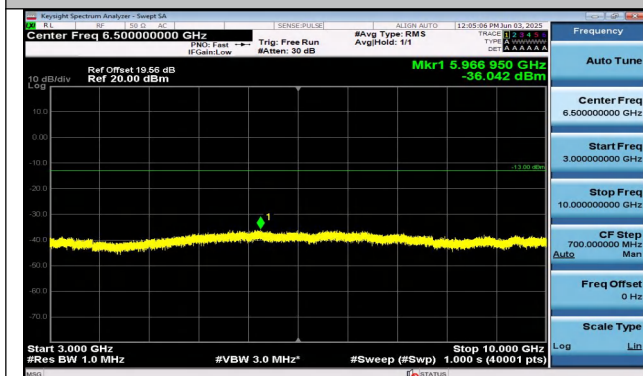
Band26(814-824)-3MHz-16QAM-26705-1RB#14-3000~10. 000-PASS
