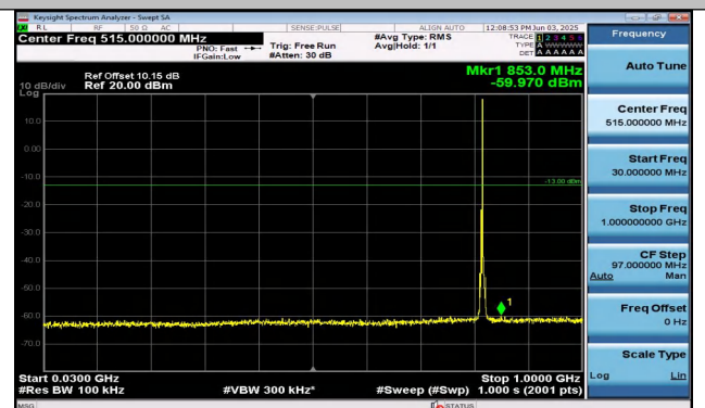
Band26(814-824)-3MHz-QPSK-26740-1RB#14-30~1000- PASS
