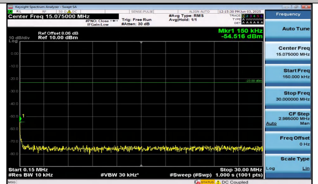
Band26(814-824)-3MHz-QPSK-26775-15RB#0-0.15~30-P ASS
