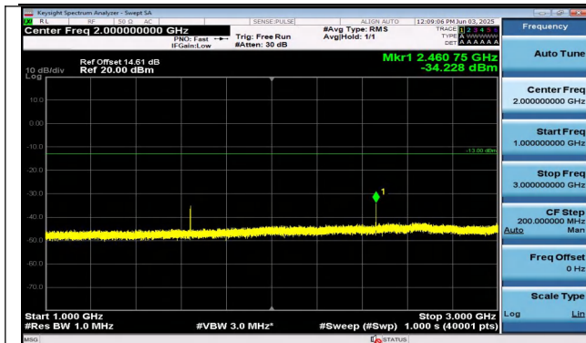
Band26(814-824)-3MHz-QPSK-26740-1RB#14-1000~3000 -PASS
