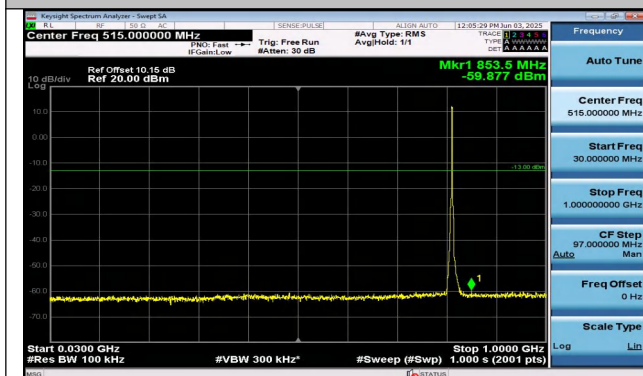
Band26(814-824)-3MHz-QPSK-26705-15RB#0-30~1000-P ASS
