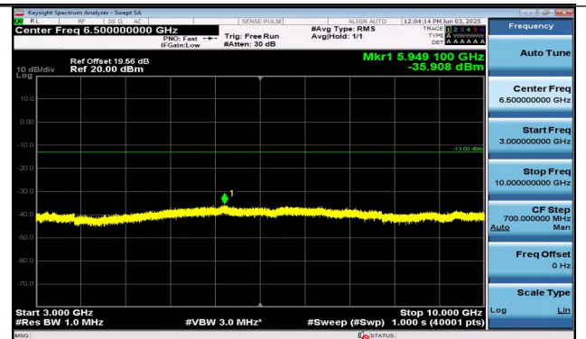
Band26(814-824)-3MHz-QPSK-26705-1RB#14-3000~100 00-PASS
