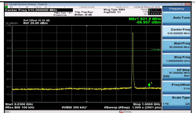
Band26(814-824)-3MHz-16QAM-26705-15RB#0-30~1000 -PASS
