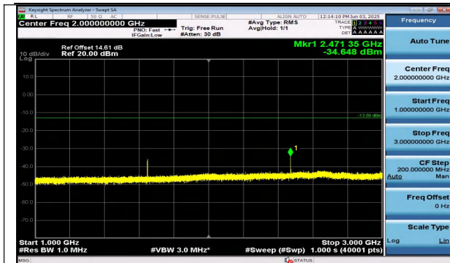
Band26(814-824)-3MHz-QPSK-26775-1RB#14-1000~3000 -PASS
