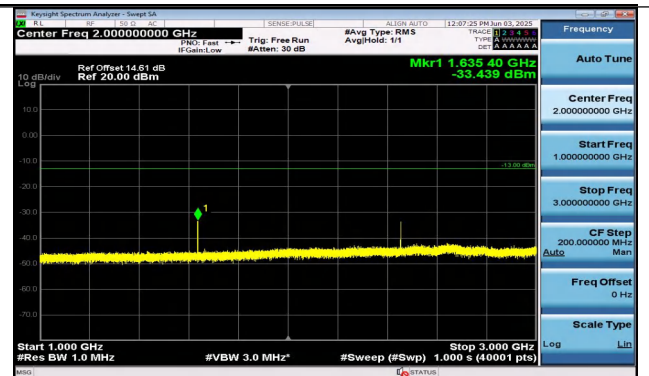
Band26(814-824)-3MHz-QPSK-26740-1RB#0-1000~3000- PASS
