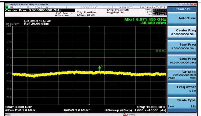
Band26(814-824)-3MHz-QPSK-26775-1RB#14-3000~100 00-PASS
