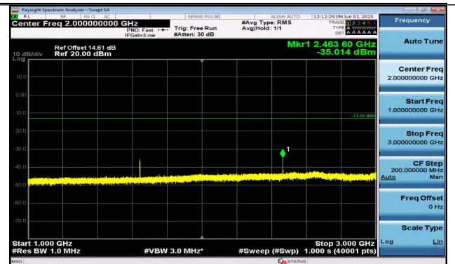
Band26(814-824)-3MHz-QPSK-26775-1RB#0-1000~3000- PASS
