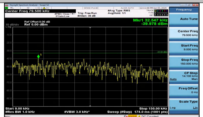
Band26(814-824)-3MHz-16QAM-26740-15RB#0-0.009~0. 15-PASS
