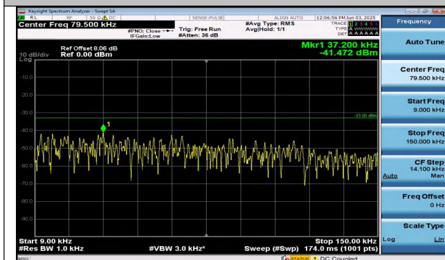
Band26(814-824)-3MHz-QPSK-26740-1RB#0-0.009~0.15- PASS
