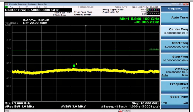
Band26(814-824)-3MHz-16QAM-26740-15RB#0-3000~10 000-PASS
