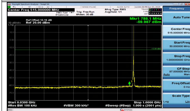
Band26(814-824)-3MHz-16QAM-26705-1RB#14-30~1000. PASS
