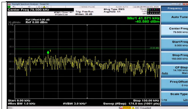
Band26(814-824)-3MHz-16QAM-26740-1RB#14-0.009~0. 15-PASS
