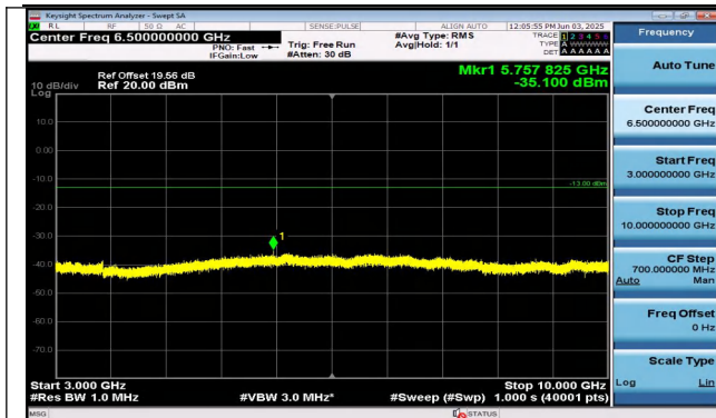
Band26(814-824)-3MHz-QPSK-26705-15RB#0-3000~1000 0-PASS
