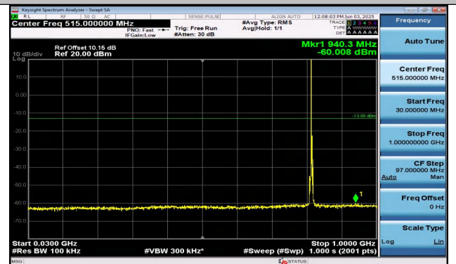
Band26(814-824)-3MHz-16QAM-26740-1RB#0-30~1000- PASS
