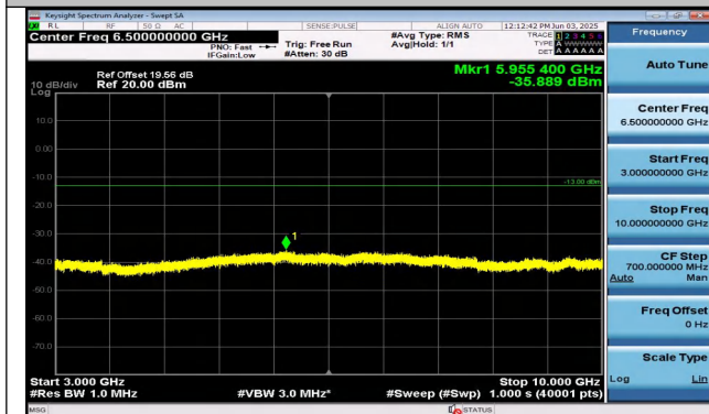
Band26(814-824)-3MHz-QPSK-26775-1RB#0-3000~10000- -PASS
