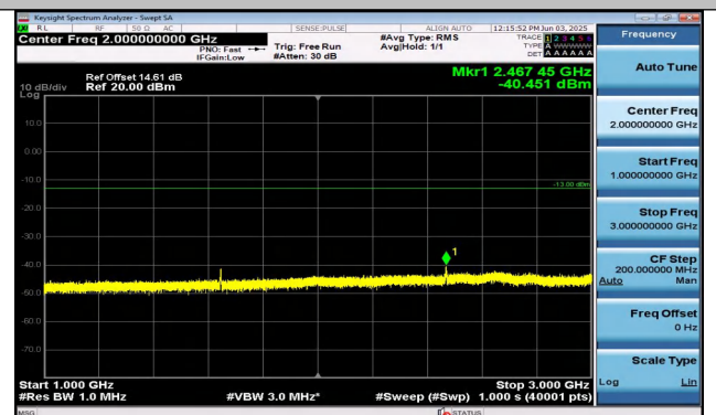
Band26(814-824)-3MHz-QPSK-26775-15RB#0-1000~300 0-PASS
