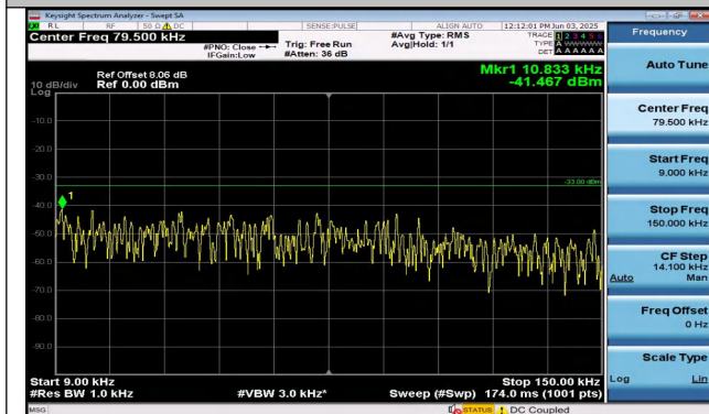
Band26(814-824)-3MHz-QPSK-26775-1RB#0-0.009~0.15- PASS
