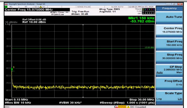
Band26(814-824)-3MHz-QPSK-26705-15RB#0-0.15~30-P ASS
