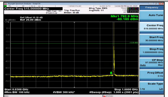
Band26(814-824)-3MHz-16QAM-26705-1RB#0-30~1000- PASS
