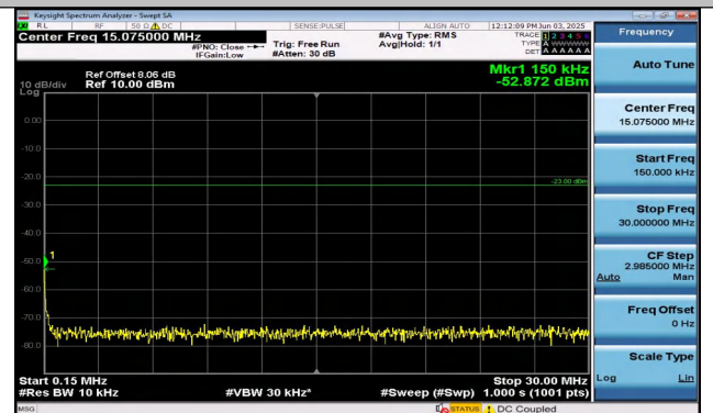
Band26(814-824)-3MHz-QPSK-26775-1RB#0-0.15~30-PA SS
