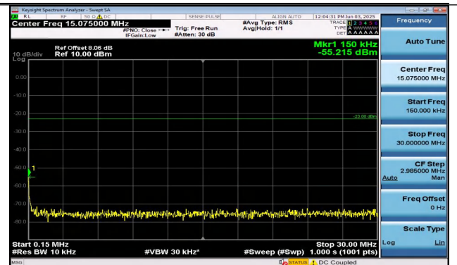
Band26(814-824)-3MHz-16QAM-26705-1RB#14-0.15~30. PASS
