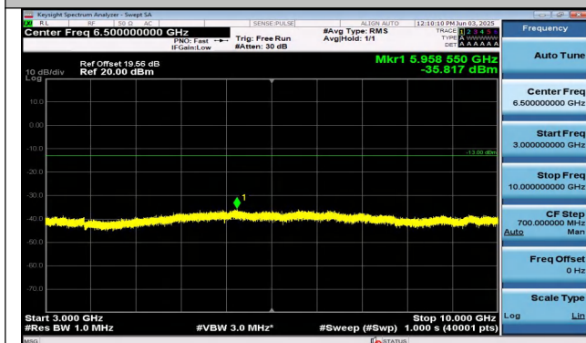
Band26(814-824)-3MHz-16QAM-26740-1RB#14-3000~10. 000-PASS
