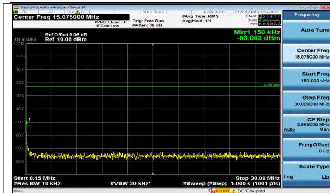
Band26(814-824)-3MHz-16QAM-26705-15RB#0-0.15~30- PASS
