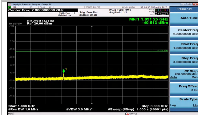
Band26(814-824)-3MHz-16QAM-26705-15RB#0-1000~30 00-PASS
