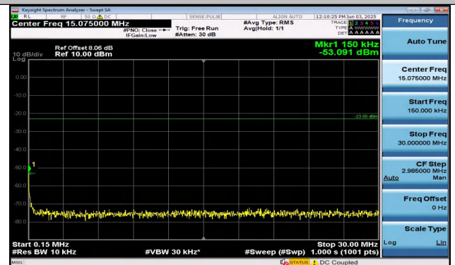
Band26(814-824)-3MHz-QPSK-26740-15RB#0-0.15~30-P ASS
