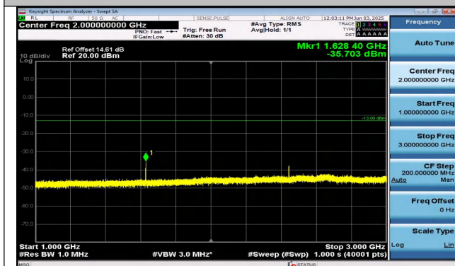
Band26(814-824)-3MHz-16QAM-26705-1RB#0-1000~300 0-PASS
