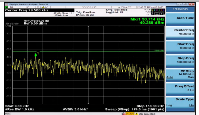
Band26(814-824)-3MHz-QPSK-26740-1RB#14-0.009~0.1 5-PASS
