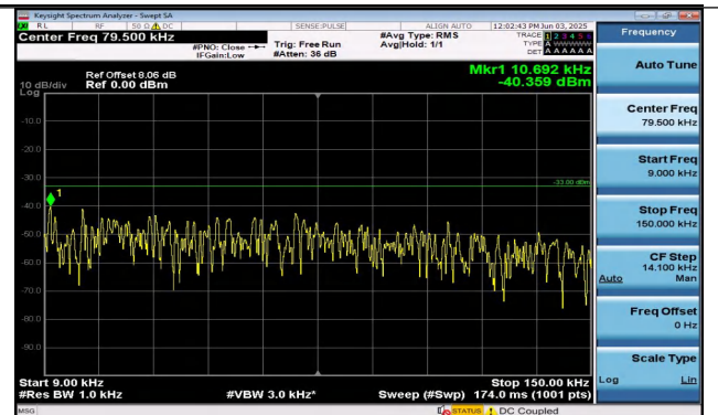
Band26(814-824)-3MHz-16QAM-26705-1RB#0-0.009~0.1 5-PASS
