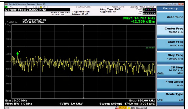
Band26(814-824)-3MHz-16QAM-26740-1RB#0-0.009~0.1 5-PASS
