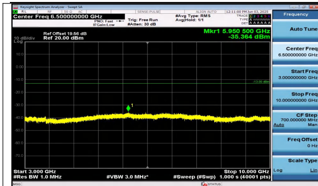
Band26(814-824)-3MHz-QPSK-26740-15RB#0-3000~1000 0-PASS
