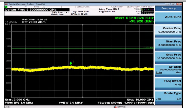
Band26(814-824)-3MHz-16QAM-26705-15RB#0-3000~10 000-PASS
