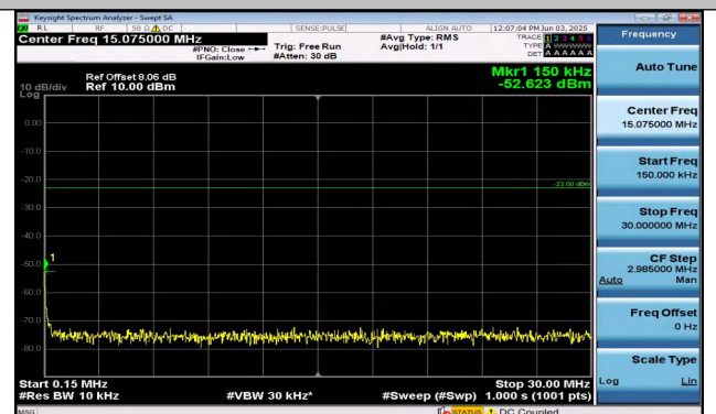
Band26(814-824)-3MHz-QPSK-26740-1RB#0-0.15~30-PA SS
