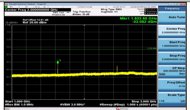
Band26(814-824)-3MHz-16QAM-26705-1RB#14-1000~30. 00-PASS
