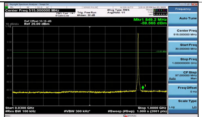
Band26(814-824)-3MHz-16QAM-26740-15RB#0-30~1000 -PASS
