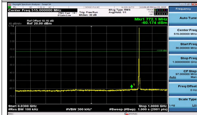
Band26(814-824)-3MHz-16QAM-26740-1RB#14-30~1000. PASS
