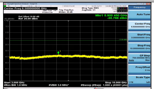
Band26(814-824)-3MHz-16QAM-26740-1RB#0-3000~100 00-PASS
