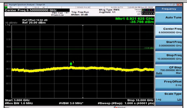
Band26(814-824)-3MHz-16QAM-26705-1RB#0-3000~100 00-PASS
