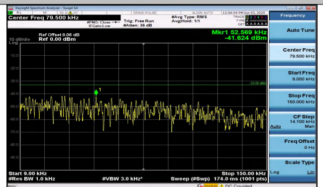
Band26(814-824)-3MHz-16QAM-26705-15RB#0-0.009~0. 15-PASS
