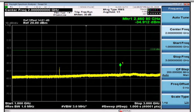
Band26(814-824)-3MHz-16QAM-26740-1RB#14-1000~30. 00-PASS
