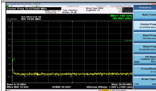
Band26(814-824)-3MHz-QPSK-26775-1RB#14-0.15~30-P ASS
