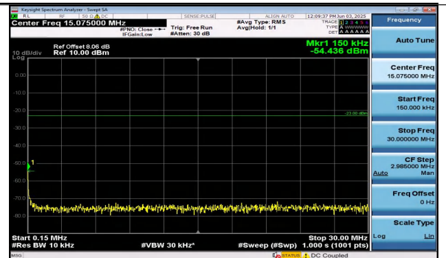
Band26(814-824)-3MHz-16QAM-26740-1RB#14-0.15~30. PASS
