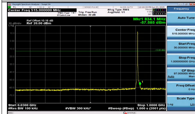
Band26(814-824)-3MHz-QPSK-26740-15RB#0-30~1000-P ASS
