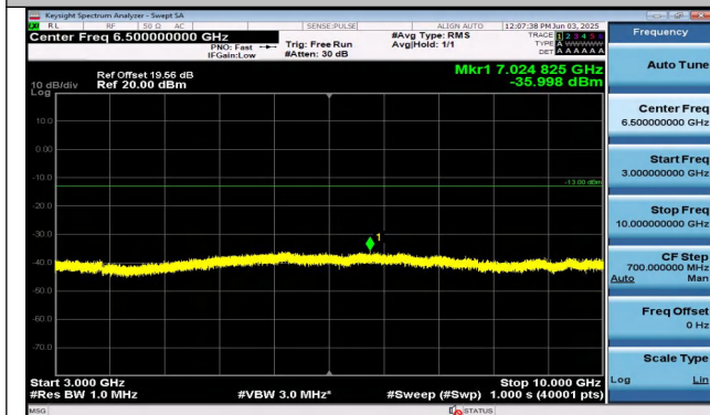
Band26(814-824)-3MHz-QPSK-26740-1RB#0-3000~10000 -PASS
