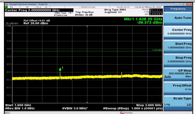
Band26(814-824)-3MHz-QPSK-26740-15RB#0-1000~300 0-PASS
