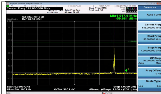
Band26(814-824)-3MHz-QPSK-26775-1RB#0-30~1000-PA SS
