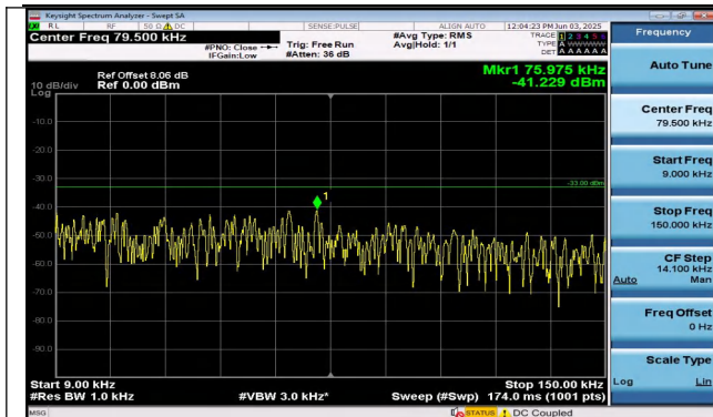
Band26(814-824)-3MHz-16QAM-26705-1RB#14-0.009~0. 15-PASS
