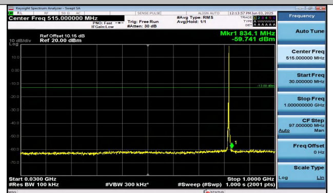
Band26(814-824)-3MHz-QPSK-26775-1RB#14-30~1000- PASS
