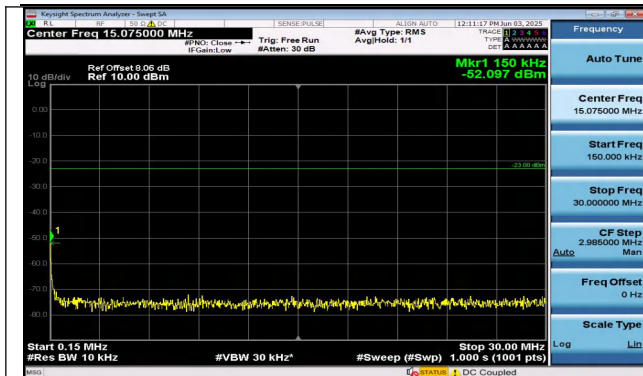
Band26(814-824)-3MHz-16QAM-26740-15RB#0-0.15~30- PASS
