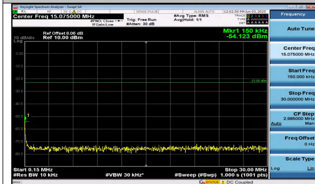
Band26(814-824)-3MHz-16QAM-26705-1RB#0-0.15~30-P ASS
