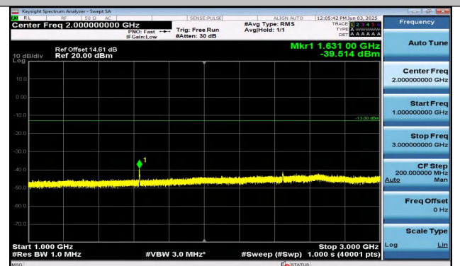
Band26(814-824)-3MHz-QPSK-26705-15RB#0-1000~300 0-PASS
