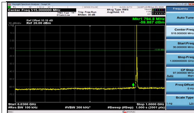
Band26(814-824)-3MHz-QPSK-26740-1RB#0-30~1000-PA SS
