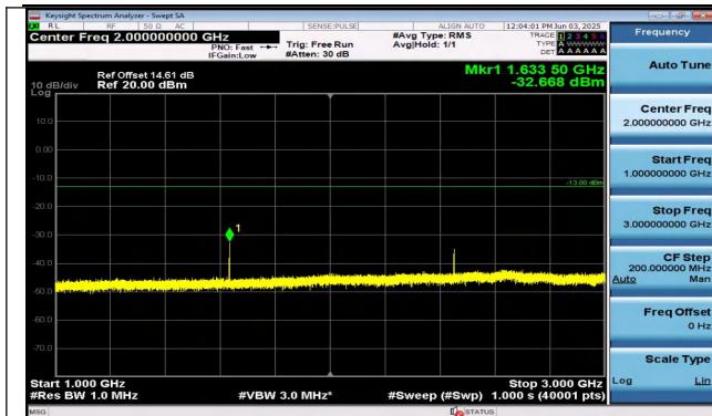
Band26(814-824)-3MHz-QPSK-26705-1RB#14-1000~3000 -PASS
