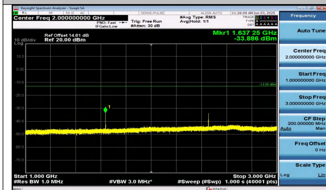
Band26(814-824)-1.4MHz-16QAM-26740-1RB#0-1000~30 00-PASS
