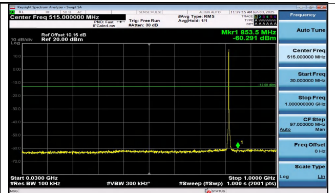
Band26(814-824)-1.4MHz-16QAM-26740-6RB#0-30~1000 -PASS
