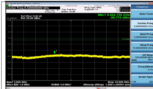
Band26(814-824)-1.4MHz-QPSK-26783-6RB#0-3000~100 00-PASS
