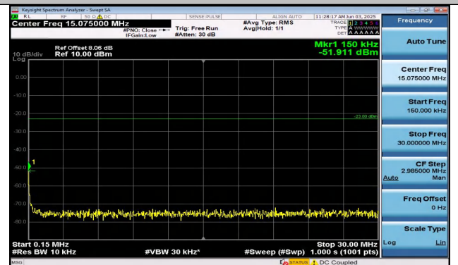
Band26(814-824)-1.4MHz-QPSK-26740-6RB#0-0.15~30- PASS
