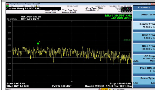
Band26(814-824)-1.4MHz-QPSK-26783-1RB#0-0.009~0.1 5-PASS
