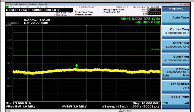
Band26(814-824)-1.4MHz-16QAM-26783-6RB#0-3000~10- 000-PASS
