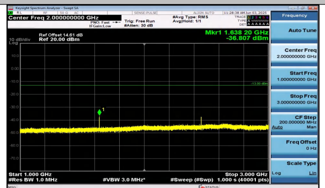
Band26(814-824)-1.4MHz-QPSK-26740-6RB#0-1000~300 0-PASS
