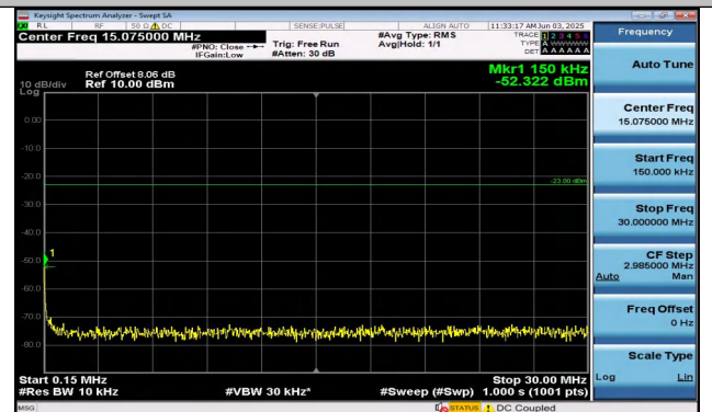
Band26(814-824)-1.4MHz-QPSK-26783-6RB#0-0.15~30- PASS
