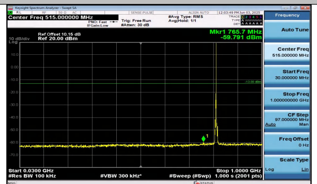
Band26(814-824)-3MHz-QPSK-26705-1RB#14-30~1000- PASS
