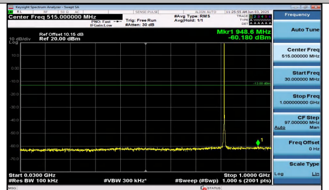
Band26(814-824)-1.4MHz-16QAM-26740-1RB#0-30~1000- -PASS
