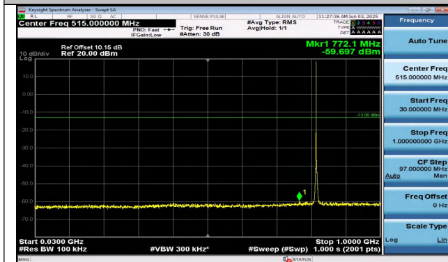
Band26(814-824)-1.4MHz-16QAM-26740-1RB#5-30~1000 -PASS
