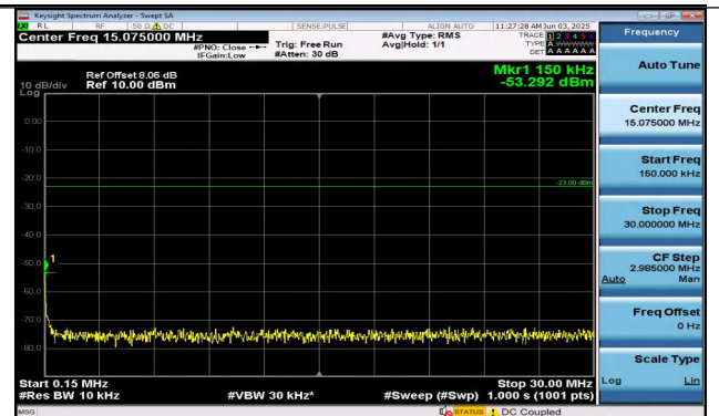
Band26(814-824)-1.4MHz-16QAM-26740-1RB#5-0.15~30 -PASS
