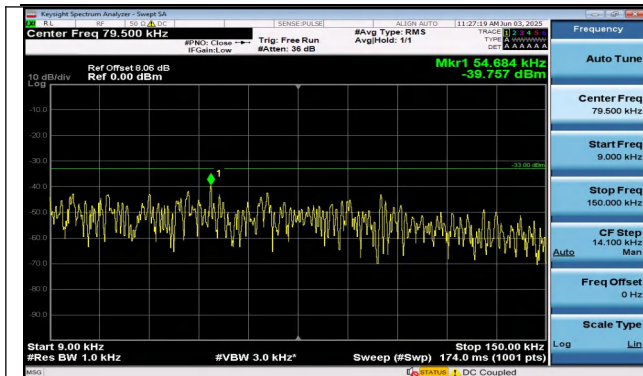
Band26(814-824)-1.4MHz-16QAM-26740-1RB#5-0.009~0. 15-PASS
