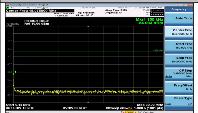
Band26(814-824)-1.4MHz-QPSK-26783-1RB#0-0.15~30- PASS
