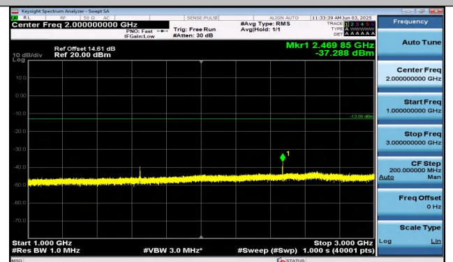
Band26(814-824)-1.4MHz-QPSK-26783-6RB#0-1000~300 0-PASS
