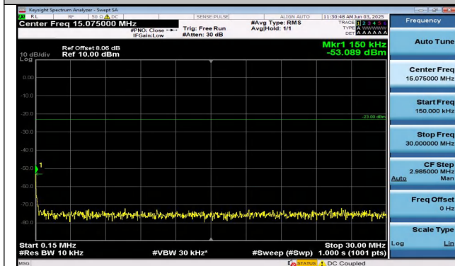
Band26(814-824)-1.4MHz-16QAM-26783-1RB#0-0.15~30- PASS
