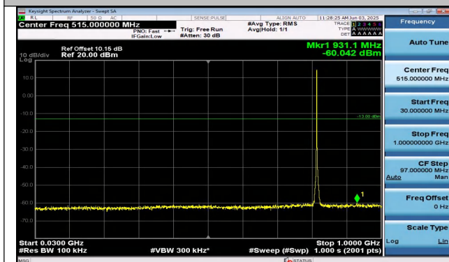
Band26(814-824)-1.4MHz-QPSK-26740-6RB#0-30~1000- PASS
