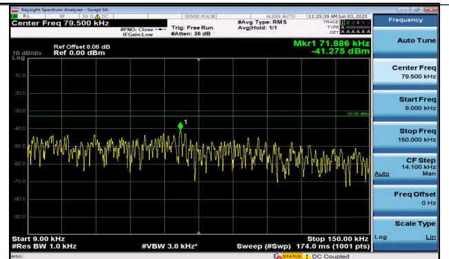
Band26(814-824)-1.4MHz-16QAM-26740-1RB#0-0.009~0. 15-PASS
