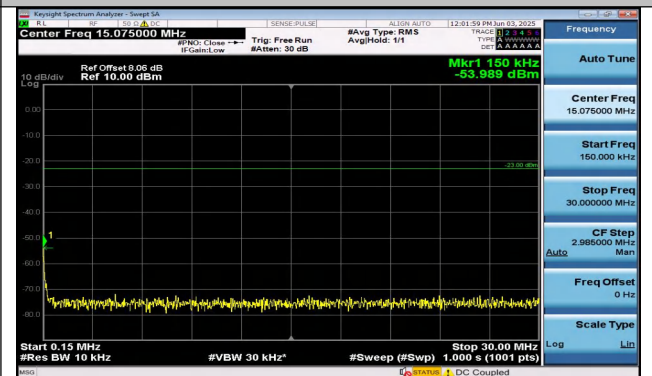
Band26(814-824)-3MHz-QPSK-26705-1RB#0-0.15~30-PA- SS
