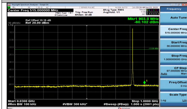
Band26(814-824)-1.4MHz-QPSK-26783-6RB#0-30~1000- PASS
