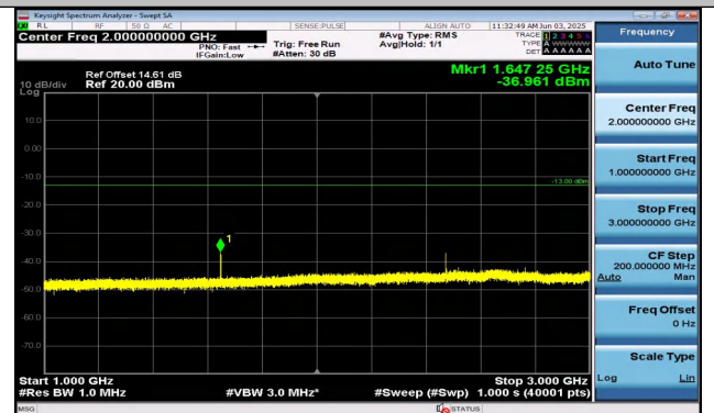
Band26(814-824)-1.4MHz-16QAM-26783-1RB#5-1000~3000-PASS
