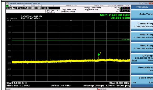
Band26(814-824)-1.4MHz-16QAM-26783-6RB#0-1000~30- 00-PASS
