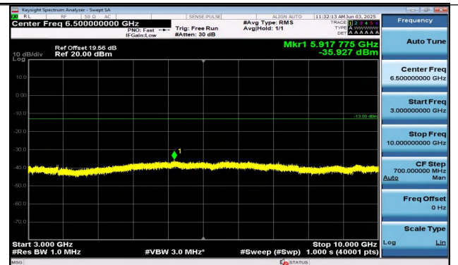
Band26(814-824)-1.4MHz-QPSK-26783-1RB#5-3000~100 00-PASS
