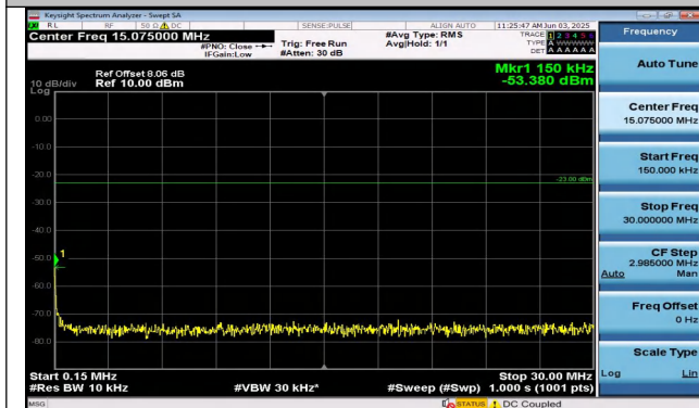
Band26(814-824)-1.4MHz-16QAM-26740-1RB#0-0.15~30- PASS
