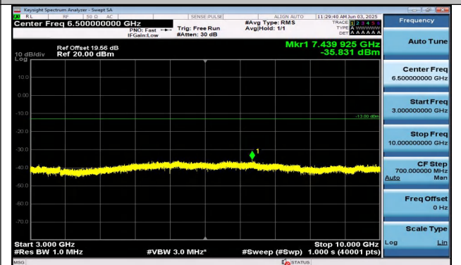
Band26(814-824)-1.4MHz-16QAM-26740-6RB#0-3000~10 000-PASS
