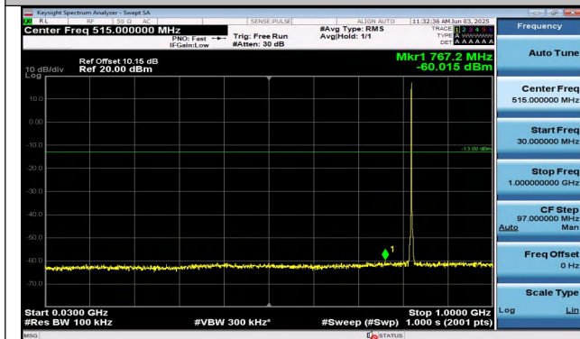
Band26(814-824)-1.4MHz-16QAM-26783-1RB#5-30~1000-PASS
