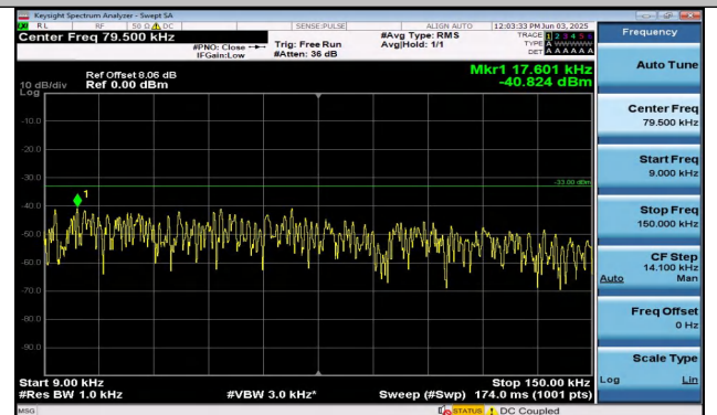
Band26(814-824)-3MHz-QPSK-26705-1RB#14-0.009~0.1 5-PASS
