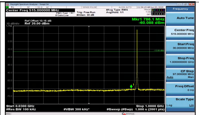
Band26(814-824)-1.4MHz-16QAM-26783-6RB#0-30~1000- -PASS
