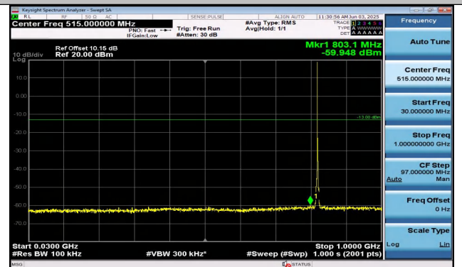
Band26(814-824)-1.4MHz-16QAM-26783-1RB#0-30~1000- -PASS
