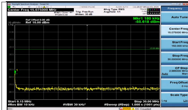
Band26(814-824)-1.4MHz-16QAM-26740-6RB#0-0.15~30- PASS
