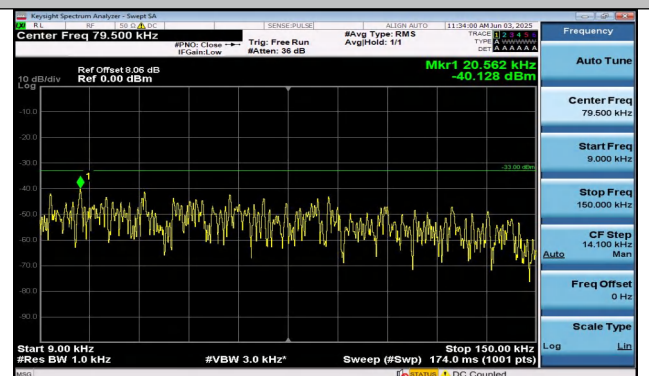
Band26(814-824)-1.4MHz-16QAM-26783-6RB#0-0.009~0.15-PASS
