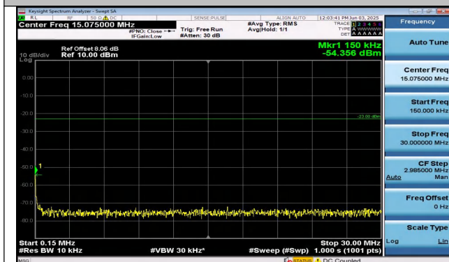
Band26(814-824)-3MHz-QPSK-26705-1RB#14-0.15~30-P ASS
