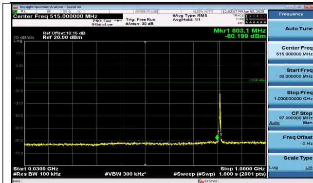
Band26(814-824)-3MHz-QPSK-26705-1RB#0-30~1000-PA SS
