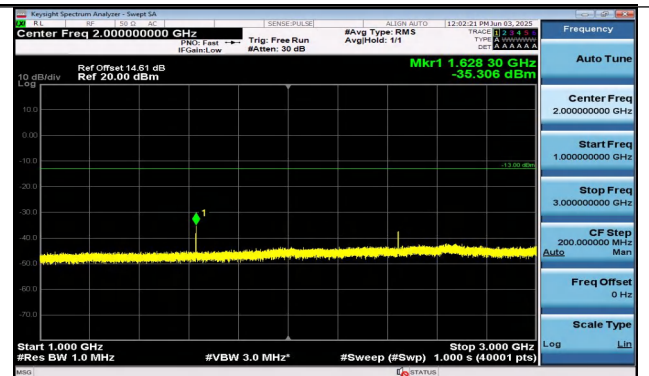
Band26(814-824)-3MHz-QPSK-26705-1RB#0-1000~3000- PASS
