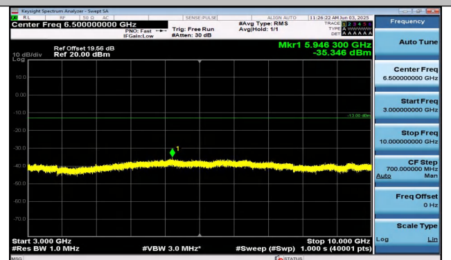
Band26(814-824)-1.4MHz-16QAM-26740-1RB#0-3000~10 000-PASS
