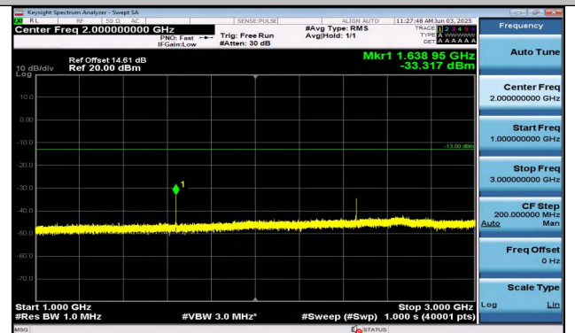
Band26(814-824)-1.4MHz-16QAM-26740-1RB#5-1000~30 00-PASS
