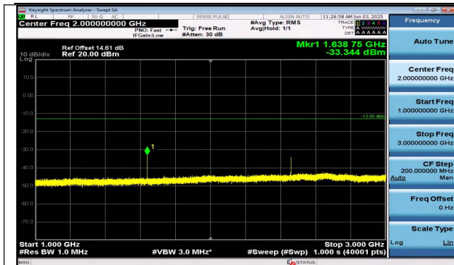
Band26(814-824)-1.4MHz-QPSK-26740-1RB#5-1000~300 0-PASS
