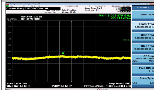
Band26(814-824)-1.4MHz-16QAM-26783-1RB#5-3000~10000-PASS
