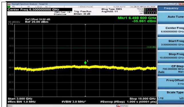
Band26(814-824)-1.4MHz-QPSK-26740-6RB#0-3000~100 00-PASS
