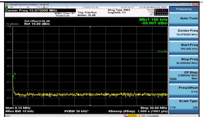
Band26(814-824)-1.4MHz-16QAM-26783-1RB#5-0.15~30-PASS
