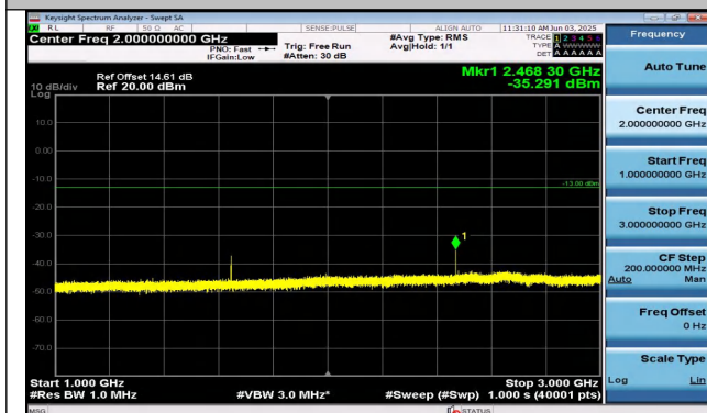
Band26(814-824)-1.4MHz-16QAM-26783-1RB#0-1000~30 00-PASS
