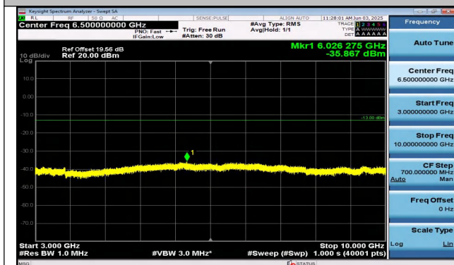
Band26(814-824)-1.4MHz-16QAM-26740-1RB#5-3000~10 000-PASS
