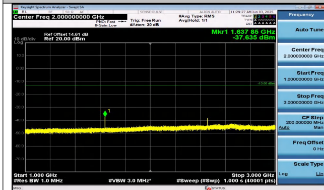
Band26(814-824)-1.4MHz-16QAM-26740-6RB#0-1000~30 00-PASS
