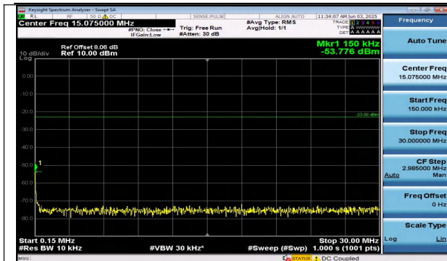
Band26(814-824)-1.4MHz-16QAM-26783-6RB#0-0.15~30- PASS
