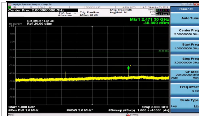
Band26(814-824)-1.4MHz-QPSK-26783-1RB#5-1000~300 0-PASS
