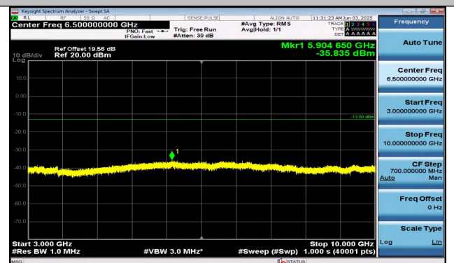
Band26(814-824)-1.4MHz-16QAM-26783-1RB#0-3000~10 000-PASS
