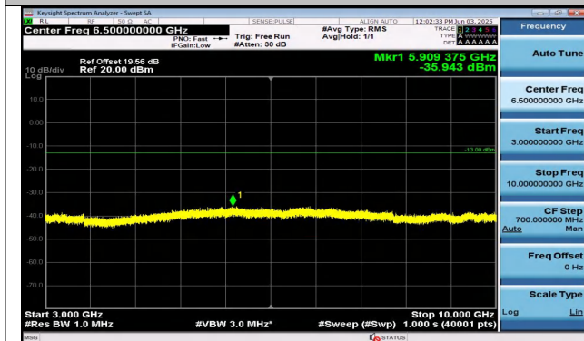
Band26(814-824)-3MHz-QPSK-26705-1RB#0-3000~10000 -PASS
