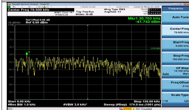
Band26(814-824)-3MHz-QPSK-26705-1RB#0-0.009~0.15- PASS
