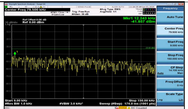
Band26(814-824)-1.4MHz-16QAM-26697-1RB#0-0.009~0. 15-PASS
