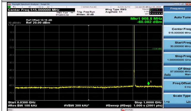
Band26(814-824)-1.4MHz-16QAM-26697-1RB#5-30~1000 -PASS
