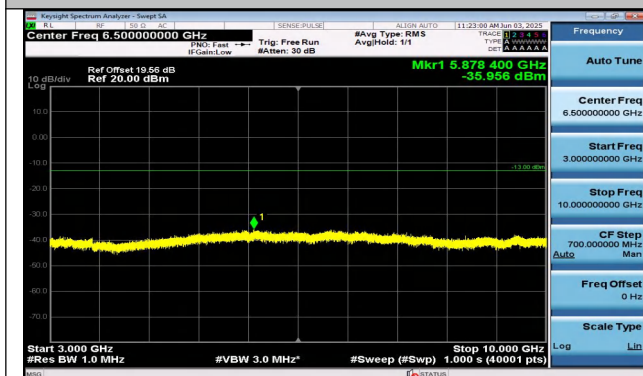
Band26(814-824)-1.4MHz-16QAM-26697-1RB#5-3000~10 000-PASS
