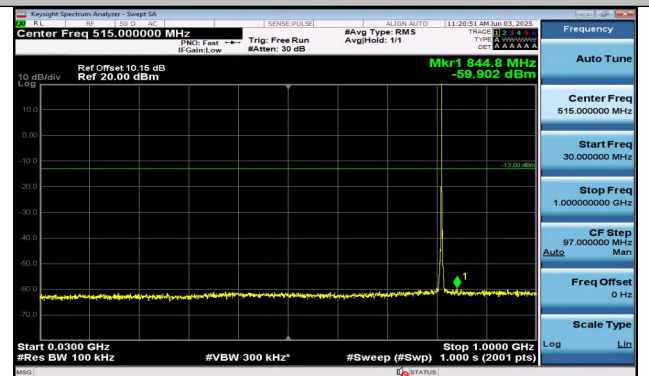
Band26(814-824)-1.4MHz-16QAM-26697-1RB#0-30~1000- -PASS
