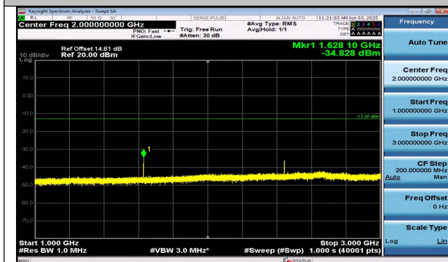
Band26(814-824)-1.4MHz-16QAM-26697-1RB#0-1000~30 00-PASS
