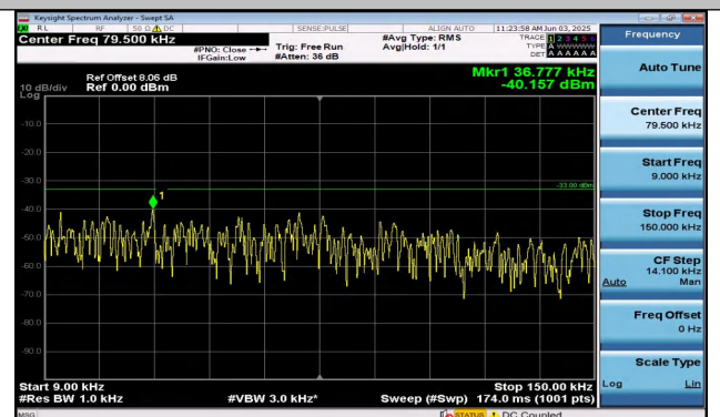
Band26(814-824)-1.4MHz-16QAM-26697-6RB#0-0.009~0. 15-PASS
