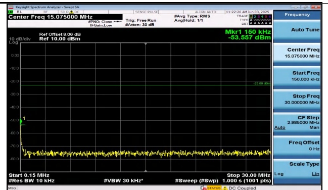
Band26(814-824)-1.4MHz-16QAM-26697-1RB#5-0.15~30 -PASS
