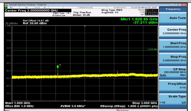
Band26(814-824)-1.4MHz-QPSK-26697-6RB#0-1000~300 0-PASS
