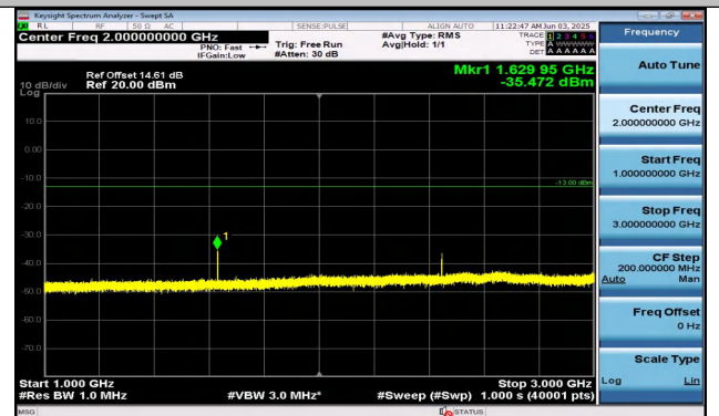
Band26(814-824)-1.4MHz-16QAM-26697-1RB#5-1000~30 00-PASS
