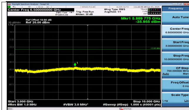
Band26(814-824)-1.4MHz-QPSK-26697-6RB#0-3000~100 00-PASS
