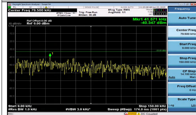
Band26(814-824)-1.4MHz-QPSK-26697-6RB#0-0.009~0.1 5-PASS
