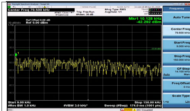
Band26(814-824)-1.4MHz-16QAM-26697-1RB#5-0.009~0. 15-PASS
