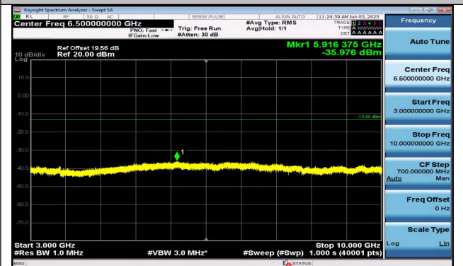
Band26(814-824)-1.4MHz-16QAM-26697-6RB#0-3000~10 000-PASS
