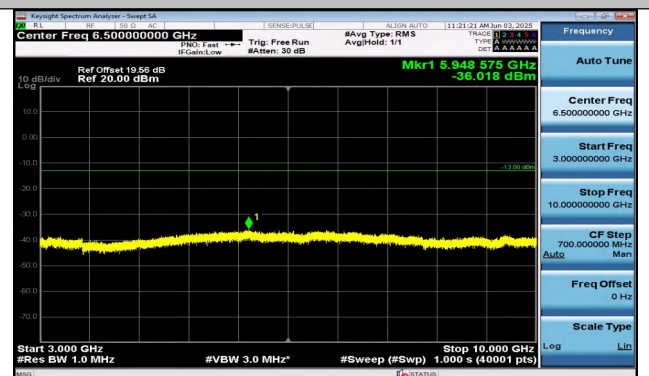
Band26(814-824)-1.4MHz-16QAM-26697-1RB#0-3000~10 000-PASS
