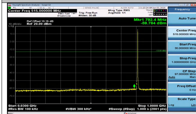
Band26(814-824)-1.4MHz-QPSK-26697-6RB#0-30~1000- PASS
