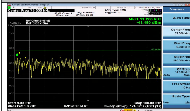
Band26(814-824)-1.4MHz-QPSK-26740-1RB#0-0.009~0.1 5-PASS
