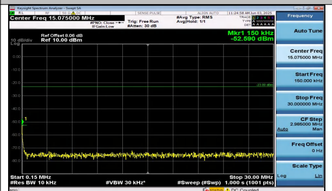
Band26(814-824)-1.4MHz-QPSK-26740-1RB#0-0.15~30- PASS
