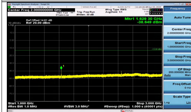
Band26(814-824)-1.4MHz-16QAM-26697-6RB#0-1000~30 00-PASS
