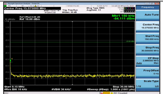
Band26(814-824)-1.4MHz-QPSK-26697-6RB#0-0.15~30- PASS
