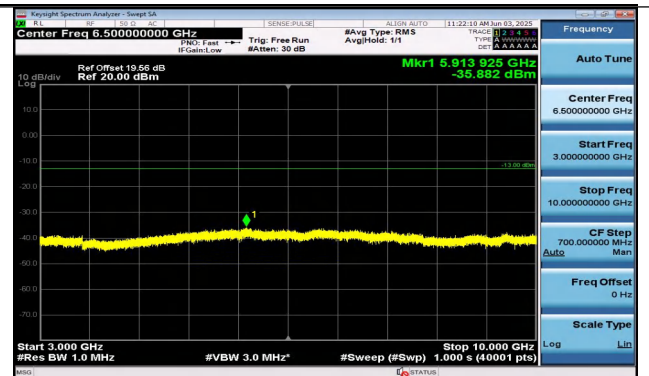
Band26(814-824)-1.4MHz-QPSK-26697-1RB#5-3000~100 00-PASS
