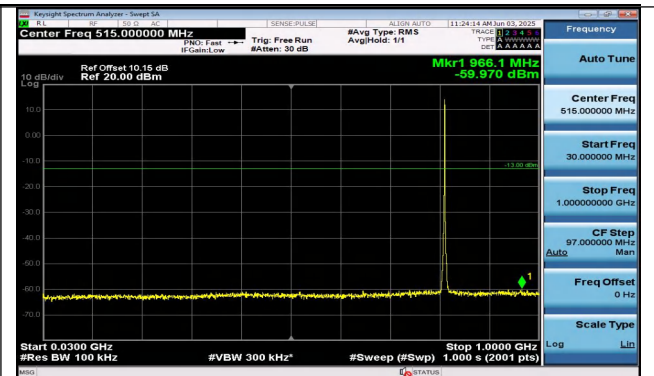
Band26(814-824)-1.4MHz-16QAM-26697-6RB#0-30~1000 -PASS
