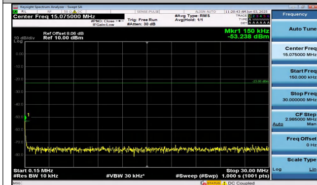
Band26(814-824)-1.4MHz-16QAM-26697-1RB#0-0.15~30- PASS
