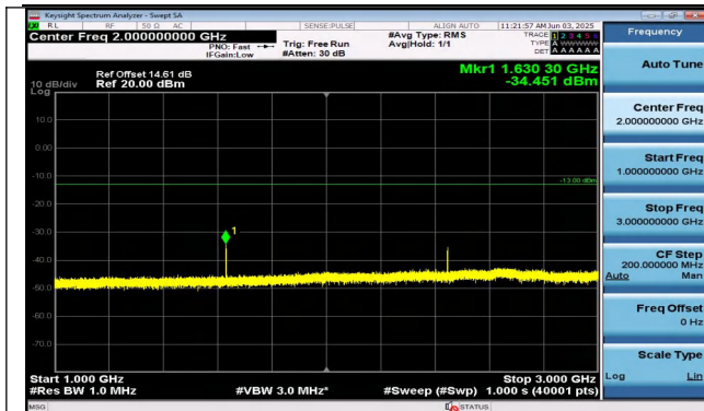
Band26(814-824)-1.4MHz-QPSK-26697-1RB#5-1000~300 0-PASS
