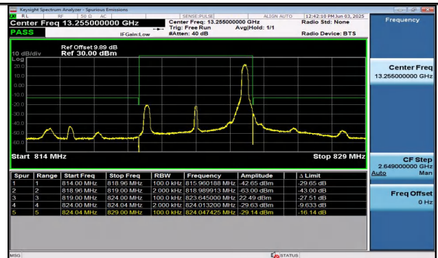
Band26(814-824)-5MHz-QPSK-26765-1RB#24-PASS
