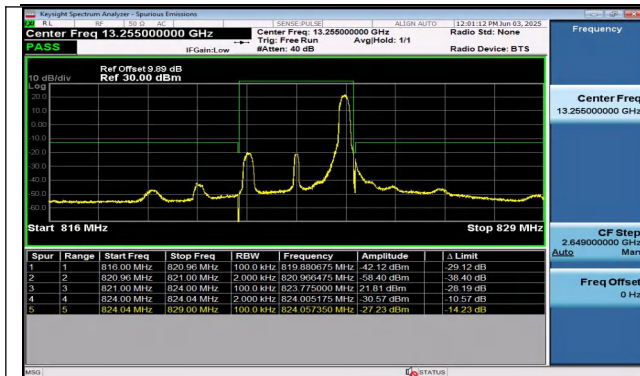
Band26(814-824)-3MHz-16QAM-26775-1RB#14-PASS
