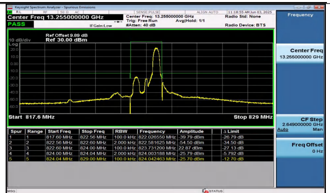
Band26(814-824)-1.4MHz-QPSK-26783-1RB#5-PASS
