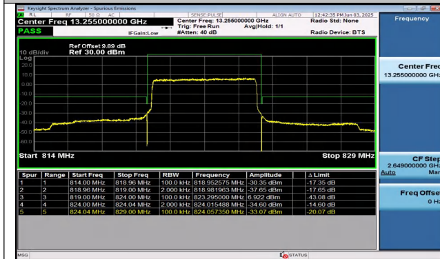
Band26(814-824)-5MHz-QPSK-26765-25RB#0-PASS
