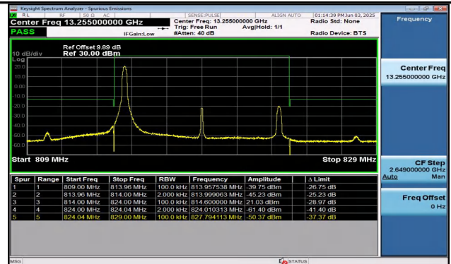
Band26(814-824)-10MHz-16QAM-26740-1RB#0-PASS
