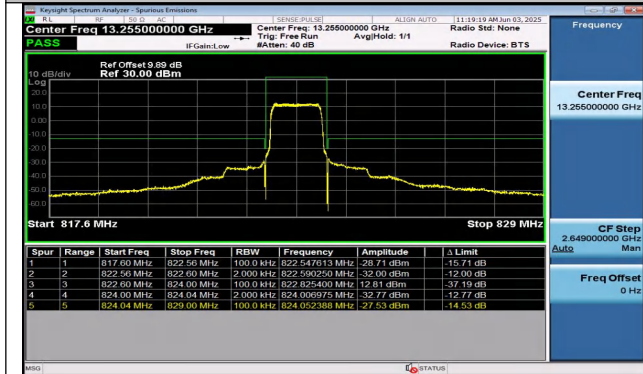
Band26(814-824)-1.4MHz-QPSK-26783-6RB#0-PASS
