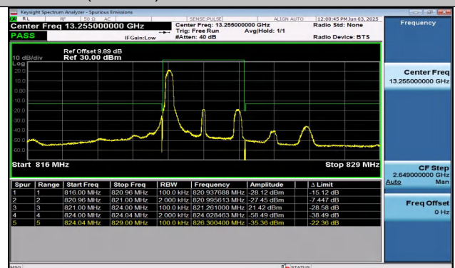
Band26(814-824)-3MHz-16QAM-26775-1RB#0-PASS
