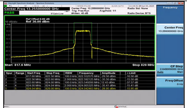
Band26(814-824)-1.4MHz-16QAM-26783-6RB#0-PASS
