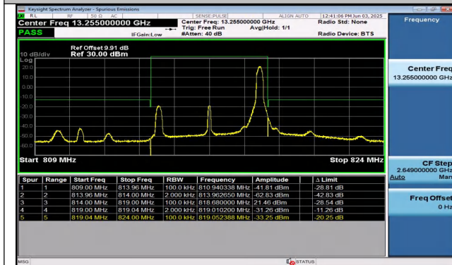
Band26(814-824)-5MHz-16QAM-26715-1RB#24-PASS
