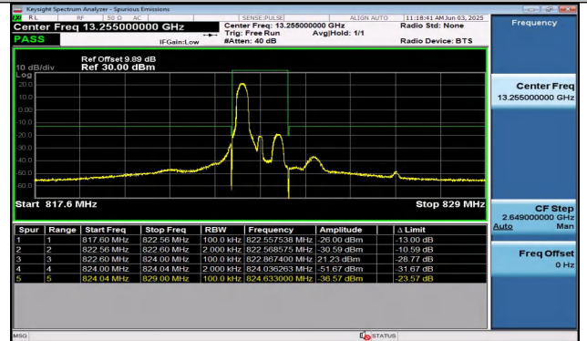
Band26(814-824)-1.4MHz-16QAM-26783-1RB#0-PASS
