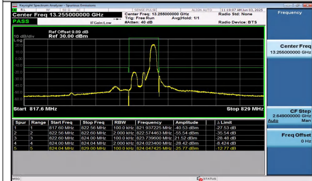
Band26(814-824)-1.4MHz-16QAM-26783-1RB#5-PASS
