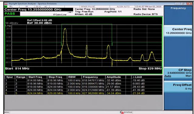
Band26(814-824)-5MHz-16QAM-26765-1RB#0-PASS
