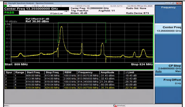
Band26(814-824)-5MHz-16QAM-26715-1RB#0-PASS
