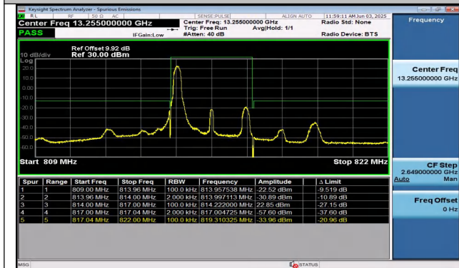
Band26(814-824)-3MHz-QPSK-26705-1RB#0-PASS
