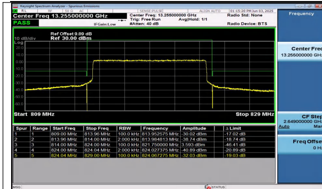
Band26(814-824)-10MHz-QPSK-26740-50RB#0-PASS
