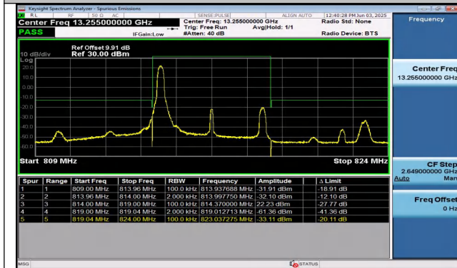
Band26(814-824)-5MHz-QPSK-26715-1RB#0-PASS
