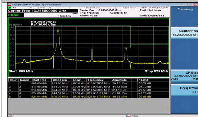
Band26(814-824)-10MHz-QPSK-26740-1RB#0-PASS
