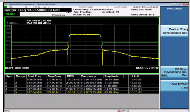
Band26(814-824)-3MHz-16QAM-26705-15RB#0-PASS
