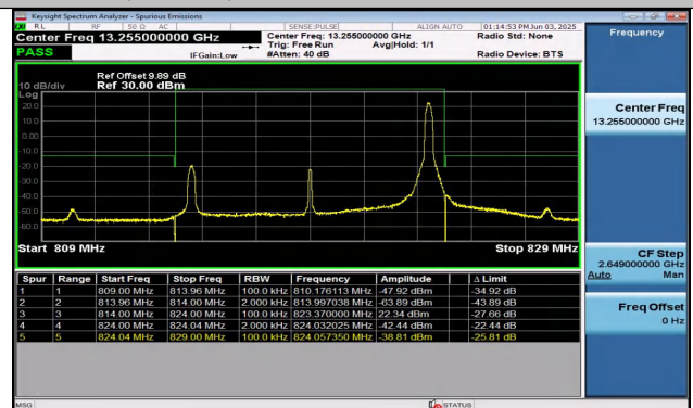
Band26(814-824)-10MHz-QPSK-26740-1RB#49-PASS
