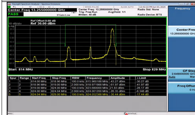
Band26(814-824)-5MHz-16QAM-26765-1RB#24-PASS
