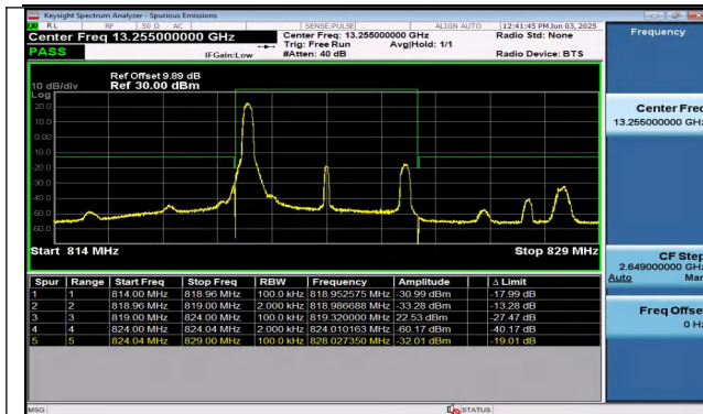
Band26(814-824)-5MHz-QPSK-26765-1RB#0-PASS
