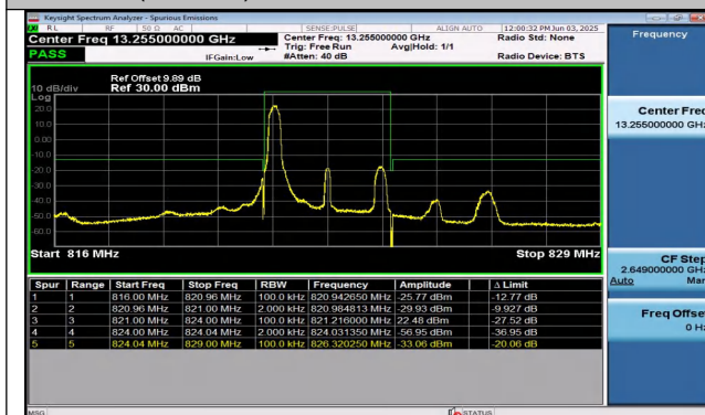
Band26(814-824)-3MHz-QPSK-26775-1RB#0-PASS
