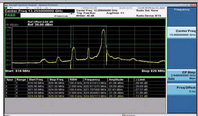
Band26(814-824)-3MHz-QPSK-26775-1RB#14-PASS
