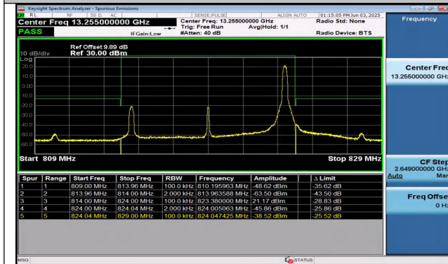
Band26(814-824)-10MHz-16QAM-26740-1RB#49-PASS
