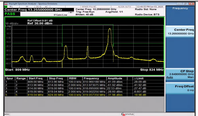
Band26(814-824)-5MHz-QPSK-26715-15RB#24-PASS
