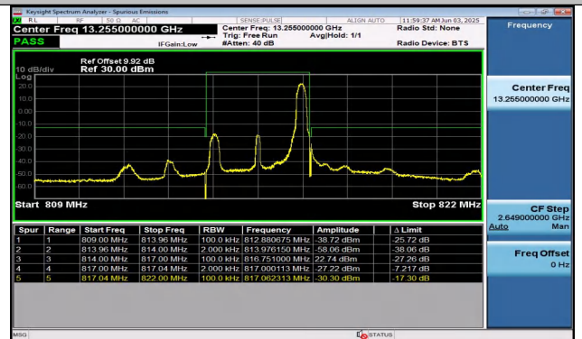
Band26(814-824)-3MHz-QPSK-26705-1RB#14-PASS
