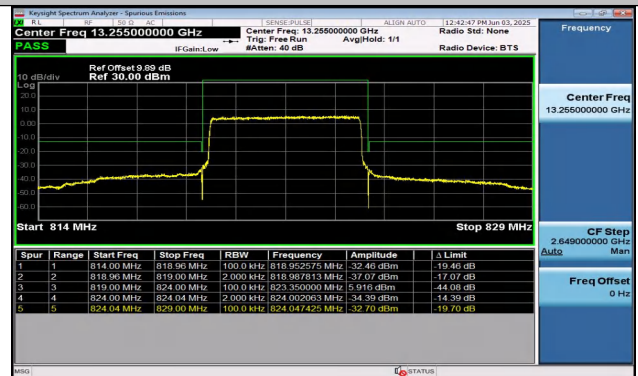
Band26(814-824)-5MHz-16QAM-26765-25RB#0-PASS
