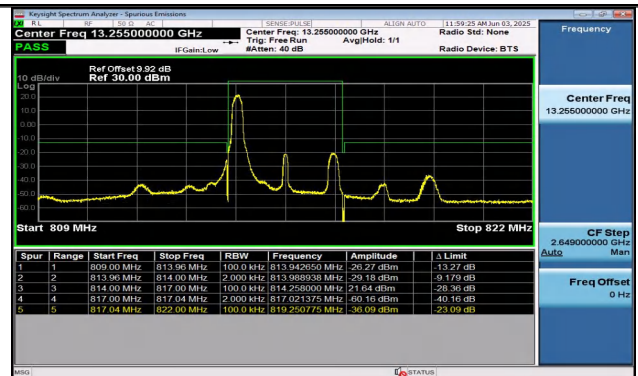
Band26(814-824)-3MHz-16QAM-26705-1RB#0-PASS
