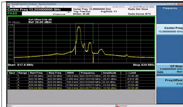
Band26(814-824)-1.4MHz-QPSK-26783-1RB#0-PASS
