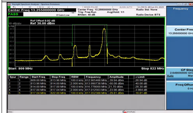
Band26(814-824)-3MHz-16QAM-26705-1RB#14-PASS
