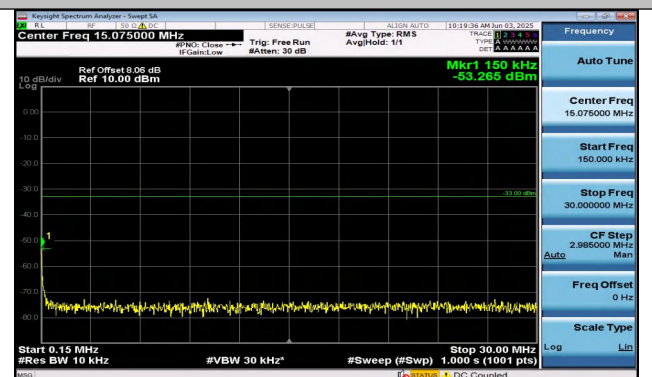
Band25-15MHz-QPSK-26615-1RB#74-0.15~30-PASS
