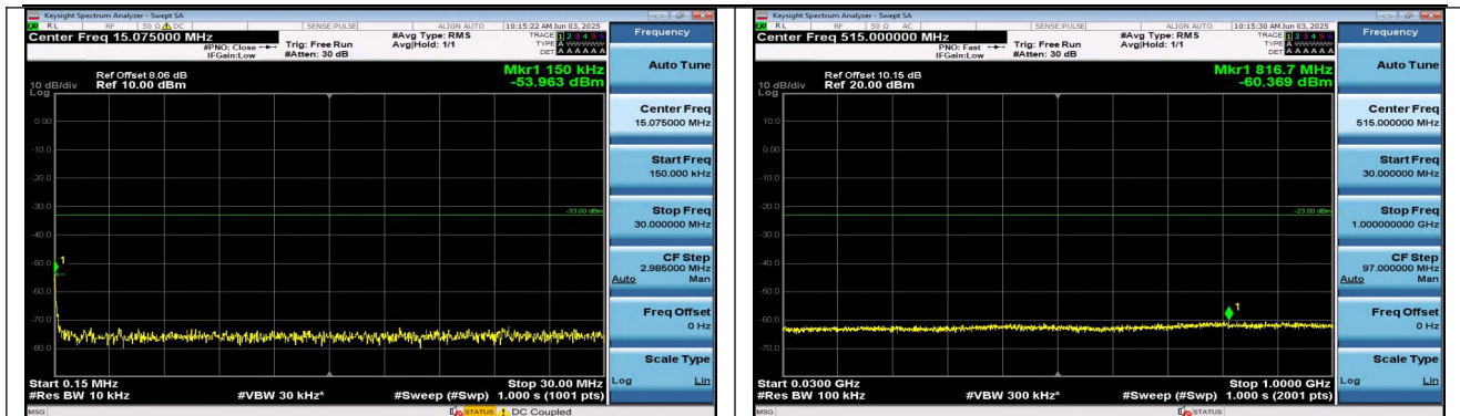
Band25-15MHz-16QAM-26365-1RB#0-0.15~30-PASS
