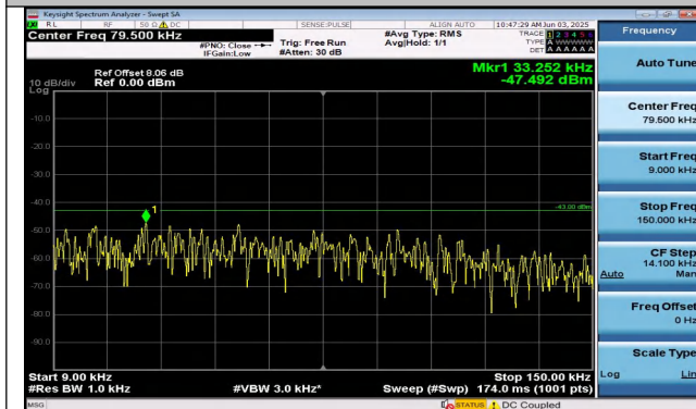
Band25-20MHz-16QAM-26140-1RB#99-0.009~0.15-PASS
