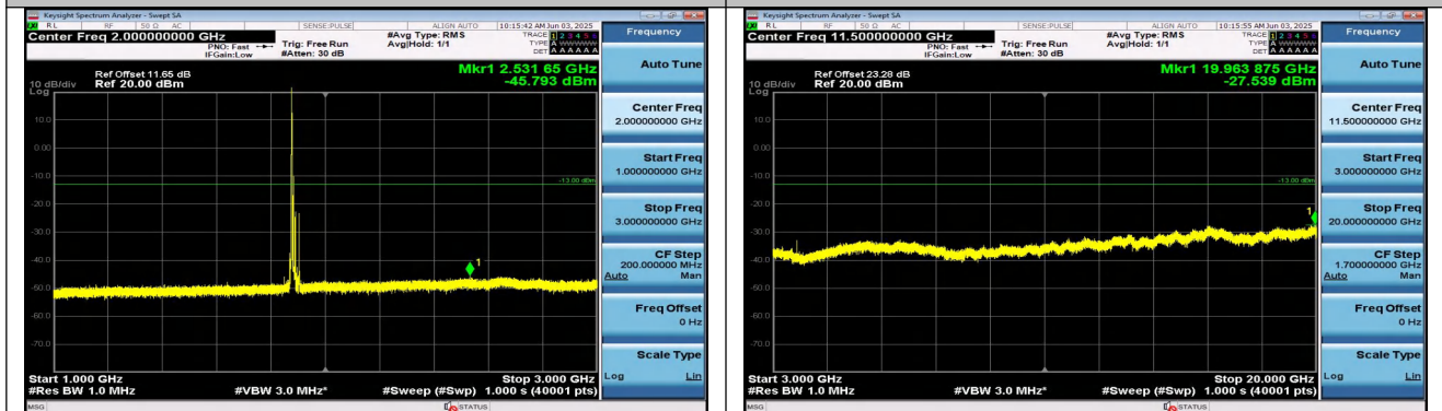
Band25-15MHz-16QAM-26365-1RB#0-1000~3000-PASS
