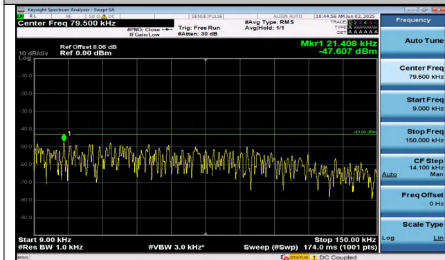
Band25-20MHz-QPSK-26140-1RB#0-0.009~0.15-PASS
