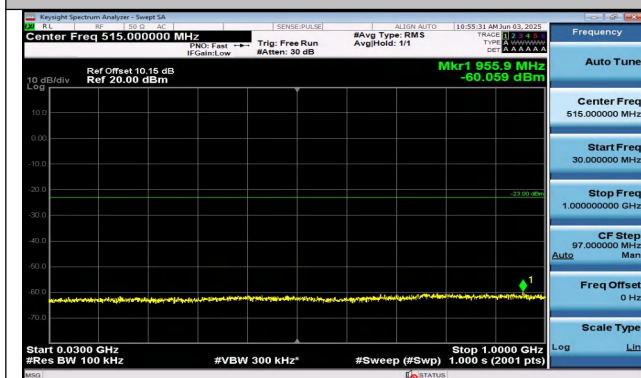
Band25-20MHz-QPSK-26140-100RB#0-30~1000-PASS
