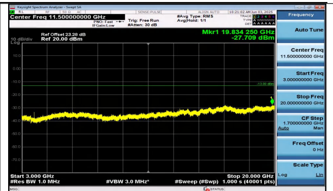
Band25-15MHz-16QAM-26615-1RB#74-3000~20000-PAS S
