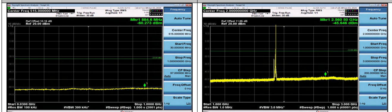
Band25-15MHz-16QAM-26365-1RB#74-30~1000-PASS
