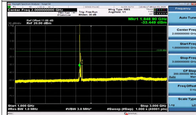
Band25-20MHz-16QAM-26140-1RB#0-1000~3000-PASS
