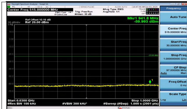
Band25-20MHz-16QAM-26140-1RB#99-30~1000-PASS
