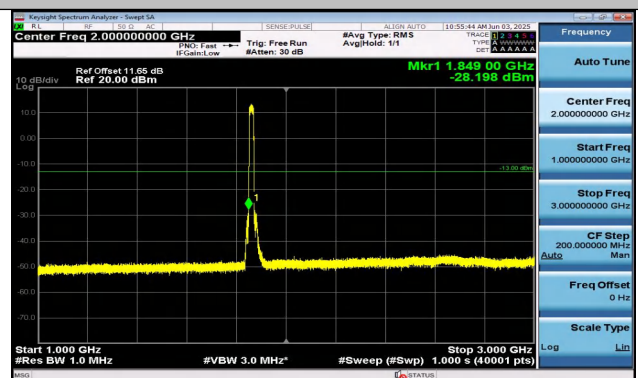
Band25-20MHz-QPSK-26140-100RB#0-1000~3000-PASS
