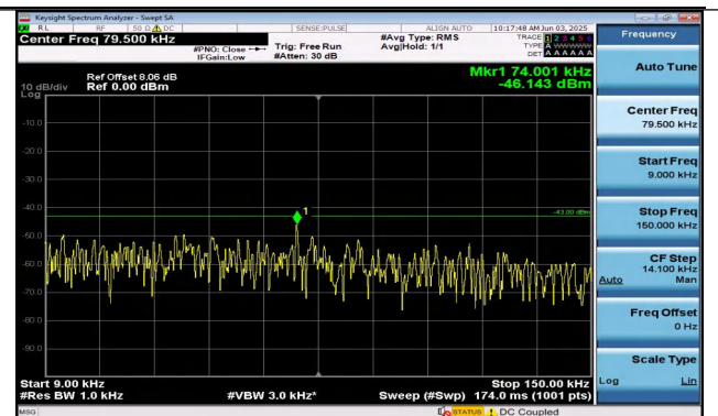
Band25-15MHz-QPSK-26615-1RB#0-0.009~0.15-PASS
