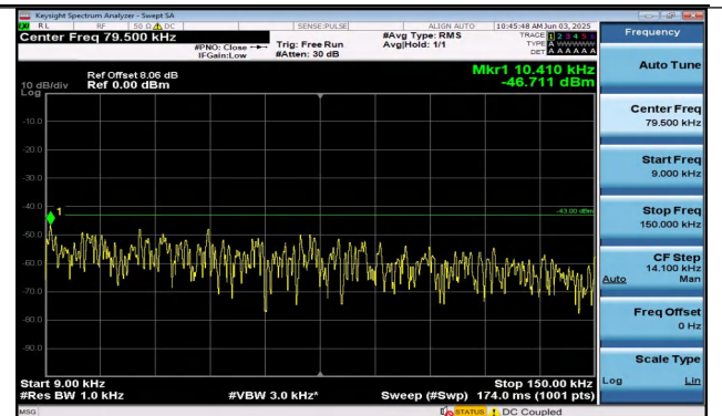
Band25-20MHz-16QAM-26140-1RB#0-0.009~0.15-PASS
