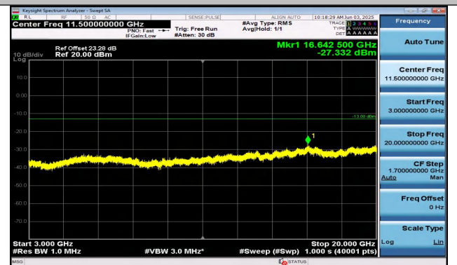
Band25-15MHz-QPSK-26615-1RB#0-3000~20000-PASS
