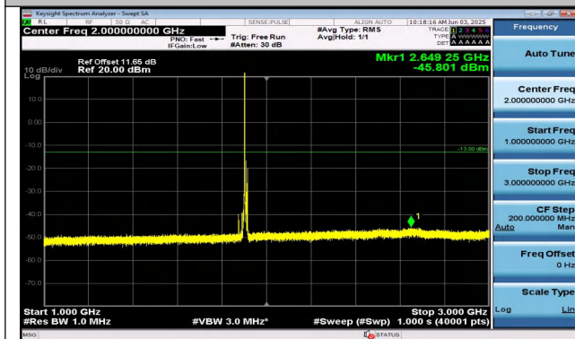
Band25-15MHz-QPSK-26615-1RB#0-1000~3000-PASS
