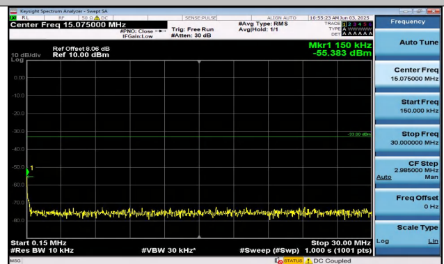
Band25-20MHz-QPSK-26140-100RB#0-0.15~30-PASS
