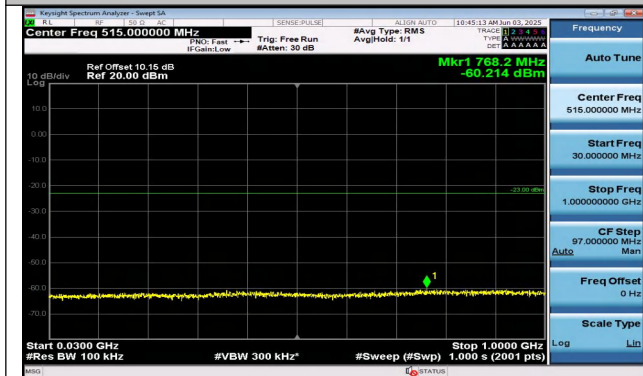
Band25-20MHz-QPSK-26140-1RB#0-30~1000-PASS
