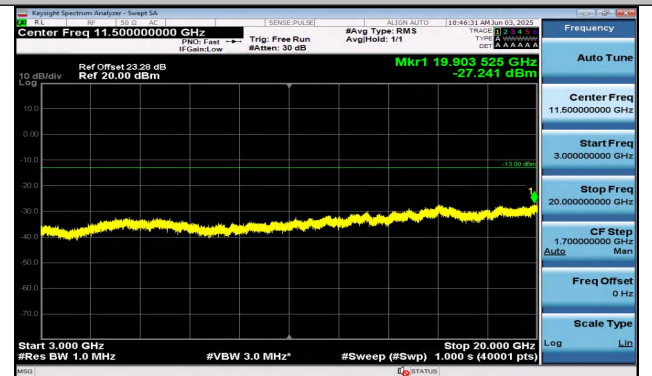
Band25-20MHz-16QAM-26140-1RB#0-3000~20000-PASS
