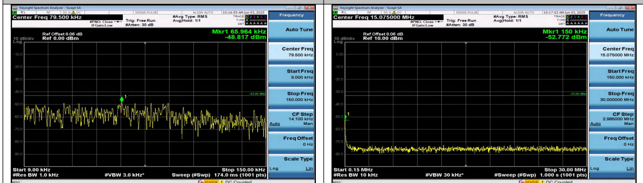
Band25-15MHz-16QAM-26365-1RB#74-0.009~0.15-PASS
