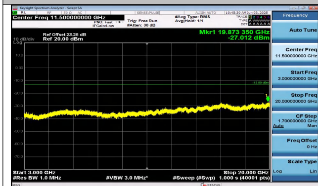
Band25-20MHz-QPSK-26140-1RB#0-3000~20000-PASS
