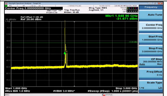
Band25-20MHz-QPSK-26140-1RB#0-1000~3000-PASS
