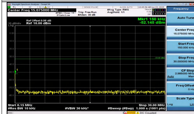
Band25-20MHz-16QAM-26140-1RB#0-0.15~30-PASS
