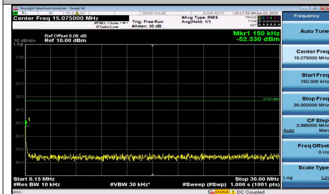
Band25-15MHz-QPSK-26615-1RB#0-0.15~30-PASS
