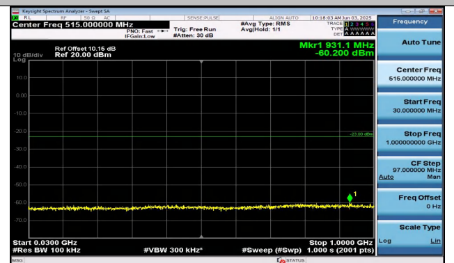
Band25-15MHz-QPSK-26615-1RB#0-30~1000-PASS
