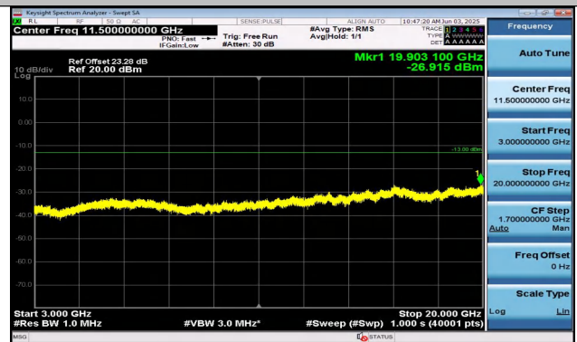
Band25-20MHz-QPSK-26140-1RB#99-3000~20000-PASS
