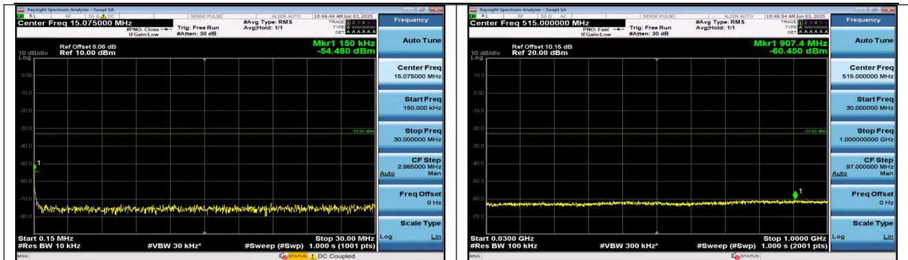
Band25-20MHz-QPSK-26140-1RB#99-0.15~30-PASS
