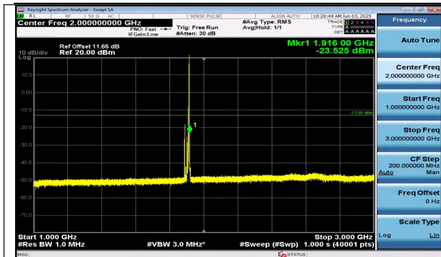
Band25-15MHz-16QAM-26615-1RB#74-1000~3000-PASS
