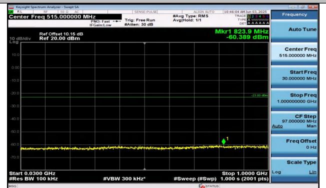
Band25-20MHz-16QAM-26140-1RB#0-30~1000-PASS
