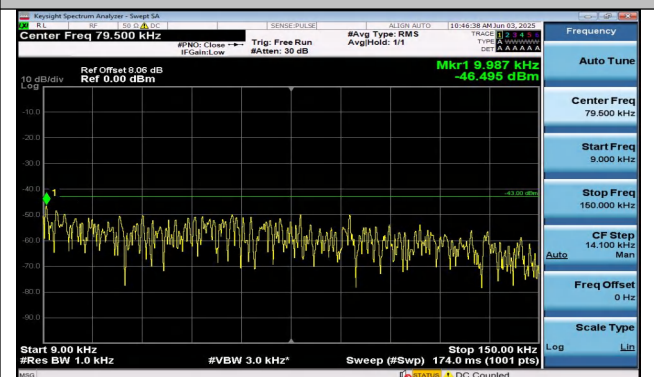
Band25-20MHz-QPSK-26140-1RB#99-0.009~0.15-PASS
