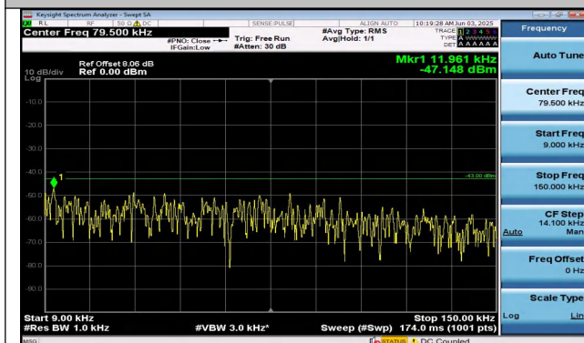
Band25-15MHz-QPSK-26615-1RB#74-0.009~0.15-PASS
