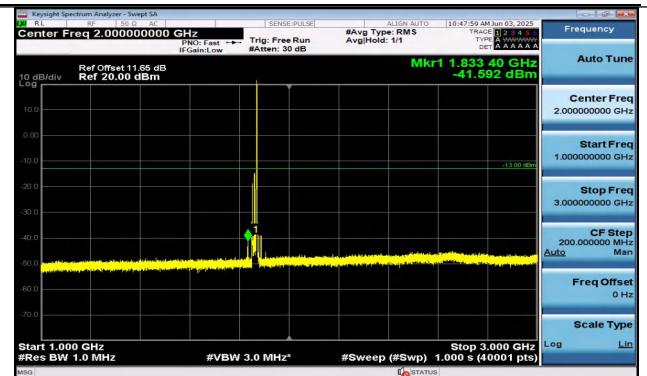
Band25-20MHz-16QAM-26140-1RB#99-1000~3000-PASS
