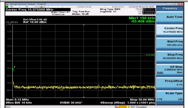
Band25-20MHz-QPSK-26140-1RB#0-0.15~30-PASS
